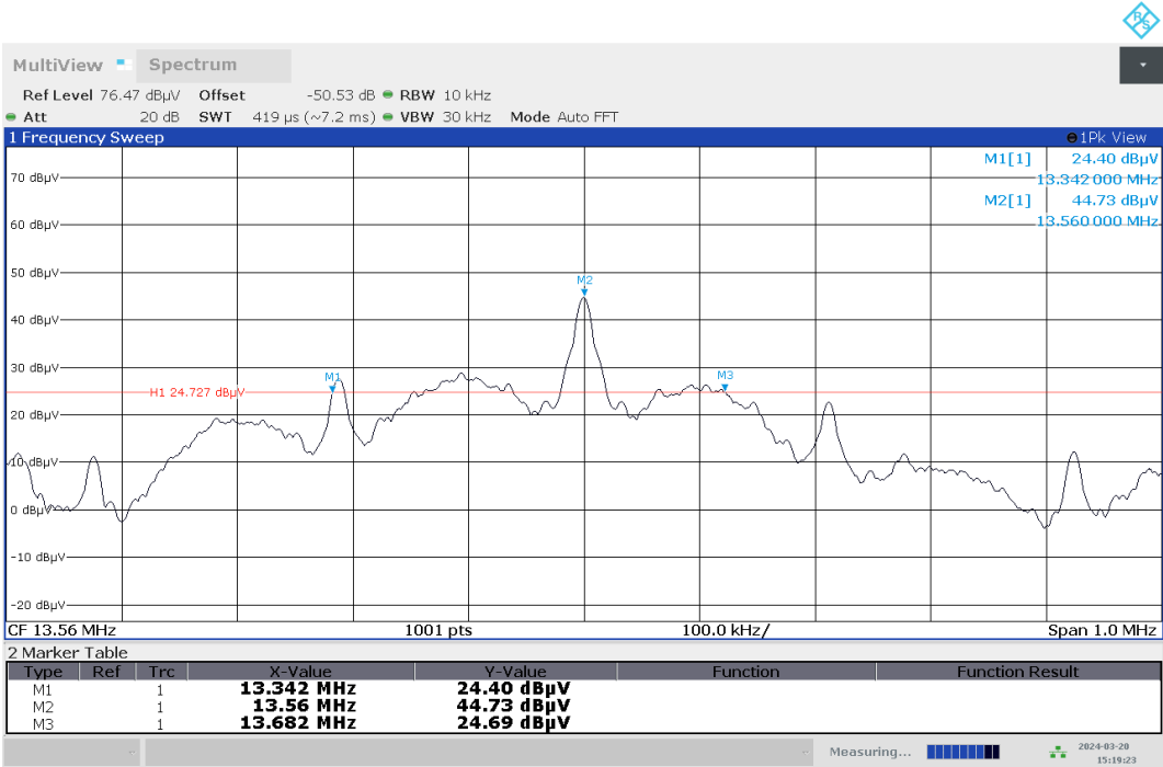
Plot No. 20: 20 dB bandwidth
