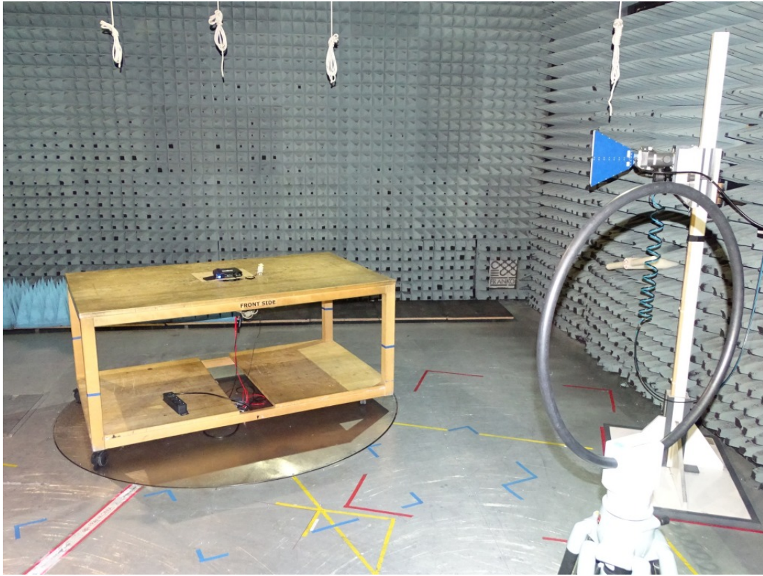
Photo 1: Test setup for radiated measurements (Enclosure, semi-anechoic chamber, H-Field)
