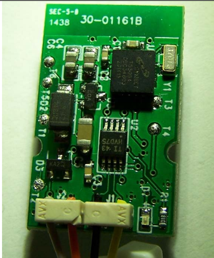
Main Board Component Side
