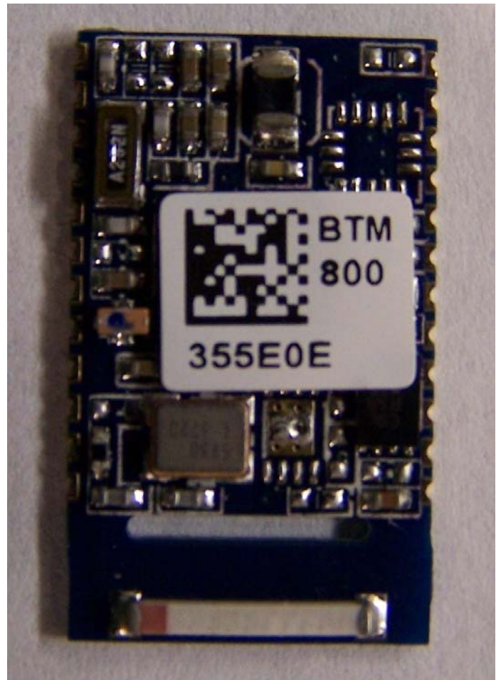
Radio Module Back and Top
