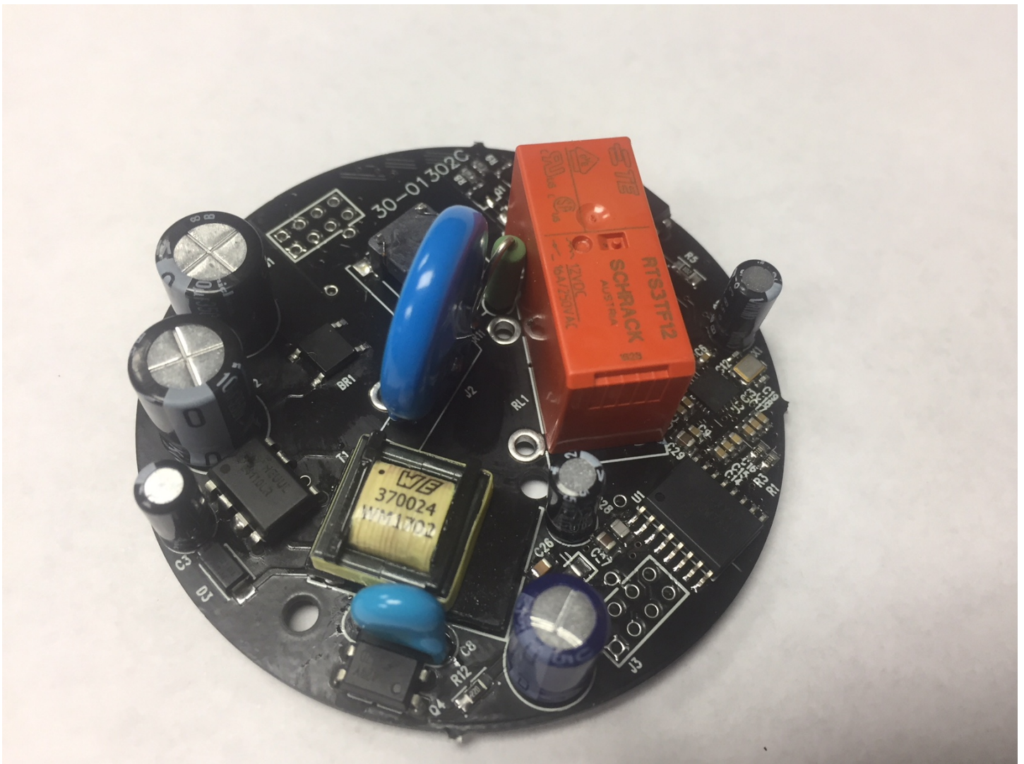
Board 1 Top; power board
