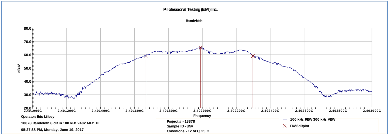
6 dB, Low Channel
