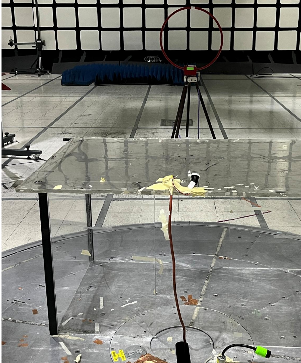
Radiated Emissions (9kHz – 30MHz)
