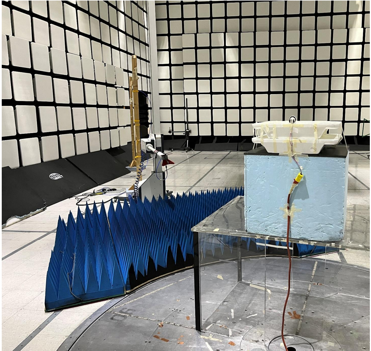
Radiated Emissions Above 1GHz
