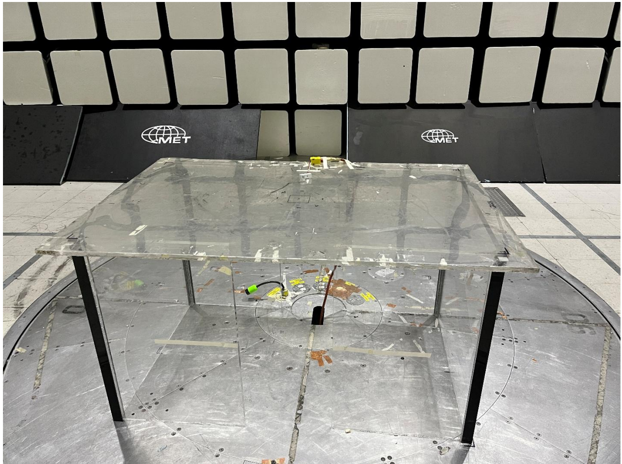
Radiated Emissions (Front Side Below 1GHz)
