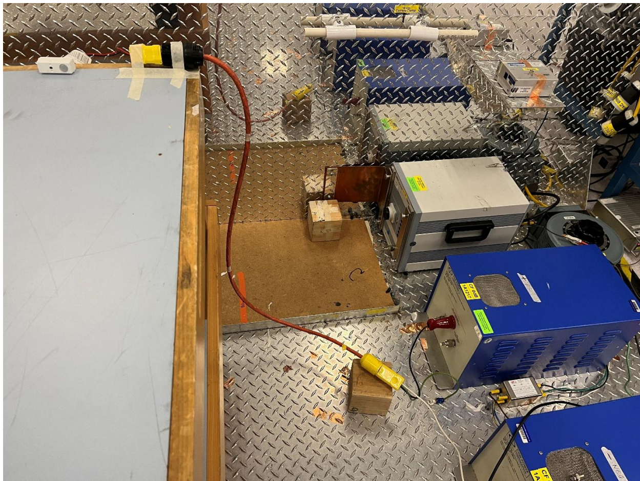
Conducted Emissions at Mains Terminals
