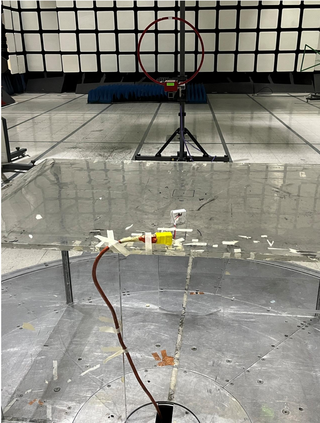
Radiated Emissions 9kHz – 30MHz
