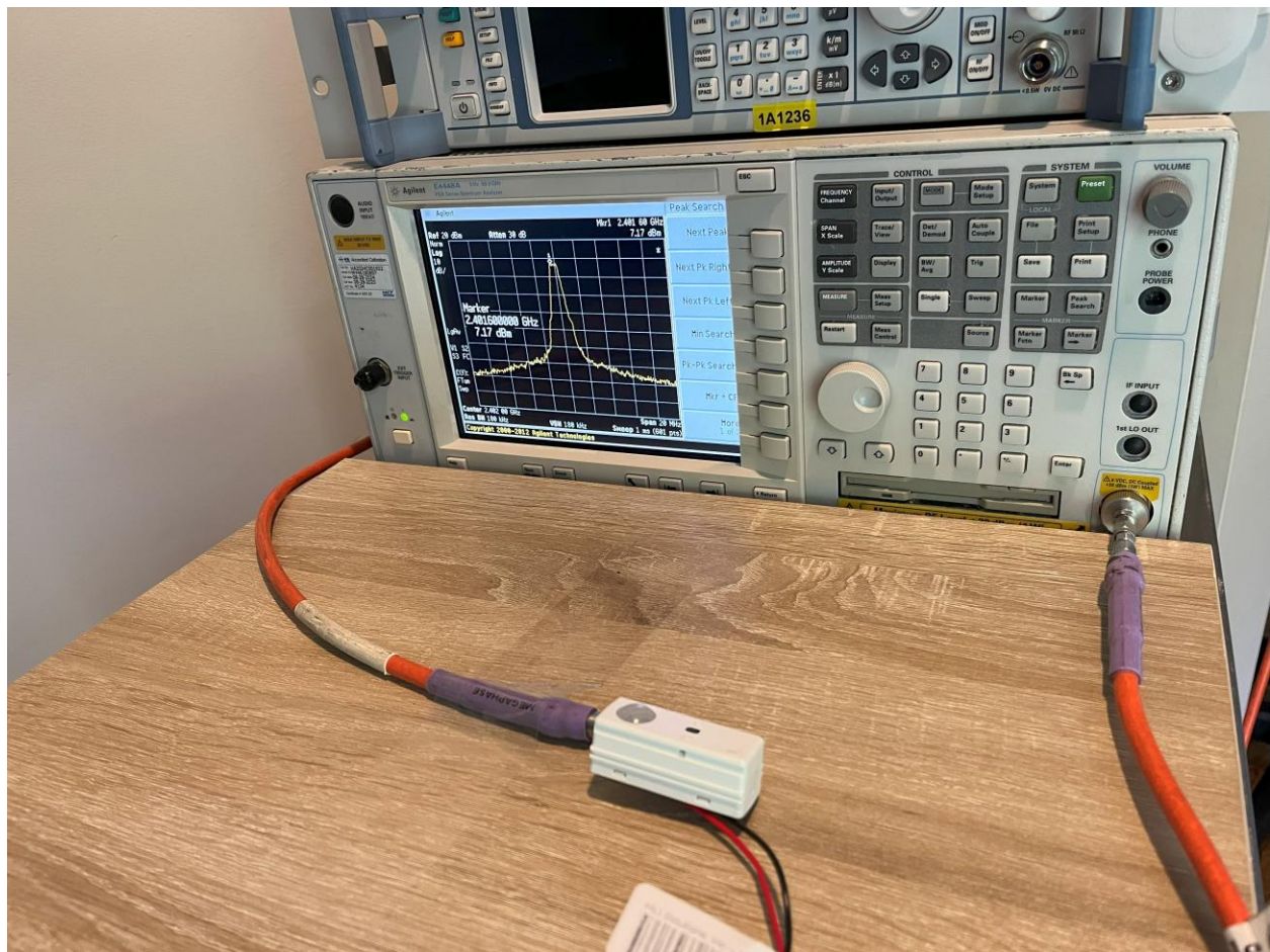
Conducted Measurements at Antenna Terminals
