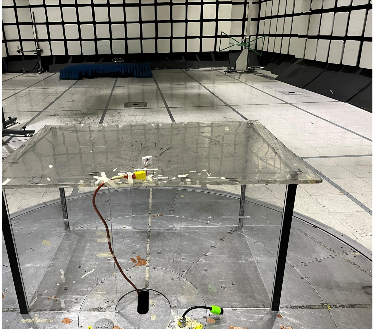
Radiated Emissions 30MHz – 1GHz
