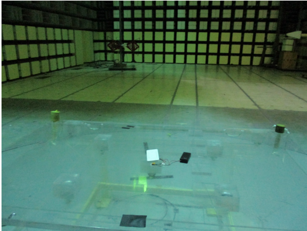
Radiated Emissions to 1 GHz
