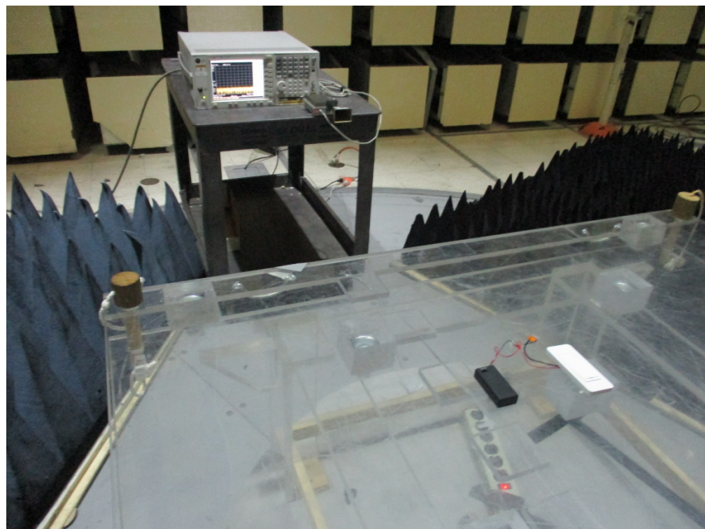
Spurious Emissions to 26.5GHz
