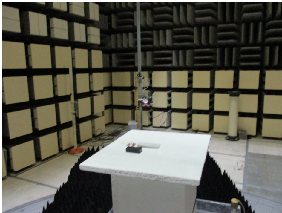
Radiated Output Power, Spurious Emissions to 18GHz
