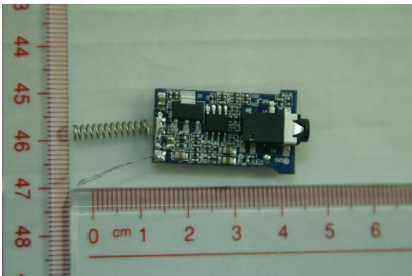
MAIN BOARD BACK VIEW 1
