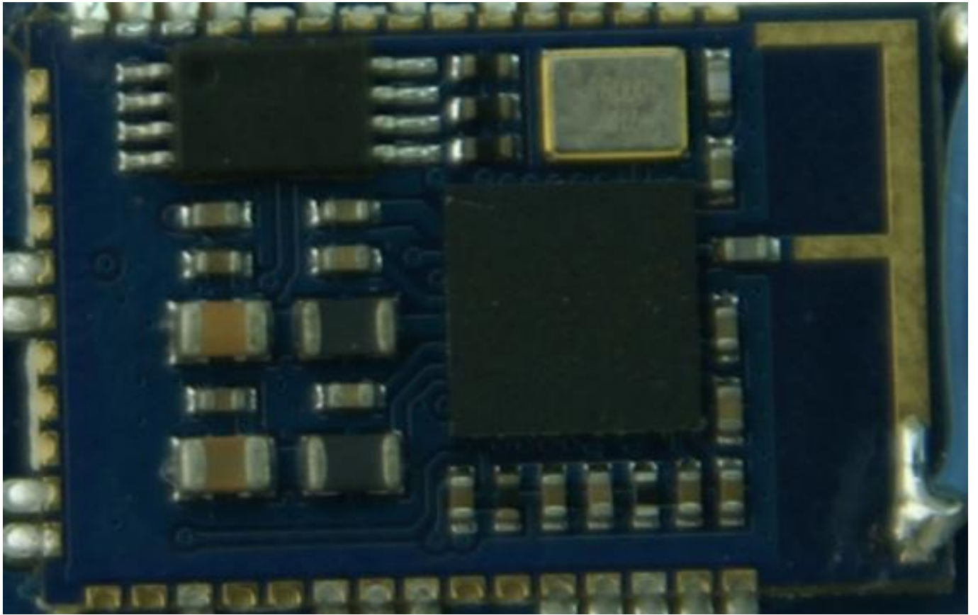
RF BOARD TOP VIEW
