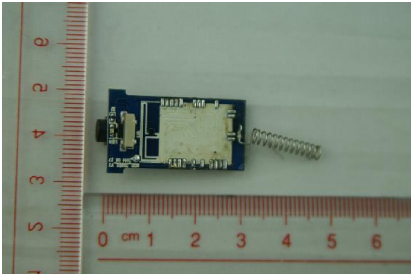
MAIN BOARD TOP VIEW 1-1
