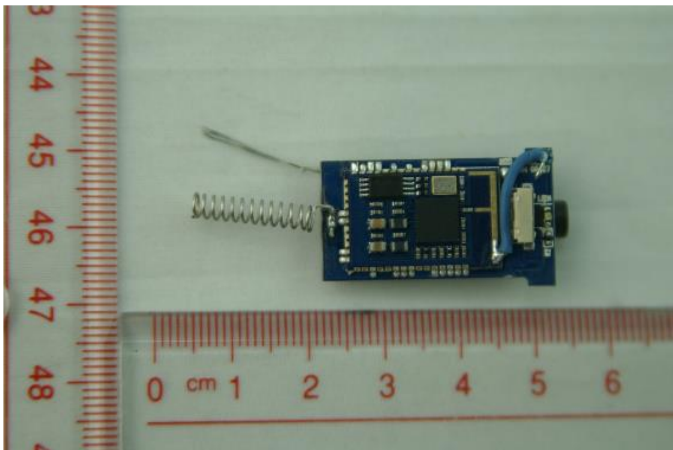
MAIN BOARD TOP VIEW 1
