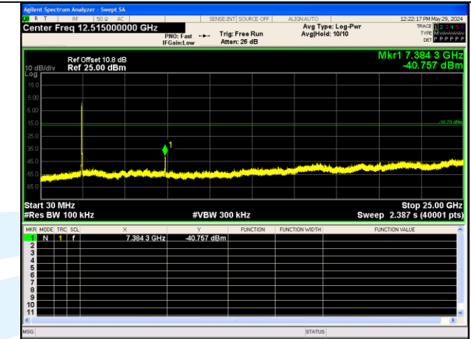
30.0 MHz - 25000.0 MHz IEEE 802.11n Channel 11 20MHz Antenna 0
