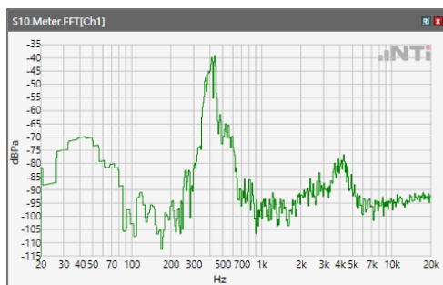
ANSI/TIA 5050-2018 \ 2N HAC ON \ WB 23.85 kbps\ 5.2 Receive path – distortion and noise\ LTE Band 28
