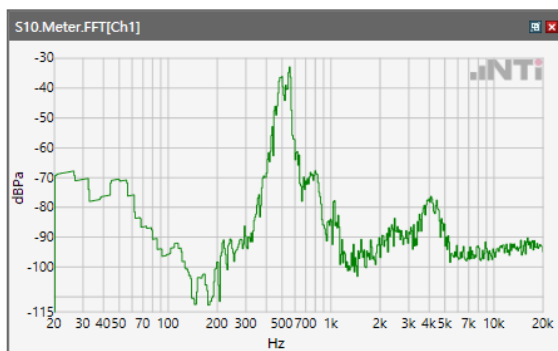
ANSI/TIA 5050-2018 \ 2N HAC ON \ WB 23.85 kbps\ 5.2 Receive path – distortion and noise\ LTE Band 2
