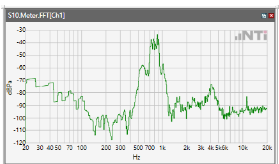
ANSI/TIA 5050-2018 \ 2N HAC ON \ WB 23.85 kbps\ 5.2 Receive path – distortion and noise\ LTE Band 28
