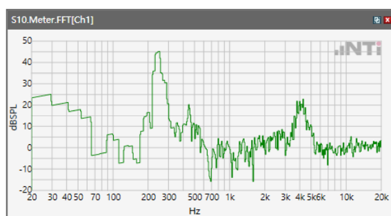
ANSI/TIA 5050-2018 \ 2N HAC ON \ WB 23.85 kbps\ 5.2 Receive path – distortion and noise\ WLAN 5.3GHz
