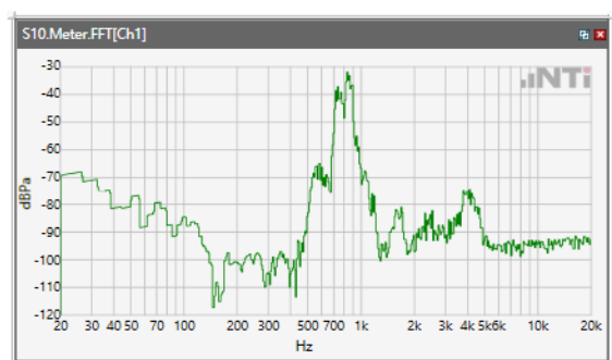
ANSI/TIA 5050-2018 \ 2N HAC ON \ WB 23.85 kbps\ 5.2 Receive path – distortion and noise\ LTE Band 13
