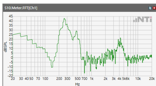
ANSI/TIA 5050-2018 \ 2N HAC ON \ WB 23.85 kbps\ 5.2 Receive path – distortion and noise\ WLAN 5.2GHz
