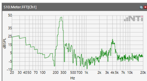
ANSI/TIA 5050-2018 \ 2N HAC ON \ WB 23.85 kbps\ 5.2 Receive path – distortion and noise\ LTE Band 13
