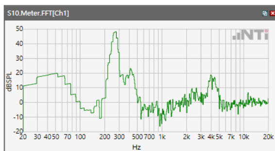
ANSI/TIA 5050-2018 \ 2N HAC ON \ WB 23.85 kbps\ 5.2 Receive path – distortion and noise\ LTE Band 28
