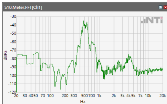
ANSI/TIA 5050-2018 \ 2N HAC ON \ WB 23.85 kbps\ 5.2 Receive path – distortion and noise\ LTE Band 5
