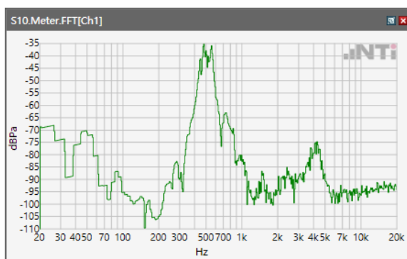
ANSI/TIA 5050-2018 \ 2N HAC ON \ WB 23.85 kbps\ 5.2 Receive path – distortion and noise\ WCDMA V
