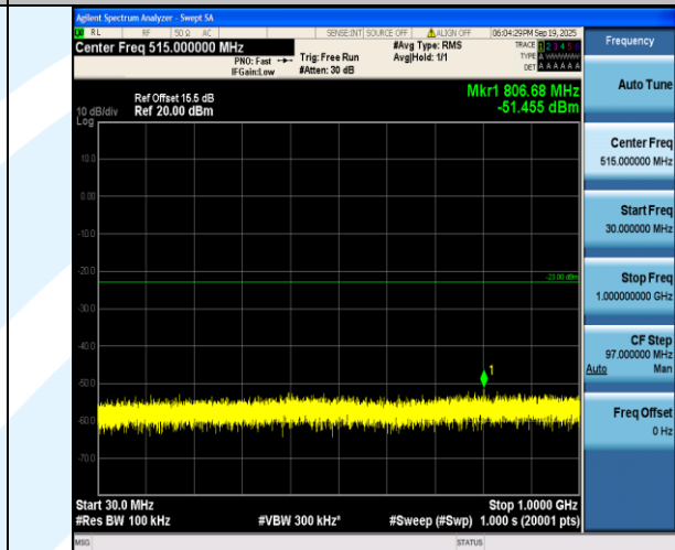
Band4-15MHz-16QAM-20325-1RB#0-30~1000-PASS
