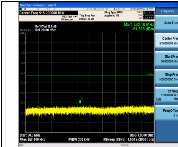
Band4-15MHz-16QAM-20175-1RB#0-30~1000-PASS
