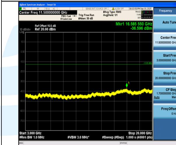
Band4-15MHz-16QAM-20175-1RB#0-3000~20000-PASS
