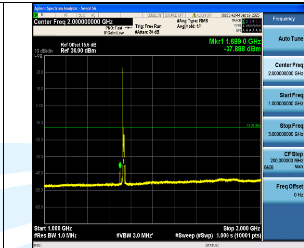
Band4-15MHz-16QAM-20175-1RB#0-1000~3000-PASS
