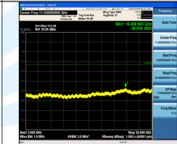
Band4-15MHz-16QAM-20325-1RB#0-3000~20000-PASS
