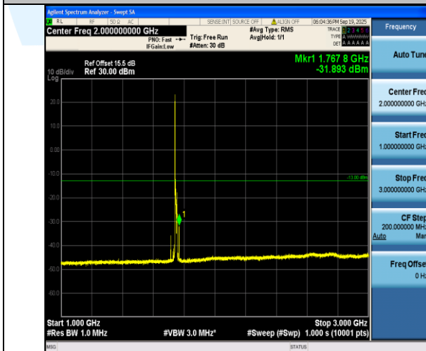
Band4-15MHz-16QAM-20325-1RB#0-1000~3000-PASS
