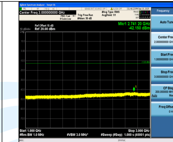
Band5-1.4MHz-QPSK-20643-1RB#0-1000~3000-PASS
