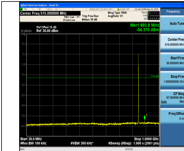
Band5-1.4MHz-QPSK-20643-1RB#0-30~1000-PASS
