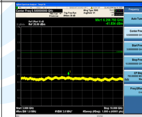
Band5-1.4MHz-16QAM-20407-1RB#0-3000~10000-PASS
