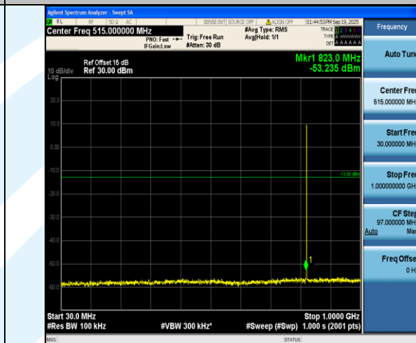
Band5-1.4MHz-16QAM-20407-1RB#0-30~1000-PASS
