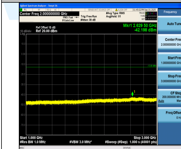
Band5-1.4MHz-16QAM-20407-1RB#0-1000~3000-PASS
