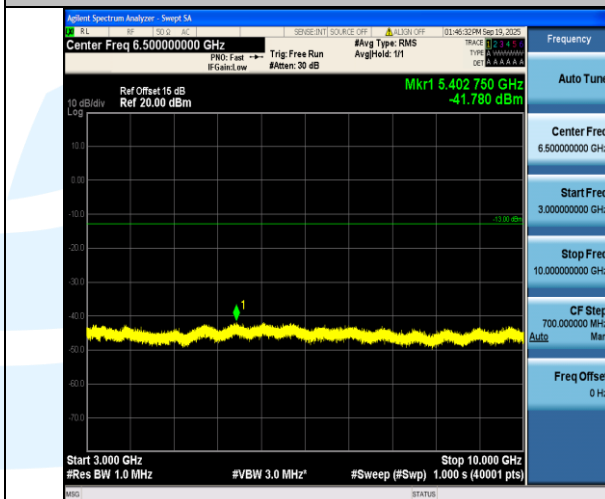
Band5-1.4MHz-QPSK-20643-1RB#0-3000~10000-PASS
