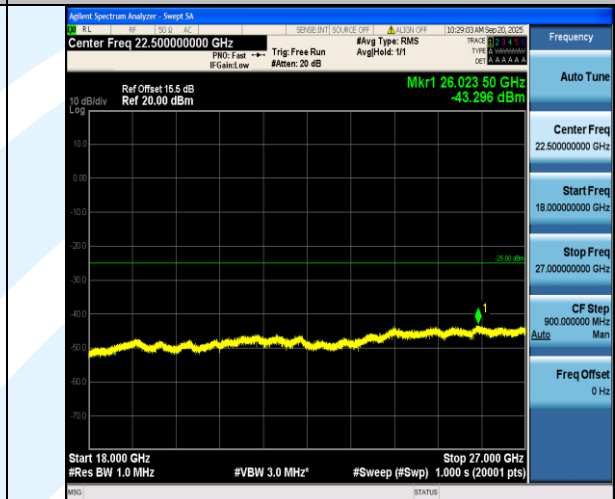
Band7-10MHz-QPSK-20800-1RB#0-18000~27000-PASS
