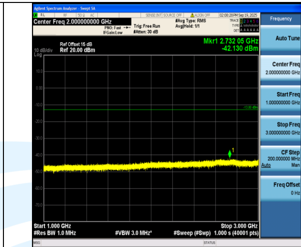
Band5-10MHz-QPSK-20600-1RB#0-1000~3000-PASS
