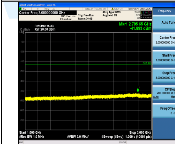
Band5-10MHz-16QAM-20450-1RB#0-1000~3000-PASS
