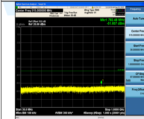
Band7-10MHz-QPSK-21100-1RB#0-30~1000-PASS
