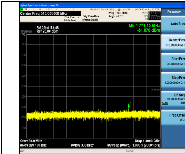
Band7-10MHz-QPSK-20800-1RB#0-30~1000-PASS
