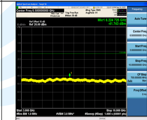
Band5-10MHz-16QAM-20450-1RB#0-3000~10000-PASS
