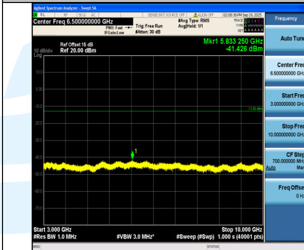
Band5-10MHz-QPSK-20600-1RB#0-3000~10000-PASS
