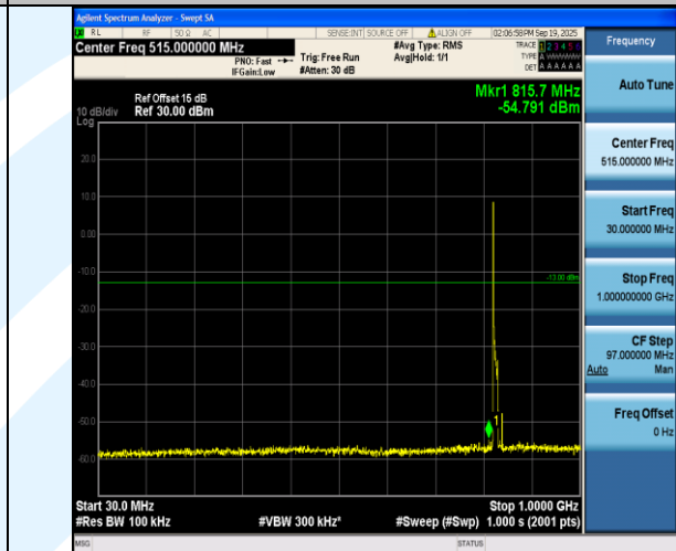
Band5-10MHz-16QAM-20450-1RB#0-30~1000-PASS
