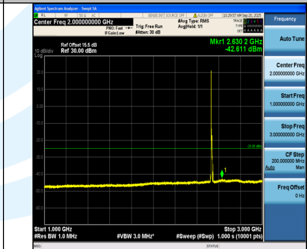
Band7-10MHz-QPSK-21100-1RB#0-1000~3000-PASS
