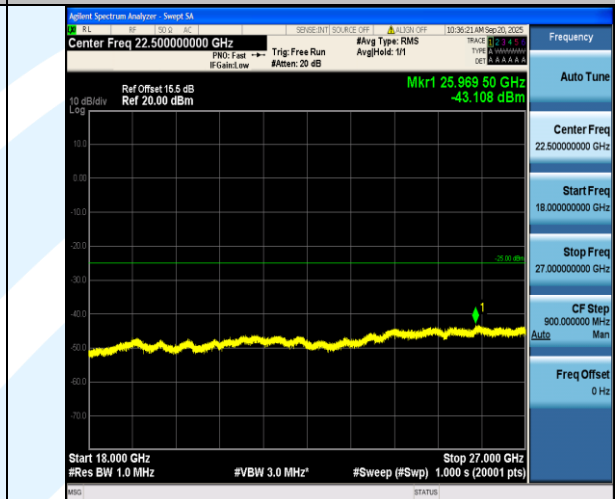
Band7-20MHz-QPSK-20850-1RB#0-18000~27000-PASS
