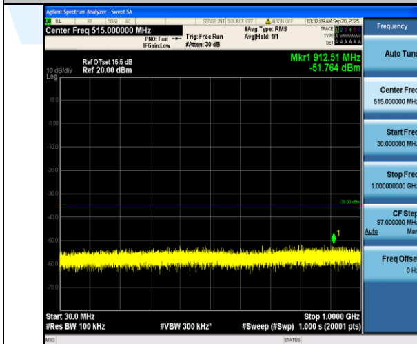
Band7-20MHz-QPSK-21100-1RB#0-30~1000-PASS
