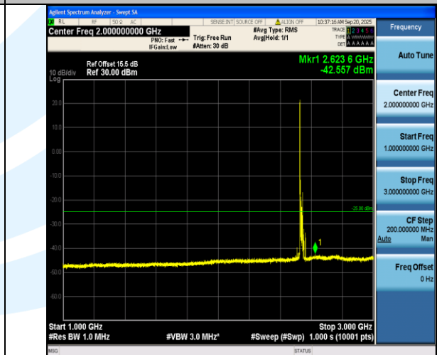
Band7-20MHz-QPSK-21100-1RB#0-1000~3000-PASS
