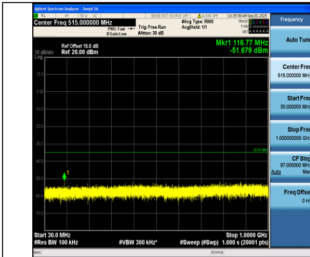
Band7-20MHz-QPSK-20850-1RB#0-30~1000-PASS
