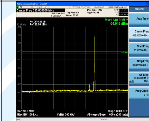
Band71-5MHz-16QAM-133447-1RB#0-30~1000-PASS
