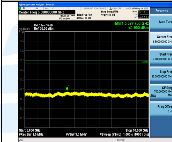
Band71-5MHz-16QAM-133297-1RB#0-3000~10000-PASS
