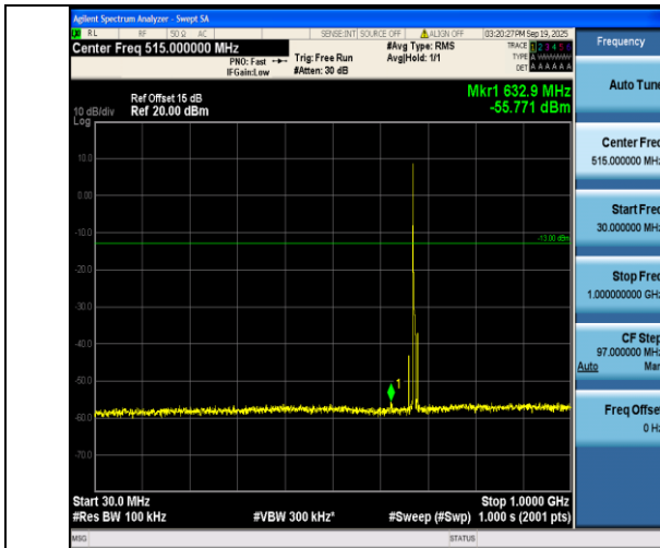
Band71-5MHz-16QAM-133297-1RB#0-30~1000-PASS
