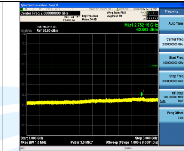
Band71-5MHz-16QAM-133297-1RB#0-1000~3000-PASS
