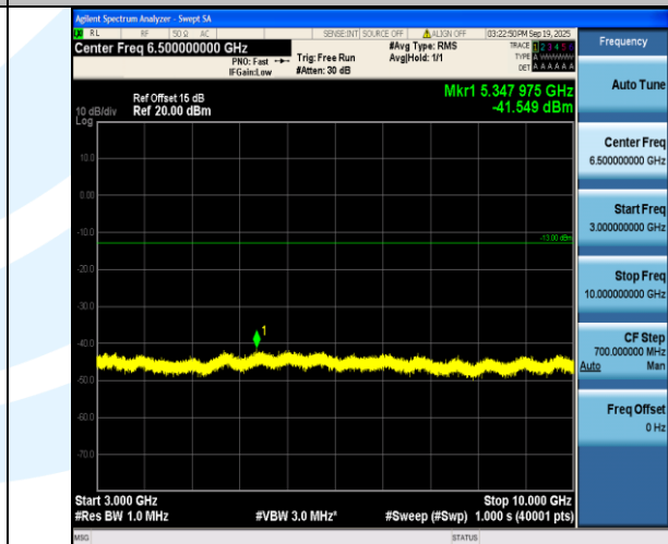
Band71-5MHz-16QAM-133447-1RB#0-3000~10000-PASS
