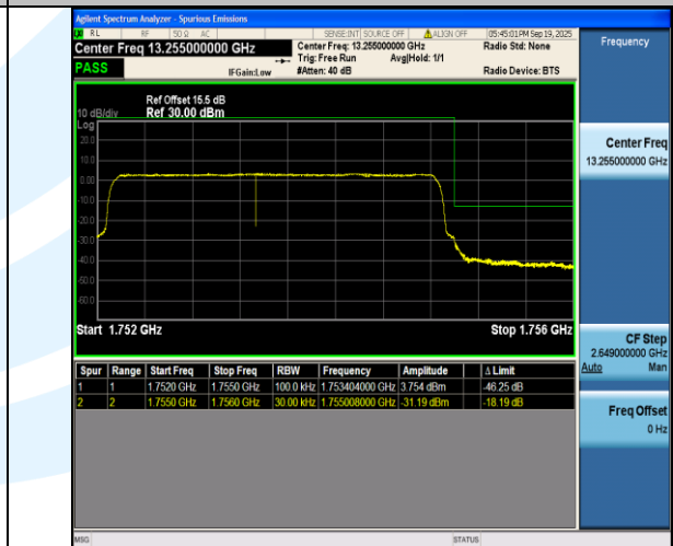
Band4-3MHz-16QAM-20385-15RB#0-PASS
