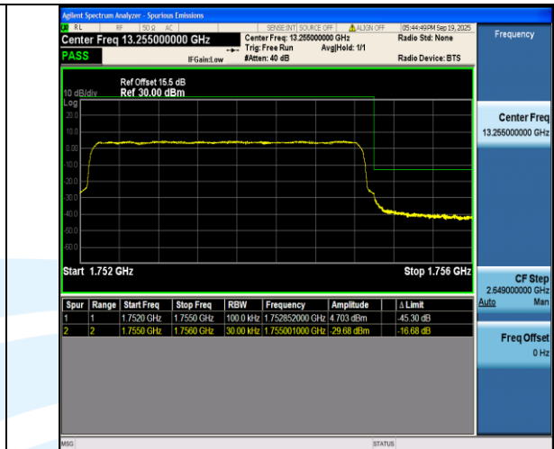
Band4-3MHz-QPSK-20385-15RB#0-PASS
