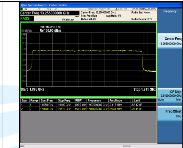
Band2-15MHz-QPSK-19125-75RB#0-PASS
