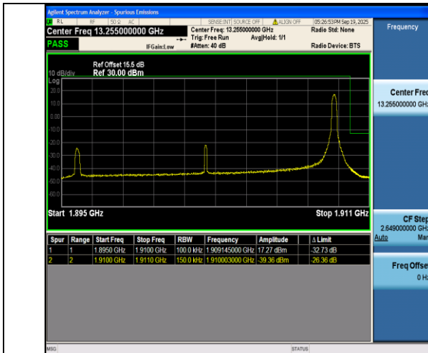
Band2-15MHz-QPSK-19125-1RB#74-PASS
