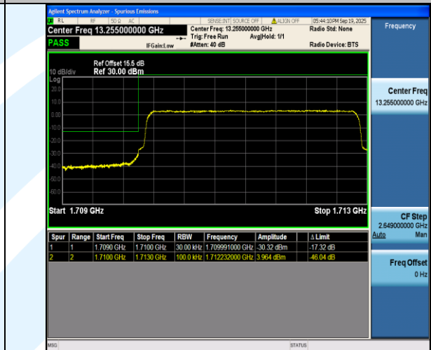
Band4-3MHz-16QAM-19965-15RB#0-PASS
