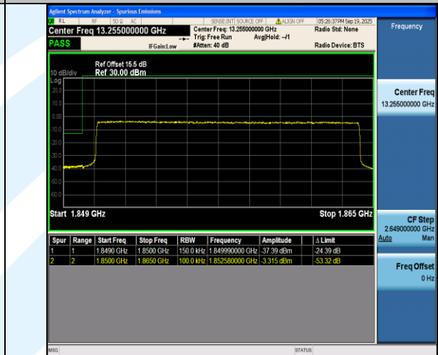
Band2-15MHz-16QAM-18675-75RB#0-PASS
