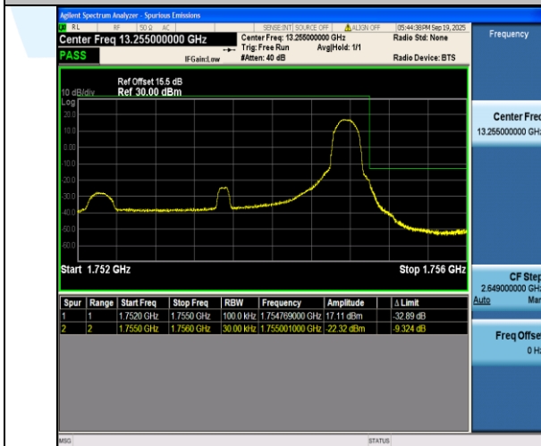
Band4-3MHz-16QAM-20385-1RB#14-PASS
