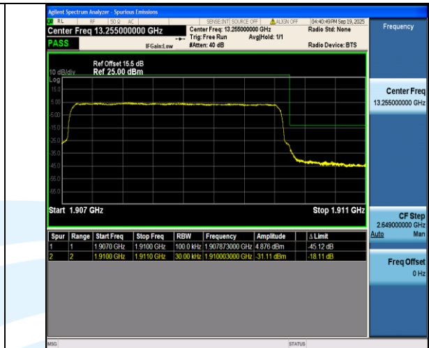
Band2-3MHz-QPSK-19185-15RB#0-PASS
