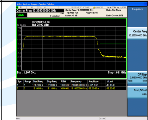
Band2-3MHz-16QAM-19185-15RB#0-PASS
