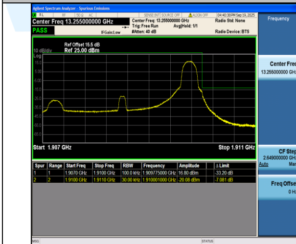
Band2-3MHz-16QAM-19185-1RB#14-PASS
