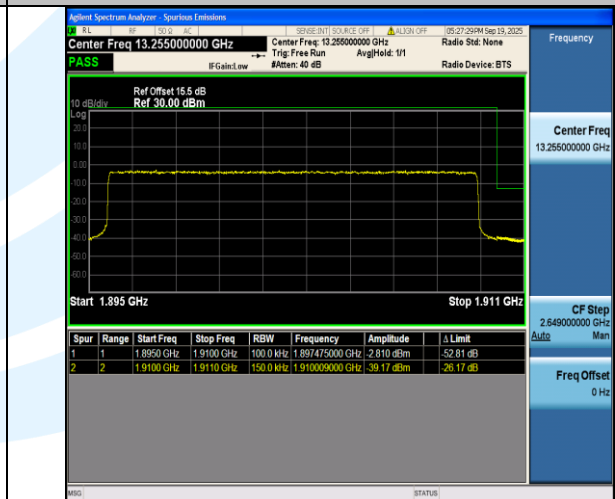
Band2-15MHz-16QAM-19125-75RB#0-PASS
