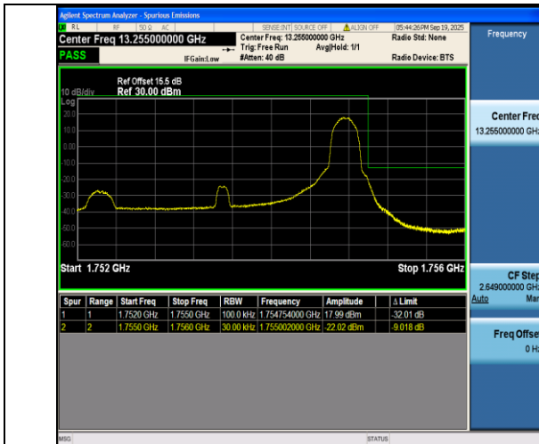
Band4-3MHz-QPSK-20385-1RB#14-PASS
