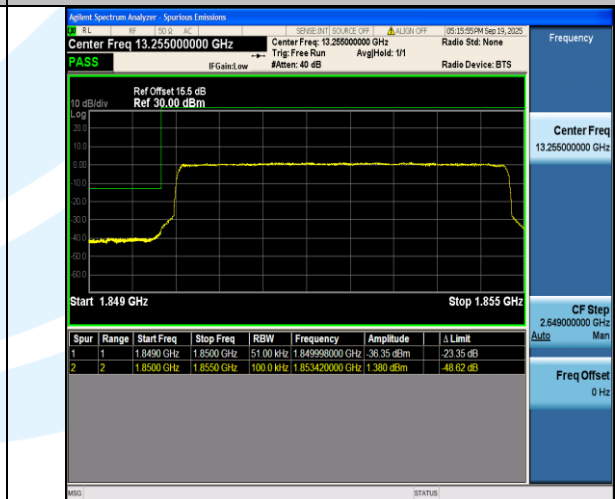
Band2-5MHz-16QAM-18625-25RB#0-PASS
