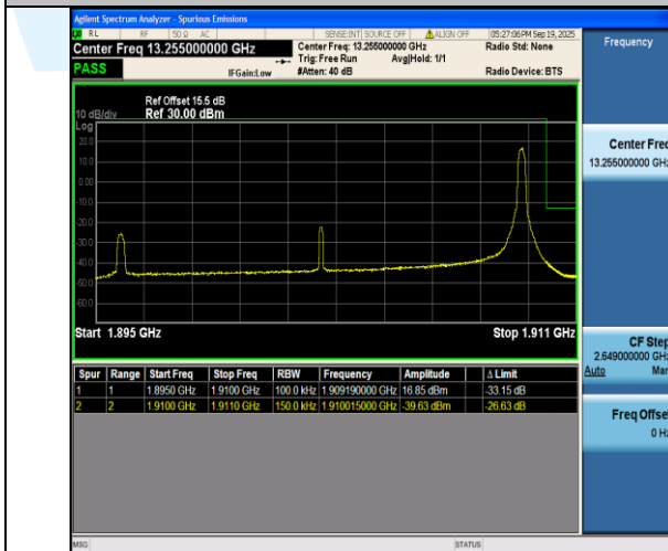
Band2-15MHz-16QAM-19125-1RB#74-PASS
