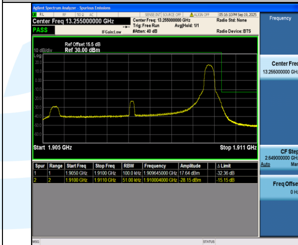
Band2-5MHz-QPSK-19175-1RB#24-PASS
