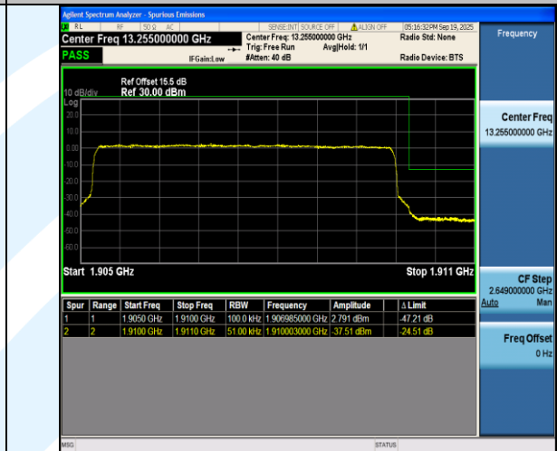
Band2-5MHz-QPSK-19175-25RB#0-PASS
