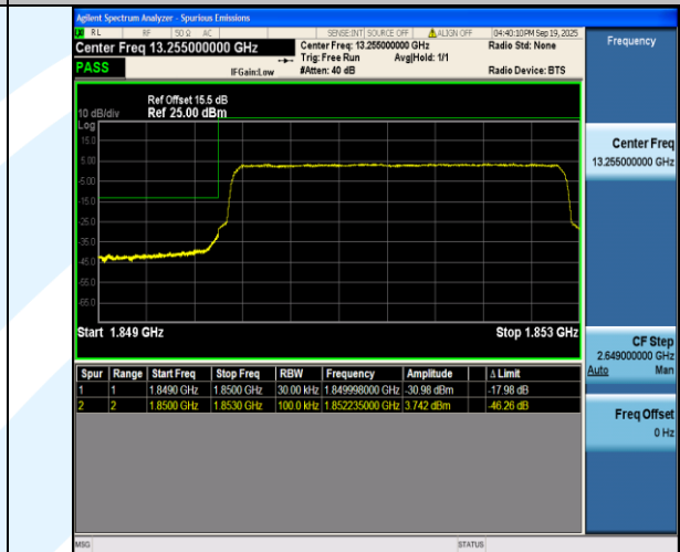
Band2-3MHz-16QAM-18615-15RB#0-PASS
