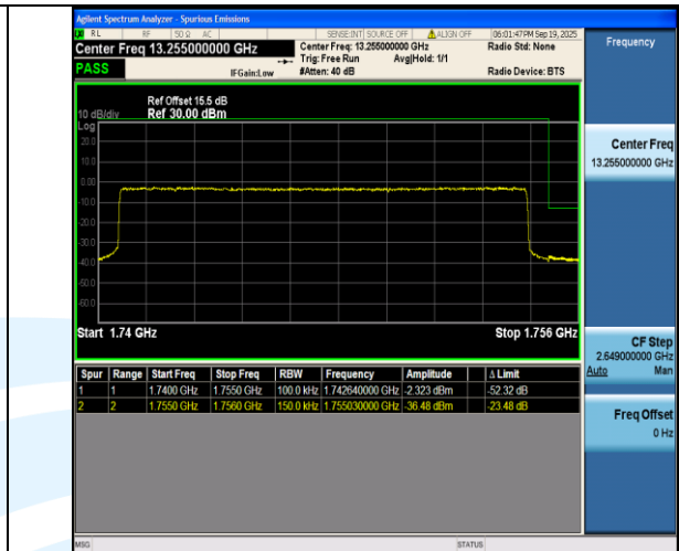
Band4-15MHz-QPSK-20325-75RB#0-PASS
