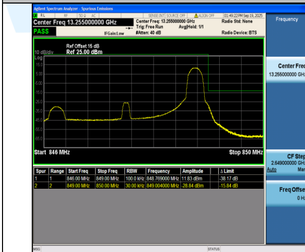
Band5-3MHz-16QAM-20635-1RB#14-PASS
