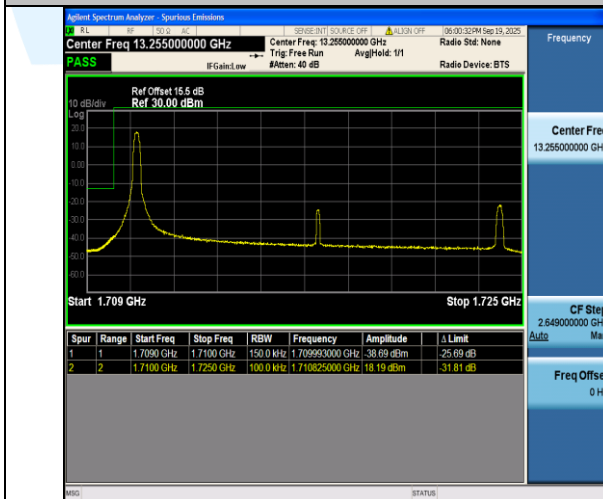
Band4-15MHz-QPSK-20025-1RB#0-PASS
