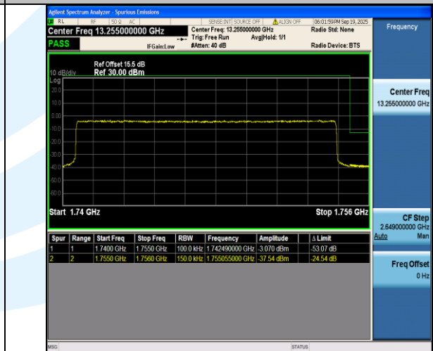
Band4-15MHz-16QAM-20325-75RB#0-PASS
