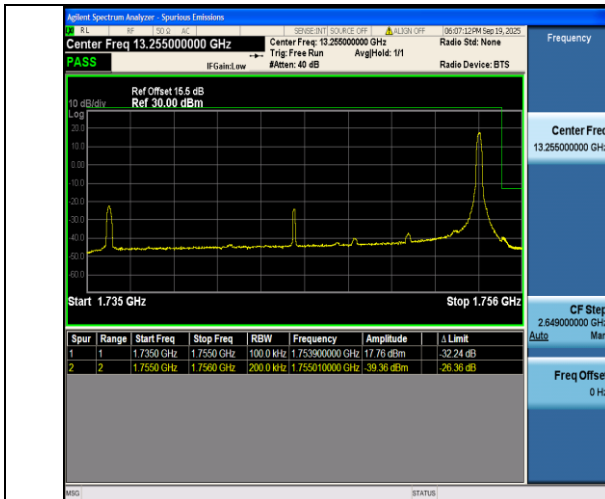
Band4-20MHz-16QAM-20300-1RB#99-PASS
