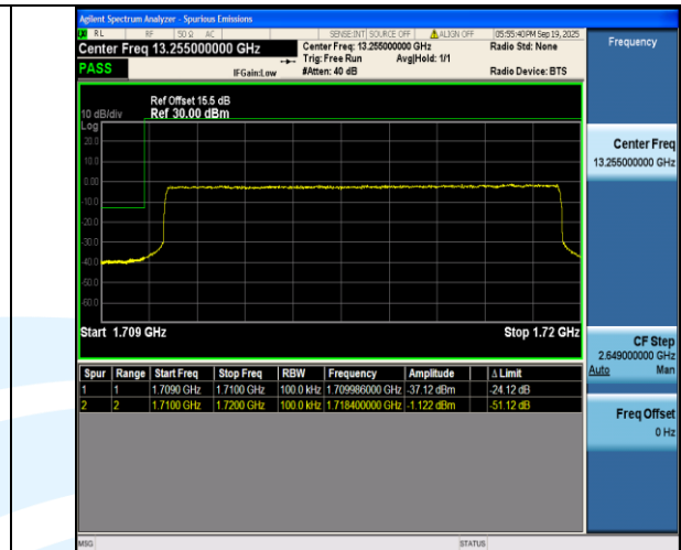
Band4-10MHz-16QAM-20000-50RB#0-PASS
