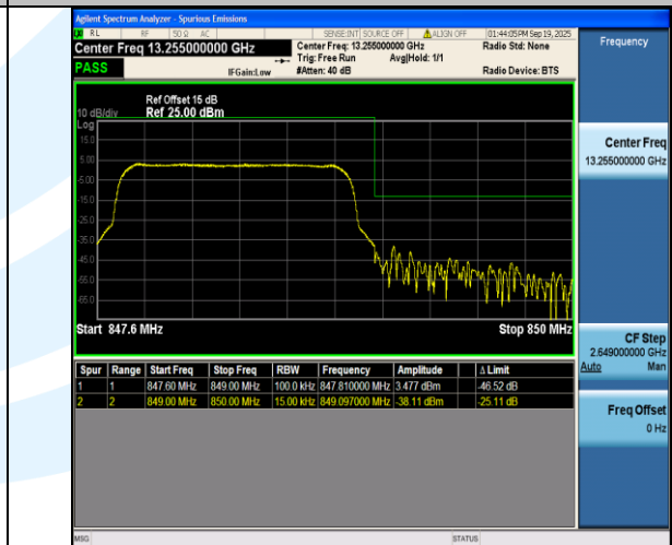
Band5-1.4MHz-QPSK-20643-6RB#0-PASS
