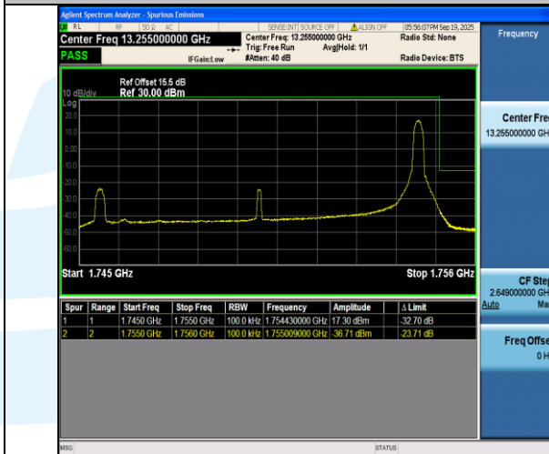
Band4-10MHz-16QAM-20350-1RB#49-PASS
