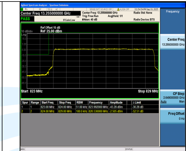
Band5-5MHz-QPSK-20425-25RB#0-PASS
