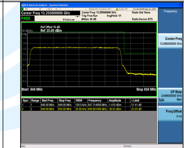
Band5-3MHz-16QAM-20635-15RB#0-PASS
