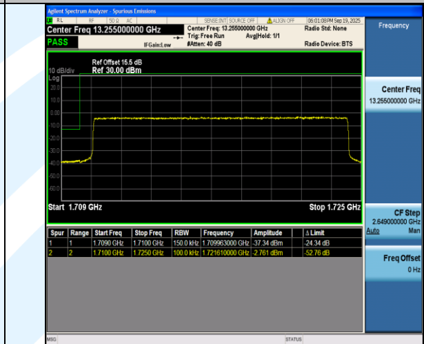
Band4-15MHz-16QAM-20025-75RB#0-PASS
