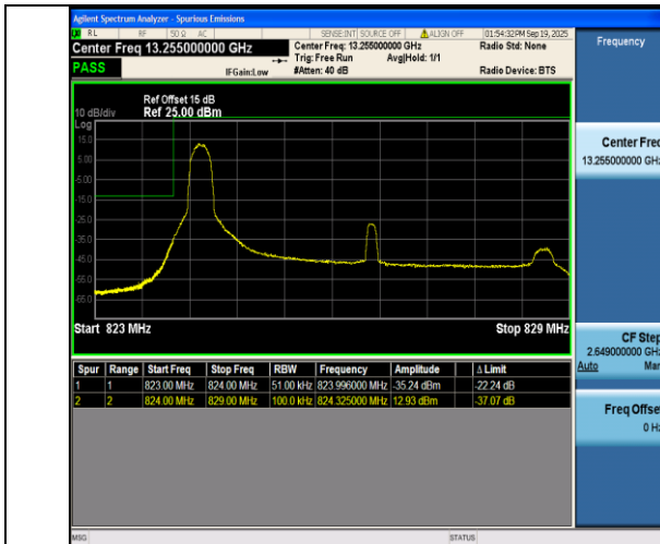
Band5-5MHz-QPSK-20425-1RB#0-PASS
