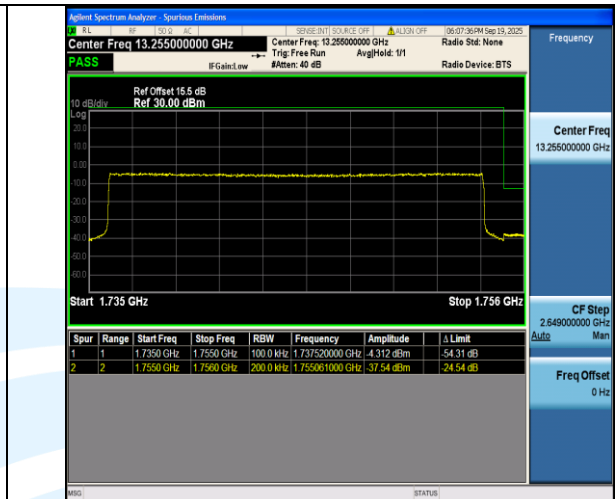
Band4-20MHz-16QAM-20300-100RB#0-PASS
