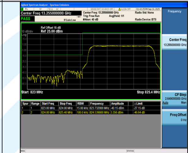
Band5-1.4MHz-QPSK-20407-6RB#0-PASS
