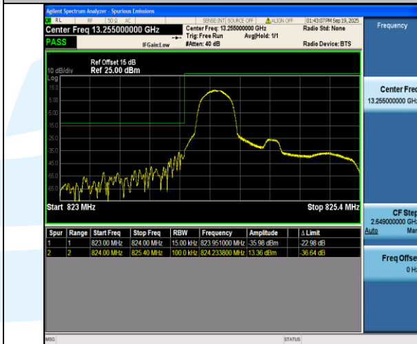
Band5-1.4MHz-QPSK-20407-1RB#0-PASS
