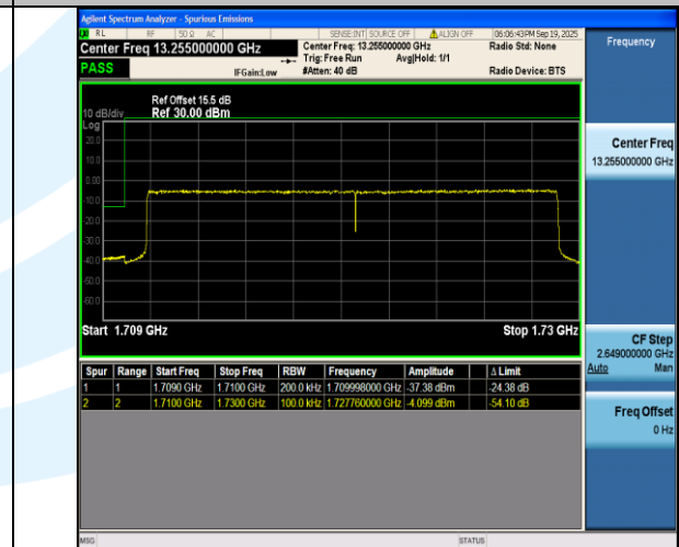
Band4-20MHz-16QAM-20050-100RB#0-PASS
