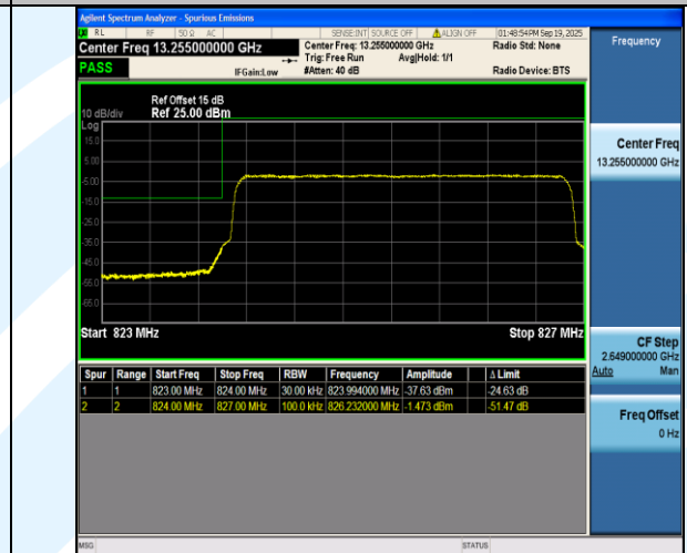
Band5-3MHz-16QAM-20415-15RB#0-PASS
