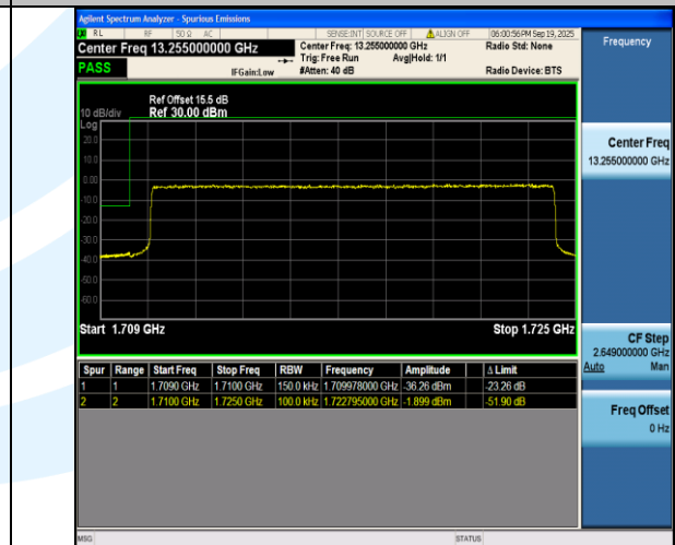
Band4-15MHz-QPSK-20025-75RB#0-PASS
