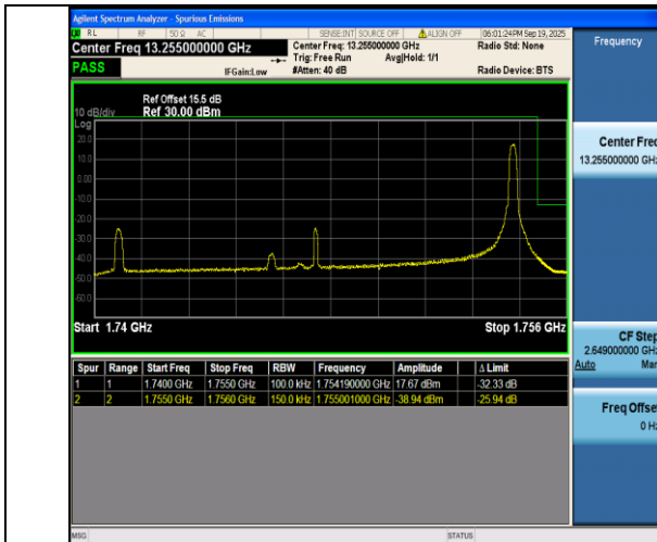
Band4-15MHz-QPSK-20325-1RB#74-PASS
