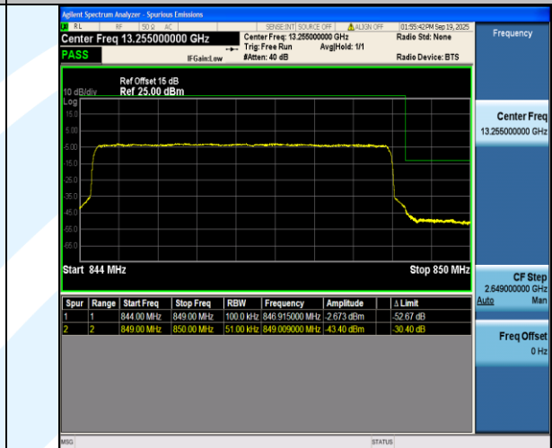
Band5-5MHz-QPSK-20625-25RB#0-PASS
