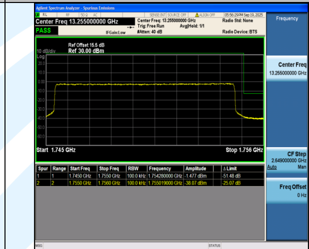
Band4-10MHz-16QAM-20350-50RB#0-PASS
