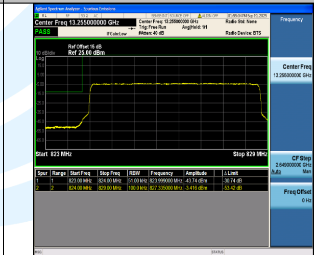
Band5-5MHz-16QAM-20425-25RB#0-PASS
