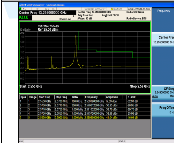
Band7-15MHz-QPSK-21375-1RB#74-PASS
