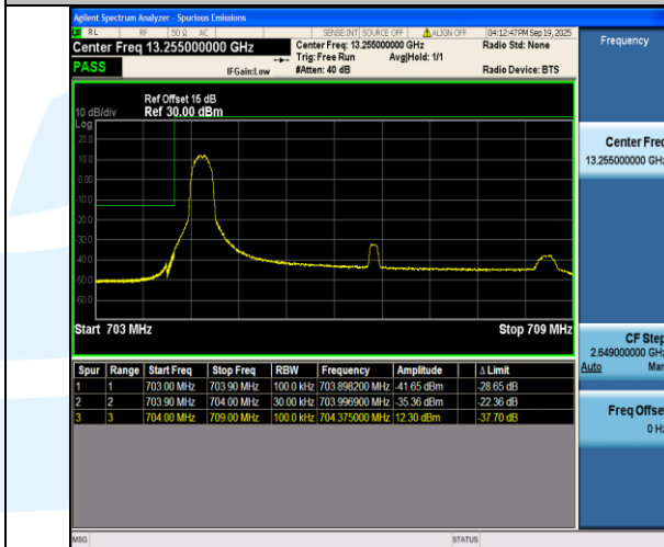
Band17-5MHz-QPSK-23755-1RB#0-PASS
