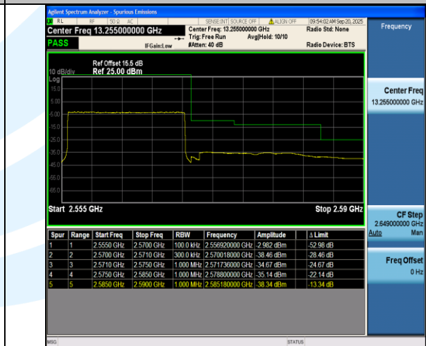
Band7-15MHz-QPSK-21375-75RB#0-PASS
