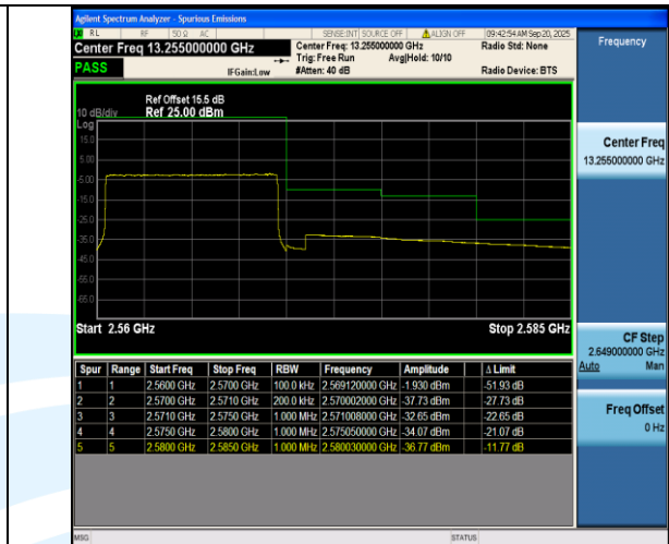
Band7-10MHz-16QAM-21400-50RB#0-PASS
