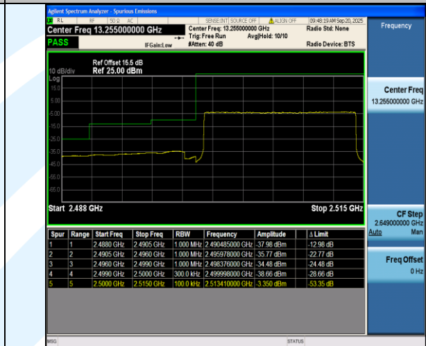
Band7-15MHz-QPSK-20825-75RB#0-PASS
