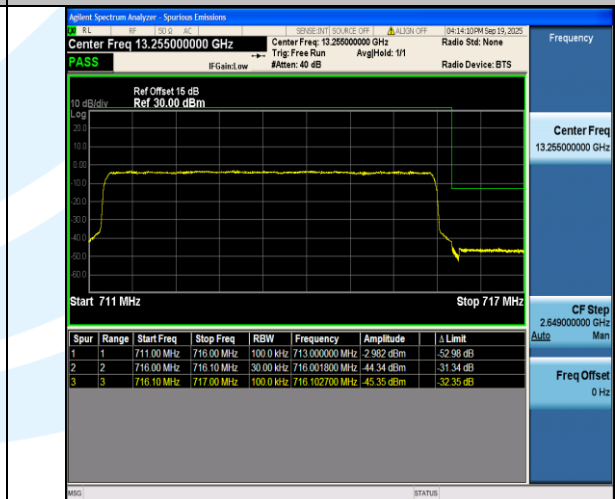
Band17-5MHz-QPSK-23825-25RB#0-PASS
