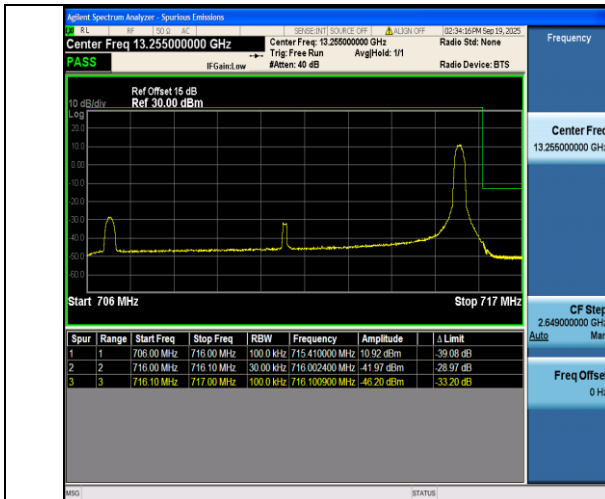
Band12-10MHz-16QAM-23130-1RB#49-PASS
