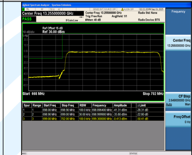
Band12-3MHz-QPSK-23025-15RB#0-PASS
