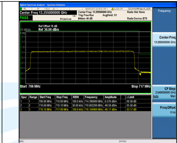
Band12-10MHz-16QAM-23130-50RB#0-PASS
