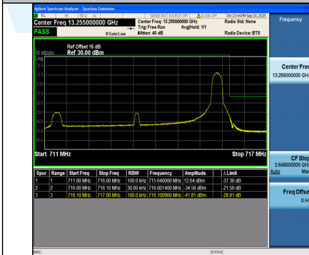
Band17-5MHz-QPSK-23825-1RB#24-PASS
