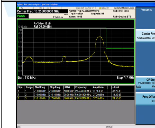
Band12-3MHz-QPSK-23165-1RB#14-PASS
