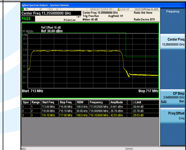
Band12-3MHz-QPSK-23165-15RB#0-PASS
