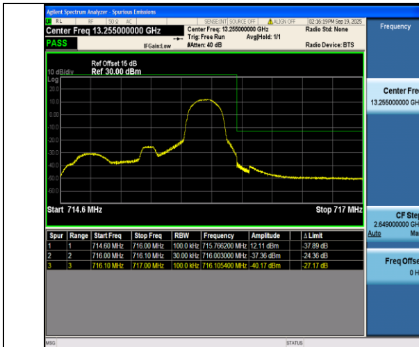
Band12-1.4MHz-16QAM-23173-1RB#5-PASS
