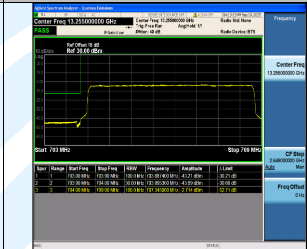
Band17-5MHz-QPSK-23755-25RB#0-PASS
