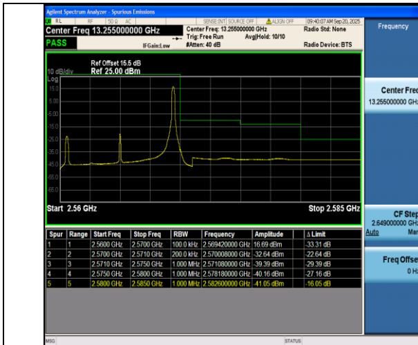
Band7-10MHz-16QAM-21400-1RB#49-PASS
