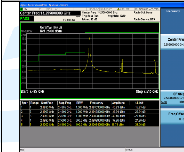
Band7-15MHz-QPSK-20825-1RB#0-PASS
