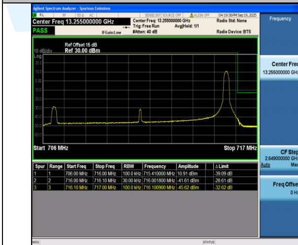
Band17-10MHz-16QAM-23800-1RB#49-PASS
