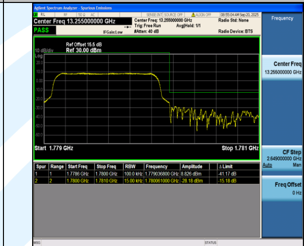
Band66-1.4MHz-QPSK-132665-6RB#0-PASS
