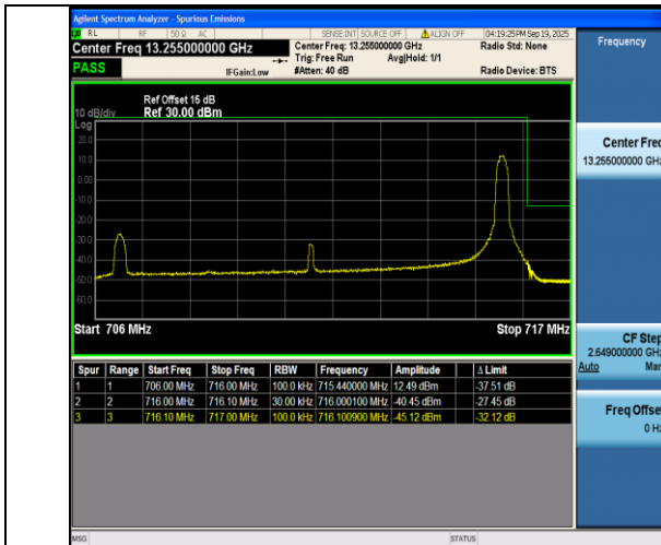
Band17-10MHz-QPSK-23800-1RB#49-PASS
