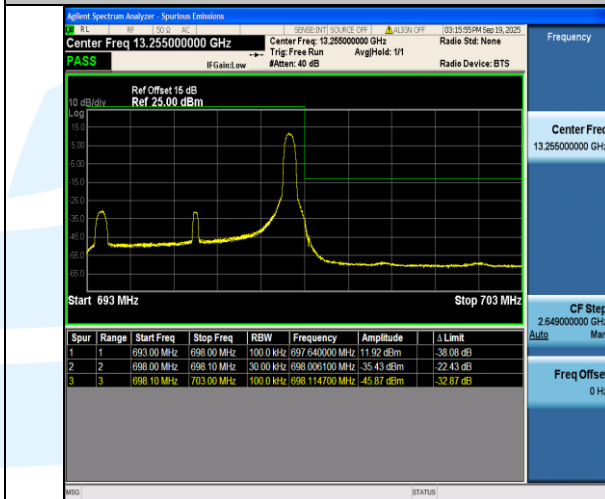
Band71-5MHz-QPSK-133447-1RB#24-PASS
