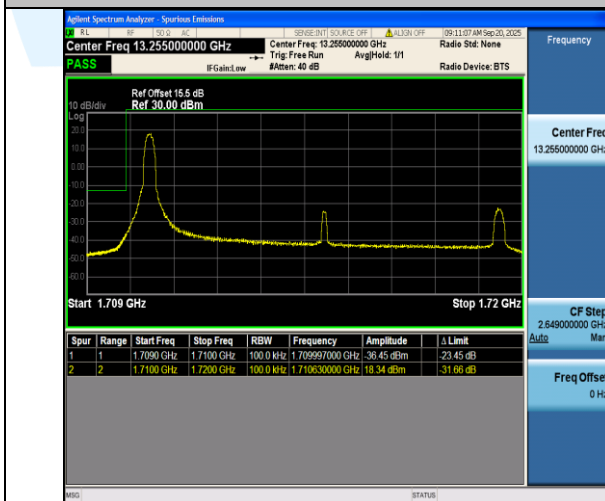
Band66-10MHz-16QAM-132022-1RB#0-PASS
