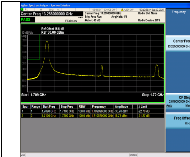
Band66-10MHz-QPSK-132022-1RB#0-PASS
