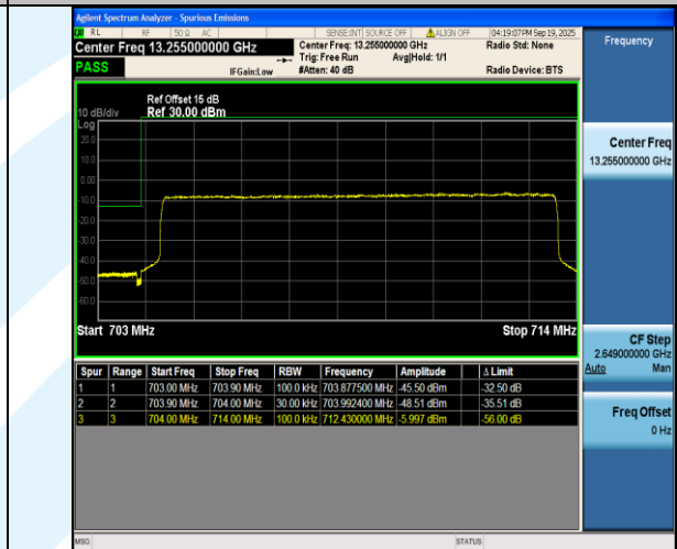
Band17-10MHz-16QAM-23780-50RB#0-PASS
