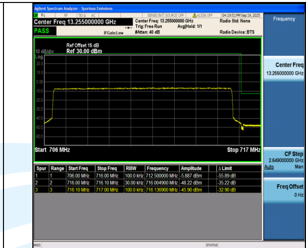
Band17-10MHz-QPSK-23800-50RB#0-PASS
