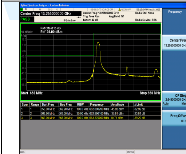
Band71-5MHz-16QAM-133147-1RB#0-PASS
