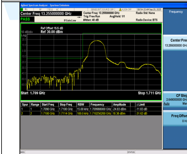
Band66-1.4MHz-16QAM-131979-1RB#0-PASS
