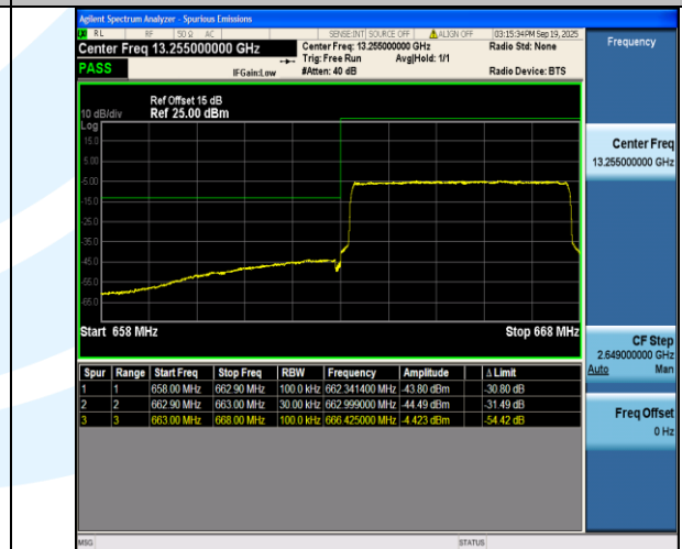
Band71-5MHz-16QAM-133147-25RB#0-PASS
