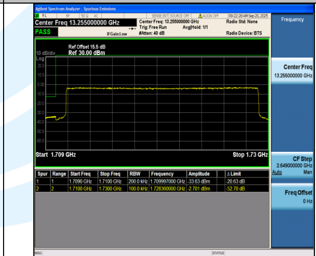
Band66-20MHz-QPSK-132072-100RB#0-PASS
