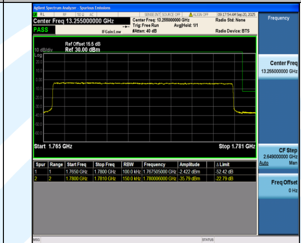
Band66-15MHz-16QAM-132597-75RB#0-PASS
