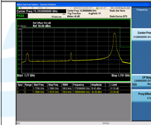
Band66-10MHz-QPSK-132622-1RB#49-PASS
