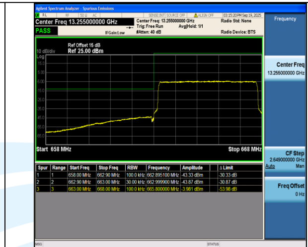
Band71-5MHz-QPSK-133147-25RB#0-PASS
