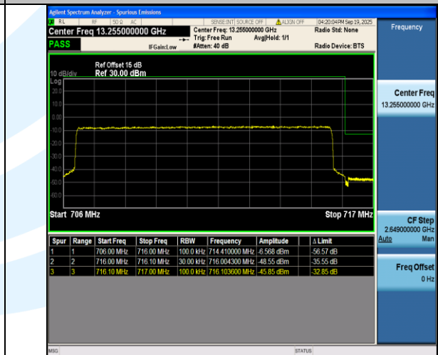
Band17-10MHz-16QAM-23800-50RB#0-PASS
