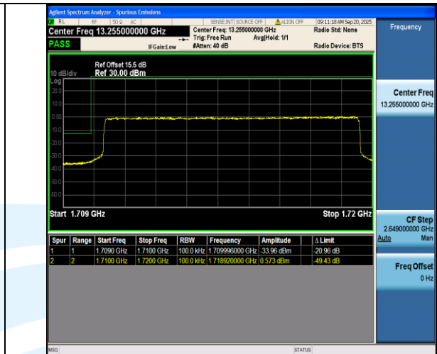
Band66-10MHz-QPSK-132022-50RB#0-PASS
