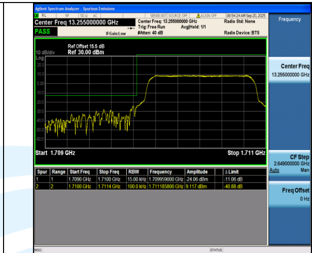
Band66-1.4MHz-QPSK-131979-6RB#0-PASS
