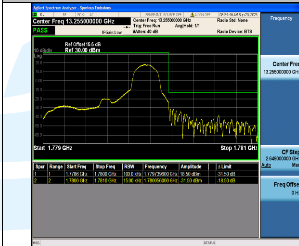
Band66-1.4MHz-QPSK-132665-1RB#5-PASS
