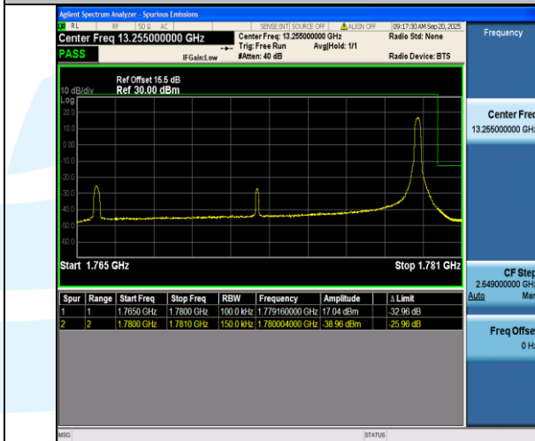
Band66-15MHz-16QAM-132597-1RB#74-PASS
