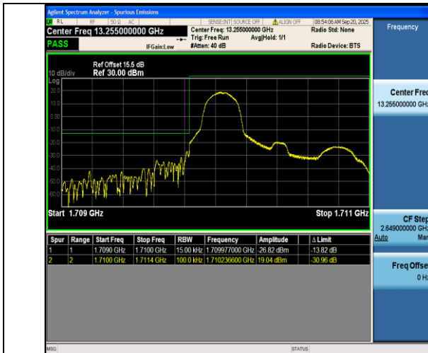
Band66-1.4MHz-QPSK-131979-1RB#0-PASS
