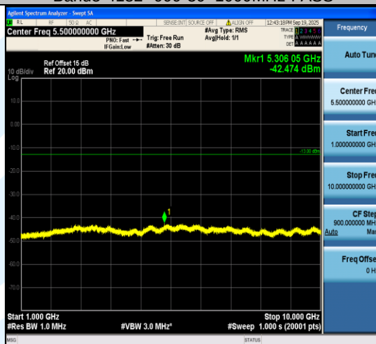
Band5-4132--999-1000~10000MHz-PASS
