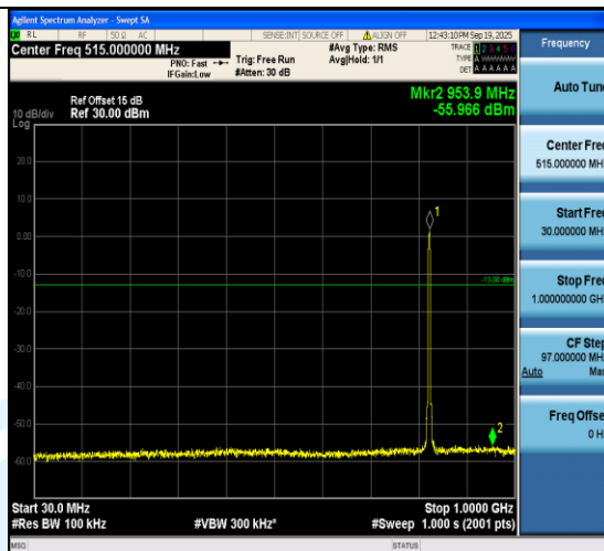
Band5-4132--999-30~1000MHz-PASS
