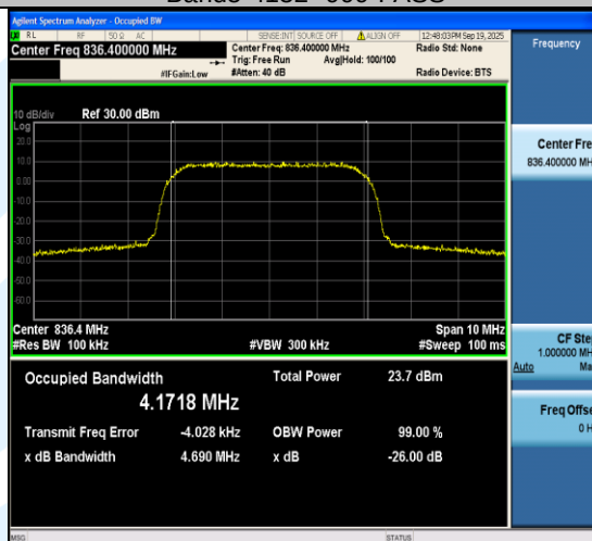
Band5-4182--999-PASS
