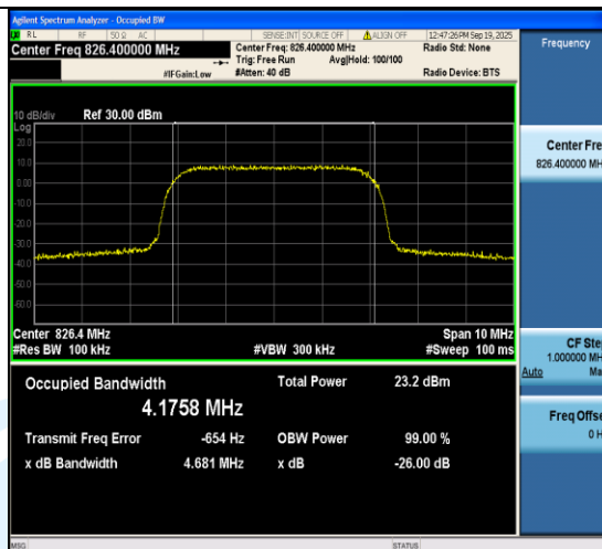
Band5-4132--999-PASS
