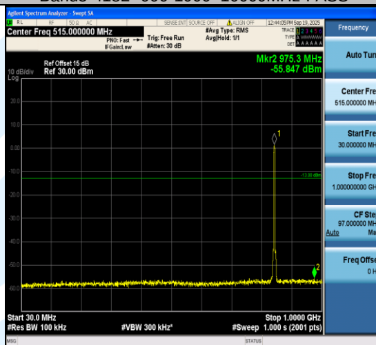
Band5-4233--999-30~1000MHz-PASS
