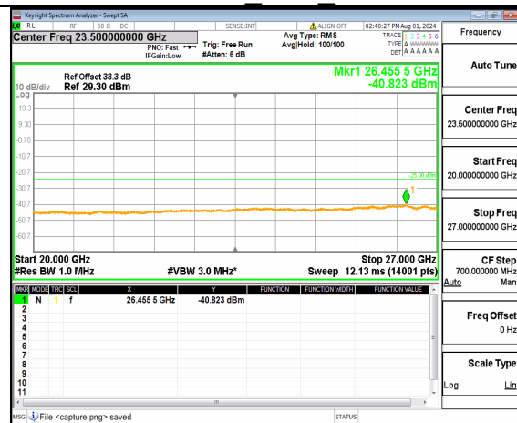
n41 (20GHz-27GHz) 15M DFT-s-OFDM BPSK Inner 1RB Right Mid
