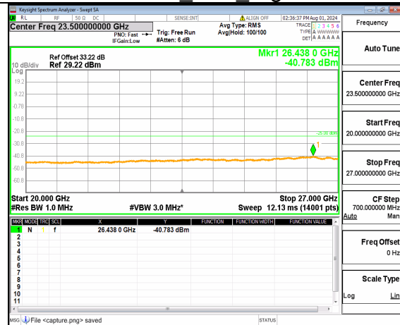
n41 (20GHz-27GHz) 15M DFT-s-OFDM QPSK Inner 1RB Left Low
