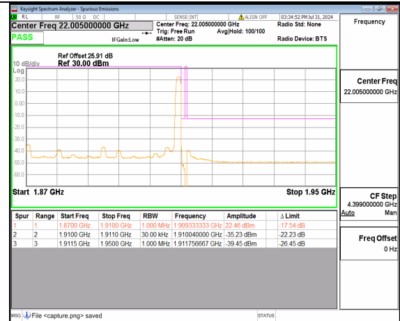
n2 40M DFT-s-OFDM BPSK Edge_1RB_Right High
