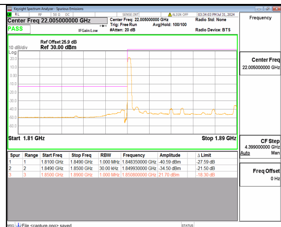
n2 40M DFT-s-OFDM QPSK Edge_1RB_Left Low
