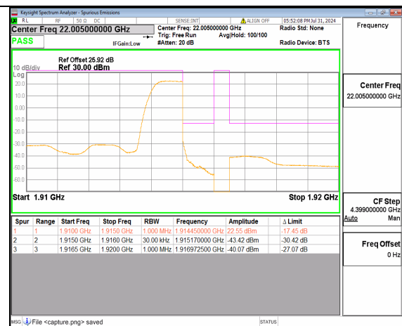
n25 5M DFT-s-OFDM BPSK Edge_1RB_Right High
