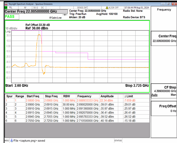
n41 10M DFT-s-OFDM BPSK Edge_1RB_Right High
