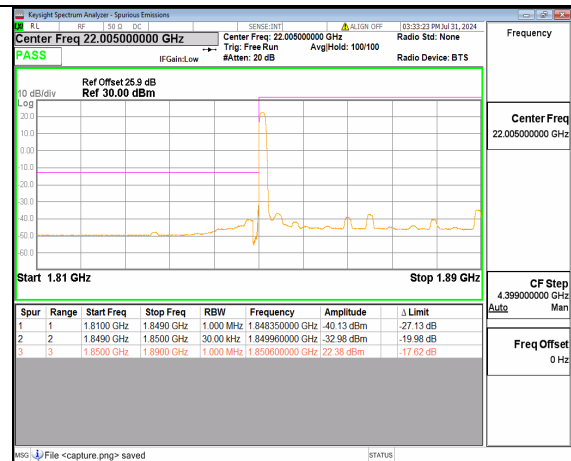
n2 40M DFT-s-OFDM BPSK Edge_1RB_Left Low
