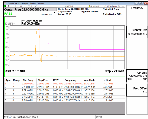
n41 15M DFT-s-OFDM BPSK Edge_1RB_Right High
