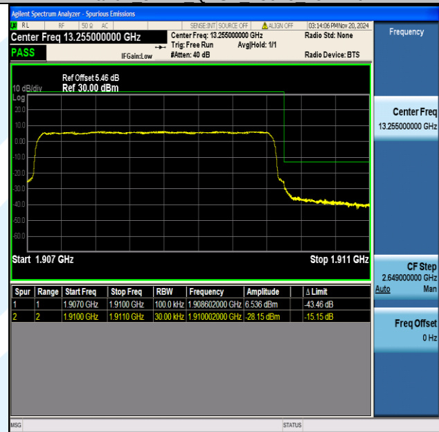
Band2_3MHz_QPSK_19185_15RB#0
