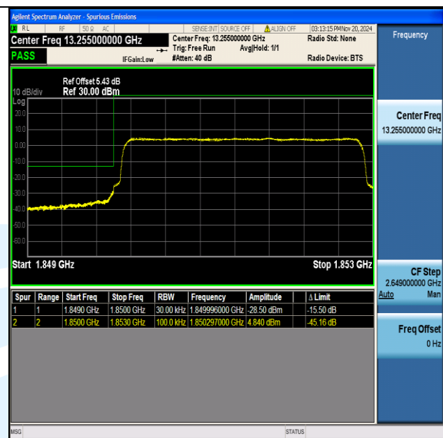
Band2_3MHz_QPSK_18615_15RB#0
