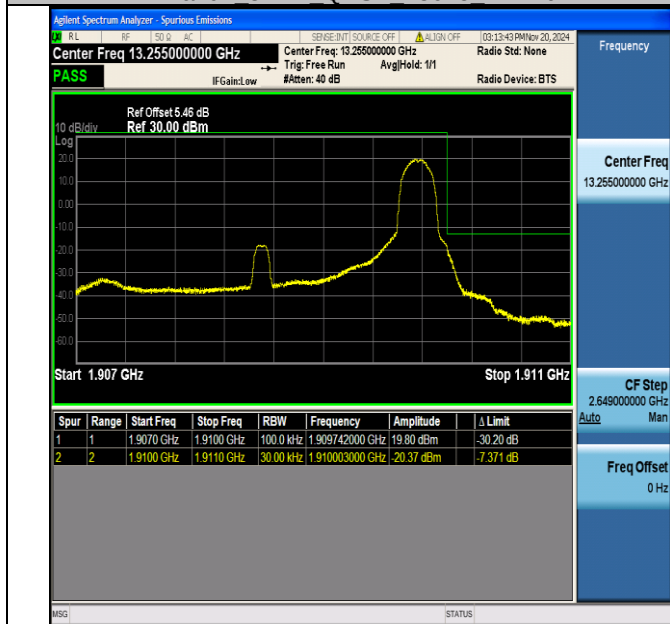
Band2_3MHz_QPSK_19185_1RB#14
