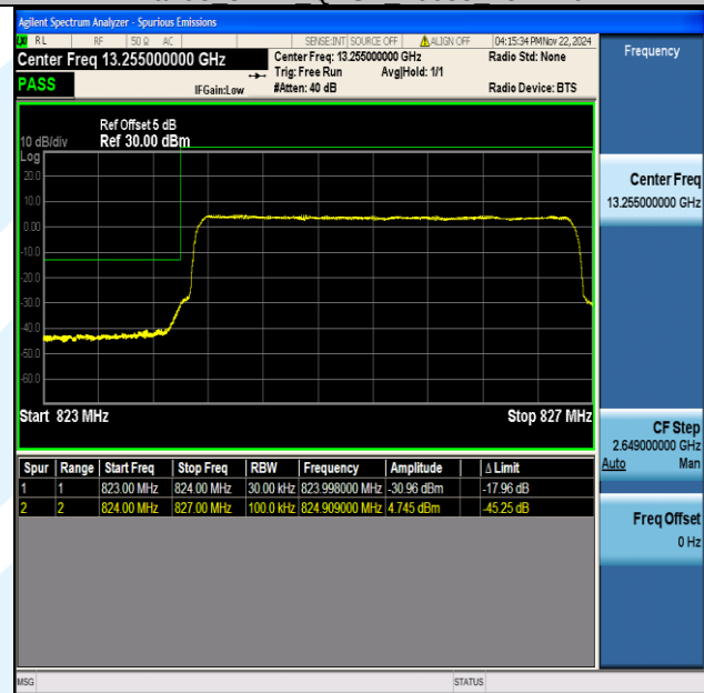
Band5 3MHz 64QAM 20415 15RB#0
