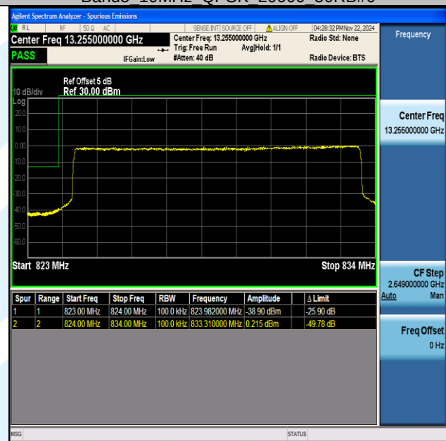
Band5 10MHz 64QAM 20450 50RB#0
