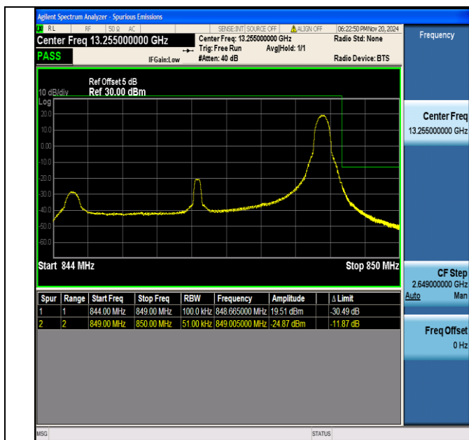
Band5 5MHz 16QAM 20625 1RB#24
