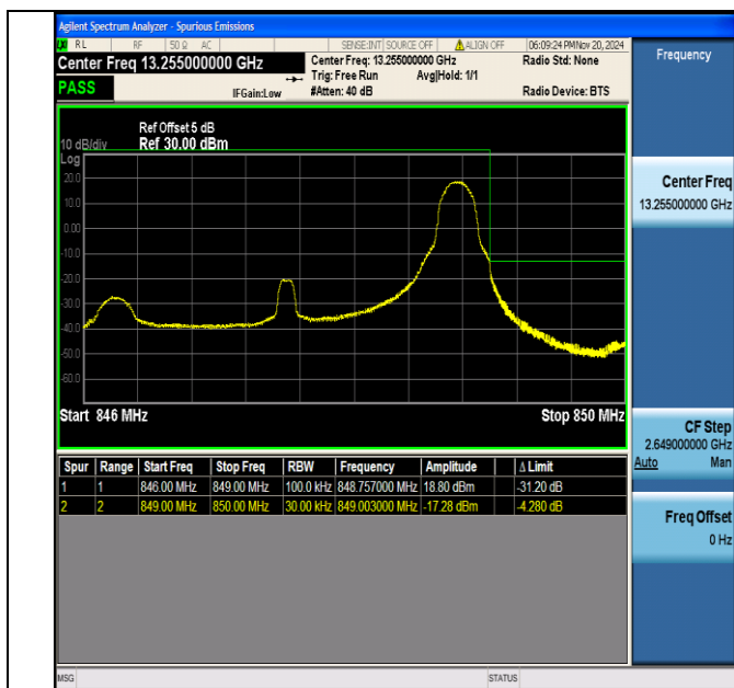
Band5 3MHz 16QAM 20635 1RB#14
