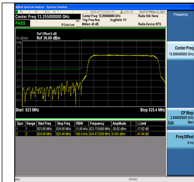
Band5 1.4MHz 64QAM 20407 6RB#0
