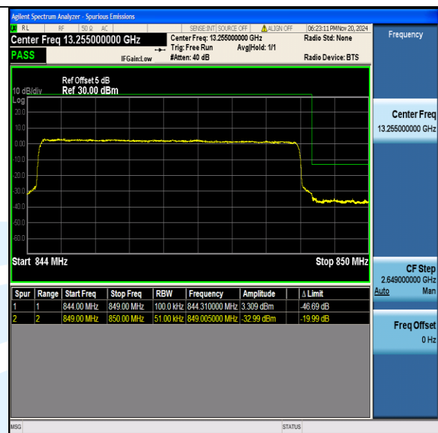
Band5 5MHz 16QAM 20625 25RB#0
