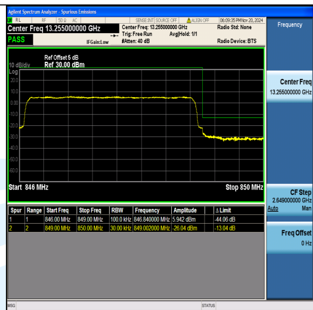
Band5 3MHz QPSK 20635 15RB#0
