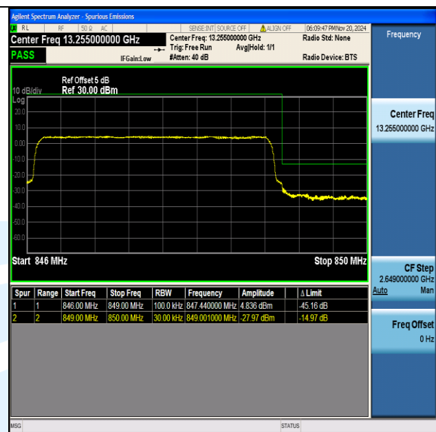
Band5 3MHz 16QAM 20635 15RB#0
