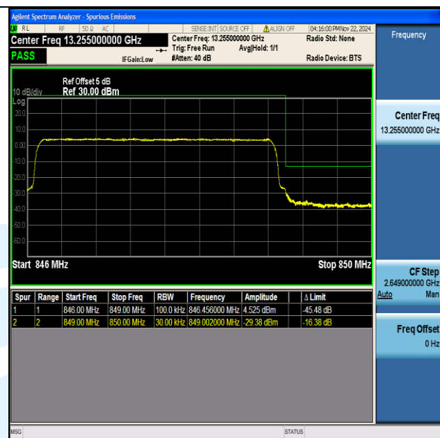
Band5 3MHz 64QAM 20635 15RB#0
