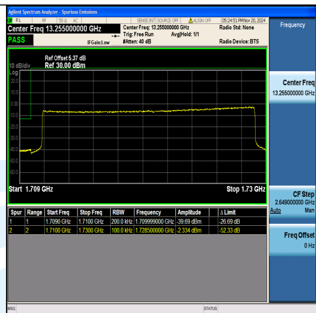
Band4 20MHz 16QAM 20050 100RB#0
