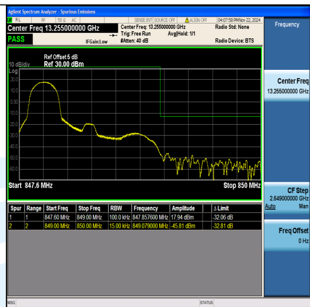
Band5 1.4MHz 64QAM 20643 1RB#0
