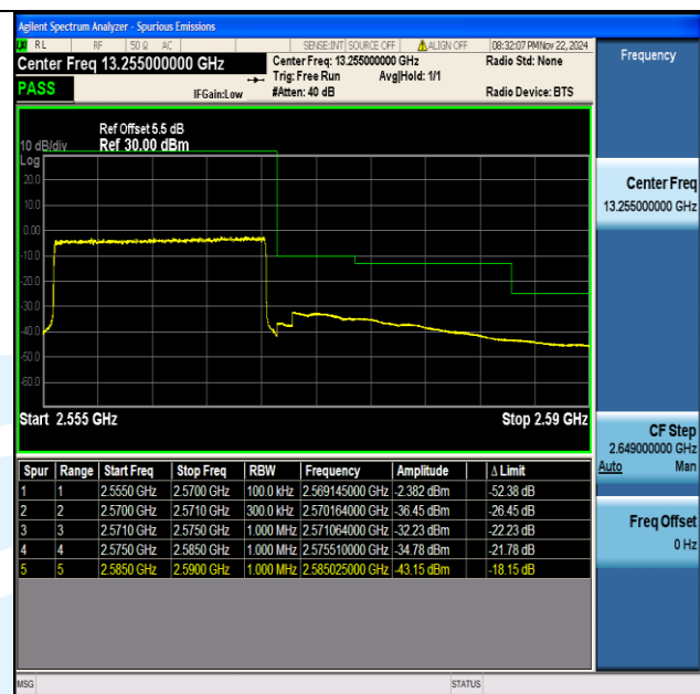
Band7 15MHz 64QAM 21375 75RB#0
