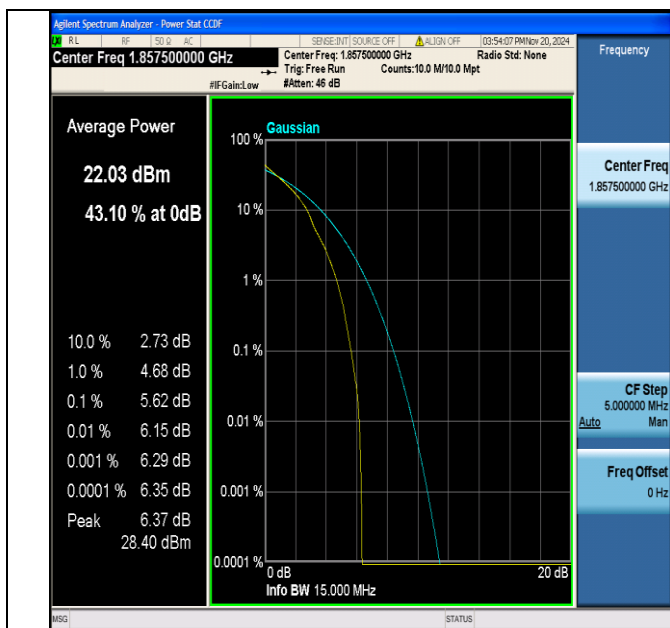
Band2-15MHz-QPSK-18675-1RB#0-PASS
