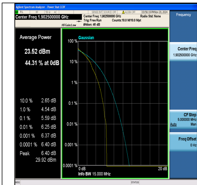
Band2-15MHz-QPSK-19125-1RB#0-PASS
