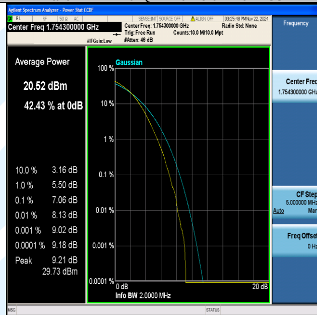
Band4-1.4MHz-64QAM-20393-6RB#0-PASS
