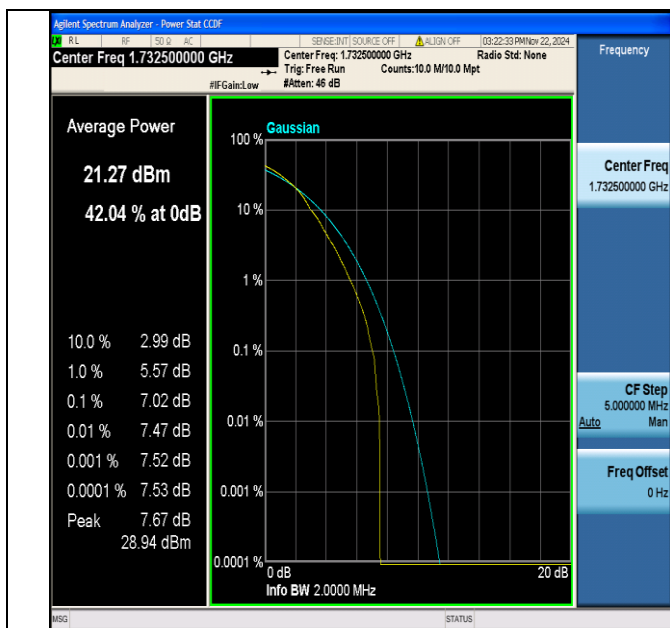
Band4-1.4MHz-64QAM-20175-1RB#0-PASS
