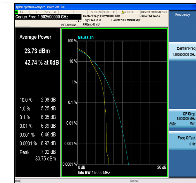
Band2-15MHz-16QAM-19125-1RB#0-PASS
