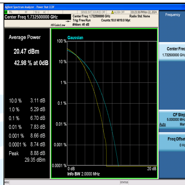
Band4-1.4MHz-64QAM-20175-6RB#0-PASS
