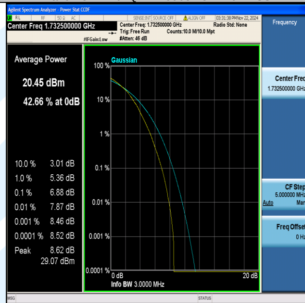
Band4-3MHz-64QAM-20175-15RB#0-PASS
