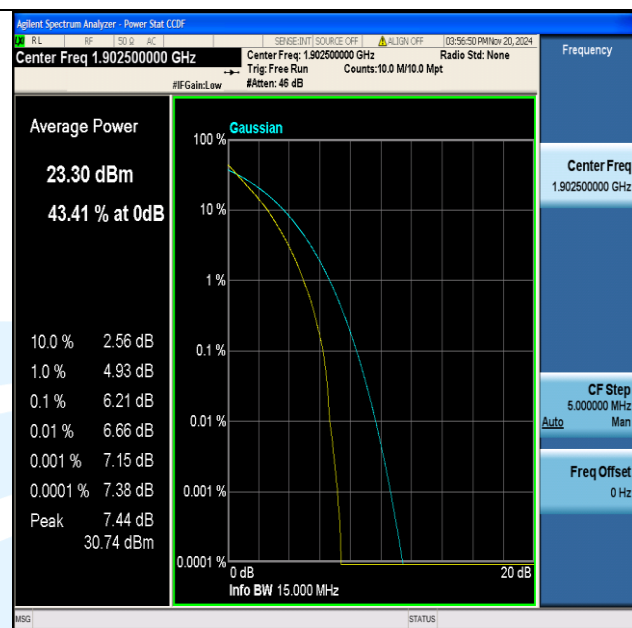
Band2-15MHz-QPSK-19125-75RB#0-PASS
