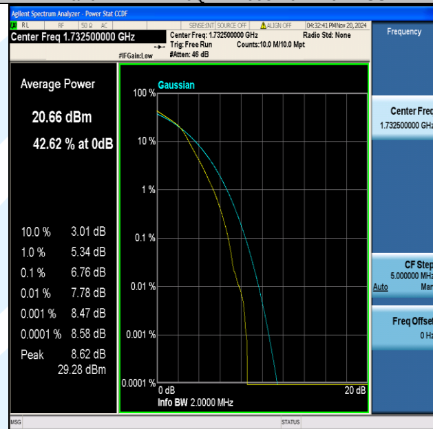
Band4-1.4MHz-16QAM-20175-6RB#0-PASS
