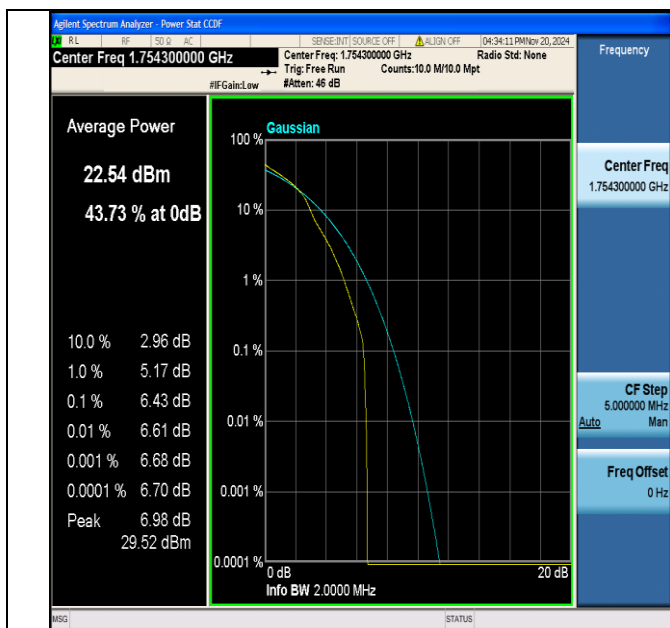
Band4-1.4MHz-16QAM-20393-1RB#0-PASS
