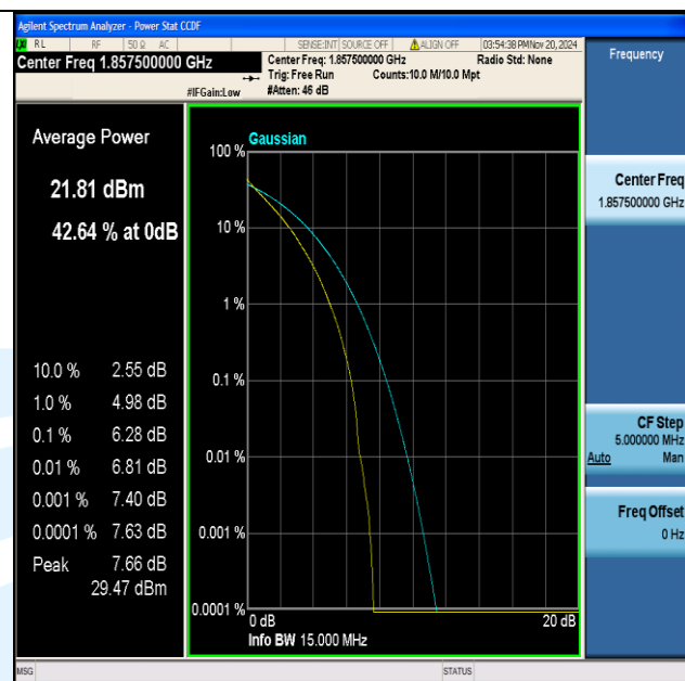
Band2-15MHz-QPSK-18675-75RB#0-PASS
