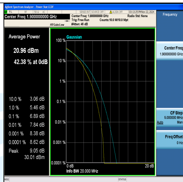
Band2-20MHz-64QAM-19100-100RB#0-PASS
