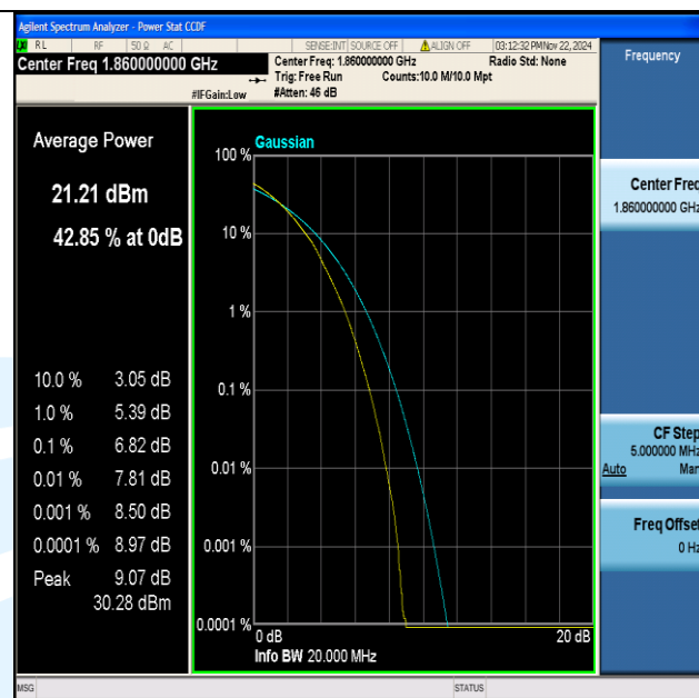
Band2-20MHz-64QAM-18700-100RB#0-PASS
