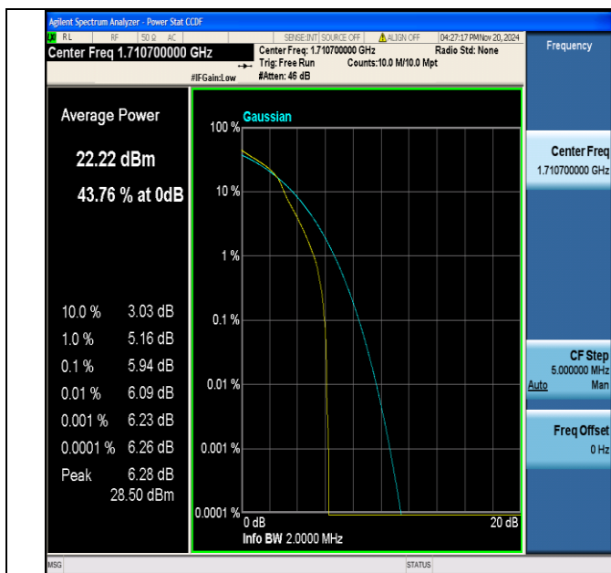
Band4-1.4MHz-16QAM-19957-1RB#0-PASS
