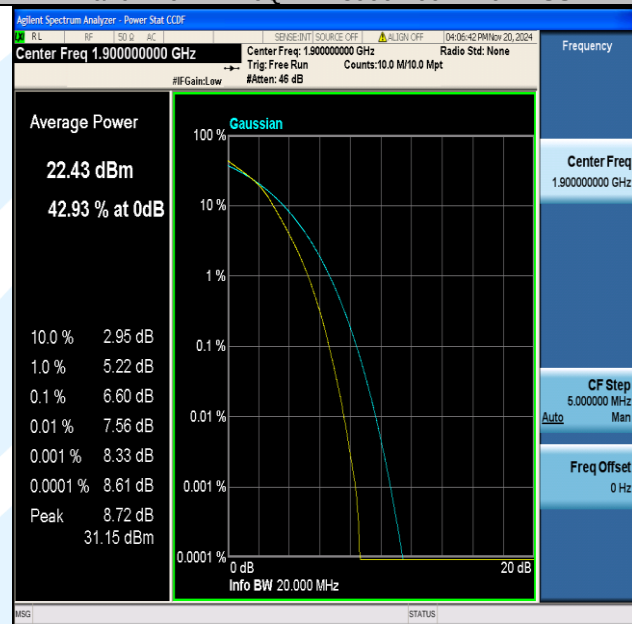
Band2-20MHz-16QAM-19100-100RB#0-PASS
