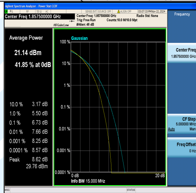
Band2-15MHz-64QAM-18675-75RB#0-PASS
