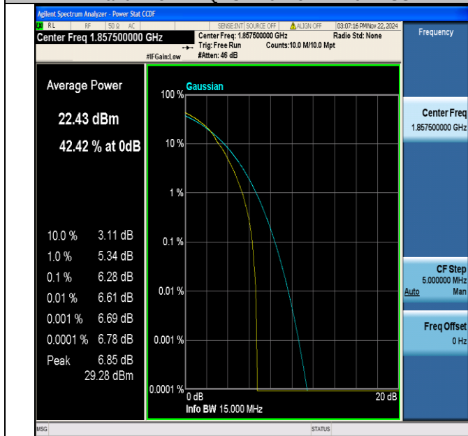
Band2-15MHz-64QAM-18675-1RB#0-PASS
