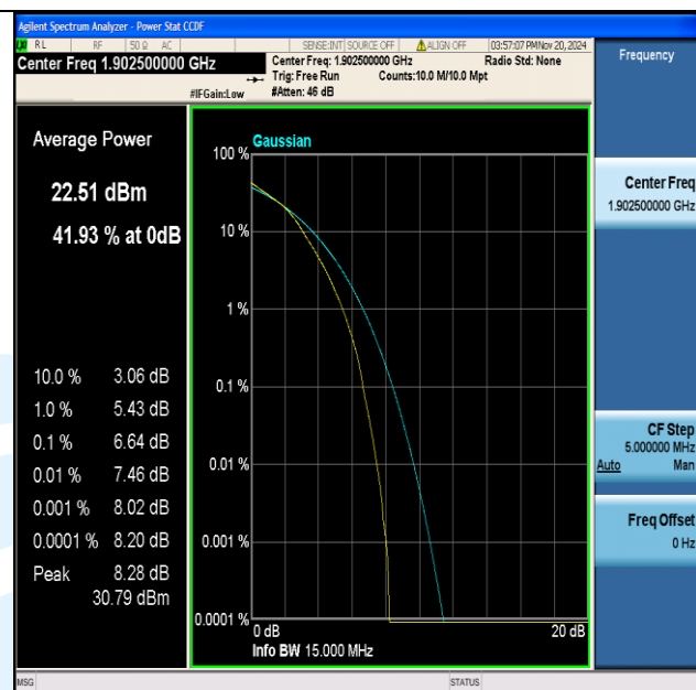
Band2-15MHz-16QAM-19125-75RB#0-PASS
