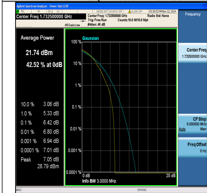
Band4-3MHz-64QAM-20175-1RB#0-PASS
