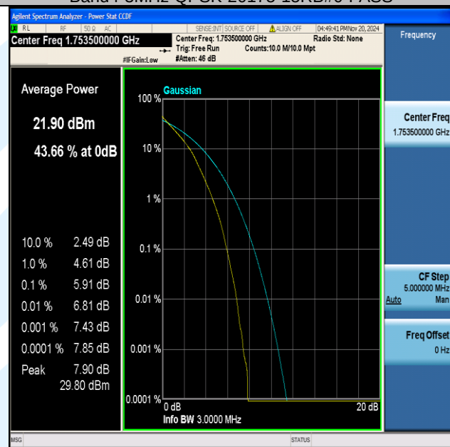
Band4-3MHz-QPSK-20385-15RB#0-PASS
