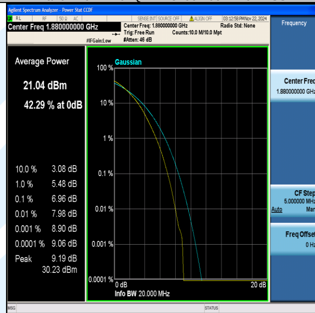
Band2-20MHz-64QAM-18900-100RB#0-PASS
