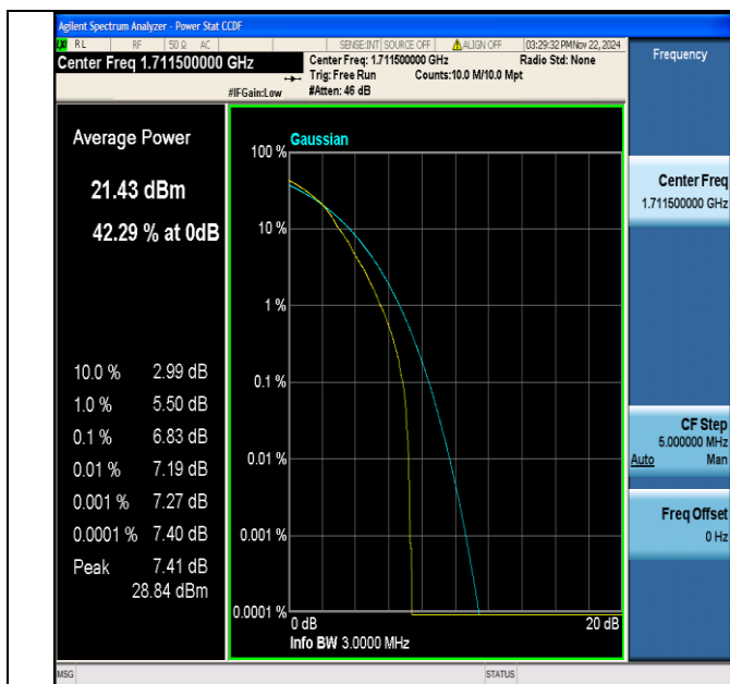
Band4-3MHz-64QAM-19965-1RB#0-PASS
