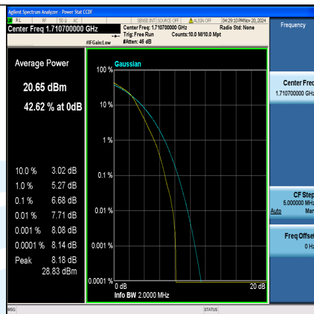
Band4-1.4MHz-16QAM-19957-6RB#0-PASS
