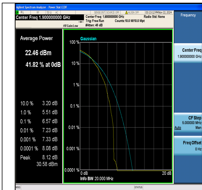
Band2-20MHz-64QAM-19100-1RB#0-PASS
