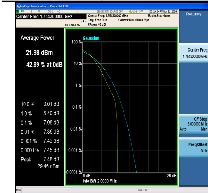
Band4-1.4MHz-64QAM-20393-1RB#0-PASS
