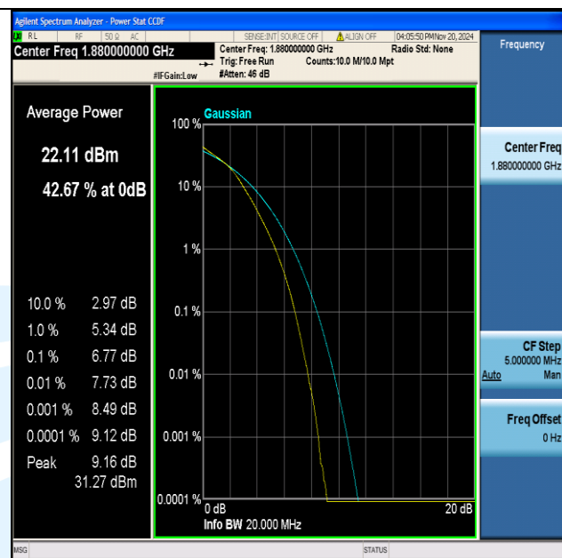
Band2-20MHz-16QAM-18900-100RB#0-PASS
