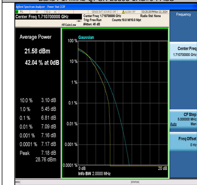
Band4-1.4MHz-64QAM-19957-1RB#0-PASS
