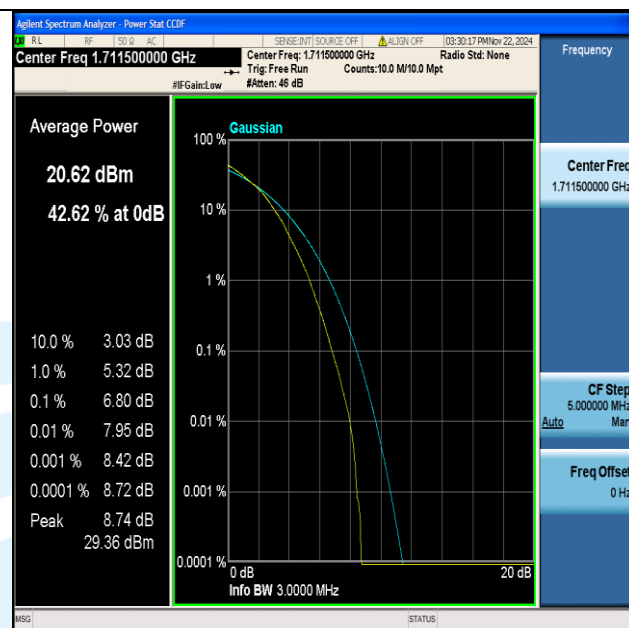
Band4-3MHz-64QAM-19965-15RB#0-PASS
