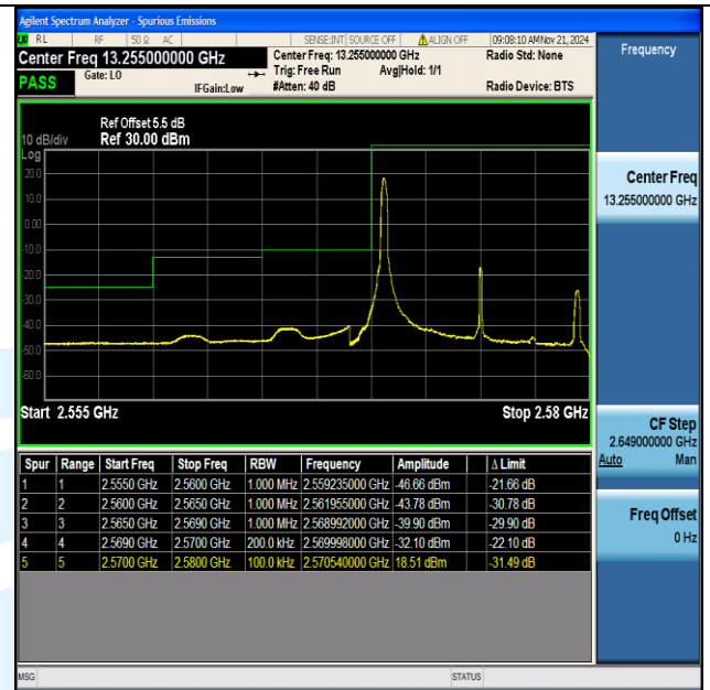
Band38 10MHz 16QAM 37800 1RB#0
