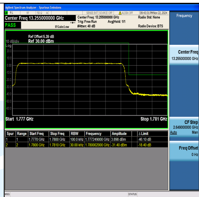
Band66 3MHz 64QAM 132657 15RB#0
