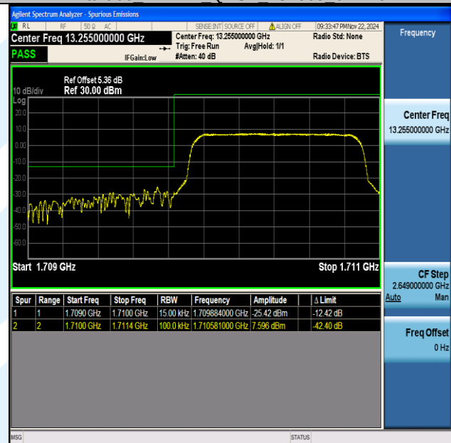
Band66 1.4MHz 64QAM 131979 6RB#0
