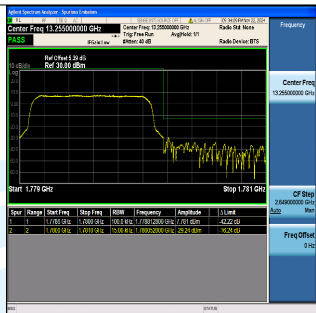
Band66 1.4MHz 64QAM 132665 6RB#0
