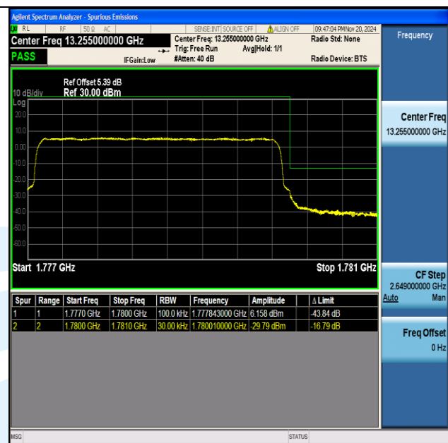
Band66 3MHz QPSK 132657 15RB#0
