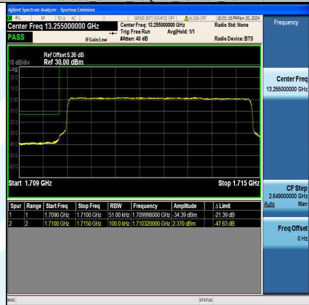
Band66 5MHz QPSK 131997 25RB#0
