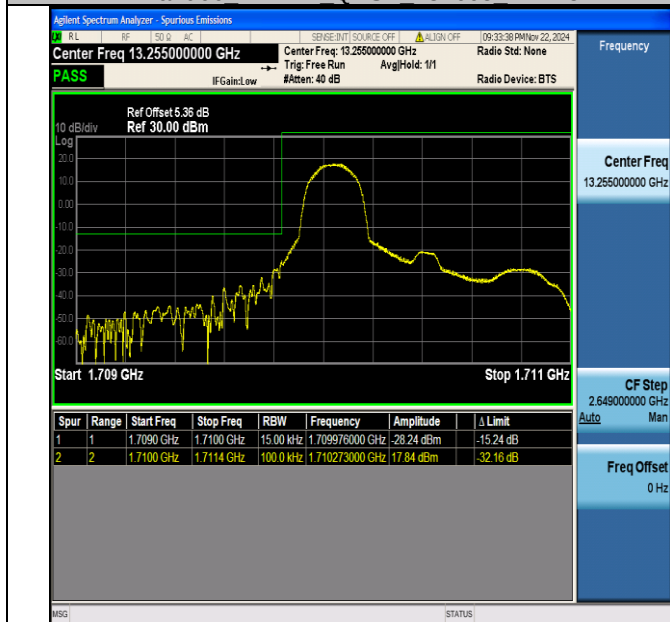
Band66 1.4MHz 64QAM 131979 1RB#0
