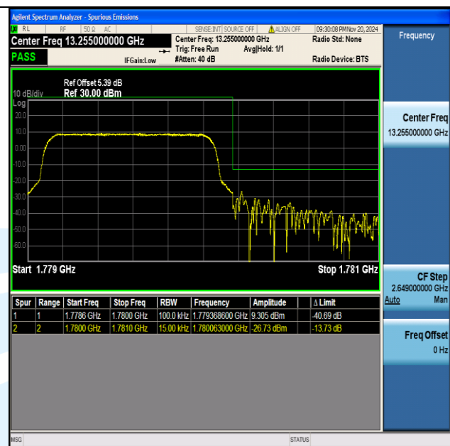
Band66 1.4MHz 16QAM 132665 6RB#0
