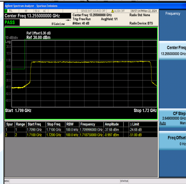
Band66 10MHz 64QAM 132022 50RB#0
