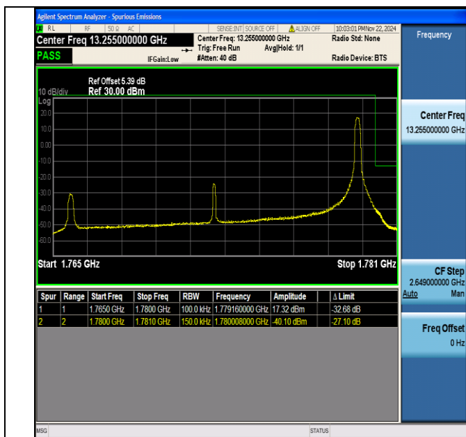
Band66 15MHz 64QAM 132597 1RB#74
