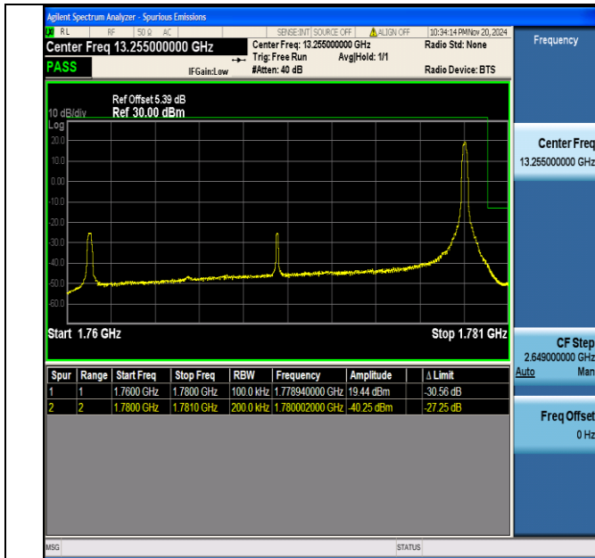
Band66 20MHz 16QAM 132572 1RB#99
