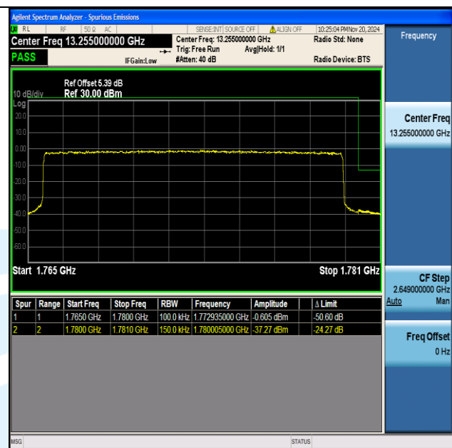
Band66 15MHz QPSK 132597 75RB#0
