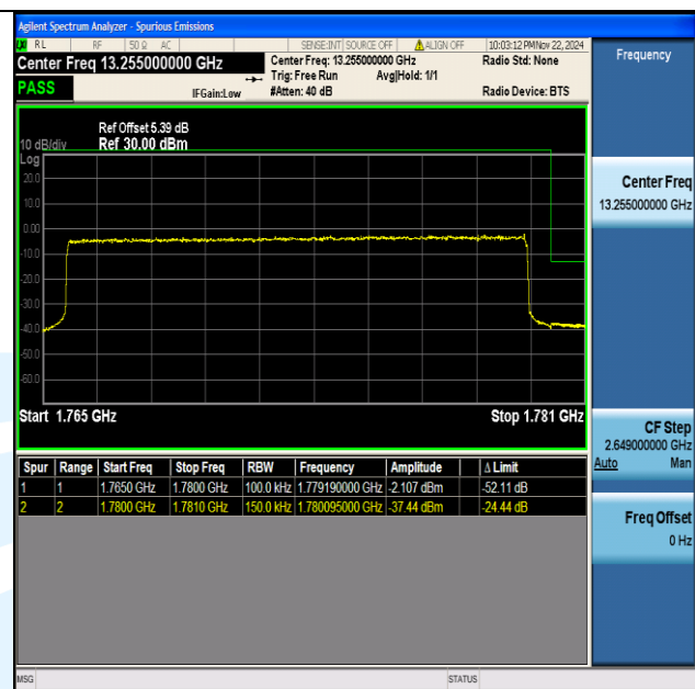
Band66 15MHz 64QAM 132597 75RB#0
