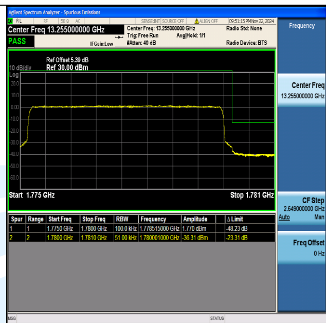
Band66 5MHz 64QAM 132647 25RB#0
