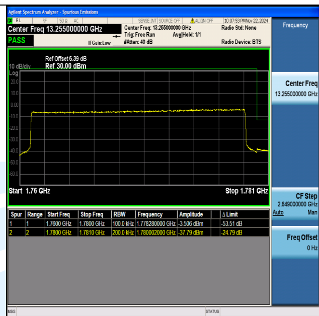
Band66 20MHz 64QAM 132572 100RB#0
