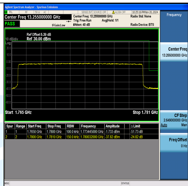
Band66 15MHz 16QAM 132597 75RB#0
