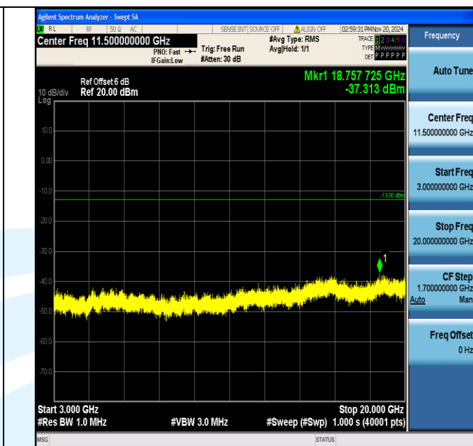
Band2_1.4MHz_QPSK_18900_1RB#0_3000~20000_3000~20000
