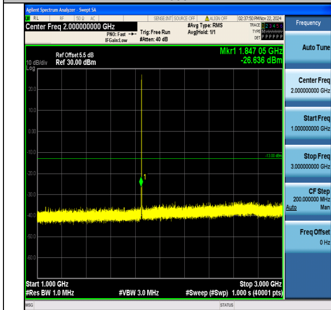
Band2_1.4MHz_64QAM_18607_1RB#0_1000~3000_1000~3000
