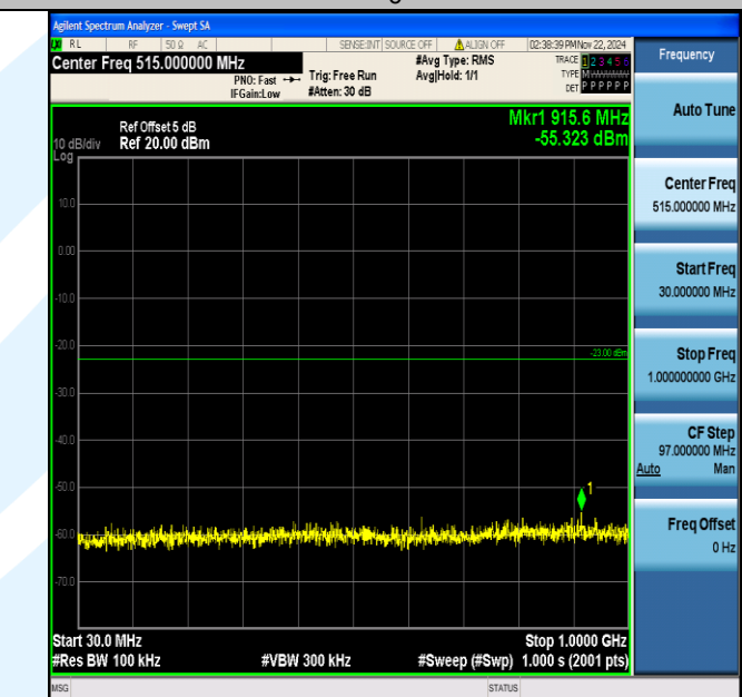
Band2_1.4MHz_64QAM_19193_1RB#0_30~1000_30~1000
