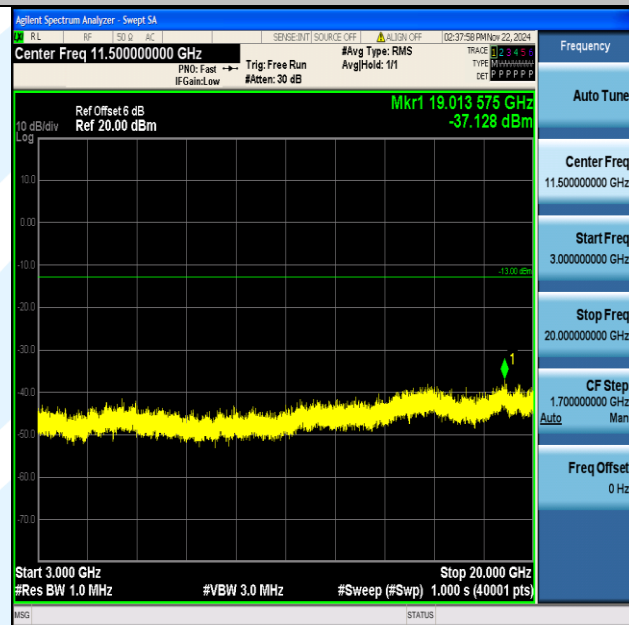
Band2_1.4MHz_64QAM_18607_1RB#0_3000~20000_3000~2000
