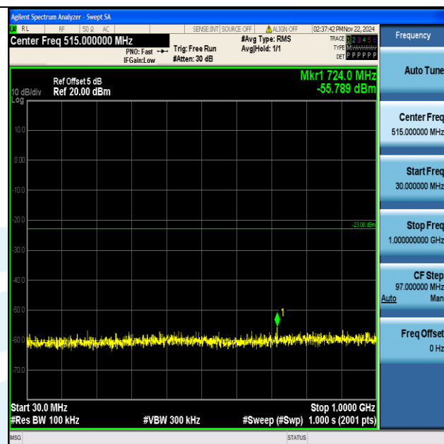
Band2_1.4MHz_64QAM_18607_1RB#0_30~1000_30~1000
