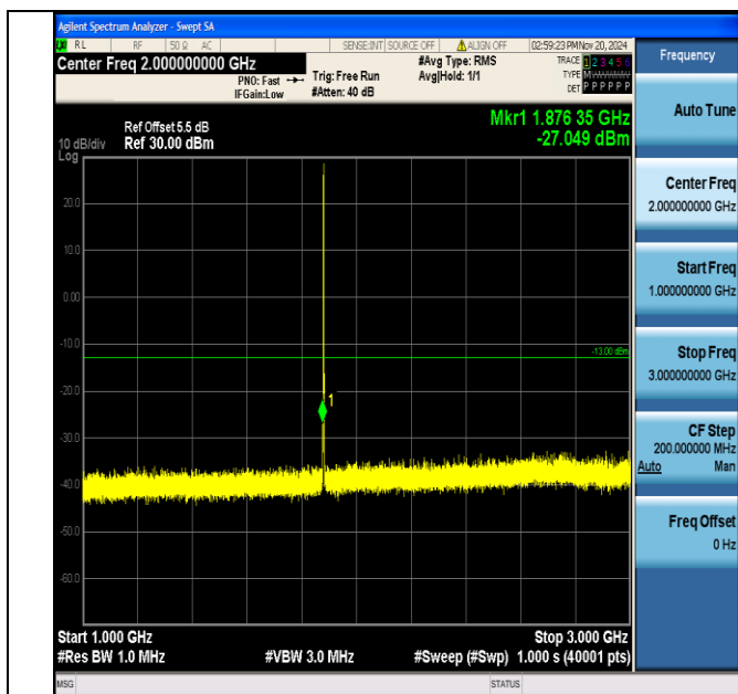
Band2_1.4MHz_QPSK_18900_1RB#0_1000~3000_1000~3000
