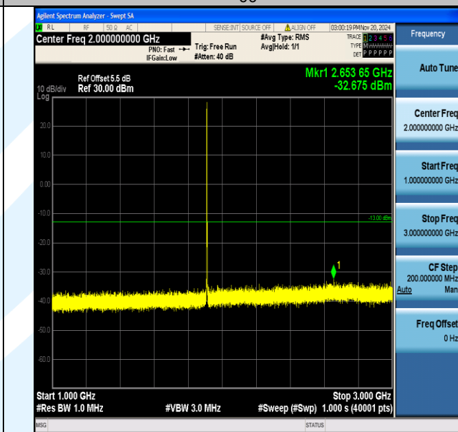
Band2_1.4MHz_QPSK_19193_1RB#0_1000~3000_1000~3000
