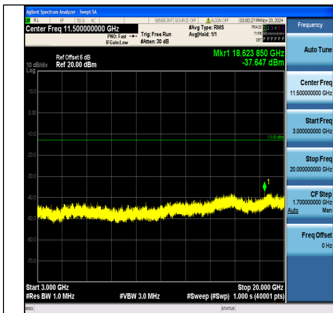
Band2_1.4MHz_QPSK_19193_1RB#0_3000~20000_3000~2000
