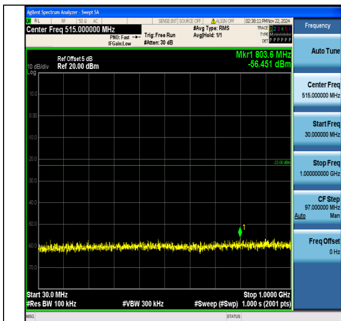
Band2_1.4MHz_64QAM_18900_1RB#0_30~1000_30~1000
