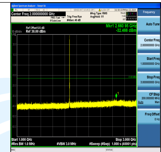
Band2_1.4MHz_64QAM_18900_1RB#0_1000~3000_1000~3000
