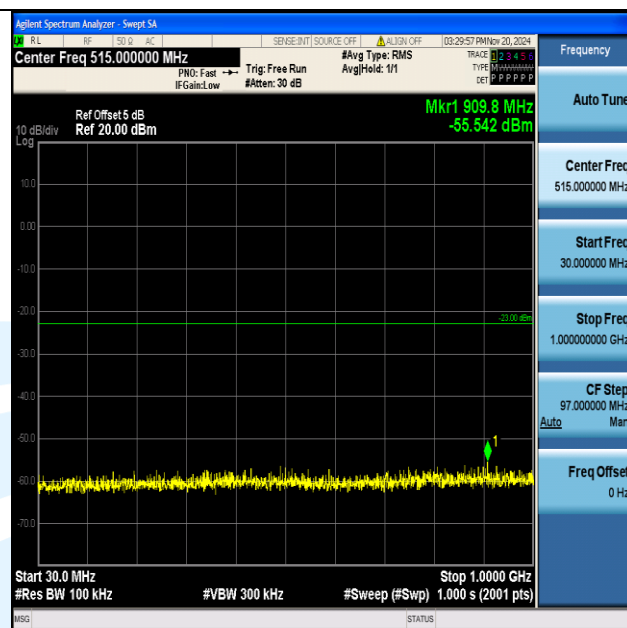
Band2_5MHz_QPSK_18900_1RB#0_30~1000_30~1000
