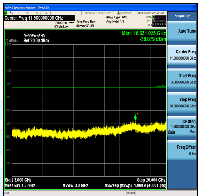
Band2_5MHz_64QAM_18625_1RB#0_3000~20000_3000~20000
