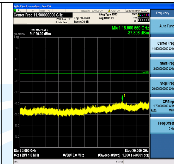
Band2_5MHz_16QAM_18900_1RB#0_3000~20000_3000~20000
