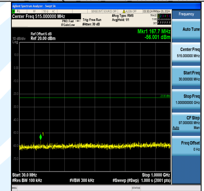
Band2_5MHz_16QAM_18900_1RB#0_30~1000_30~1000
