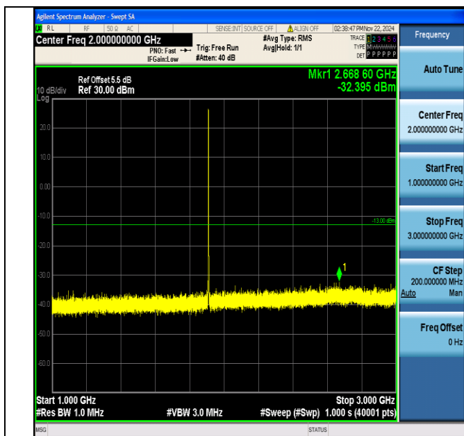
Band2_1.4MHz_64QAM_19193_1RB#0_1000~3000_1000~3000
