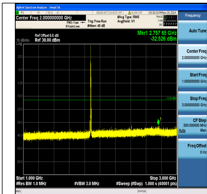
Band2_5MHz_16QAM_18900_1RB#0_1000~3000_1000~3000
