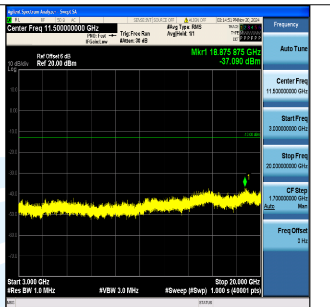
Band2_3MHz_QPSK_18615_1RB#0_3000~20000_3000~20000
