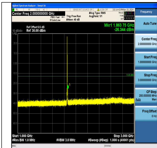
Band2_3MHz_QPSK_18615_1RB#0_1000~3000_1000~3000
