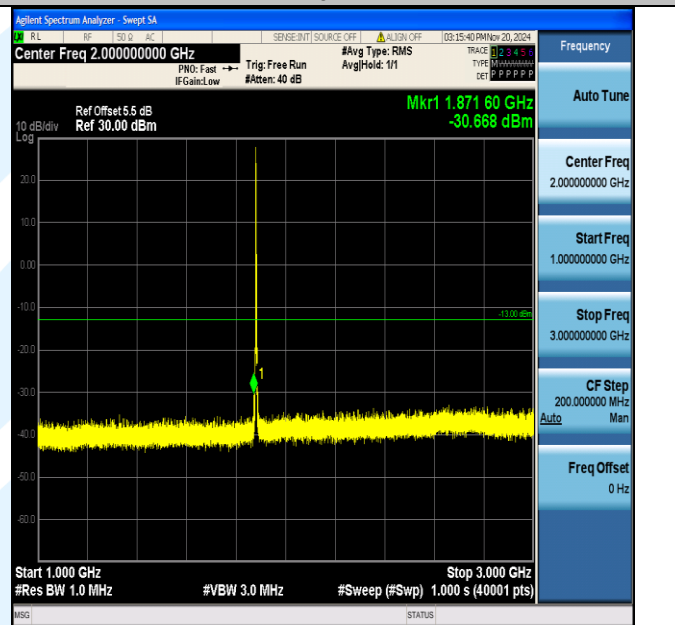
Band2_3MHz_QPSK_18900_1RB#0_1000~3000_1000~3000
