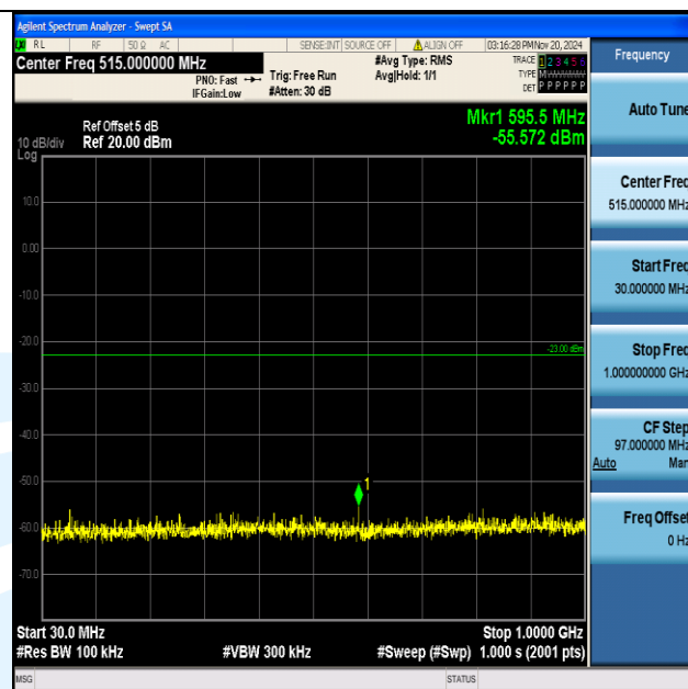
Band2_3MHz_QPSK_19185_1RB#0_30~1000_30~1000
