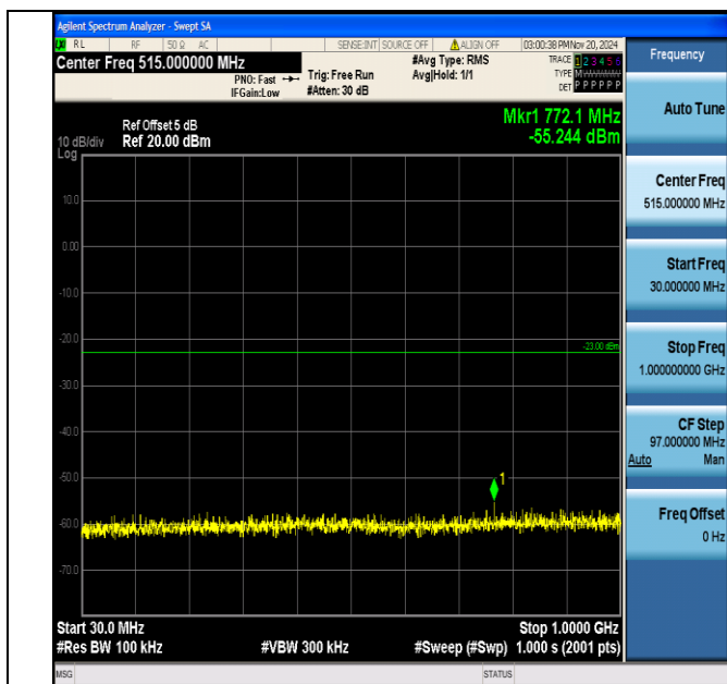
Band2_1.4MHz_16QAM_19193_1RB#0_30~1000_30~1000
