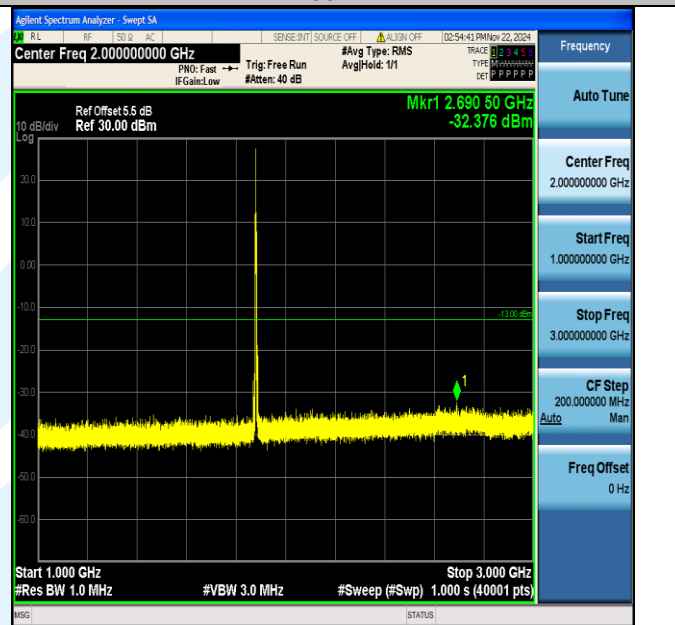
Band2_5MHz_64QAM_18900_1RB#0_1000~3000_1000~3000
