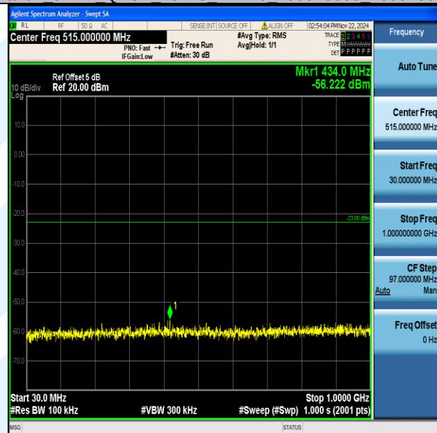
Band2_5MHz_64QAM_18625_1RB#0_30~1000_30~1000
