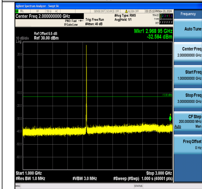
Band2_3MHz_16QAM_18615_1RB#0_1000~3000_1000~3000
