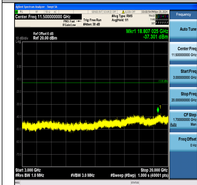
Band2_1.4MHz_16QAM_19193_1RB#0_3000~20000_3000~20000
