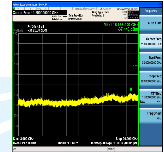
Band2_3MHz_64QAM_18900_1RB#0_3000~20000_3000~20000
