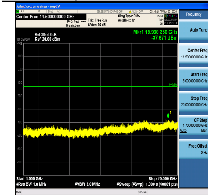
Band2_3MHz_16QAM_18900_1RB#0_3000~20000_3000~20000
