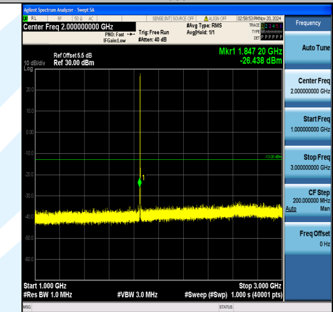
Band2_1.4MHz_16QAM_18607_1RB#0_1000~3000_1000~3000
