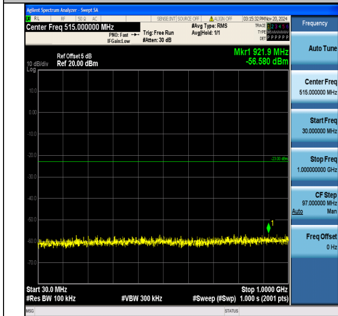
Band2_3MHz_QPSK_18900_1RB#0_30~1000_30~1000
