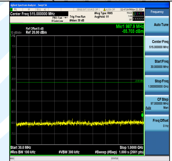
Band2_3MHz_64QAM_18900_1RB#0_30~1000_30~1000
