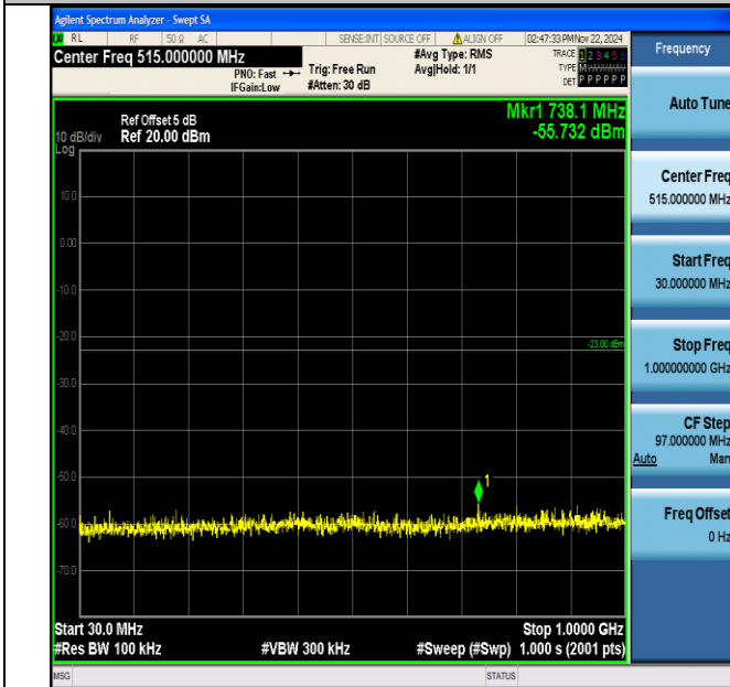
Band2_3MHz_64QAM_19185_1RB#0_30~1000_30~1000
