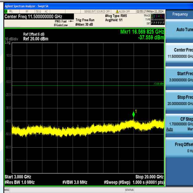
Band2_5MHz_64QAM_19175_1RB#0_3000~20000_3000~20000
