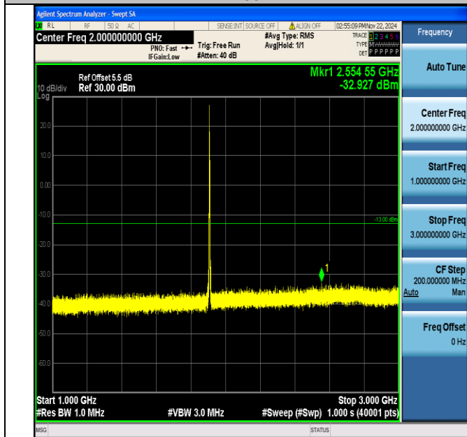
Band2_5MHz_64QAM_19175_1RB#0_1000~3000_1000~3000
