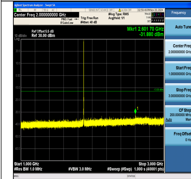
Band2_1.4MHz_16QAM_18900_1RB#0_1000~3000_1000~3000
