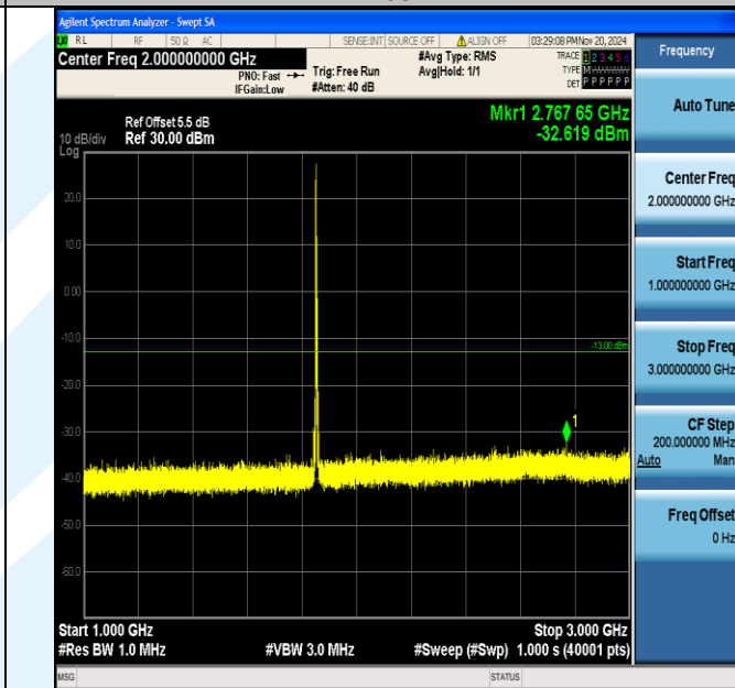
Band2_5MHz_QPSK_18625_1RB#0_1000~3000_1000~3000
