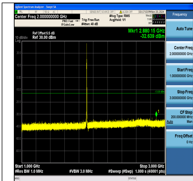
Band2_3MHz_16QAM_19185_1RB#0_1000~3000_1000~3000
