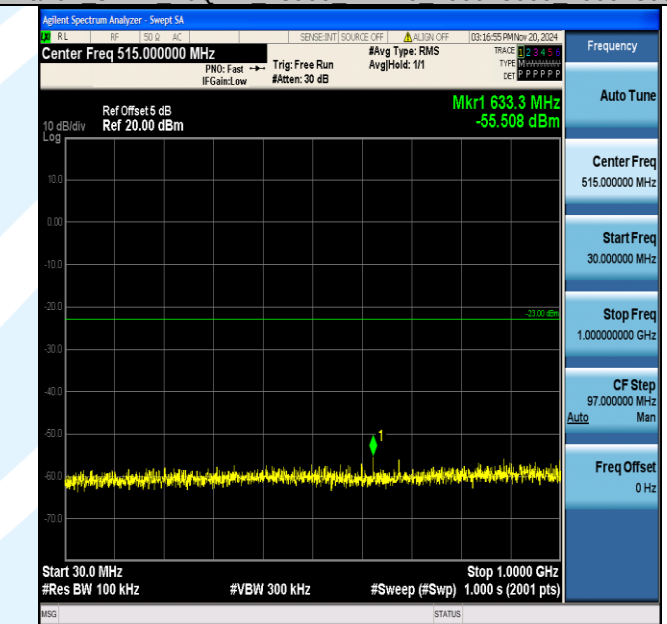
Band2_3MHz_16QAM_19185_1RB#0_30~1000_30~1000
