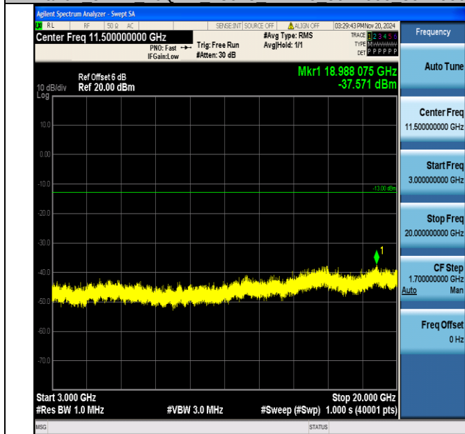
Band2_5MHz_16QAM_18625_1RB#0_3000~20000_3000~20000
