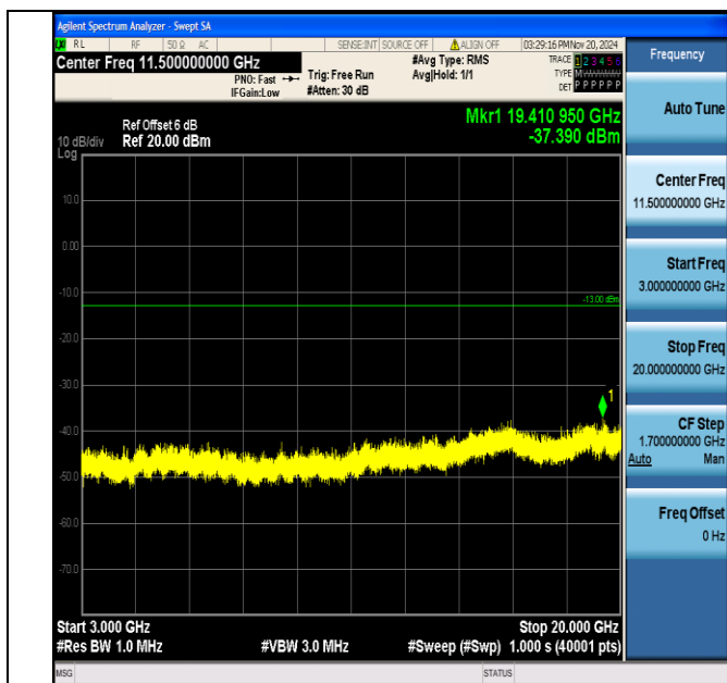
Band2_5MHz_QPSK_18625_1RB#0_3000~20000_3000~2000 0
