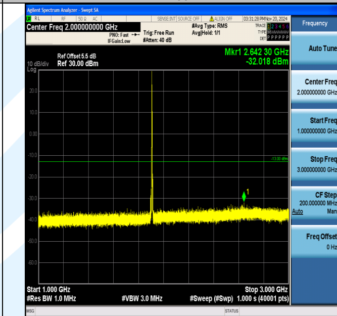
Band2_5MHz_16QAM_19175_1RB#0_1000~3000_1000~3000
