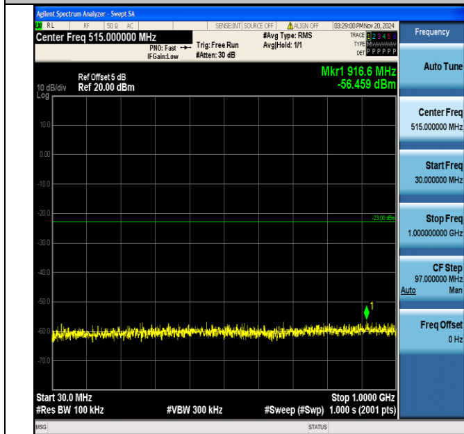
Band2_5MHz_QPSK_18625_1RB#0_30~1000_30~1000
