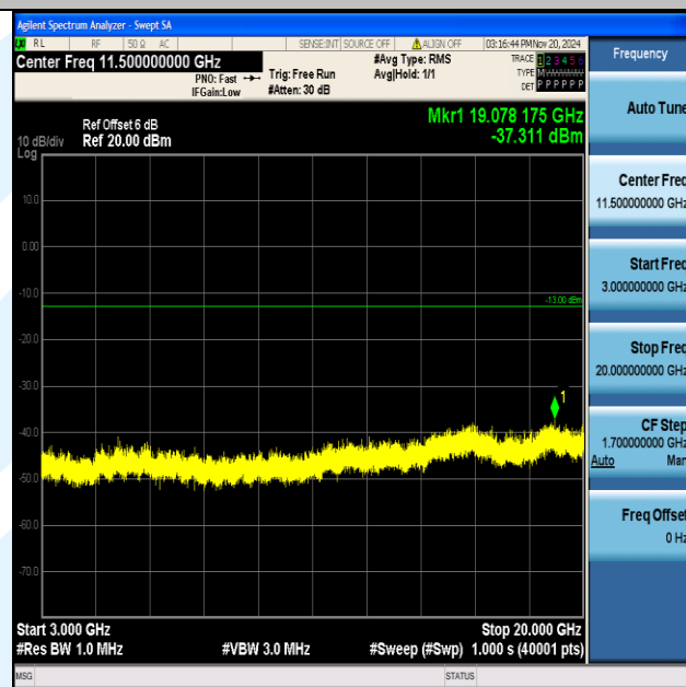
Band2_3MHz_QPSK_19185_1RB#0_3000~20000_3000~2000 0
