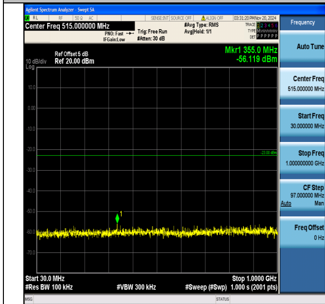
Band2_5MHz_16QAM_19175_1RB#0_30~1000_30~1000
