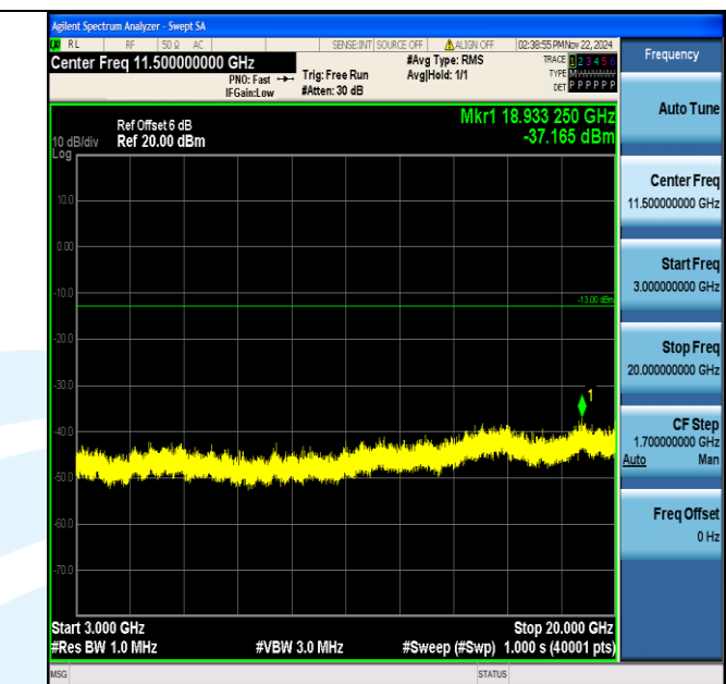
Band2_1.4MHz_64QAM_19193_1RB#0_3000~20000_3000~20000
