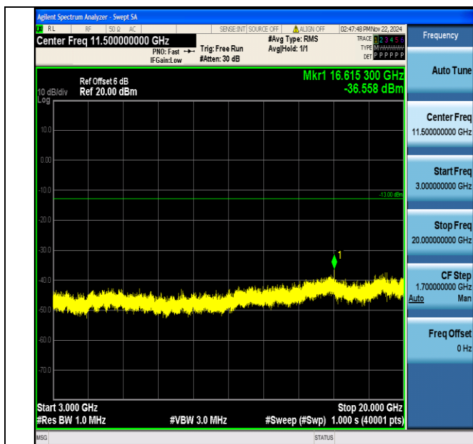
Band2_3MHz_64QAM_19185_1RB#0_3000~20000_3000~20000
