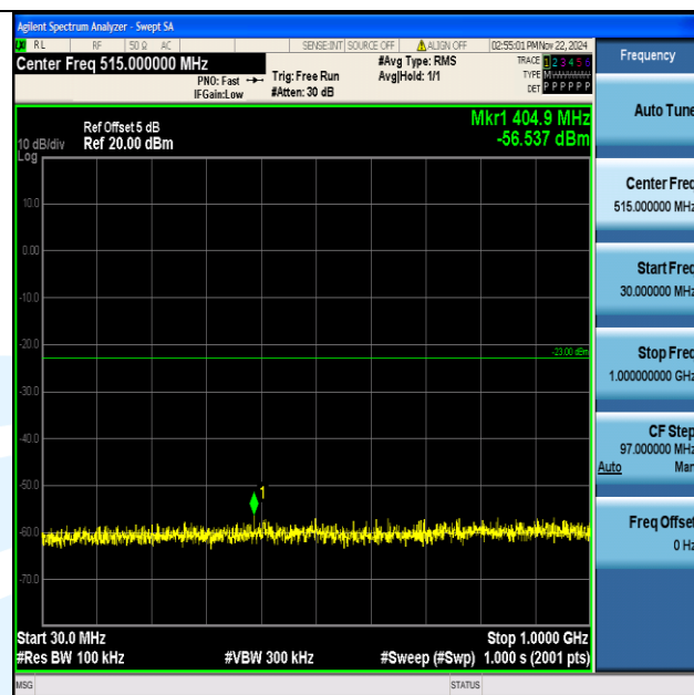
Band2_5MHz_64QAM_19175_1RB#0_30~1000_30~1000
