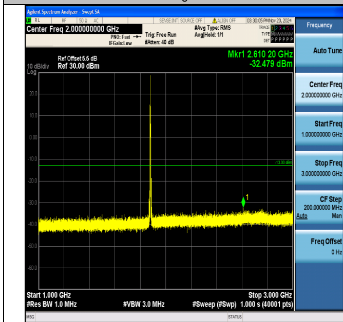
Band2_5MHz_QPSK_18900_1RB#0_1000~3000_1000~3000
