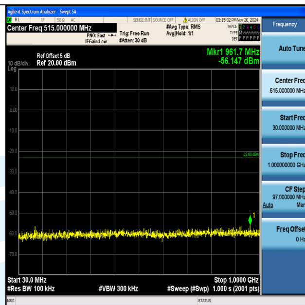
Band2_3MHz_16QAM_18615_1RB#0_30~1000_30~1000
