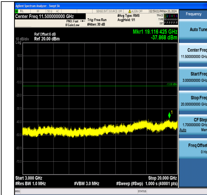
Band2_1.4MHz_16QAM_18607_1RB#0_3000~20000_3000~20000
