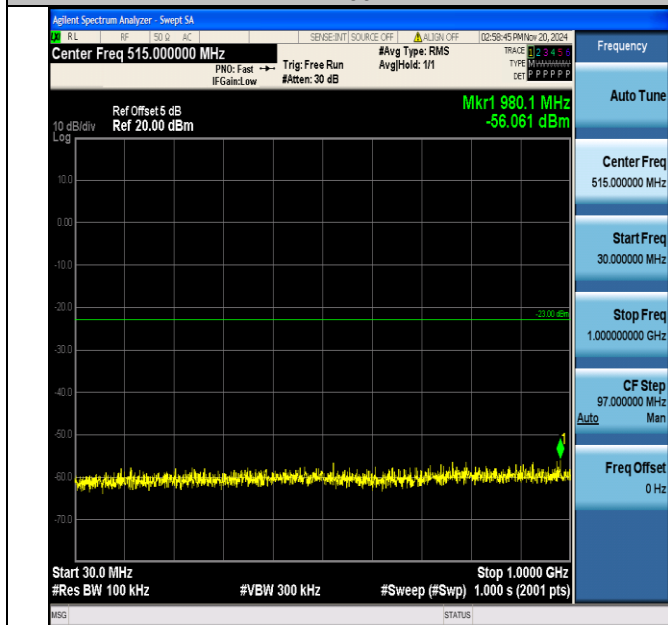
Band2_1.4MHz_16QAM_18607_1RB#0_30~1000_30~1000
