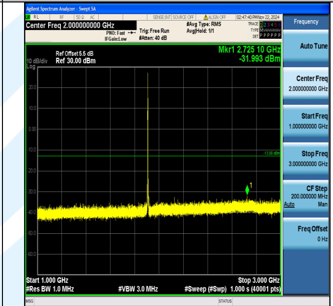
Band2_3MHz_64QAM_19185_1RB#0_1000~3000_1000~3000
