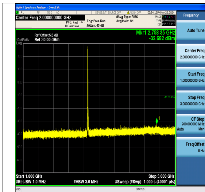
Band2_5MHz_64QAM_18625_1RB#0_1000~3000_1000~3000
