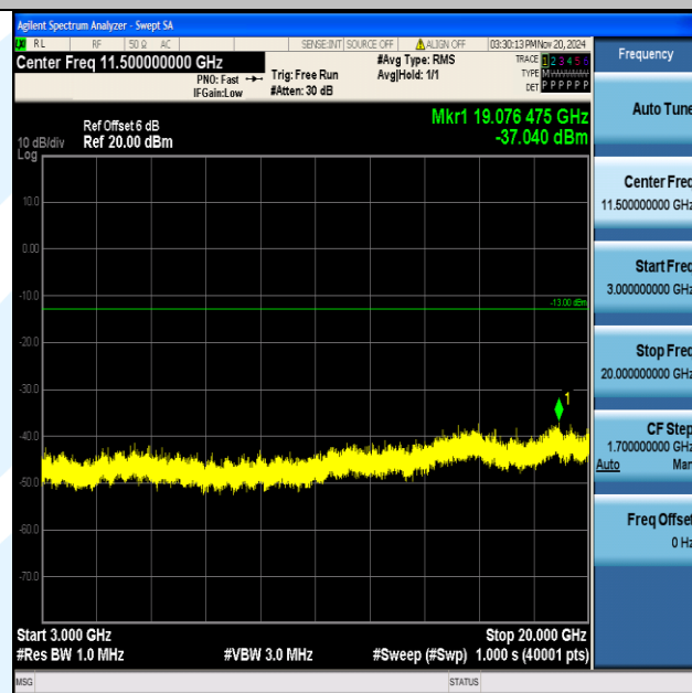
Band2_5MHz_QPSK_18900_1RB#0_3000~20000_3000~2000 0
