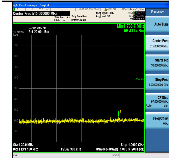
Band2_5MHz_64QAM_18900_1RB#0_30~1000_30~1000
