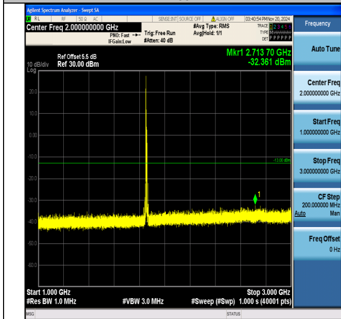
Band2_10MHz_QPSK_18650_1RB#0_1000~3000_1000~3000
