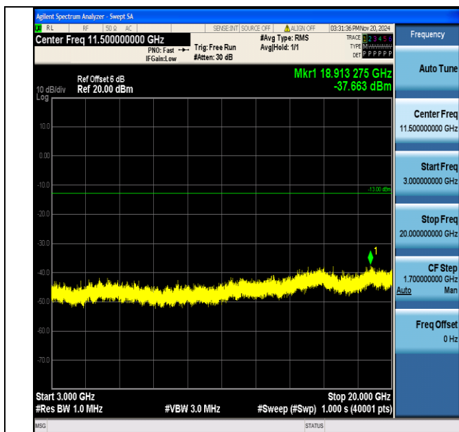
Band2_5MHz_16QAM_19175_1RB#0_3000~20000_3000~20000
