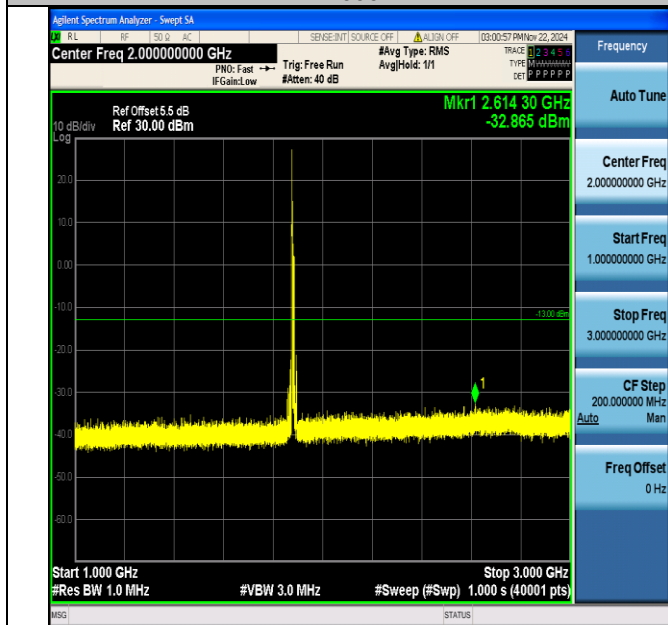
Band2_10MHz_64QAM_18900_1RB#0_1000~3000_1000~3000
