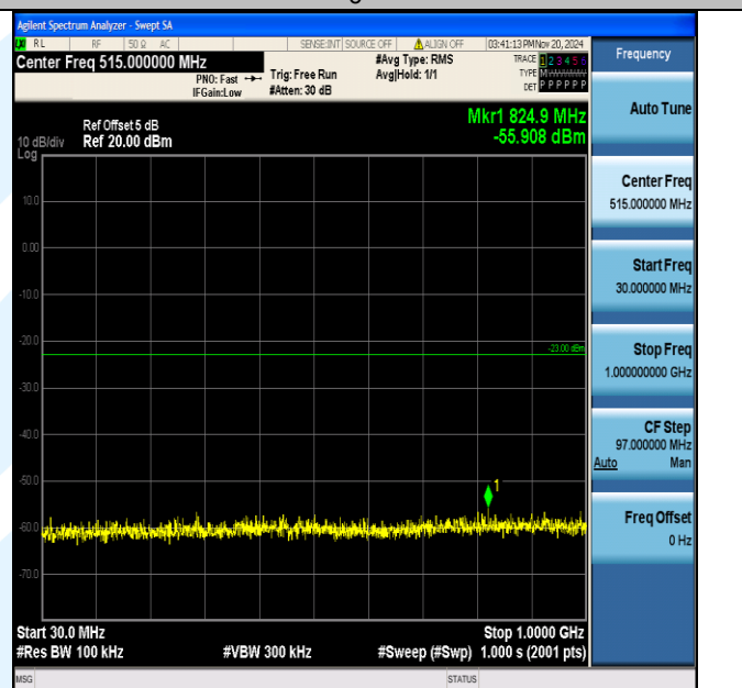
Band2_10MHz_16QAM_18650_1RB#0_30~1000_30~1000
