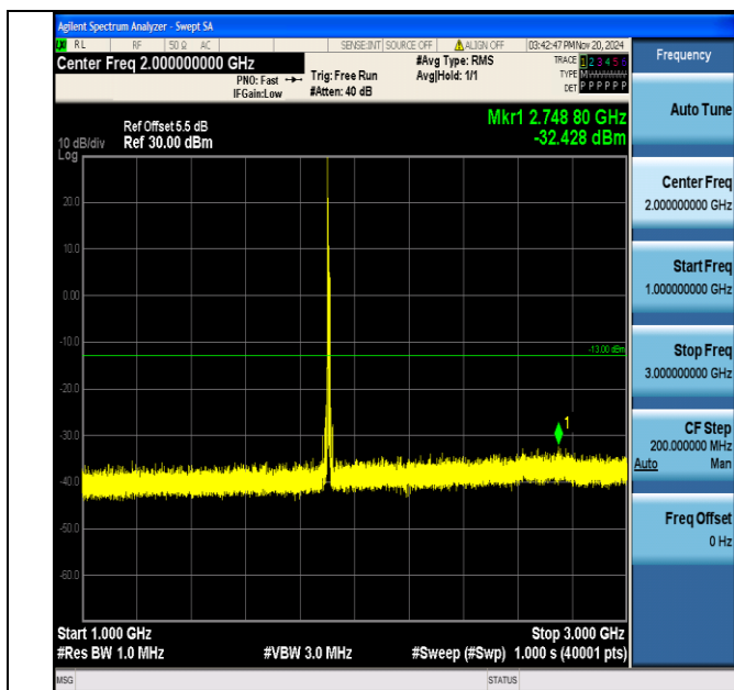
Band2_10MHz_QPSK_19150_1RB#0_1000~3000_1000~3000
