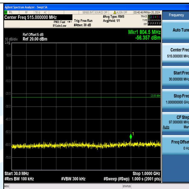
Band2_10MHz_QPSK_18650_1RB#0_30~1000_30~1000
