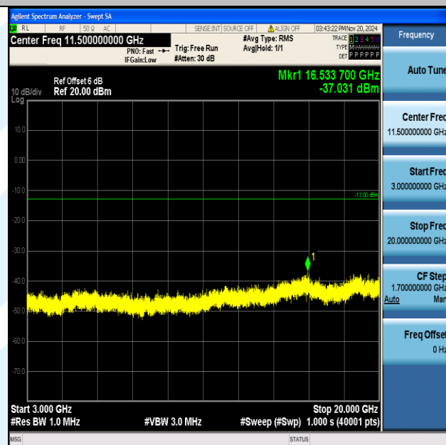
Band2_10MHz_16QAM_19150_1RB#0_3000~20000_3000~20000
