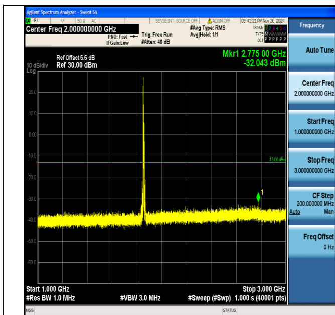
Band2_10MHz_16QAM_18650_1RB#0_1000~3000_1000~3000
