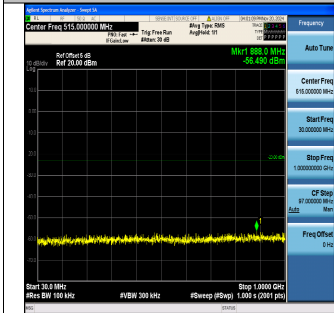
Band2_20MHz_QPSK_18900_1RB#0_30~1000_30~1000
