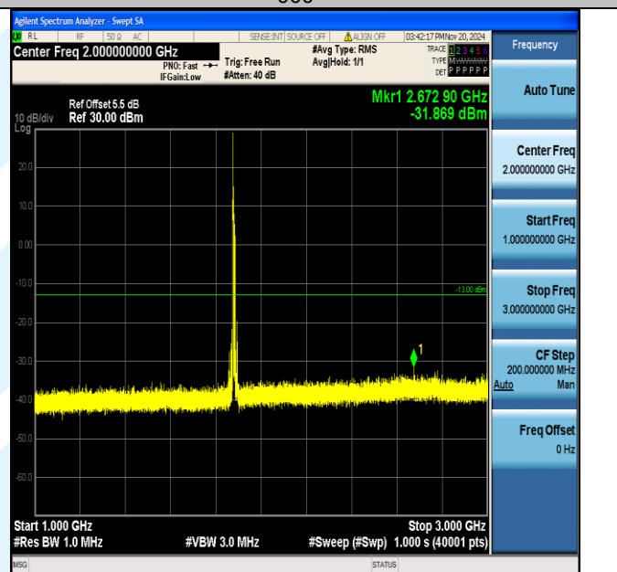
Band2_10MHz_16QAM_18900_1RB#0_1000~3000_1000~3000
