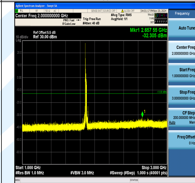
Band2_20MHz_QPSK_18900_1RB#0_1000~3000_1000~3000
