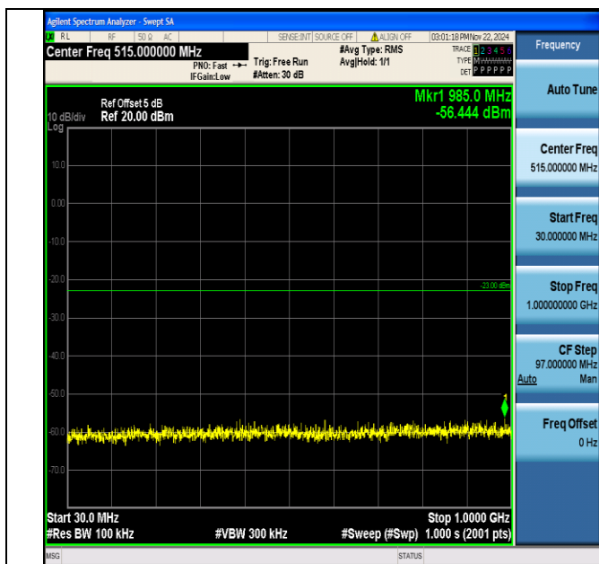
Band2_10MHz_64QAM_19150_1RB#0_30~1000_30~1000
