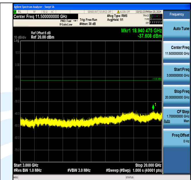
Band2_15MHz_QPSK_18900_1RB#0_3000~20000_3000~20000
