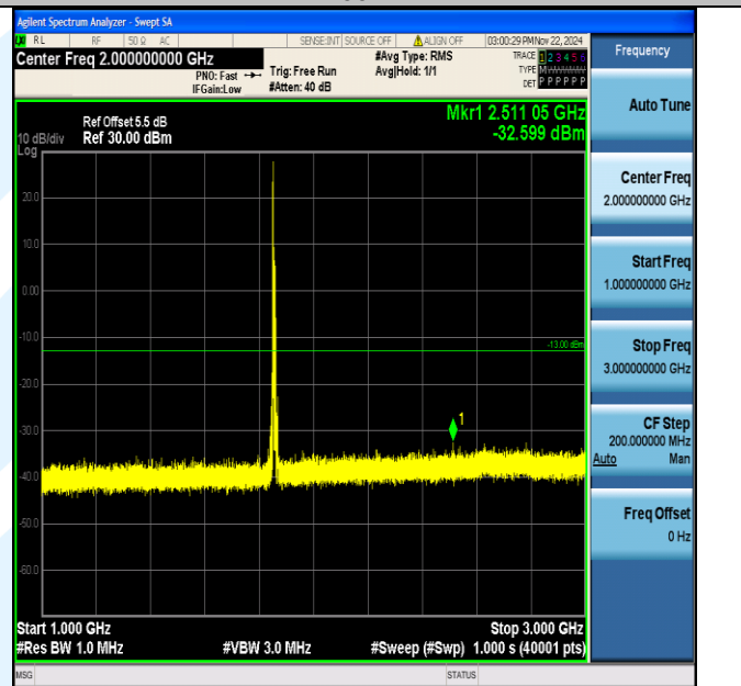
Band2_10MHz_64QAM_18650_1RB#0_1000~3000_1000~3000
