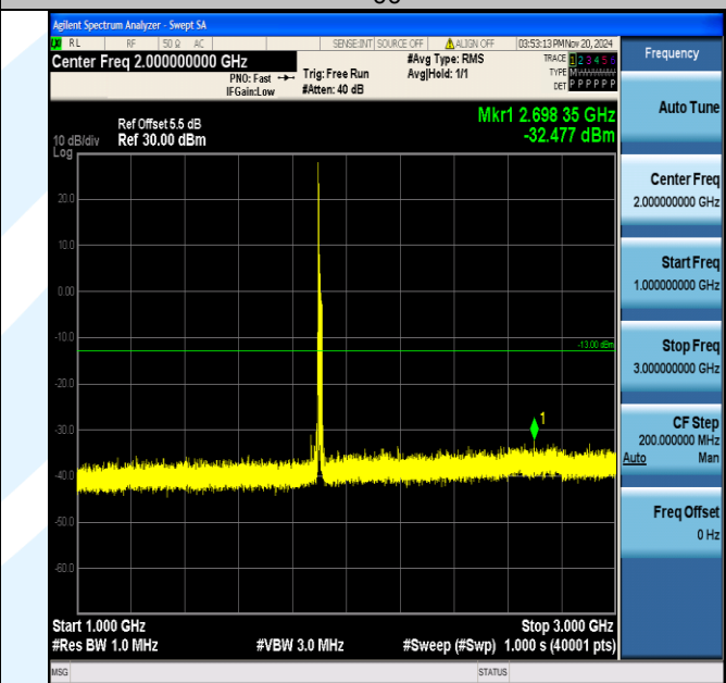
Band2_15MHz_QPSK_19125_1RB#0_1000~3000_1000~3000
