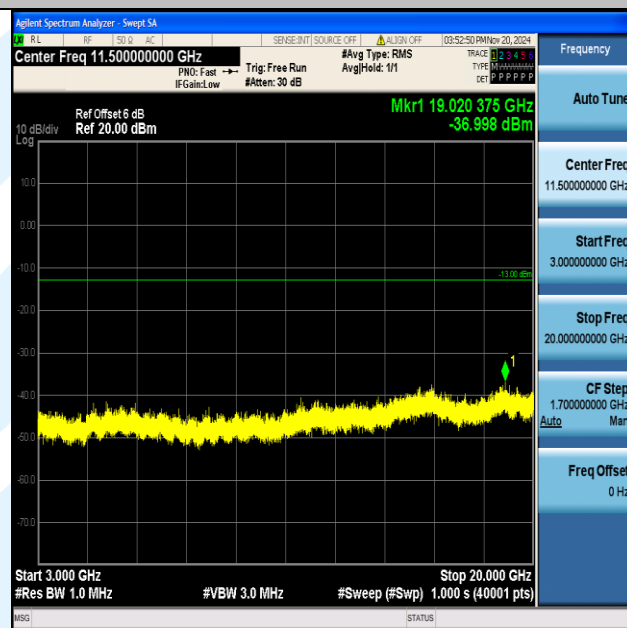
Band2_15MHz_16QAM_18900_1RB#0_3000~20000_3000~20000
