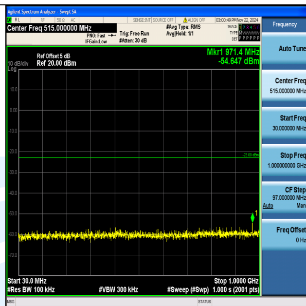
Band2_10MHz_64QAM_18900_1RB#0_30~1000_30~1000
