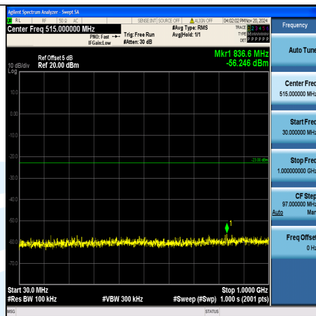
Band2_20MHz_QPSK_19100_1RB#0_30~1000_30~1000
