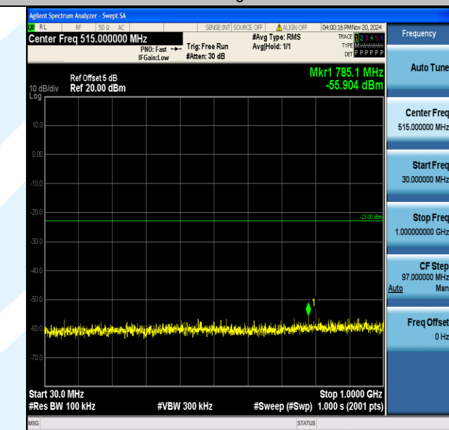
Band2_20MHz_QPSK_18700_1RB#0_30~1000_30~1000
