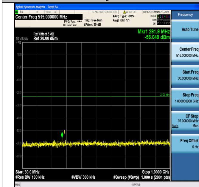
Band2_10MHz_16QAM_18900_1RB#0_30~1000_30~1000
