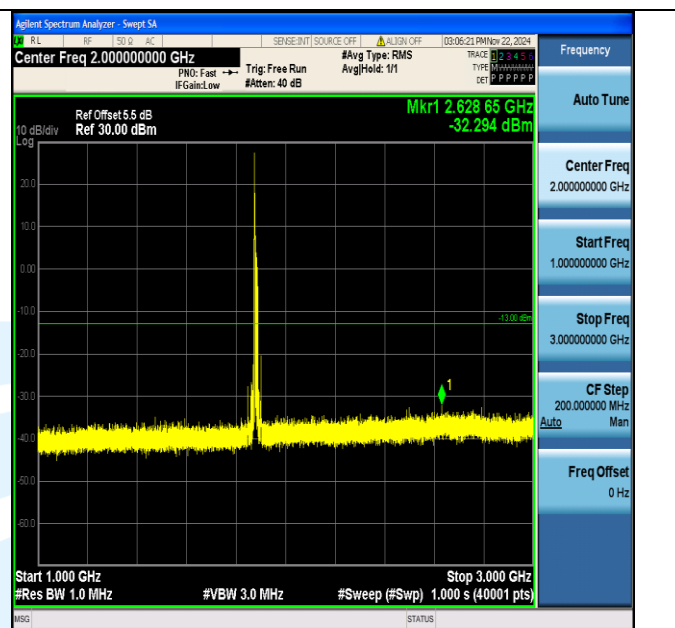
Band2_15MHz_64QAM_18900_1RB#0_1000~3000_1000~3000
