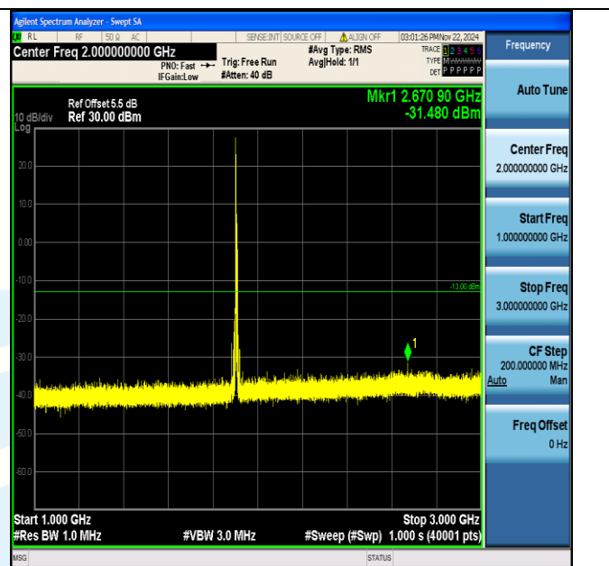
Band2_10MHz_64QAM_19150_1RB#0_1000~3000_1000~3000
