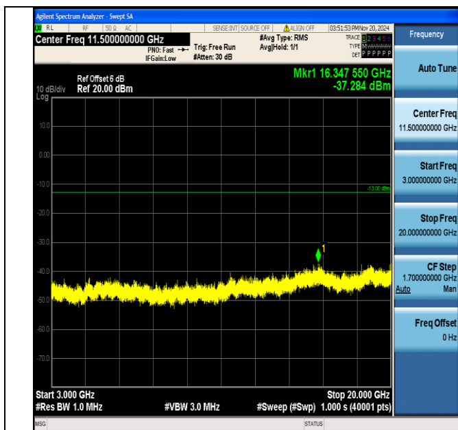
Band2_15MHz_16QAM_18675_1RB#0_3000~20000_3000~20000
