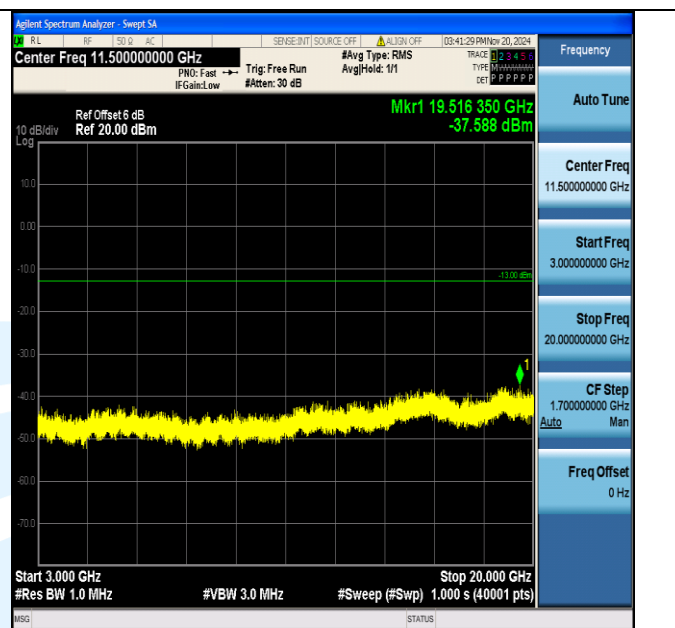
Band2_10MHz_16QAM_18650_1RB#0_3000~20000_3000~20000
