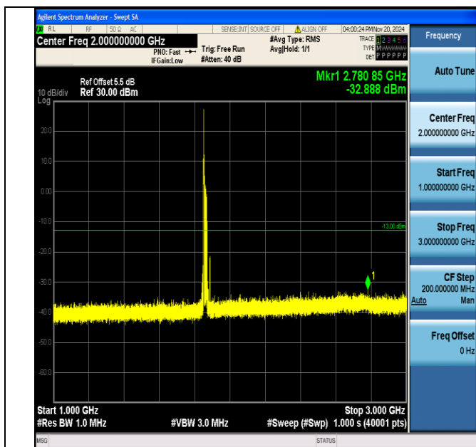
Band2_20MHz_QPSK_18700_1RB#0_1000~3000_1000~3000
