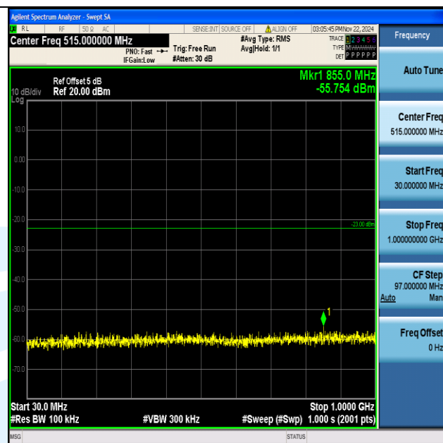
Band2_15MHz_64QAM_18675_1RB#0_30~1000_30~1000
