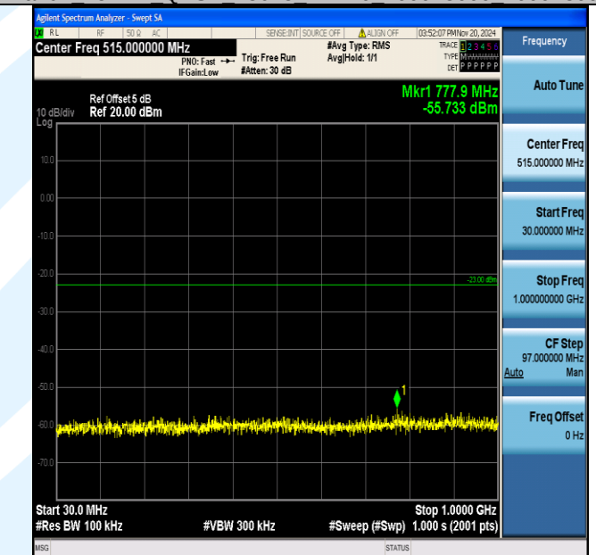
Band2_15MHz_QPSK_18900_1RB#0_30~1000_30~1000
