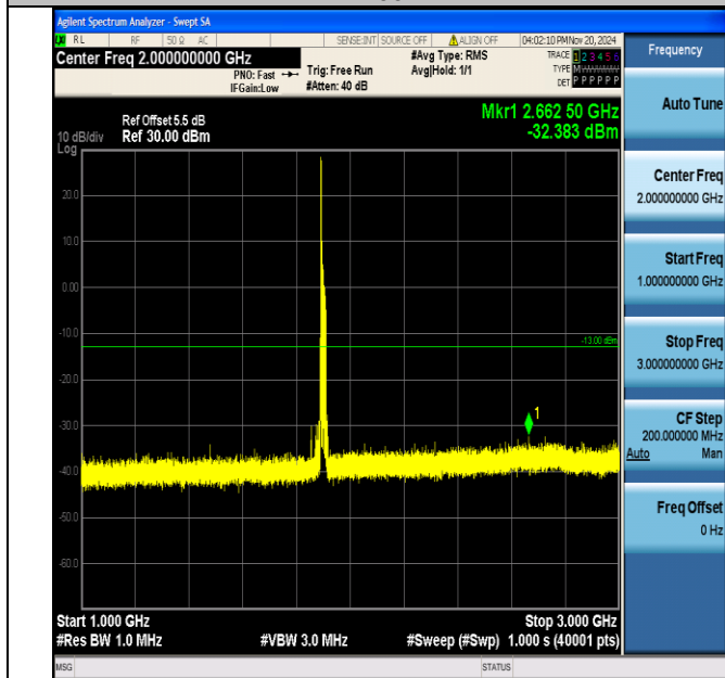
Band2_20MHz_QPSK_19100_1RB#0_1000~3000_1000~3000
