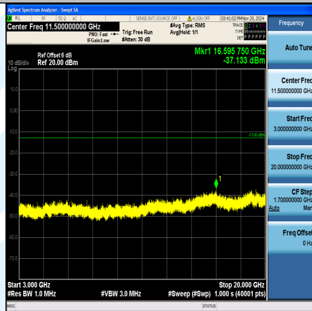
Band2_10MHz_QPSK_18650_1RB#0_3000~20000_3000~20000
