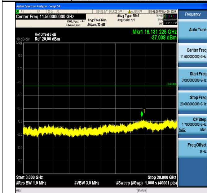
Band2_10MHz_QPSK_18900_1RB#0_3000~20000_3000~20000
