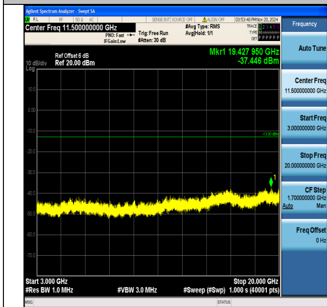
Band2_15MHz_16QAM_19125_1RB#0_3000~20000_3000~20000 000
