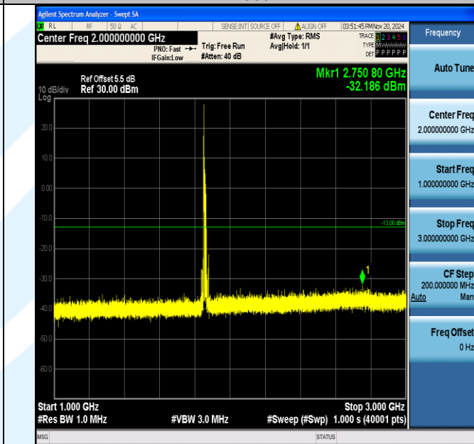
Band2_15MHz_16QAM_18675_1RB#0_1000~3000_1000~3000
