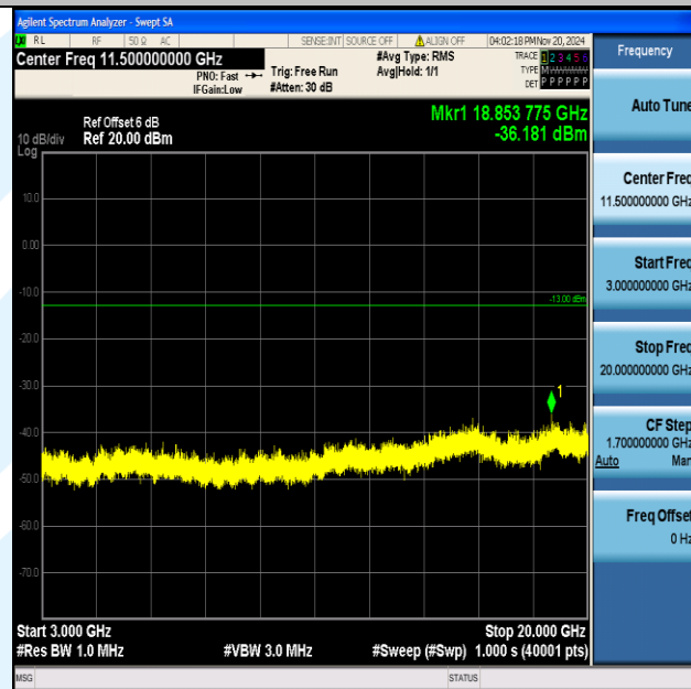
Band2_20MHz_QPSK_19100_1RB#0_3000~20000_3000~20000
