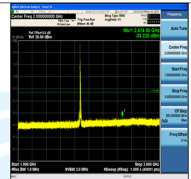
Band2_10MHz_QPSK_18900_1RB#0_1000~3000_1000~3000
