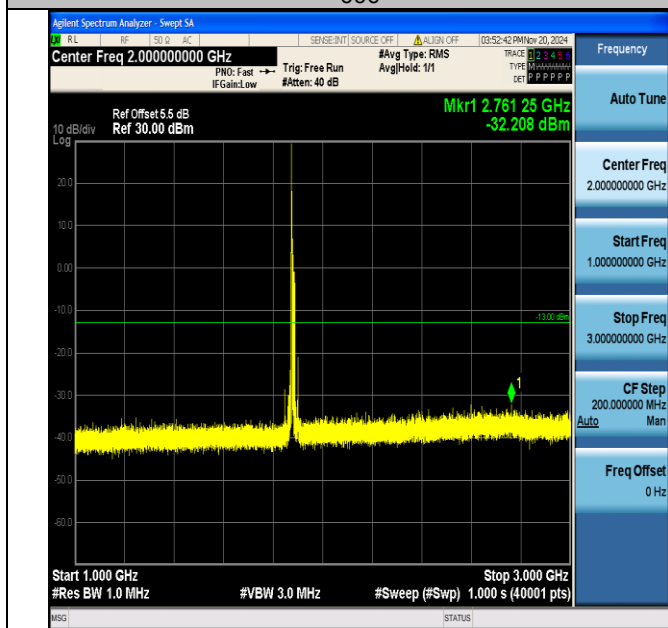
Band2_15MHz_16QAM_18900_1RB#0_1000~3000_1000~3000
