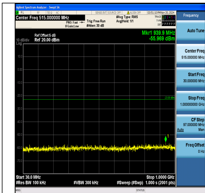
Band2_15MHz_QPSK_18675_1RB#0_30~1000_30~1000
