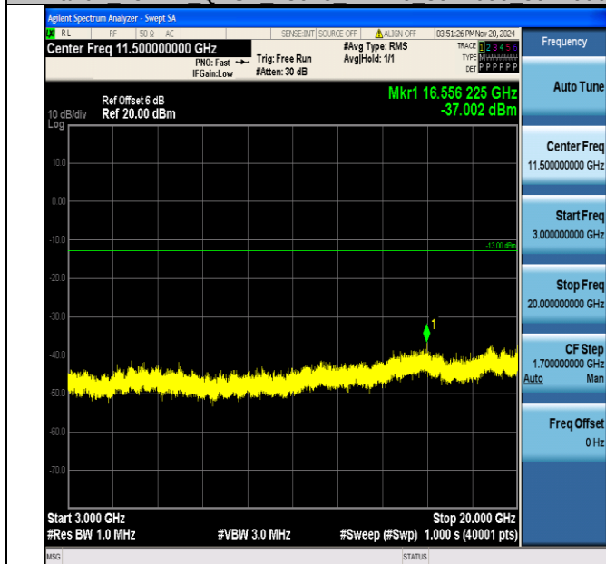
Band2_15MHz_QPSK_18675_1RB#0_3000~20000_3000~20000
