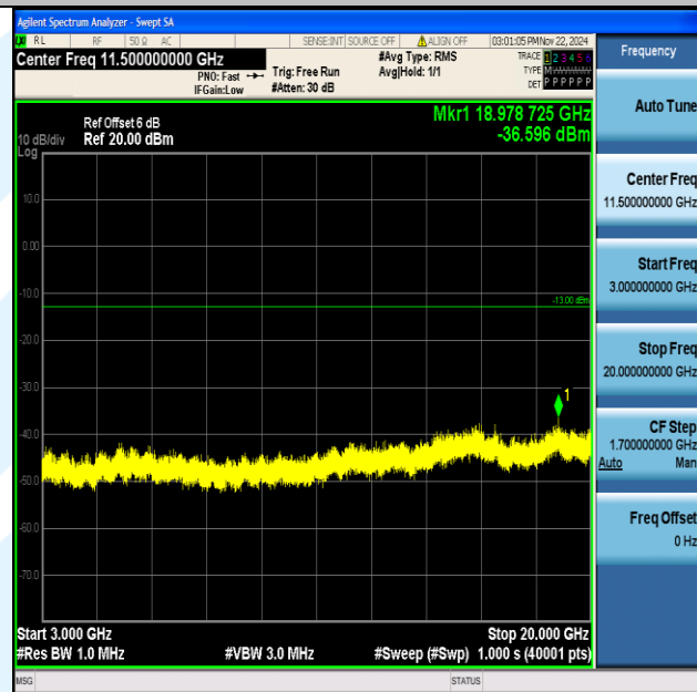
Band2_10MHz_64QAM_18900_1RB#0_3000~20000_3000~20000
