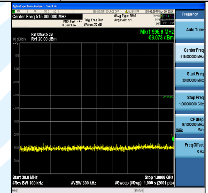
Band2_10MHz_QPSK_19150_1RB#0_30~1000_30~1000
