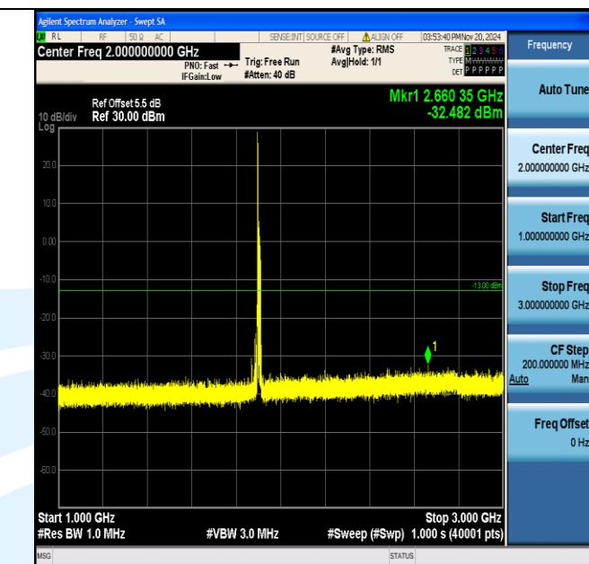
Band2_15MHz_16QAM_19125_1RB#0_1000~3000_1000~3000 0
