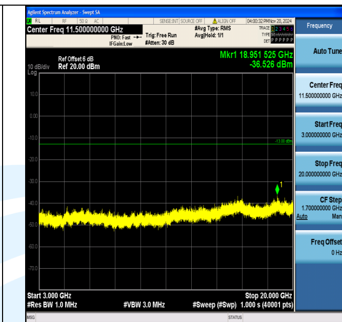
Band2_20MHz_QPSK_18700_1RB#0_3000~20000_3000~20000
