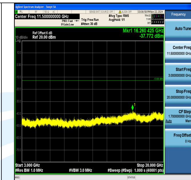
Band2_15MHz_64QAM_19125_1RB#0_3000~20000_3000~20000
