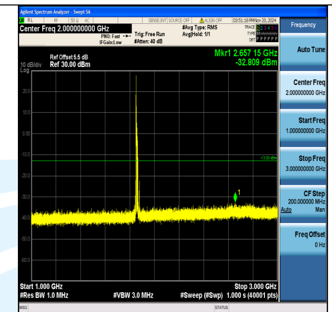
Band2_15MHz_QPSK_18675_1RB#0_1000~3000_1000~3000
