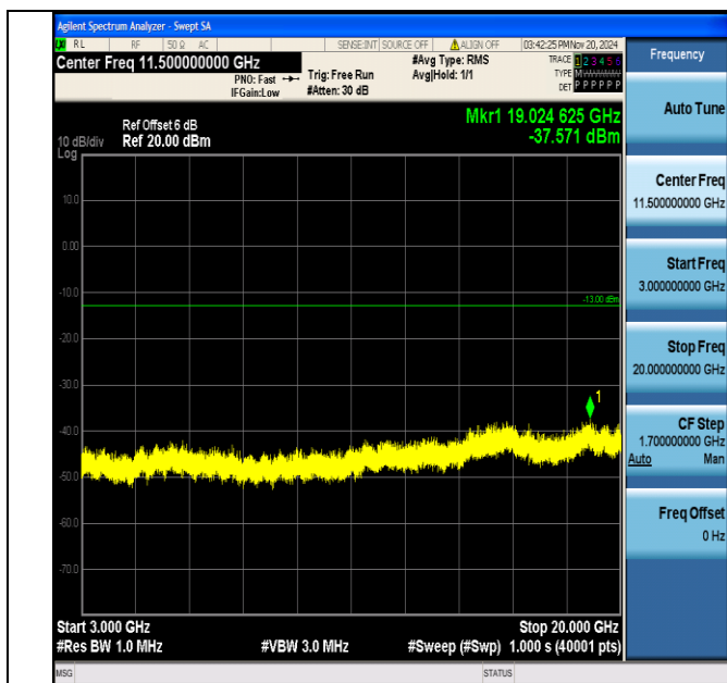
Band2_10MHz_16QAM_18900_1RB#0_3000~20000_3000~20000
