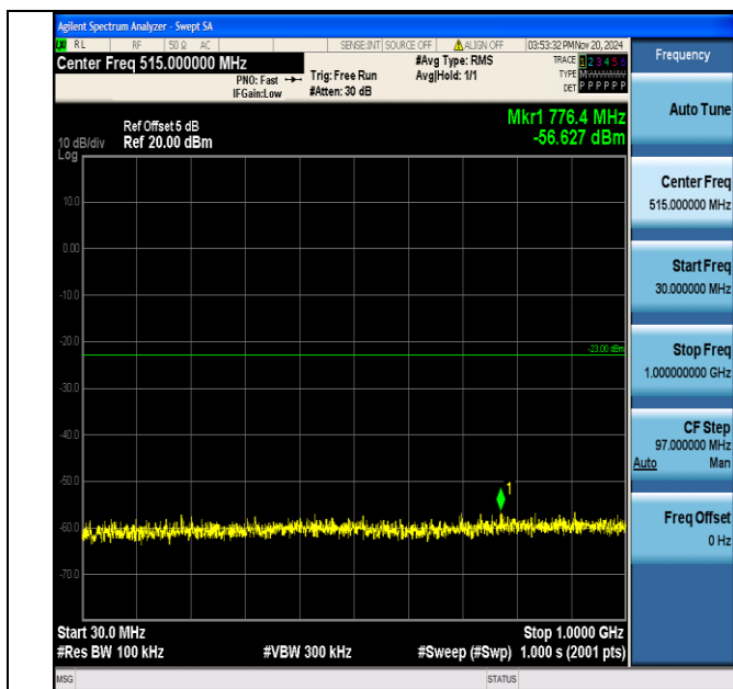
Band2_15MHz_16QAM_19125_1RB#0_30~1000_30~1000
