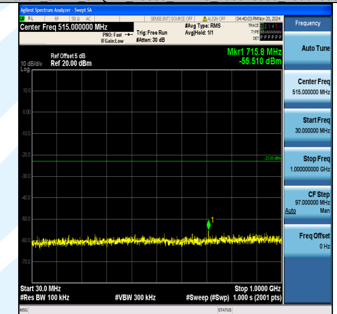
Band4_3MHz_16QAM_19965_1RB#0_30~1000_30~1000
