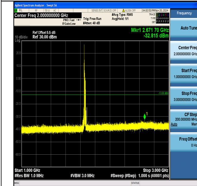
Band2_20MHz_16QAM_18700_1RB#0_1000~3000_1000~3000
