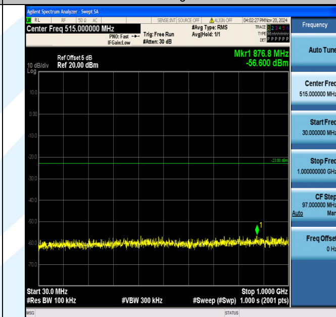
Band2_20MHz_16QAM_19100_1RB#0_30~1000_30~1000
