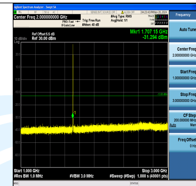
Band4_1.4MHz_16QAM_19957_1RB#0_1000~3000_1000~3000
