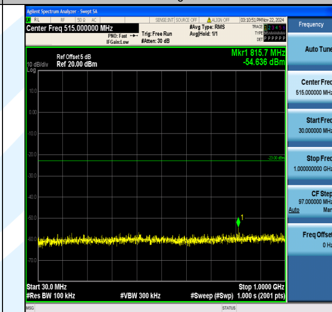
Band2_20MHz_64QAM_18900_1RB#0_30~1000_30~1000
