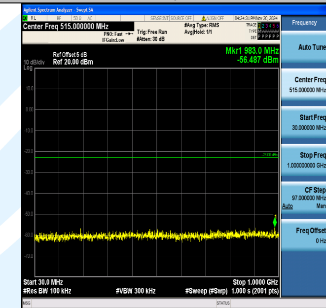
Band4_1.4MHz_16QAM_20175_1RB#0_30~1000_30~1000
