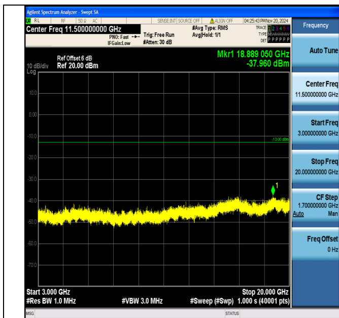
Band4_1.4MHz_16QAM_20393_1RB#0_3000~20000_3000~20000
