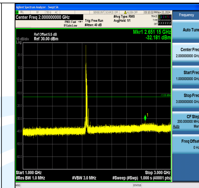
Band2_20MHz_64QAM_18700_1RB#0_1000~3000_1000~3000
