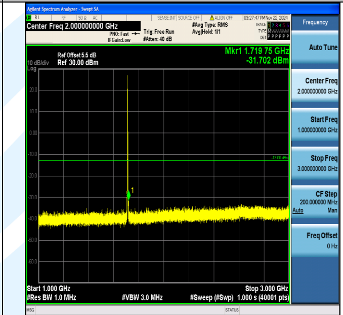
Band4 3MHz 64QAM 19965_1RB#0 1000~3000 1000~3000
