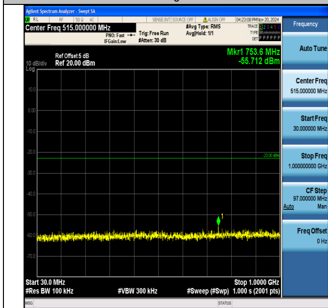
Band4_1.4MHz_QPSK_19957_1RB#0_30~1000_30~1000
