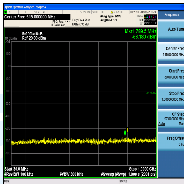
Band4_3MHz_64QAM_20175_1RB#0_30~1000_30~1000
