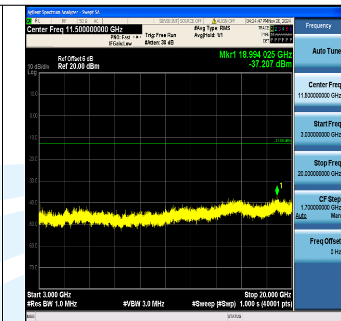
Band4_1.4MHz_16QAM_20175_1RB#0_3000~20000_3000~20000
