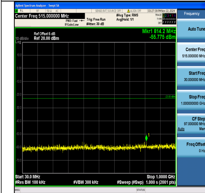
Band4 3MHz 64QAM 19965_1RB#0 30~1000 30~1000
