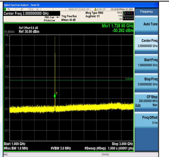
Band4_1.4MHz_64QAM_20175_1RB#0_1000~3000_1000~3000
