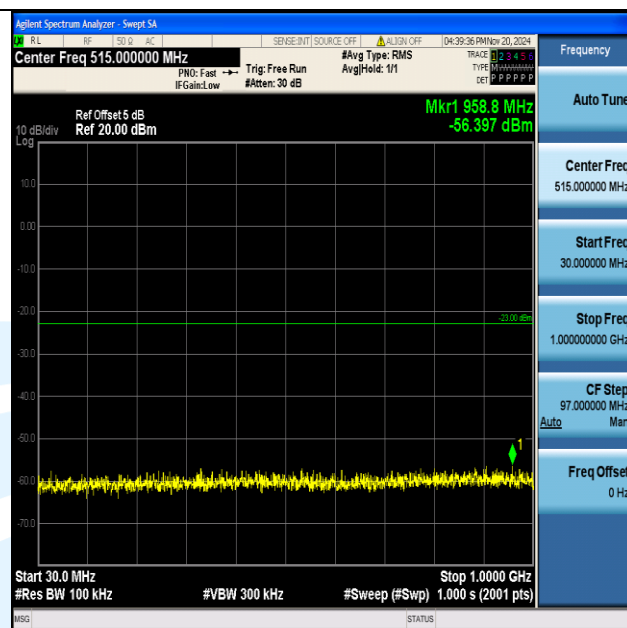
Band4_3MHz_QPSK_19965_1RB#0_30~1000_30~1000
