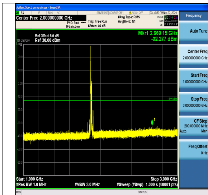
Band2_20MHz_64QAM_18900_1RB#0_1000~3000_1000~3000
