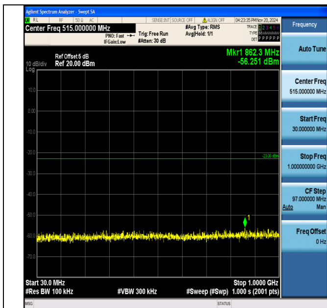
Band4_1.4MHz_16QAM_19957_1RB#0_30~1000_30~1000
