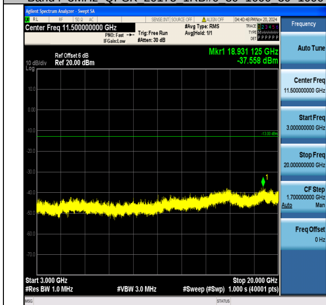
Band4_3MHz_QPSK_20175_1RB#0_3000~20000_3000~2000 0
