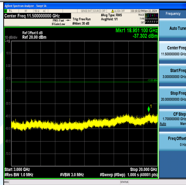
Band4_1.4MHz_64QAM_20393_1RB#0_3000~20000_3000~20000
