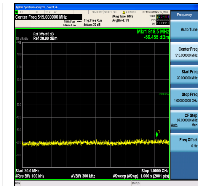
Band2_20MHz_64QAM_18700_1RB#0_30~1000_30~1000
