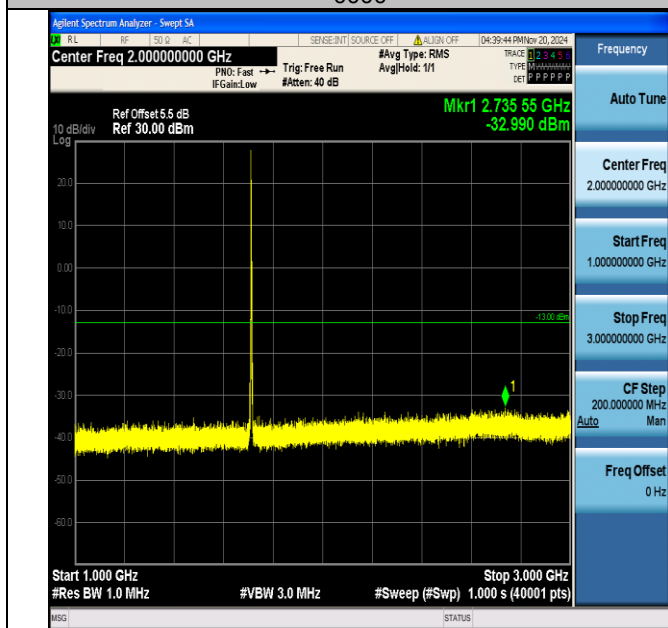
Band4_3MHz_QPSK_19965_1RB#0_1000~3000_1000~3000
