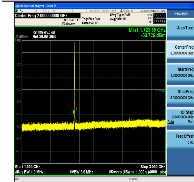
Band4_3MHz_64QAM_20175_1RB#0_1000~3000_1000~3000
