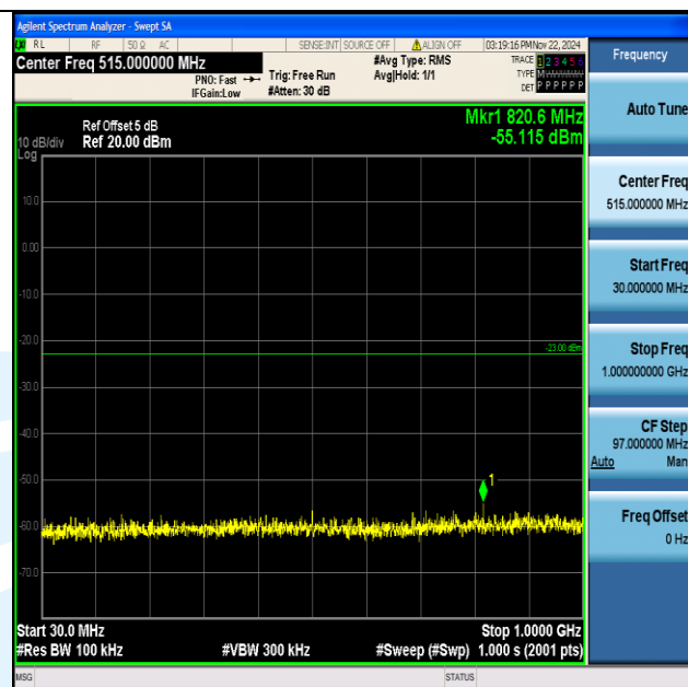
Band4_1.4MHz_64QAM_20393_1RB#0_30~1000_30~1000
