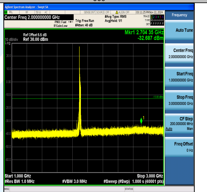
Band2_20MHz_64QAM_19100_1RB#0_1000~3000_1000~3000
