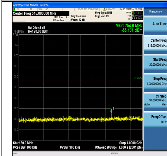
Band4_1.4MHz_16QAM_20393_1RB#0_30~1000_30~1000
