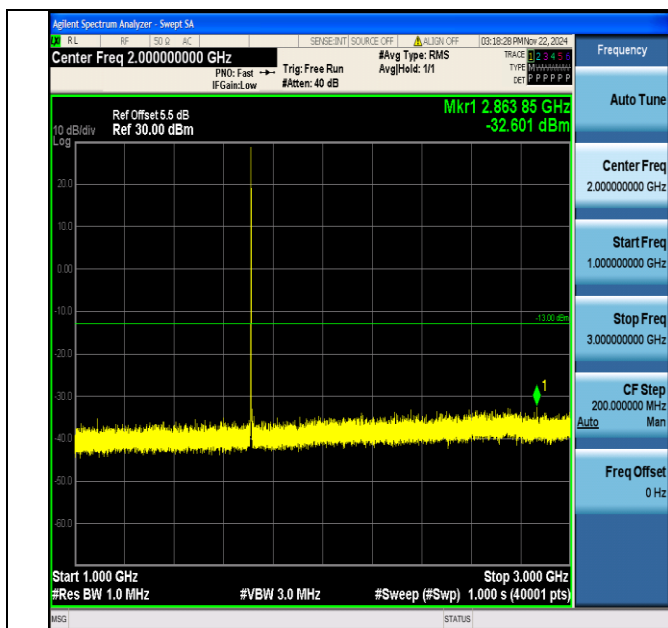
Band4_1.4MHz_64QAM_19957_1RB#0_1000~3000_1000~3000
