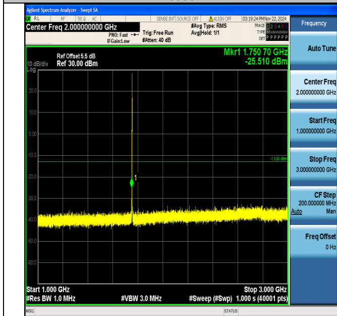
Band4_1.4MHz_64QAM_20393_1RB#0_1000~3000_1000~3000
