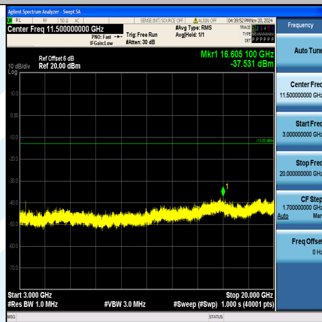
Band4_3MHz_QPSK_19965_1RB#0_3000~20000_3000~20000
