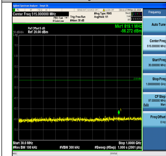
Band2_20MHz_64QAM_19100_1RB#0_30~1000_30~1000
