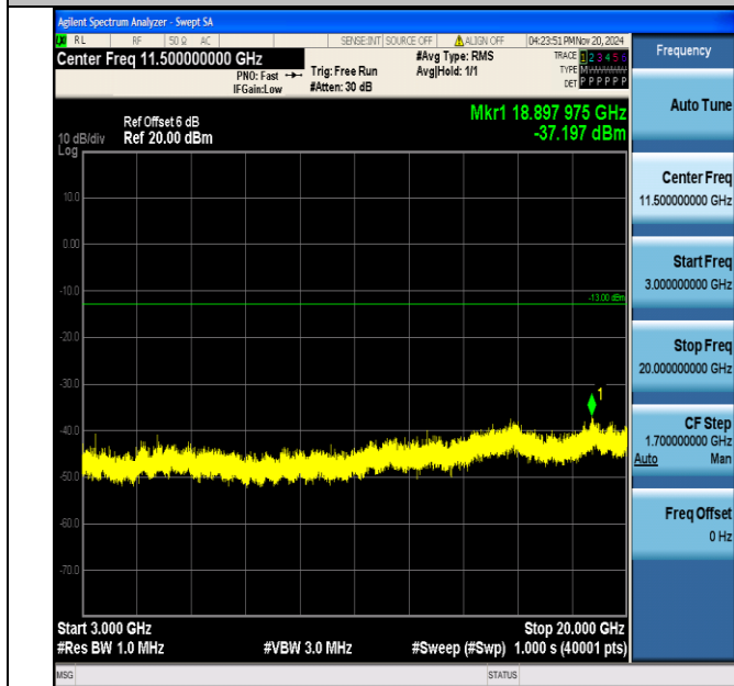
Band4_1.4MHz_16QAM_19957_1RB#0_3000~20000_3000~20000
