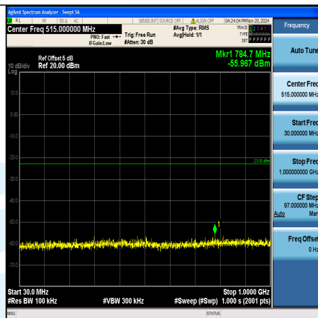
Band4_1.4MHz_QPSK_20175_1RB#0_30~1000_30~1000
