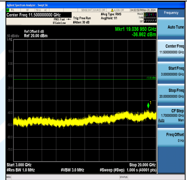
Band2_20MHz_16QAM_18700_1RB#0_3000~20000_3000~20000
