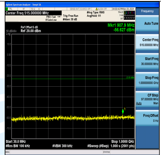
Band2_20MHz_16QAM_18700_1RB#0_30~1000_30~1000
