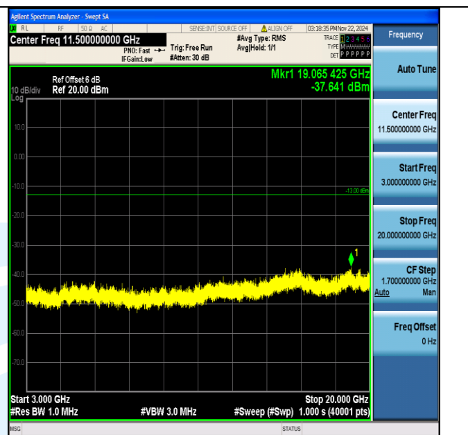
Band4_1.4MHz_64QAM_19957_1RB#0_3000~20000_3000~20000
