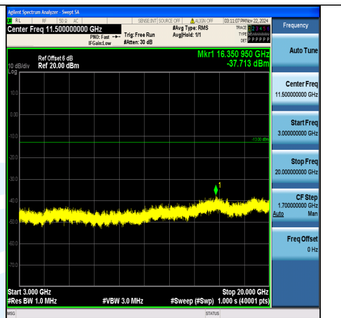
Band2_20MHz_64QAM_18900_1RB#0_3000~20000_3000~20000
