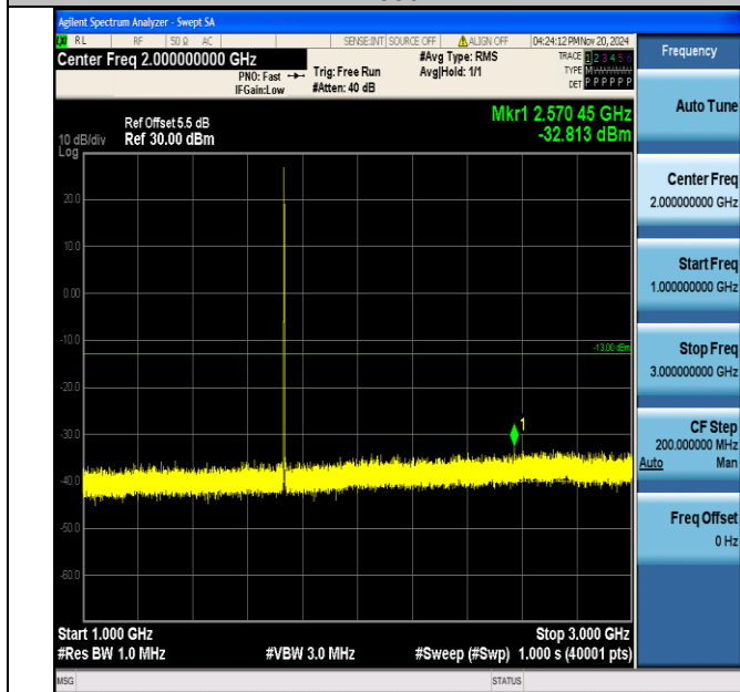
Band4_1.4MHz_QPSK_20175_1RB#0_1000~3000_1000~3000
