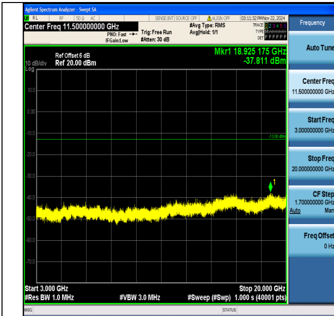
Band2_20MHz_64QAM_19100_1RB#0_3000~20000_3000~20000
