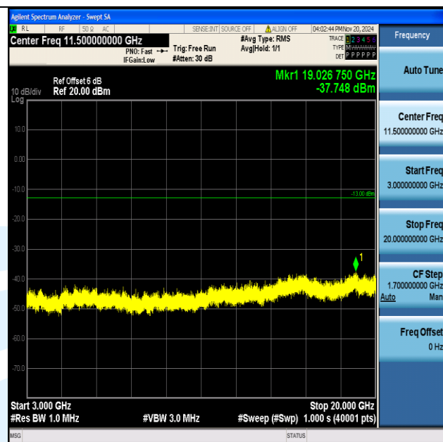
Band2_20MHz_16QAM_19100_1RB#0_3000~20000_3000~20000
