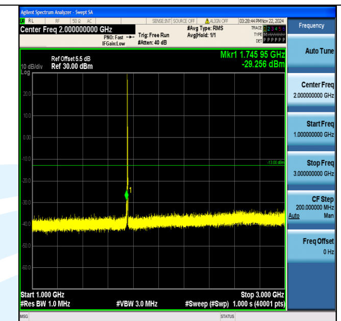
Band4 3MHz 64QAM 20385 1RB#0 1000~3000 1000~3000
