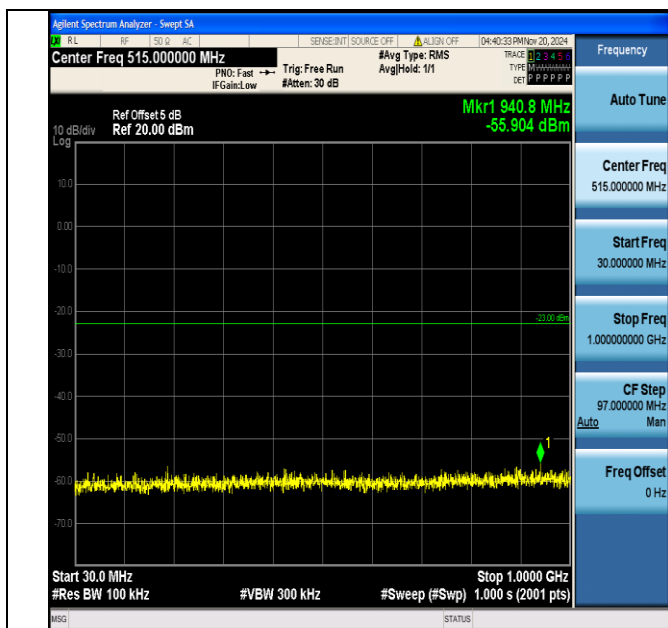
Band4 3MHz QPSK 20175 1RB#0 30~1000 30~1000
