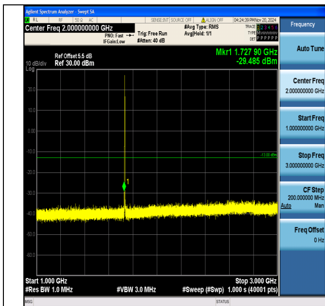
Band4_1.4MHz_16QAM_20175_1RB#0_1000~3000_1000~3000
