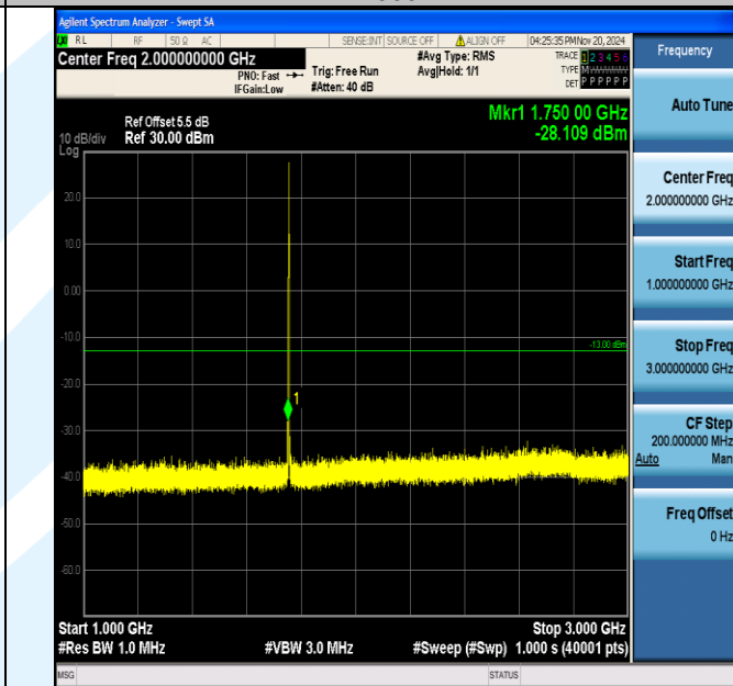
Band4_1.4MHz_16QAM_20393_1RB#0_1000~3000_1000~3000
