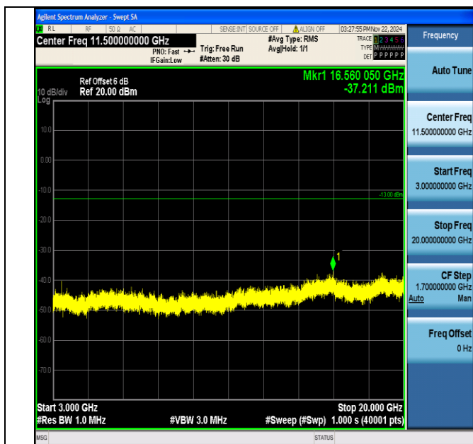
Band4_3MHz_64QAM_19965_1RB#0_3000~20000_3000~20000
