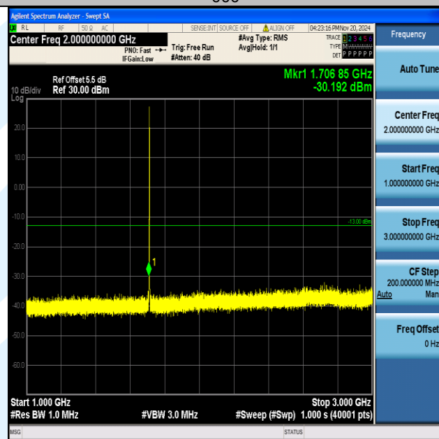
Band4_1.4MHz_QPSK_19957_1RB#0_1000~3000_1000~3000
