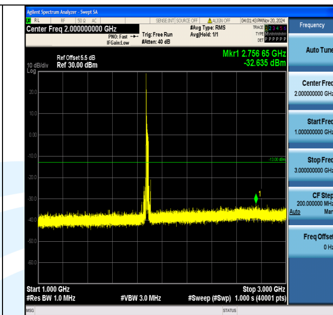
Band2_20MHz_16QAM_18900_1RB#0_1000~3000_1000~3000
