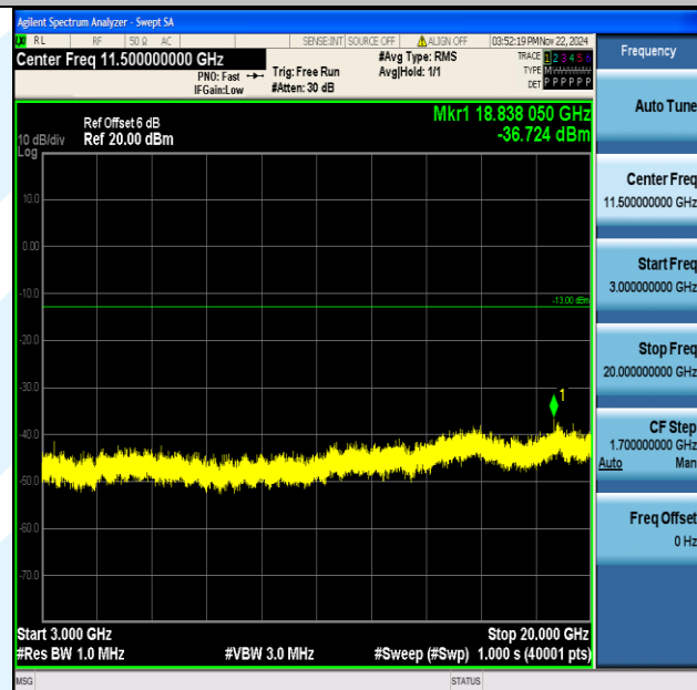
Band4_20MHz_64QAM_20175_1RB#0_3000~20000_3000~20000
