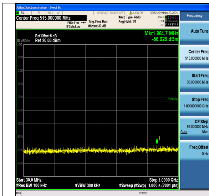
Band4_20MHz_64QAM_20300_1RB#0_30~1000_30~1000
