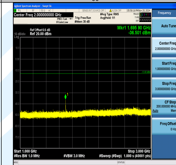
Band5_1.4MHz_QPSK_20643_1RB#0_1000~3000_1000~3000
