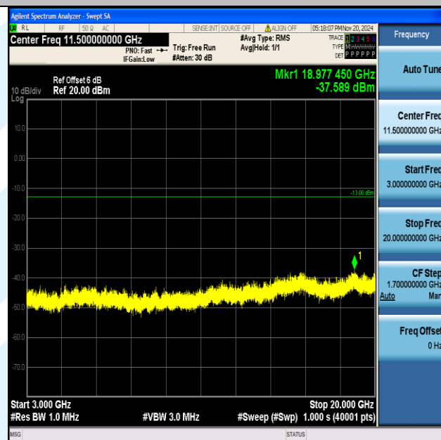
Band4_15MHz_QPSK_20175_1RB#0_3000~20000_3000~20000
