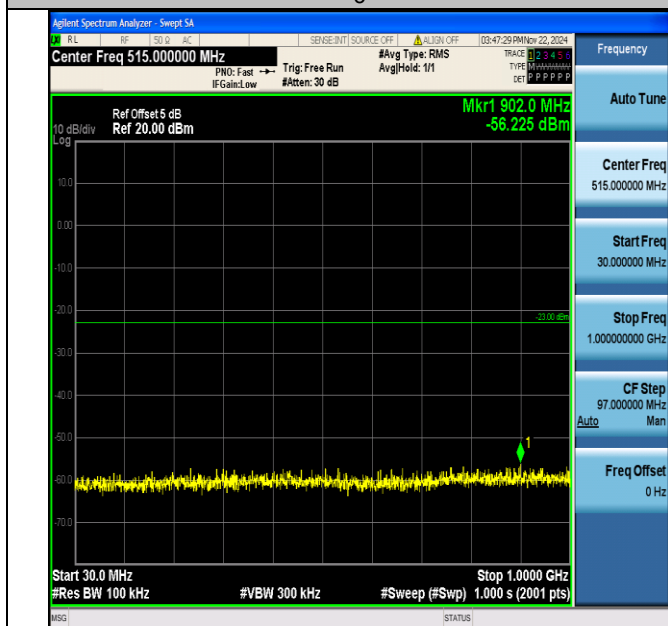
Band4_15MHz_64QAM_20175_1RB#0_30~1000_30~1000
