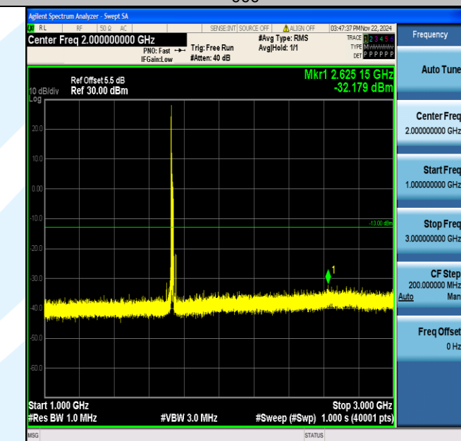
Band4_15MHz_64QAM_20175_1RB#0_1000~3000_1000~3000
