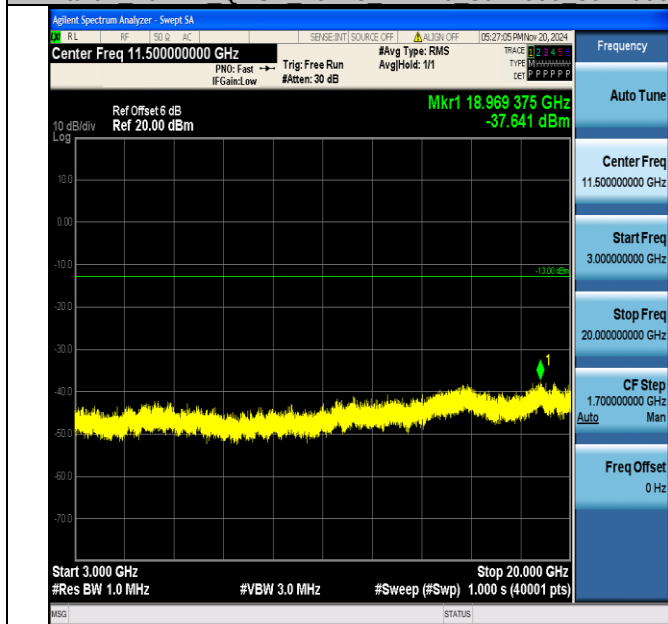
Band4_20MHz_QPSK_20175_1RB#0_3000~20000_3000~20000
