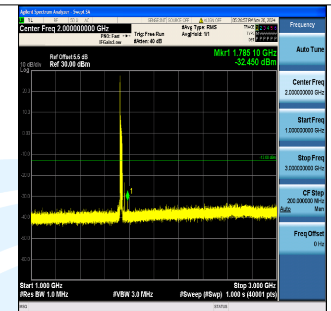
Band4_20MHz_QPSK_20175_1RB#0_1000~3000_1000~3000
