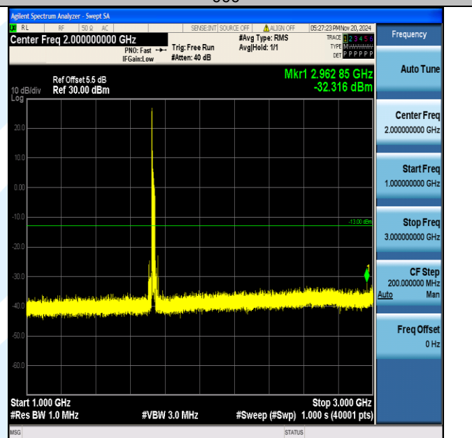
Band4_20MHz_16QAM_20175_1RB#0_1000~3000_1000~3000
