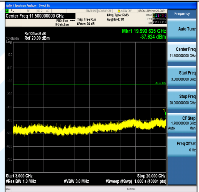
Band4_20MHz_QPSK_20050_1RB#0_3000~20000_3000~20000
