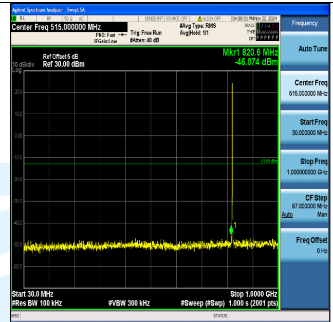
Band5_1.4MHz_64QAM_20407_1RB#0_30~1000_30~1000
