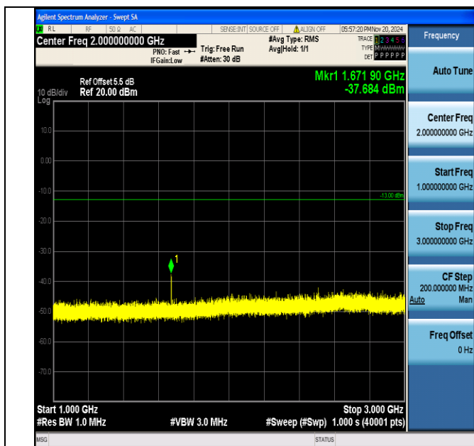
Band5_1.4MHz_QPSK_20525_1RB#0_1000~3000_1000~3000
