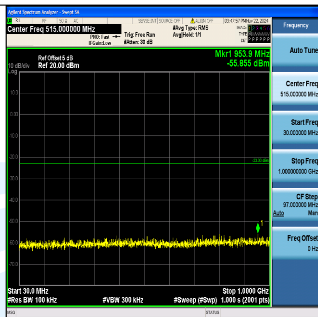
Band4_15MHz_64QAM_20325_1RB#0_30~1000_30~1000
