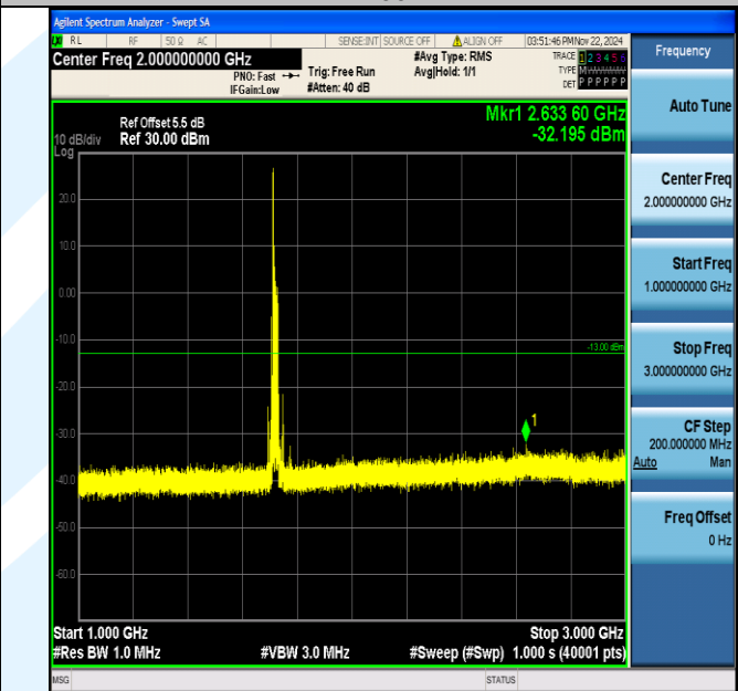
Band4_20MHz_64QAM_20050_1RB#0_1000~3000_1000~3000
