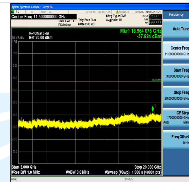
Band4_15MHz_64QAM_20025_1RB#0_3000~20000_3000~20000
