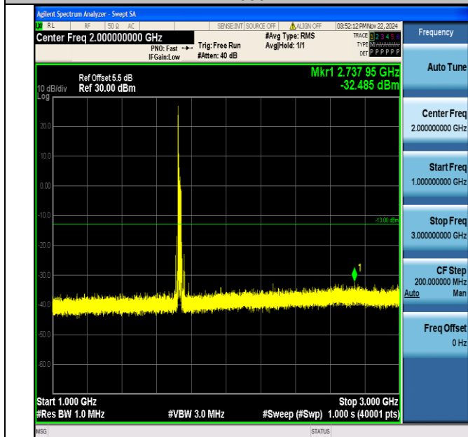
Band4_20MHz_64QAM_20175_1RB#0_1000~3000_1000~3000
