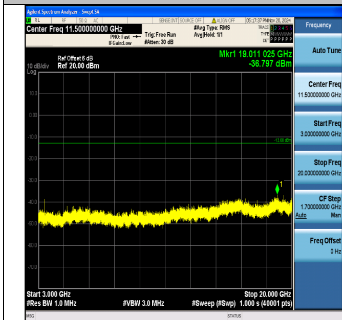
Band4_15MHz_16QAM_20025_1RB#0_3000~20000_3000~20000
