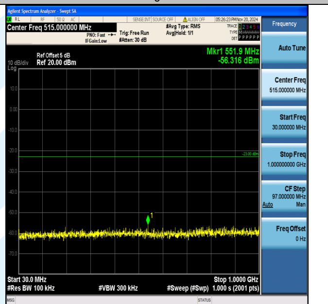
Band4_20MHz_16QAM_20050_1RB#0_30~1000_30~1000
