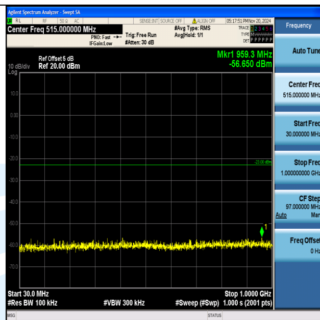
Band4_15MHz_QPSK_20175_1RB#0_30~1000_30~1000
