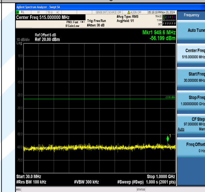
Band4_15MHz_16QAM_20175_1RB#0_30~1000_30~1000
