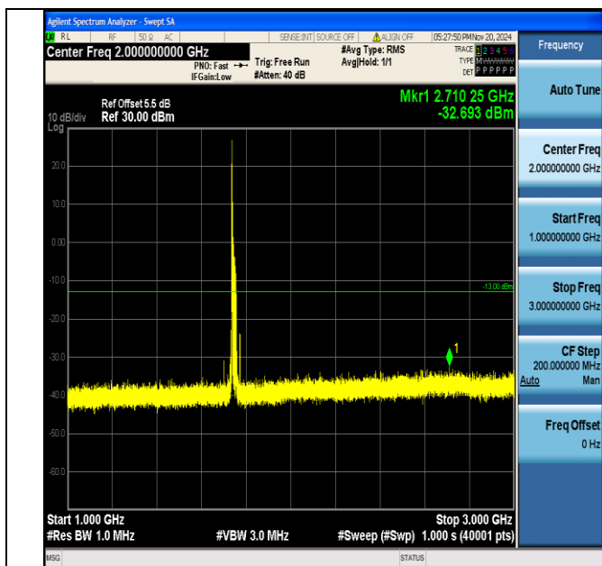
Band4_20MHz_QPSK_20300_1RB#0_1000~3000_1000~3000
