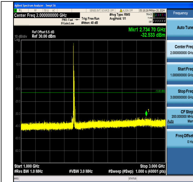
Band4_15MHz_16QAM_20175_1RB#0_1000~3000_1000~3000
