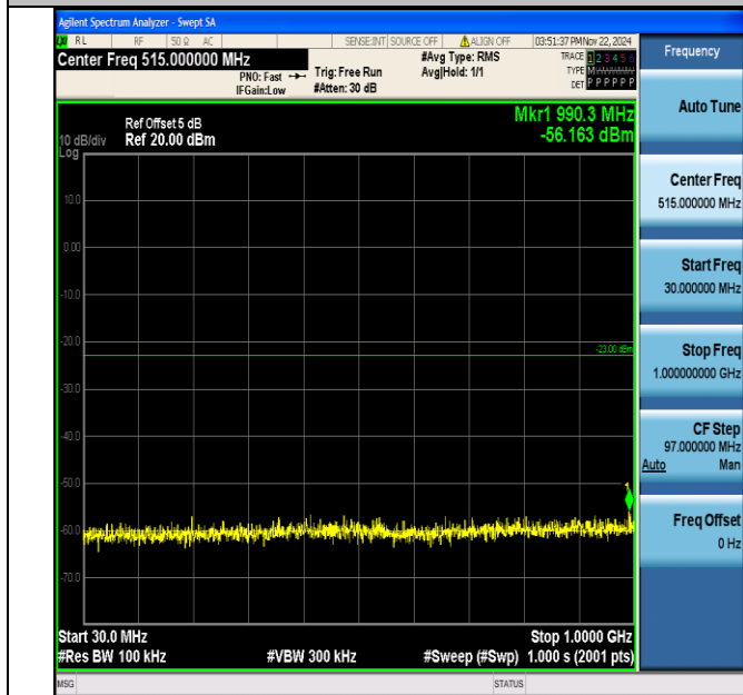
Band4_20MHz_64QAM_20050_1RB#0_30~1000_30~1000
