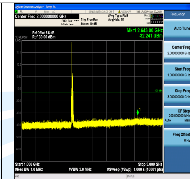
Band4_15MHz_16QAM_20025_1RB#0_1000~3000_1000~3000
