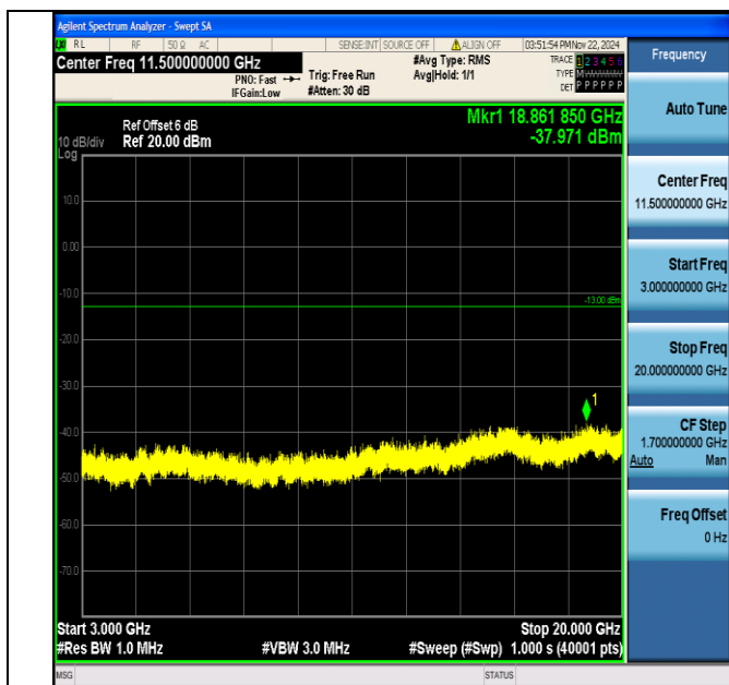
Band4_20MHz_64QAM_20050_1RB#0_3000~20000_3000~20000
