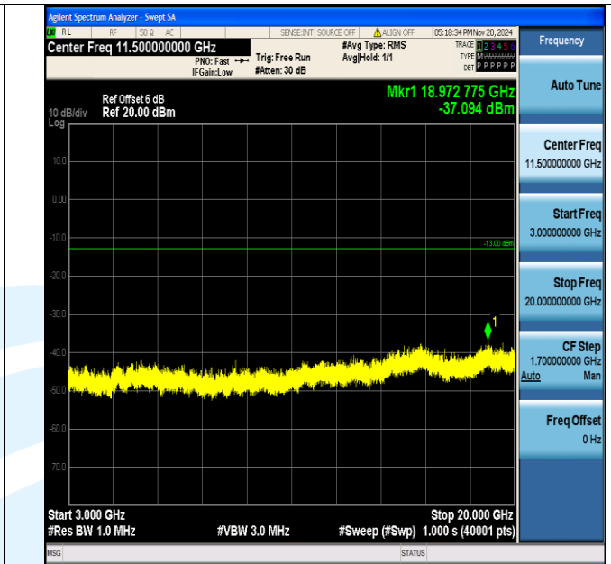
Band4_15MHz_16QAM_20175_1RB#0_3000~20000_3000~20000
