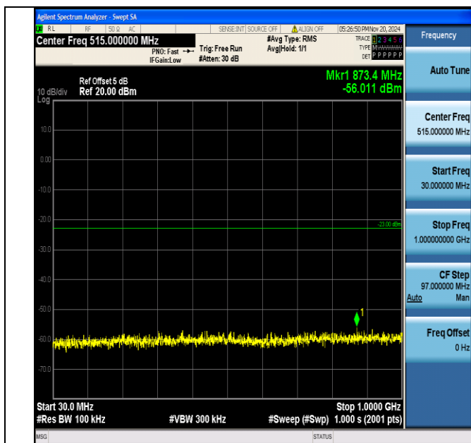
Band4_20MHz_QPSK_20175_1RB#0_30~1000_30~1000
