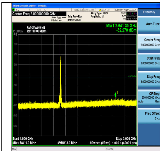
Band4_15MHz_64QAM_20025_1RB#0_1000~3000_1000~3000
