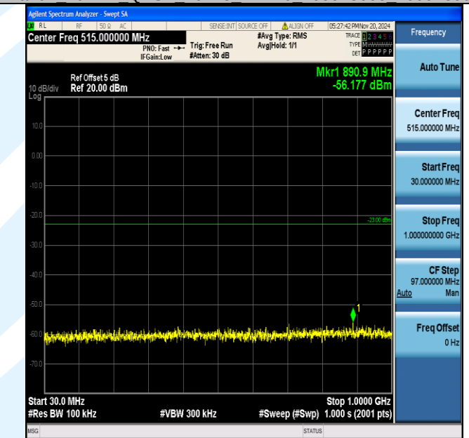
Band4_20MHz_QPSK_20300_1RB#0_30~1000_30~1000
