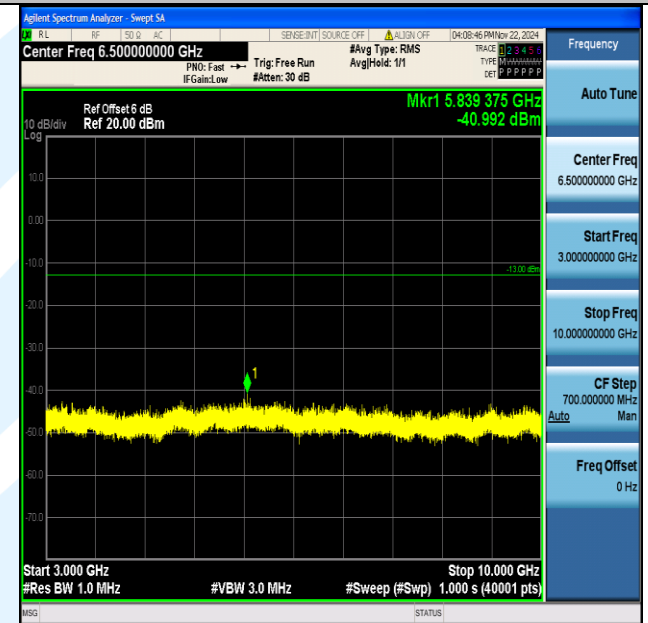
Band5_1.4MHz_64QAM_20407_1RB#0_3000~10000_3000~10000
