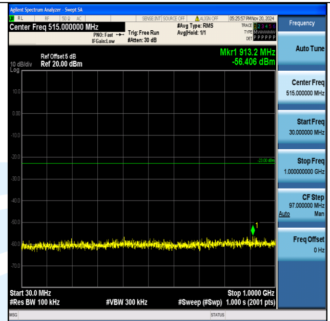
Band4_20MHz_QPSK_20050_1RB#0_30~1000_30~1000
