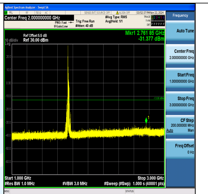
Band4_20MHz_64QAM_20300_1RB#0_1000~3000_1000~3000
