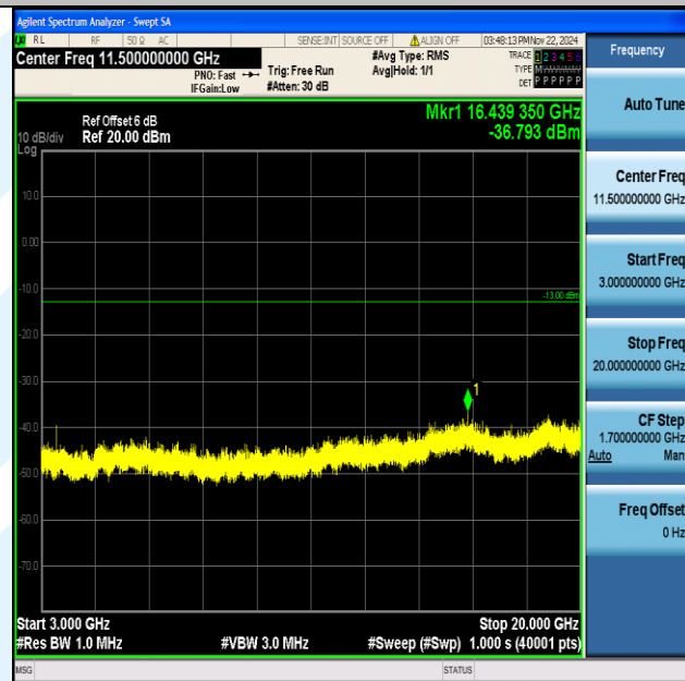
Band4_15MHz_64QAM_20325_1RB#0_3000~20000_3000~20000
