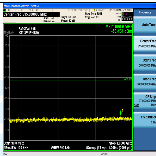
Band4_20MHz_64QAM_20175_1RB#0_30~1000_30~1000
