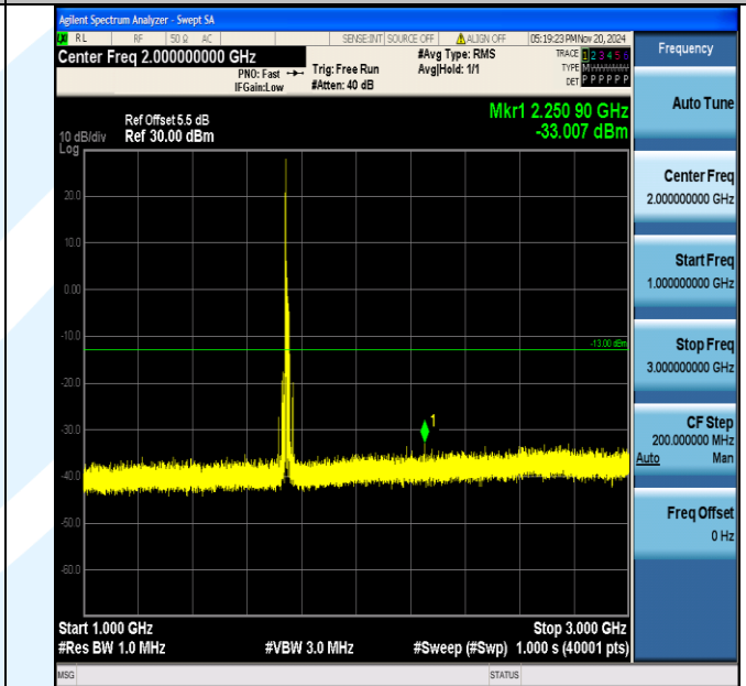
Band4_15MHz_16QAM_20325_1RB#0_1000~3000_1000~3000
