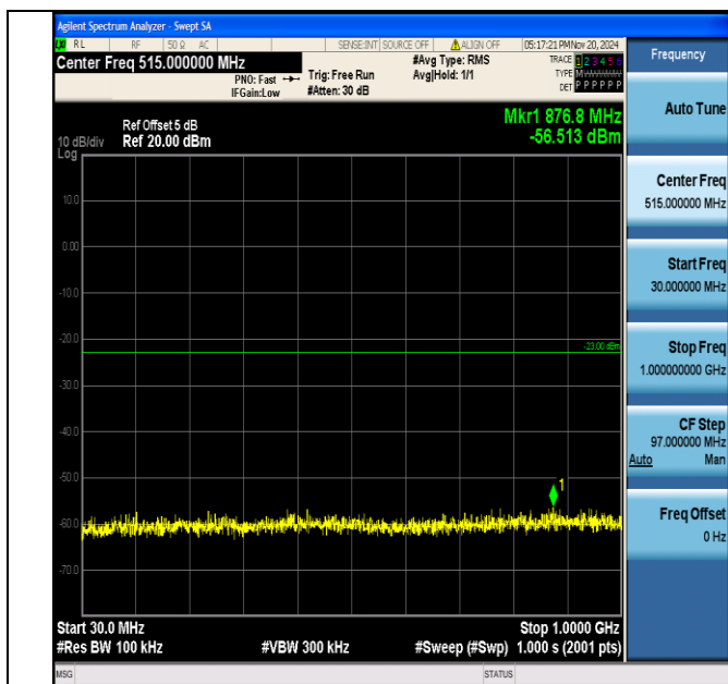
Band4_15MHz_16QAM_20025_1RB#0_30~1000_30~1000
