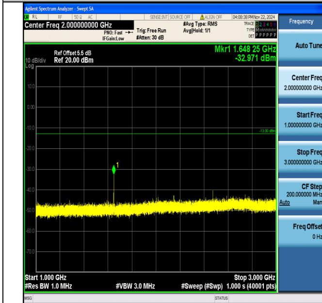
Band5_1.4MHz_64QAM_20407_1RB#0_1000~3000_1000~3000
