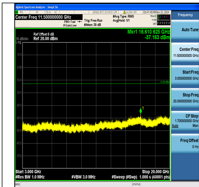
Band4_15MHz_64QAM_20175_1RB#0_3000~20000_3000~20000
