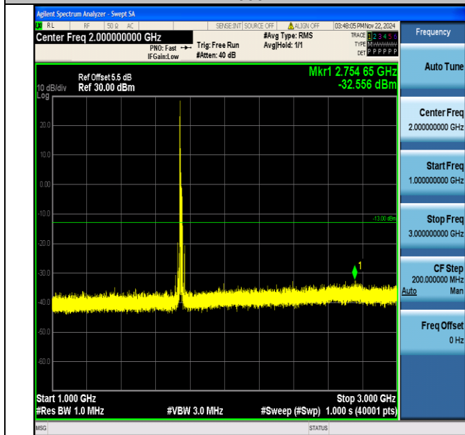
Band4_15MHz_64QAM_20325_1RB#0_1000~3000_1000~3000
