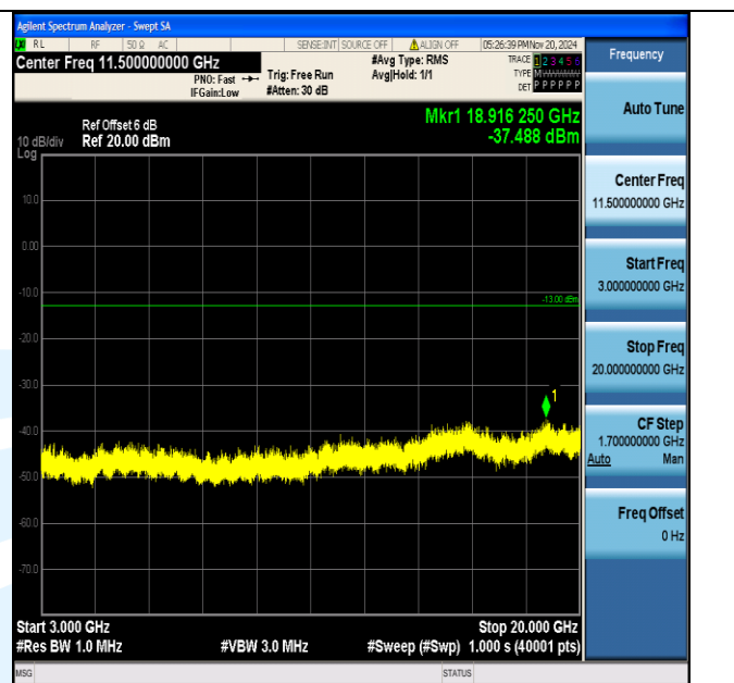
Band4_20MHz_16QAM_20050_1RB#0_3000~20000_3000~20000
