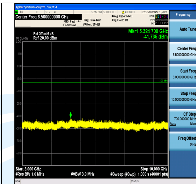
Band5_1.4MHz_QPSK_20525_1RB#0_3000~10000_3000~10000
