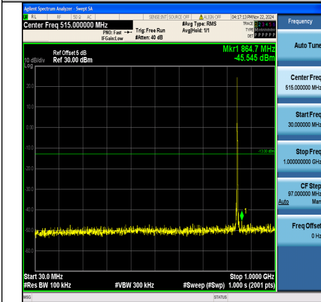
Band5 3MHz 64QAM 20635 1RB#0 30~1000 30~1000
