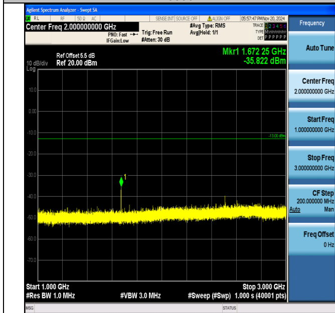
Band5_1.4MHz_16QAM_20525_1RB#0_1000~3000_1000~3000
