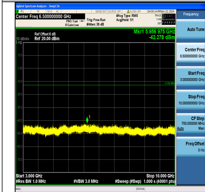
Band5_1.4MHz_64QAM_20525_1RB#0_3000~10000_3000~10000 0000
