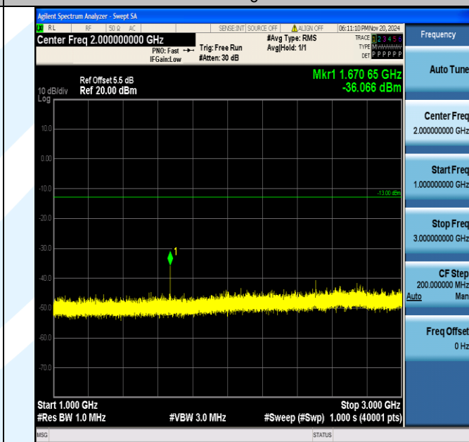
Band5_3MHz_QPSK_20525_1RB#0_1000~3000_1000~3000
