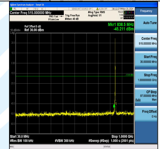
Band5_3MHz_16QAM_20635_1RB#0_30~1000_30~1000
