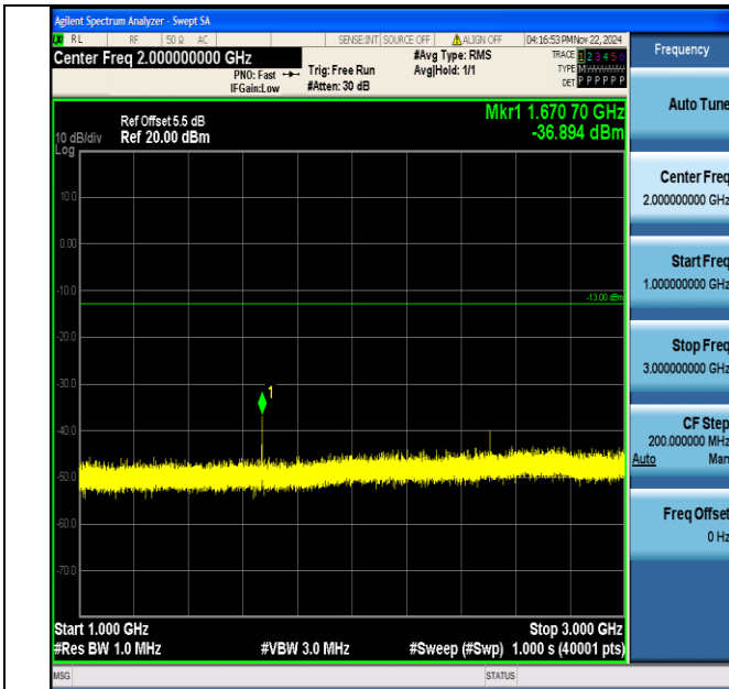
Band5_3MHz_64QAM_20525_1RB#0_1000~3000_1000~3000
