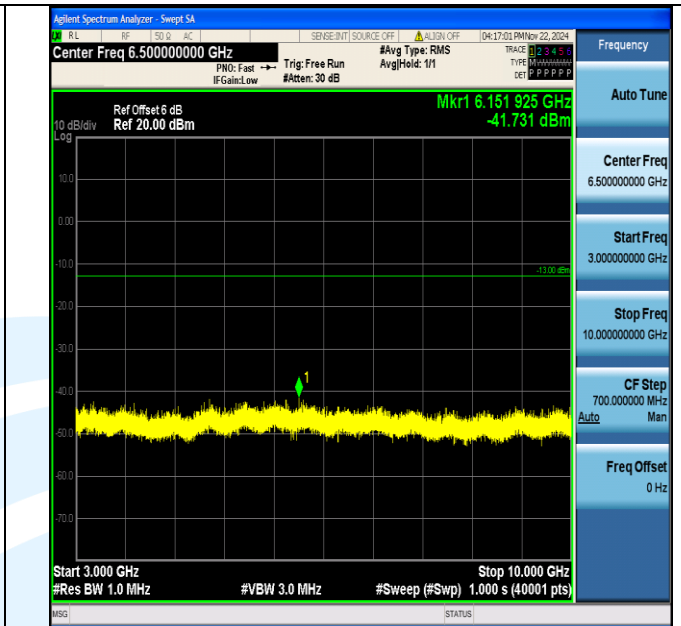
Band5_3MHz_64QAM_20525_1RB#0_3000~10000_3000~10000
