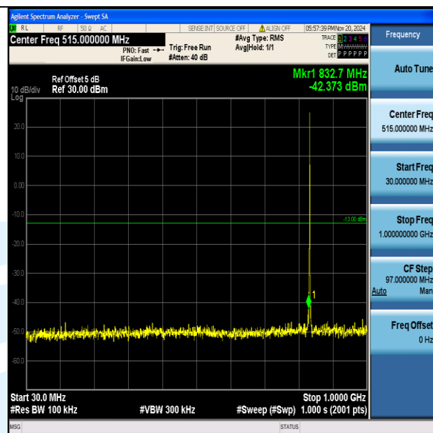
Band5_1.4MHz_16QAM_20525_1RB#0_30~1000_30~1000
