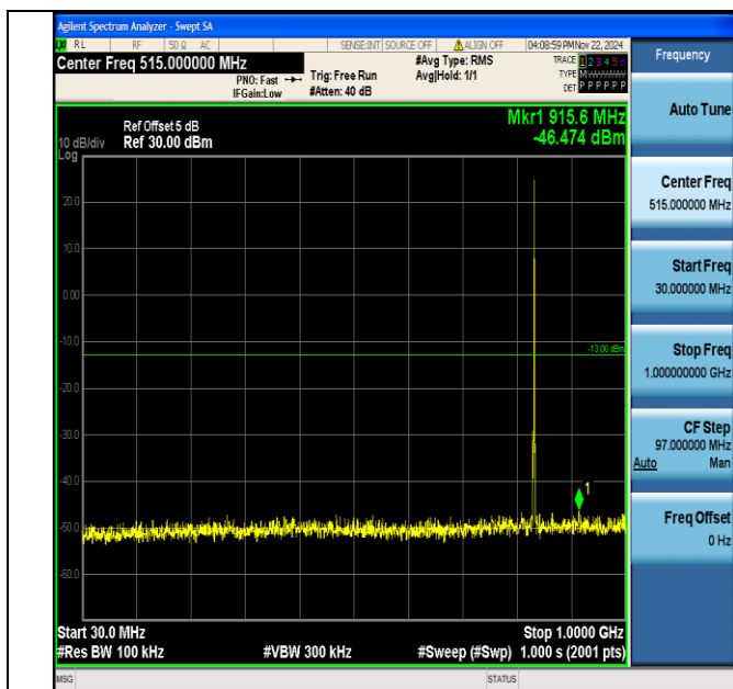
Band5_1.4MHz_64QAM_20525_1RB#0_30~1000_30~1000
