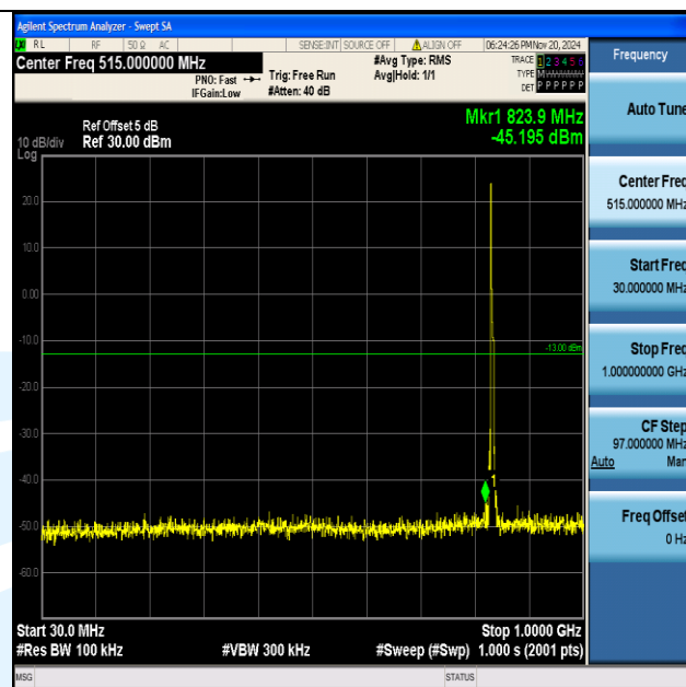
Band5_5MHz_QPSK_20525_1RB#0_30~1000_30~1000
