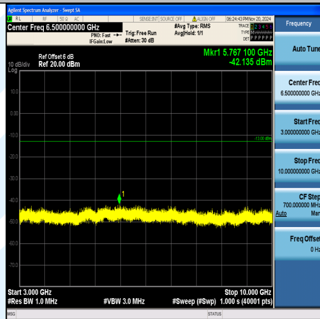
Band5_5MHz_QPSK_20525_1RB#0_3000~10000_3000~1000 0
