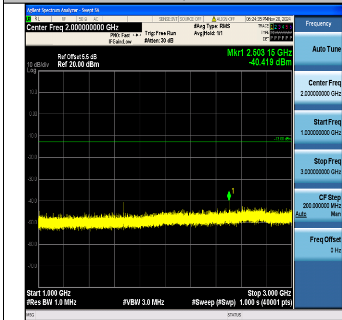
Band5_5MHz_QPSK_20525_1RB#0_1000~3000_1000~3000
