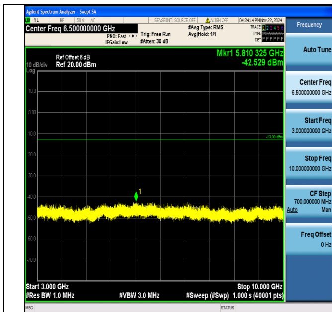
Band5_5MHz_64QAM_20525_1RB#0_3000~10000_3000~10000
