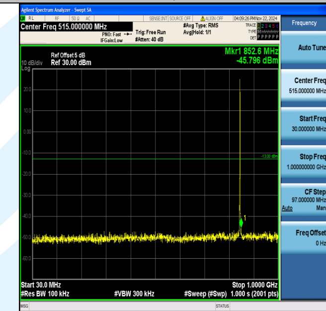
Band5_1.4MHz_64QAM_20643_1RB#0_30~1000_30~1000
