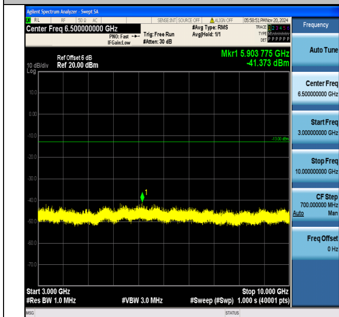
Band5_1.4MHz_16QAM_20643_1RB#0_3000~10000_3000~10000
