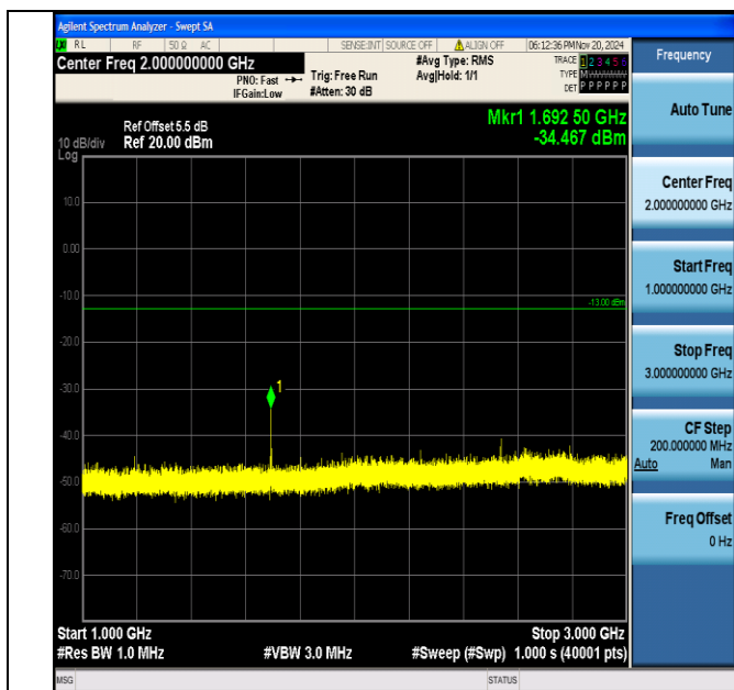
Band5_3MHz_16QAM_20635_1RB#0_1000~3000_1000~3000
