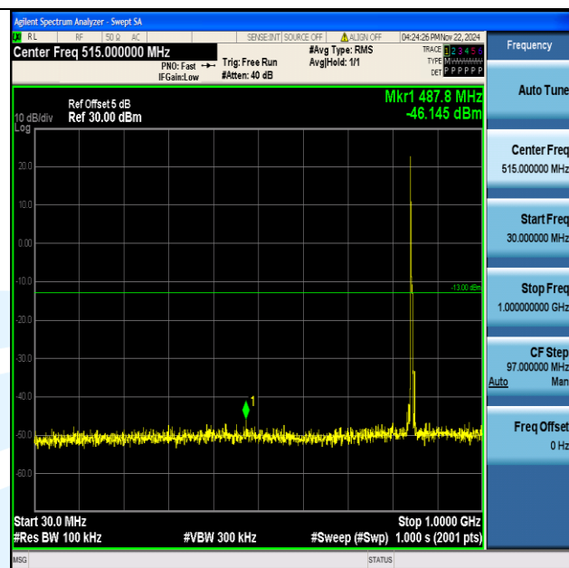
Band5_5MHz_64QAM_20625_1RB#0_30~1000_30~1000
