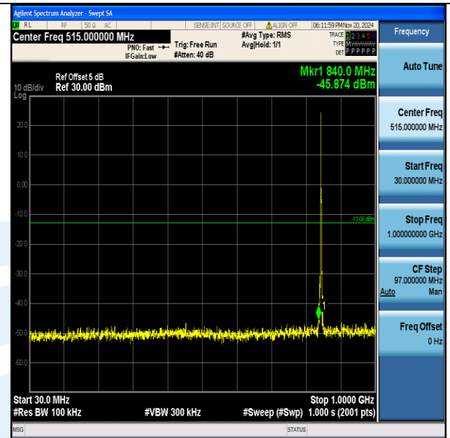
Band5_3MHz_QPSK_20635_1RB#0_30~1000_30~1000
