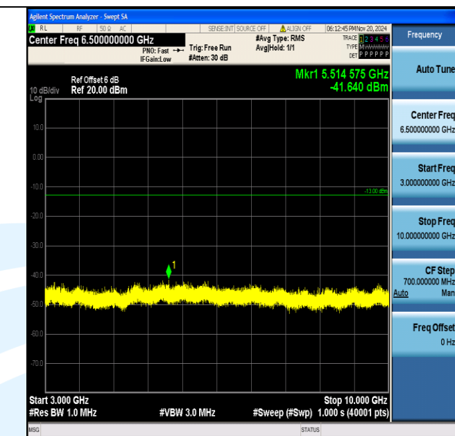
Band5_3MHz_16QAM_20635_1RB#0_3000~10000_3000~10000
