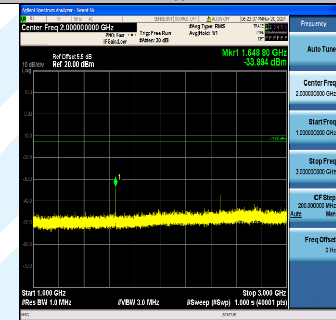
Band5_5MHz_QPSK_20425_1RB#0_1000~3000_1000~3000
