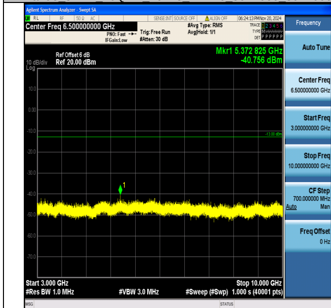
Band5_5MHz_16QAM_20425_1RB#0_3000~10000_3000~10000
