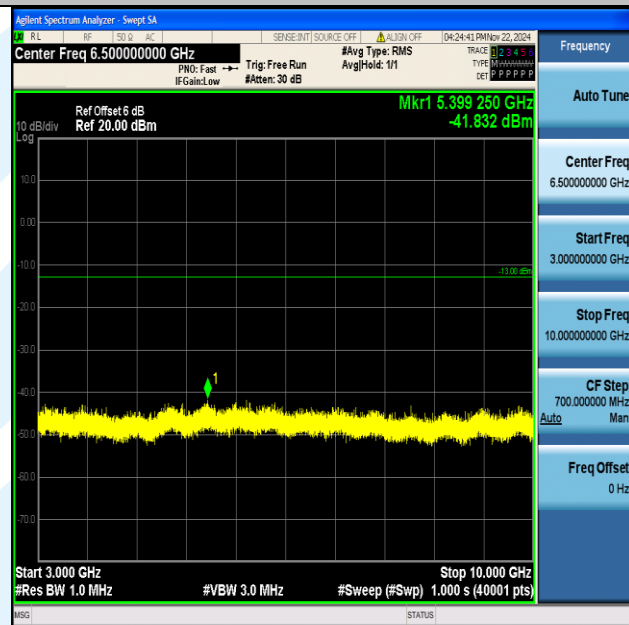
Band5_5MHz_64QAM_20625_1RB#0_3000~10000_3000~10000
