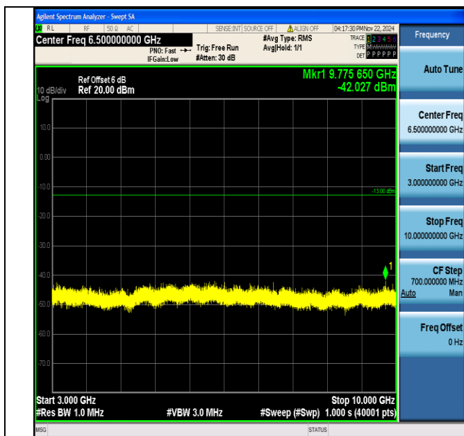
Band5_3MHz_64QAM_20635_1RB#0_3000~10000_3000~10000
