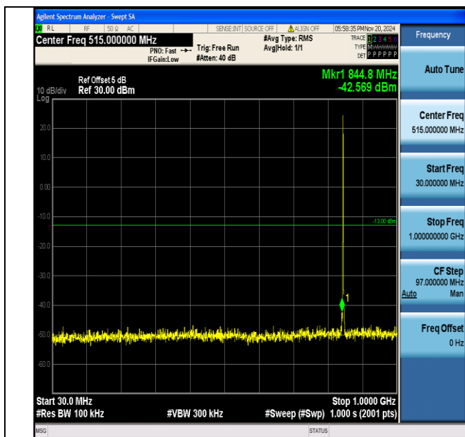
Band5_1.4MHz_16QAM_20643_1RB#0_30~1000_30~1000
