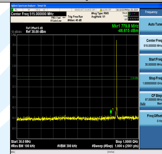
Band5_3MHz_QPSK_20415_1RB#0_30~1000_30~1000
