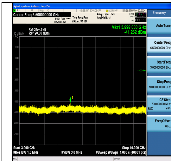
Band5_1.4MHz_16QAM_20407_1RB#0_3000~10000_3000~10000
