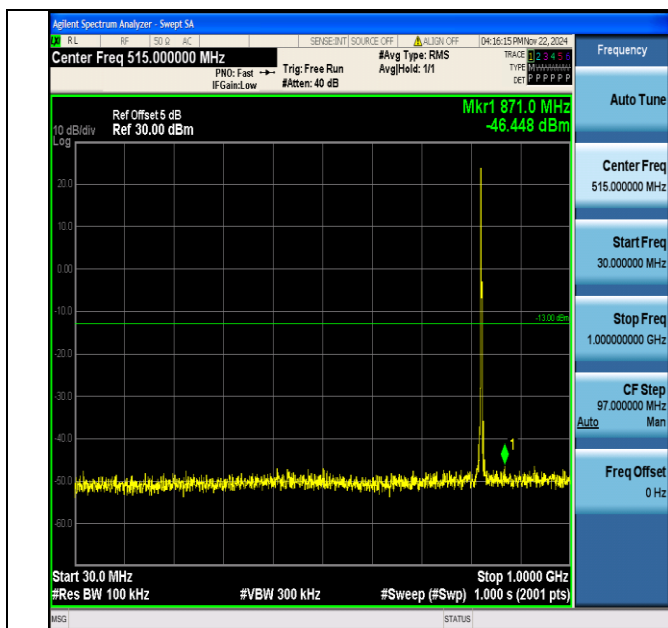
Band5 3MHz 64QAM 20415 1RB#0 30~1000 30~1000
