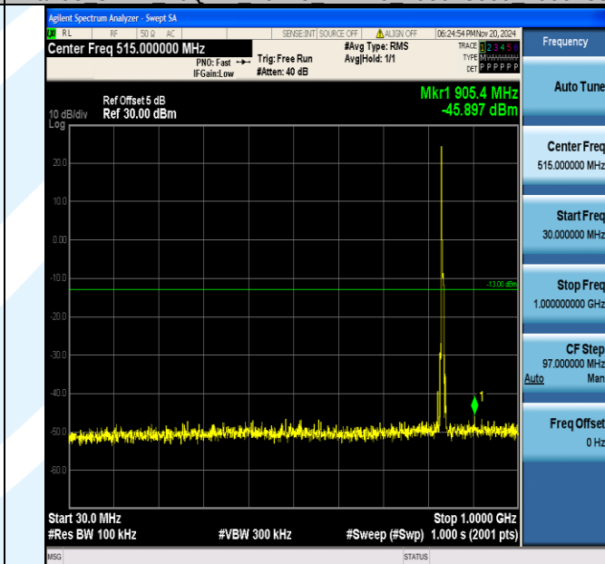
Band5_5MHz_16QAM_20525_1RB#0_30~1000_30~1000
