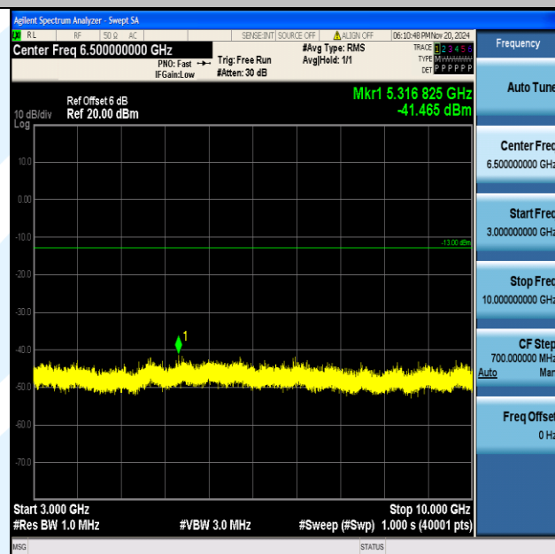
Band5_3MHz_16QAM_20415_1RB#0_3000~10000_3000~10000
