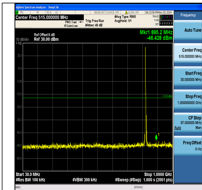
Band5 5MHz 16QAM 20425 1RB#0 30~1000 30~1000
