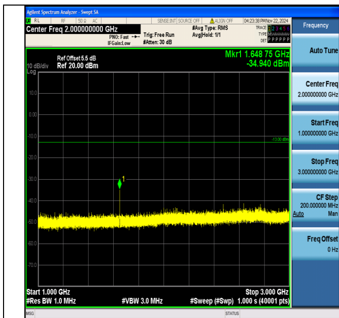
Band5_5MHz_64QAM_20425_1RB#0_1000~3000_1000~3000
