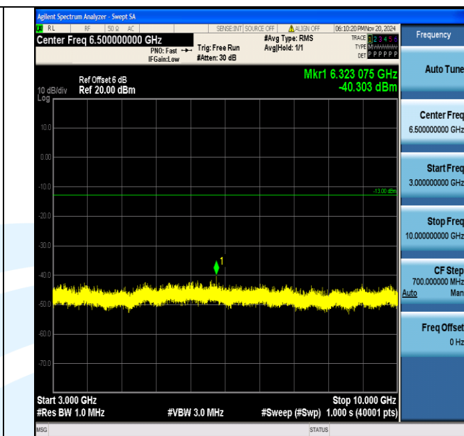
Band5_3MHz_QPSK_20415_1RB#0_3000~10000_3000~10000
