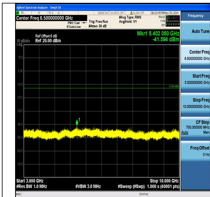
Band5_5MHz_QPSK_20425_1RB#0_3000~10000_3000~1000 0
