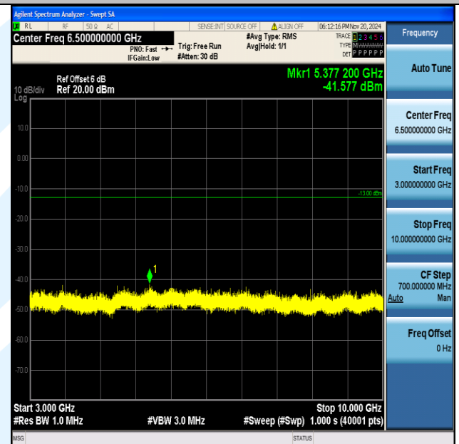
Band5_3MHz_QPSK_20635_1RB#0_3000~10000_3000~1000 0
