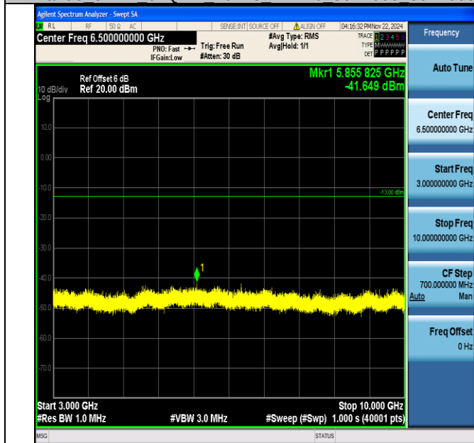
Band5_3MHz_64QAM_20415_1RB#0_3000~10000_3000~10000
