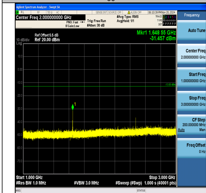
Band5_3MHz_16QAM_20415_1RB#0_1000~3000_1000~3000
