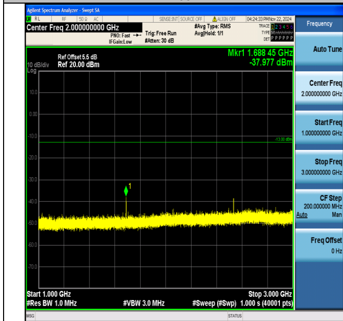
Band5_5MHz_64QAM_20625_1RB#0_1000~3000_1000~3000
