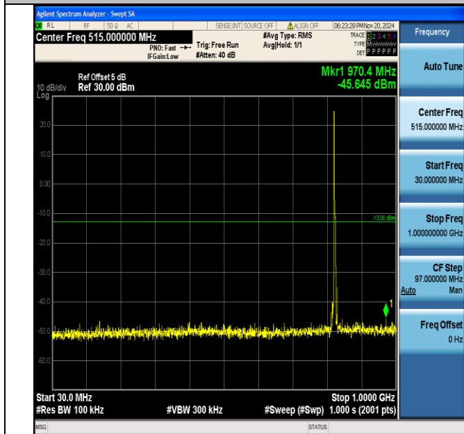
Band5_5MHz_QPSK_20425_1RB#0_30~1000_30~1000
