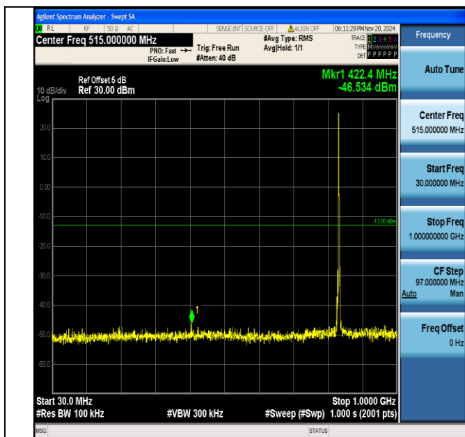
Band5 3MHz 16QAM 20525 1RB#0 30~1000 30~1000
