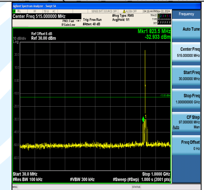
Band5_3MHz_64QAM_20525_1RB#0_30~1000_30~1000
