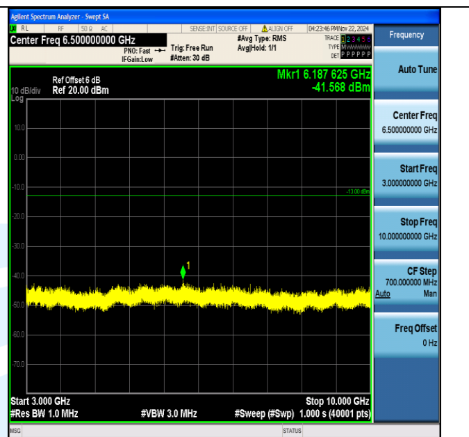
Band5_5MHz_64QAM_20425_1RB#0_3000~10000_3000~10000
