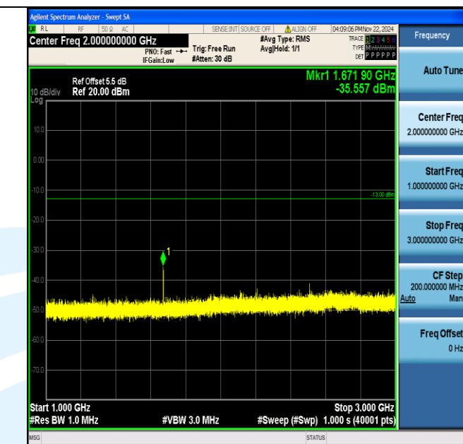
Band5_1.4MHz_64QAM_20525_1RB#0_1000~3000_1000~3000 0
