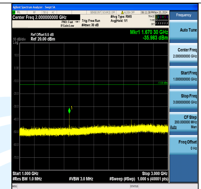
Band5 3MHz 16QAM 20525 1RB#0 1000~3000 1000~3000
