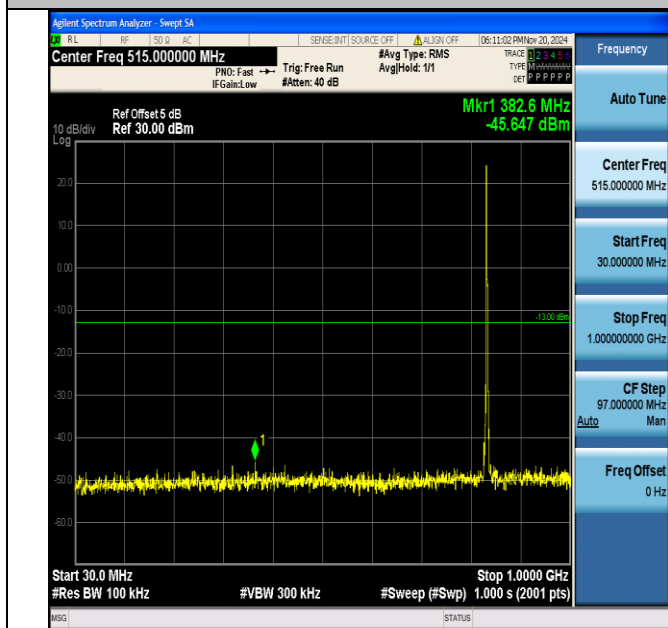
Band5_3MHz_QPSK_20525_1RB#0_30~1000_30~1000
