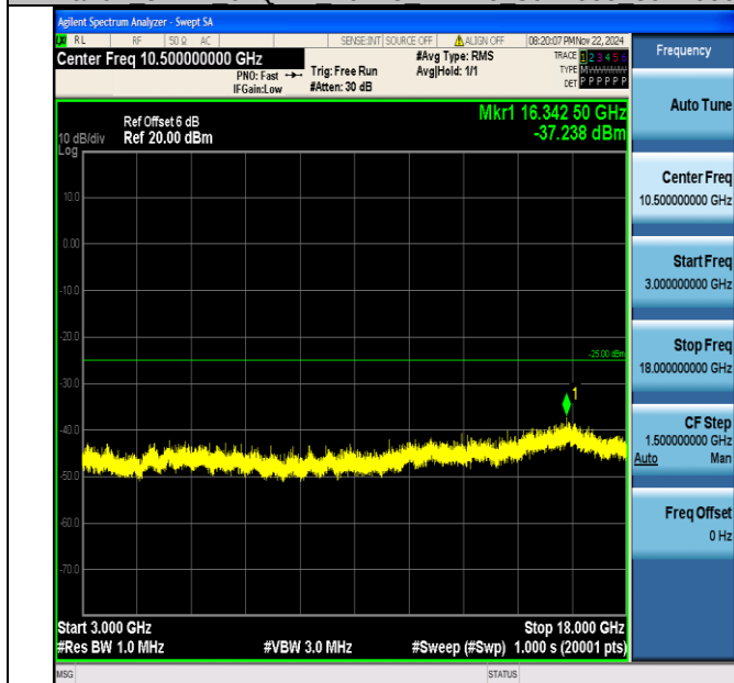
Band7_5MHz_64QAM_20775_1RB#0_3000~18000_3000~18000
