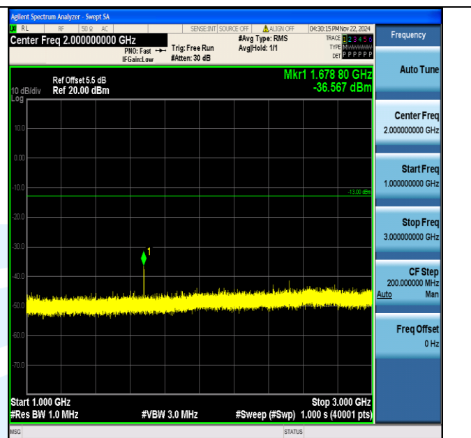
Band5_10MHz_64QAM_20600_1RB#0_1000~3000_1000~3000
