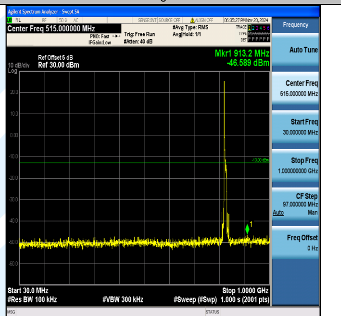
Band5_10MHz_16QAM_20450_1RB#0_30~1000_30~1000
