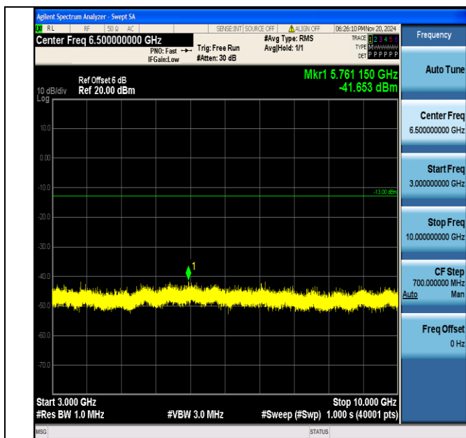
Band5_5MHz_16QAM_20625_1RB#0_3000~10000_3000~10000
