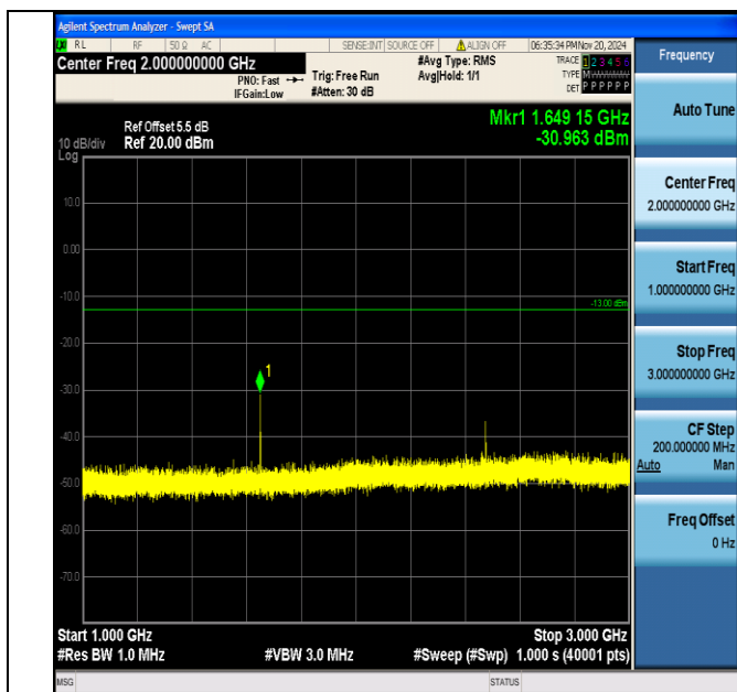
Band5_10MHz_16QAM_20450_1RB#0_1000~3000_1000~3000
