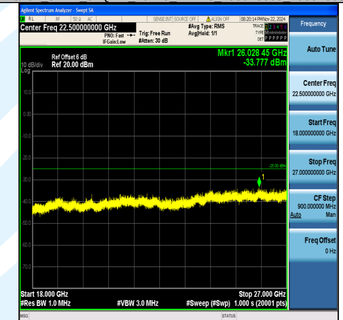
Band7_5MHz_64QAM_20775_1RB#0_18000~27000_18000~27000
