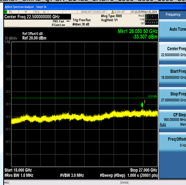
Band7_5MHz_QPSK_21425_1RB#0_18000~27000_18000~27000
