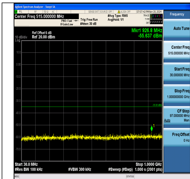
Band7_5MHz_QPSK_20775_1RB#0_30~1000_30~1000
