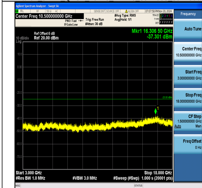
Band7_5MHz_QPSK_20775_1RB#0_3000~18000_3000~18000
