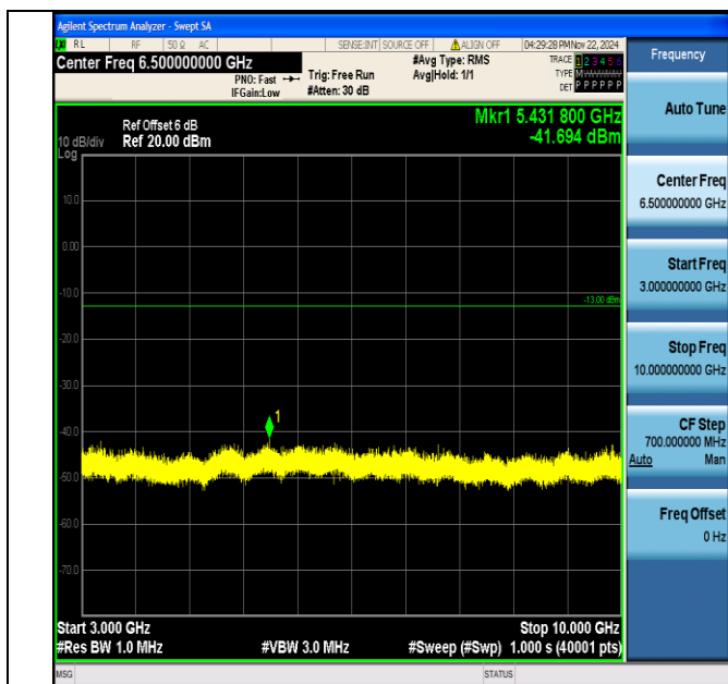
Band5_10MHz_64QAM_20450_1RB#0_3000~10000_3000~10000
