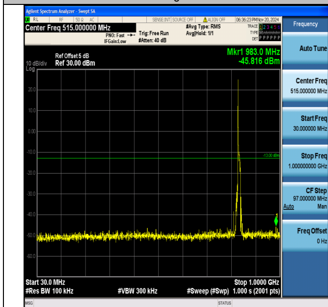
Band5_10MHz_16QAM_20525_1RB#0_30~1000_30~1000
