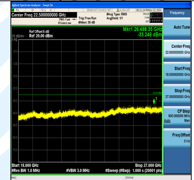
Band7_5MHz_64QAM_21425_1RB#0_18000~27000_18000~27000
