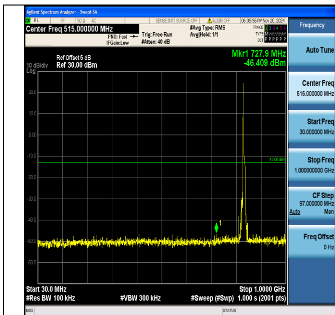
Band5 10MHz QPSK 20525 1RB#0 30~1000 30~1000
