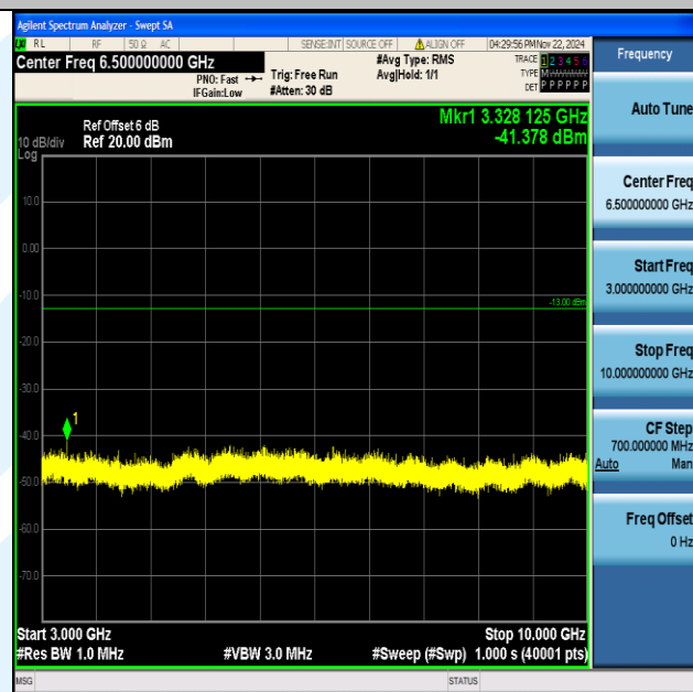
Band5_10MHz_64QAM_20525_1RB#0_3000~10000_3000~10000
