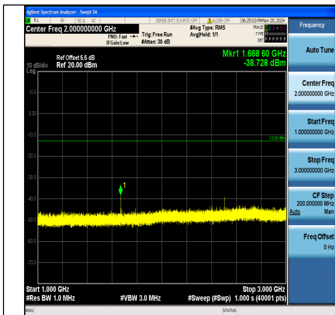
Band5_5MHz_16QAM_20525_1RB#0_1000~3000_1000~3000
