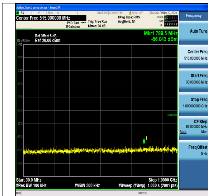
Band7 5MHz 64QAM 21425 1RB#0 30~1000 30~1000
