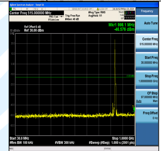
Band5_10MHz_QPSK_20600_1RB#0_30~1000_30~1000
