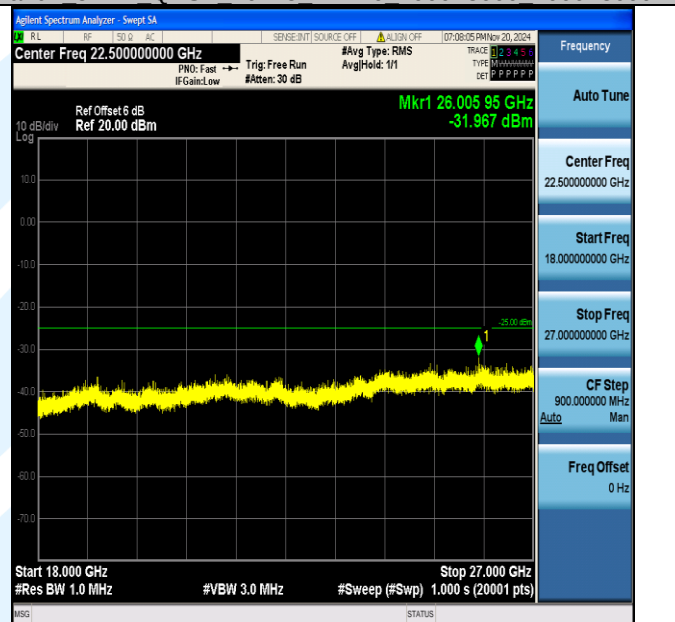
Band7_5MHz_QPSK_20775_1RB#0_18000~27000_18000~27000
