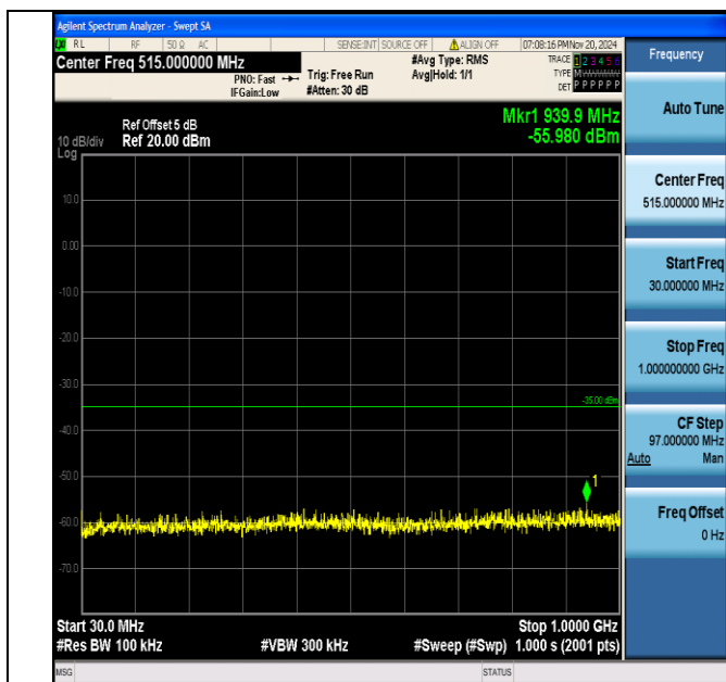
Band7_5MHz_16QAM_20775_1RB#0_30~1000_30~1000
