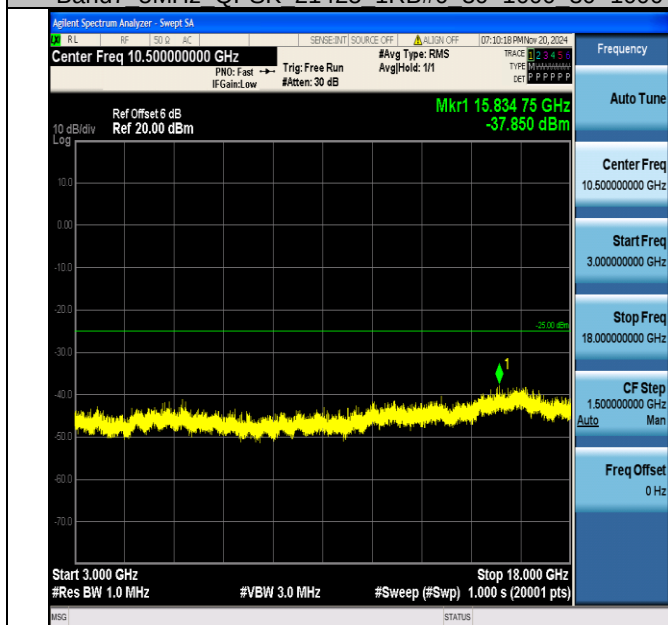
Band7_5MHz_QPSK_21425_1RB#0_3000~18000_3000~18000
