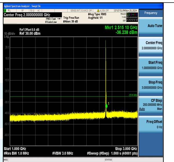
Band7_5MHz_QPSK_20775_1RB#0_1000~3000_1000~3000
