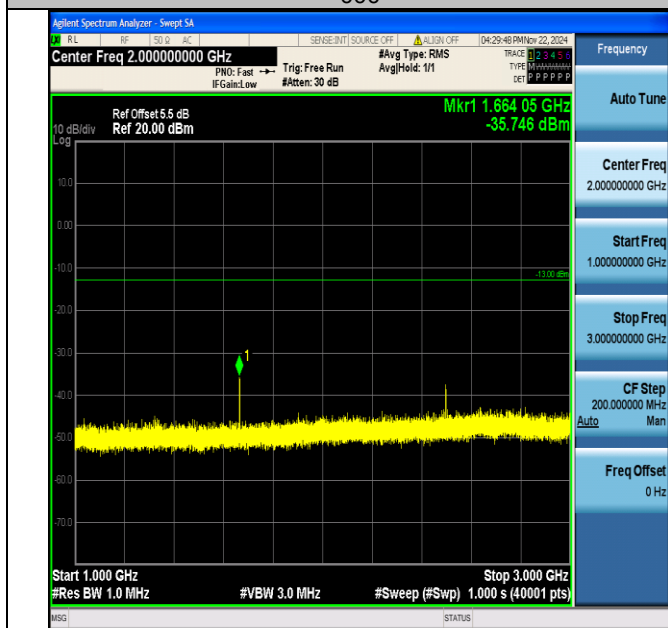
Band5_10MHz_64QAM_20525_1RB#0_1000~3000_1000~3000
