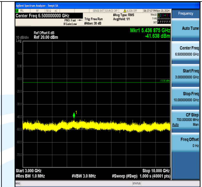
Band5_10MHz_QPSK_20600_1RB#0_3000~10000_3000~10000
