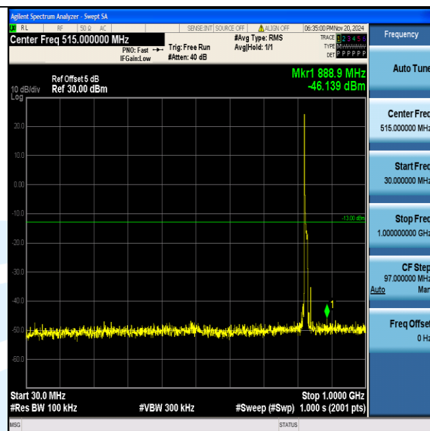
Band5_10MHz_QPSK_20450_1RB#0_30~1000_30~1000
