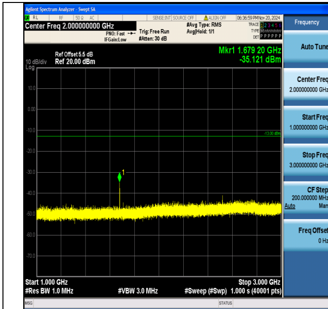
Band5_10MHz_QPSK_20600_1RB#0_1000~3000_1000~3000
