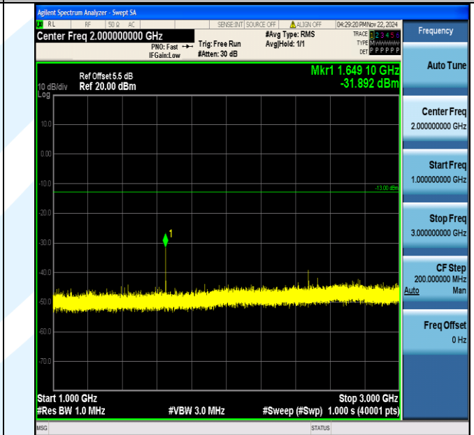
Band5_10MHz_64QAM_20450_1RB#0_1000~3000_1000~3000
