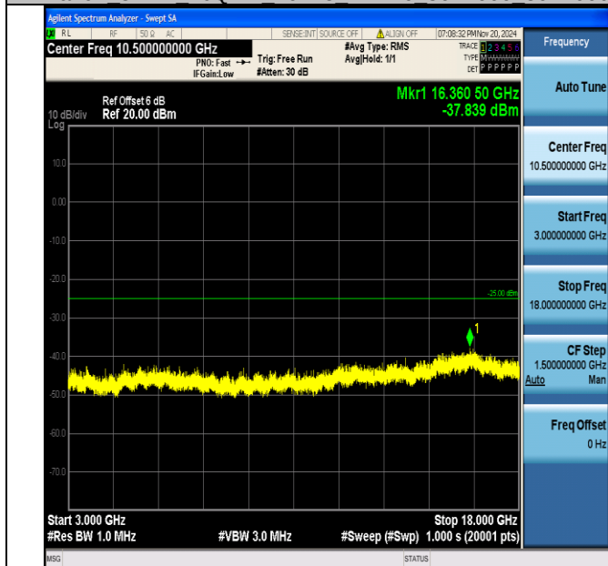
Band7_5MHz_16QAM_20775_1RB#0_3000~18000_3000~18000
