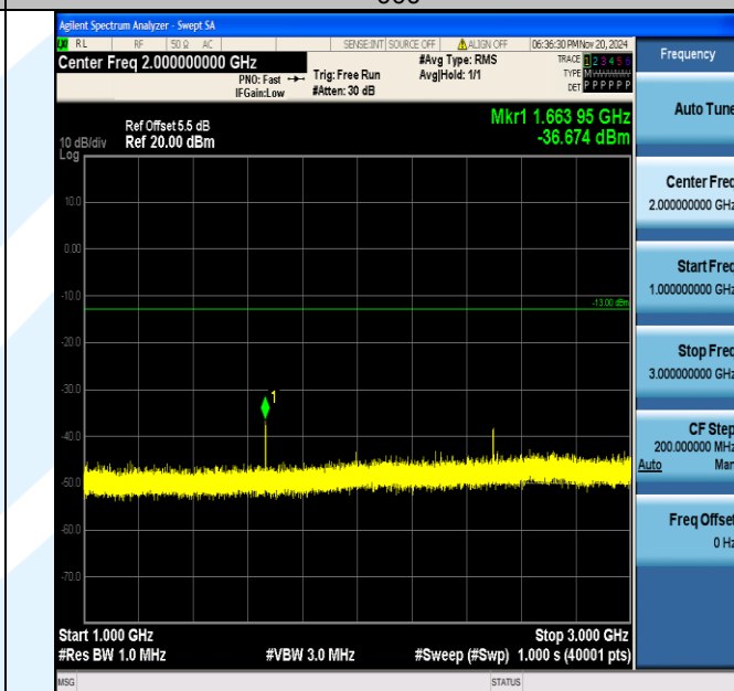
Band5_10MHz_16QAM_20525_1RB#0_1000~3000_1000~3000
