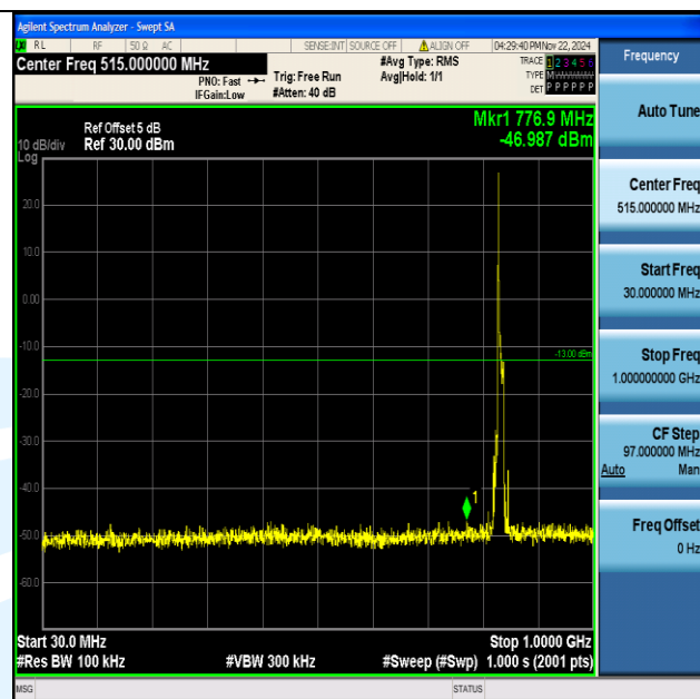
Band5_10MHz_64QAM_20525_1RB#0_30~1000_30~1000
