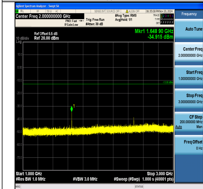
Band5_10MHz_QPSK_20450_1RB#0_1000~3000_1000~3000
