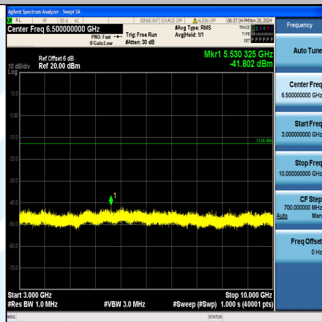
Band5_10MHz_16QAM_20600_1RB#0_3000~10000_3000~10000
