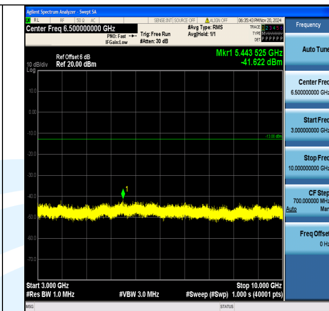
Band5_10MHz_16QAM_20450_1RB#0_3000~10000_3000~10000
