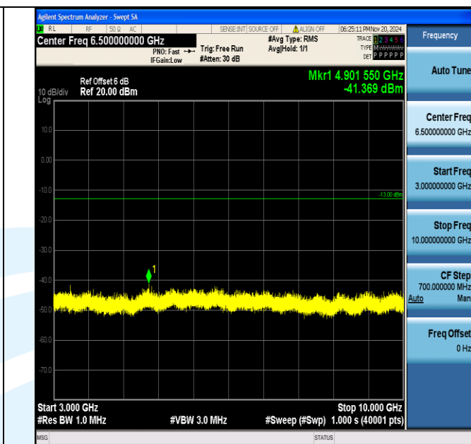
Band5_5MHz_16QAM_20525_1RB#0_3000~10000_3000~10000
