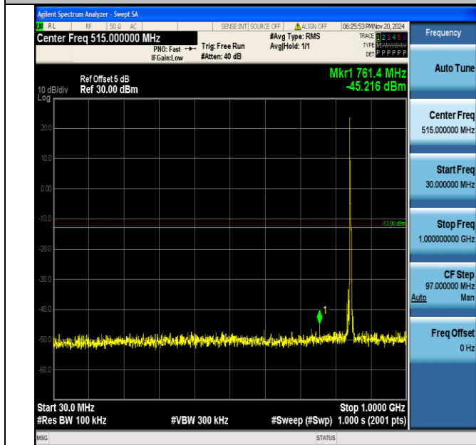
Band5_5MHz_16QAM_20625_1RB#0_30~1000_30~1000
