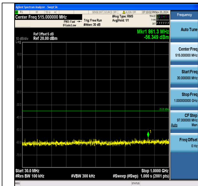
Band7_5MHz_QPSK_21425_1RB#0_30~1000_30~1000
