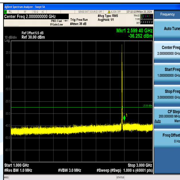
Band7_5MHz_QPSK_21425_1RB#0_1000~3000_1000~3000
