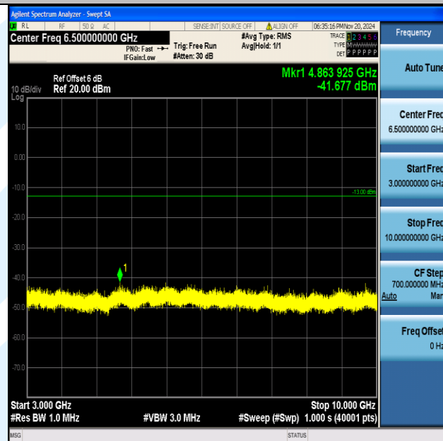
Band5_10MHz_QPSK_20450_1RB#0_3000~10000_3000~10000
