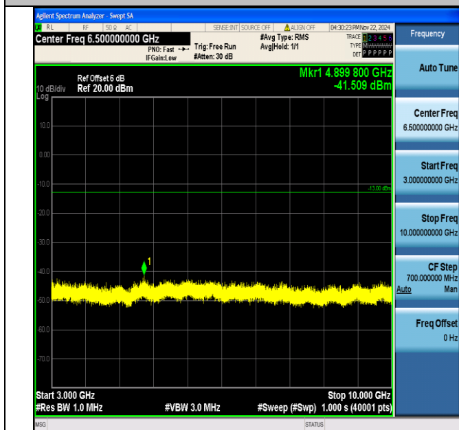
Band5_10MHz_64QAM_20600_1RB#0_3000~10000_3000~10000
