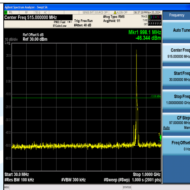
Band5_10MHz_16QAM_20600_1RB#0_30~1000_30~1000
