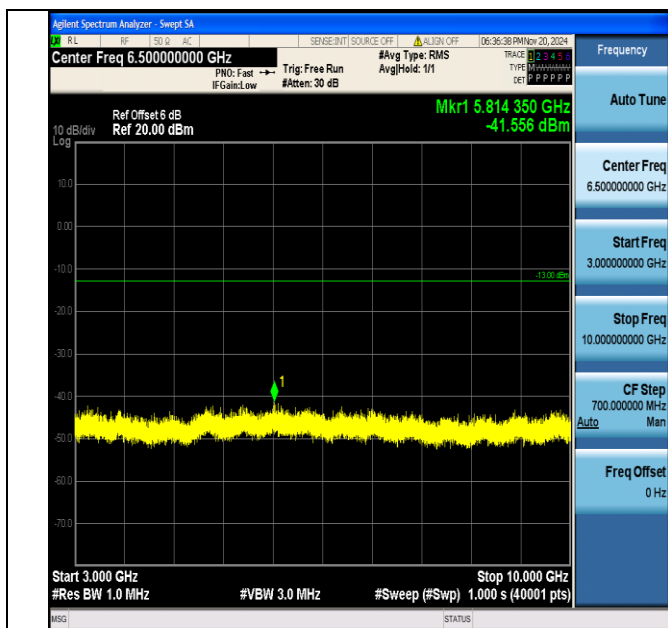
Band5_10MHz_16QAM_20525_1RB#0_3000~10000_3000~10000
