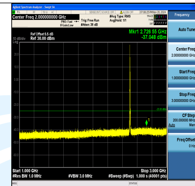
Band7_5MHz_16QAM_20775_1RB#0_1000~3000_1000~3000
