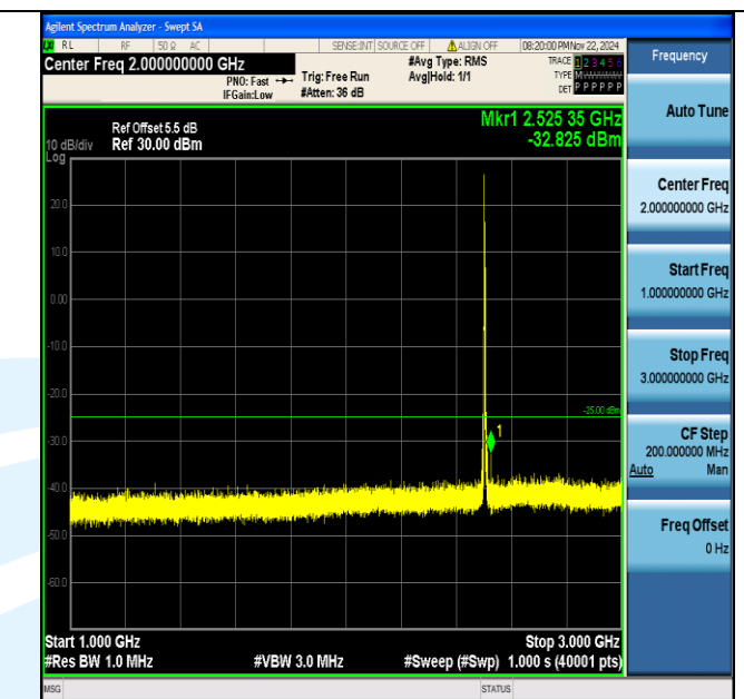
Band7_5MHz_64QAM_20775_1RB#0_1000~3000_1000~3000
