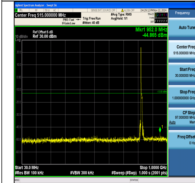
Band5_10MHz_64QAM_20450_1RB#0_30~1000_30~1000
