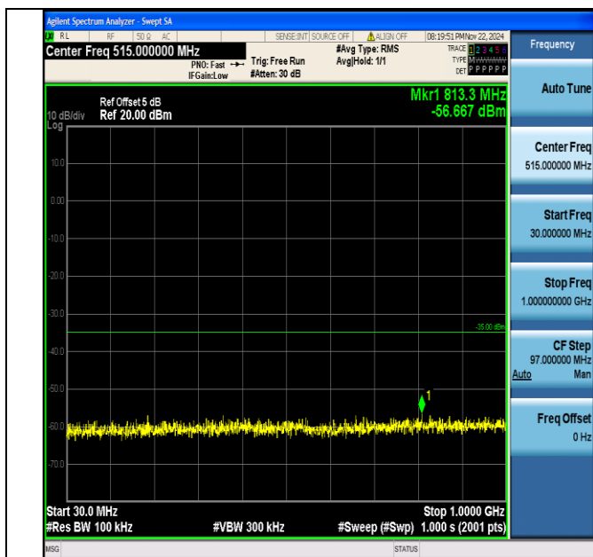
Band7_5MHz_64QAM_20775_1RB#0_30~1000_30~1000
