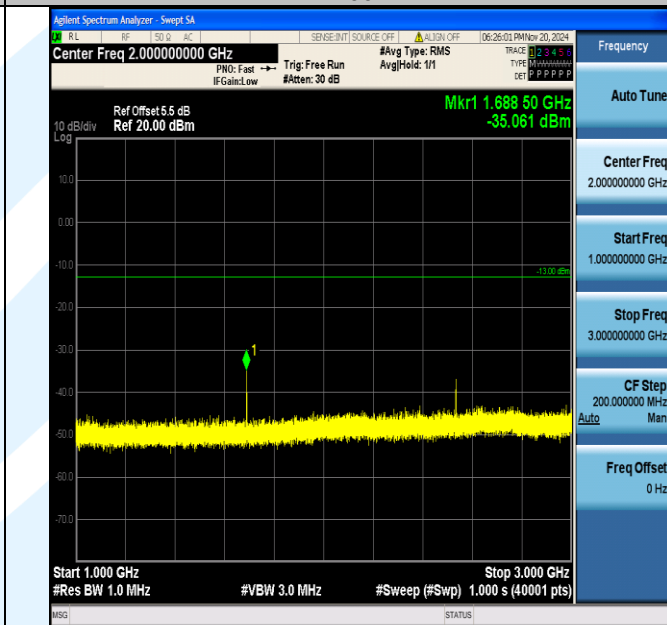
Band5_5MHz_16QAM_20625_1RB#0_1000~3000_1000~3000
