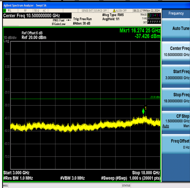
Band7_5MHz_64QAM_21425_1RB#0_3000~18000_3000~18000
