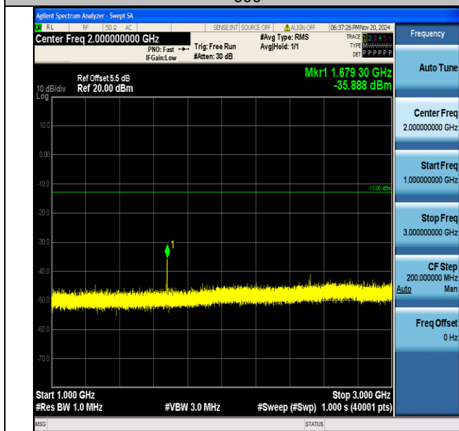
Band5_10MHz_16QAM_20600_1RB#0_1000~3000_1000~3000
