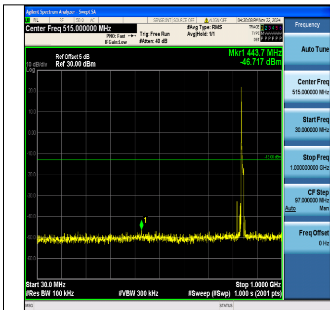
Band5_10MHz_64QAM_20600_1RB#0_30~1000_30~1000
