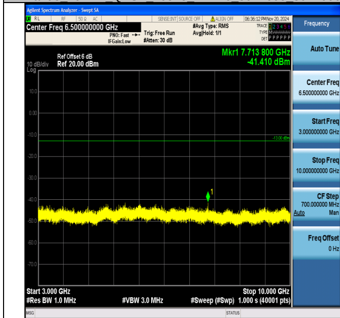
Band5_10MHz_QPSK_20525_1RB#0_3000~10000_3000~10000
