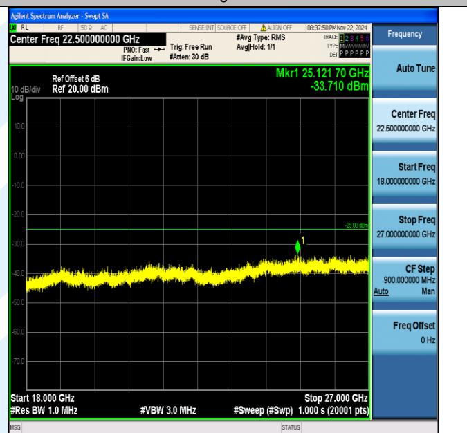
Band7_20MHz_64QAM_20850_1RB#0_18000~27000_18000~27000
