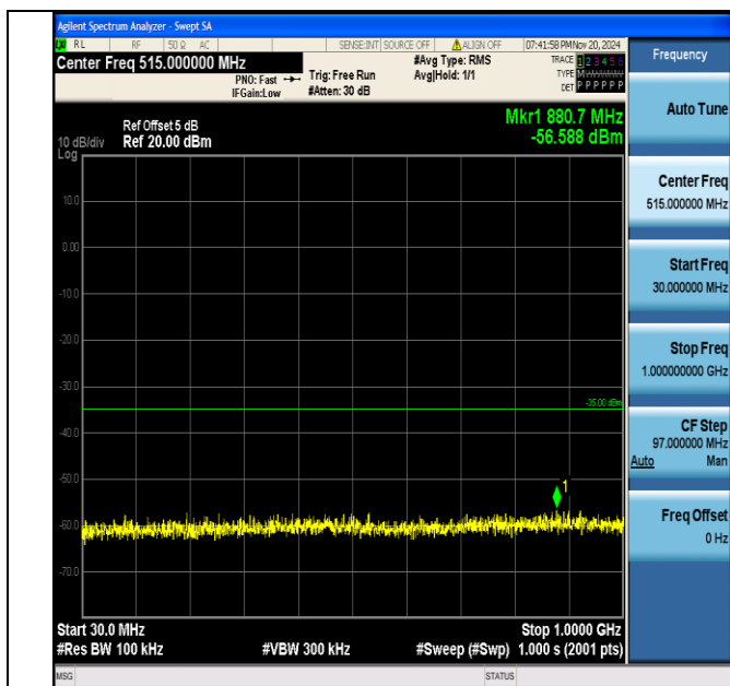
Band7_20MHz_QPSK_20850_1RB#0_30~1000_30~1000
