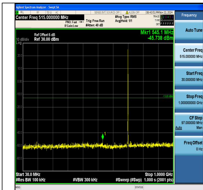
Band12_1.4MHz_64QAM_23095_1RB#0_30~1000_30~1000
