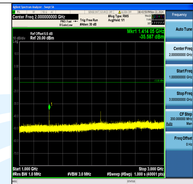
Band12_1.4MHz_64QAM_23095_1RB#0_1000~3000_1000~3000
