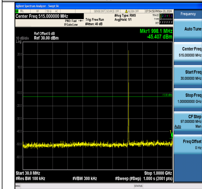
Band12_1.4MHz_QPSK_23173_1RB#0_30~1000_30~1000
