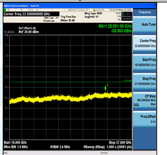
Band7_15MHz_16QAM_20825_1RB#0_18000~27000_18000~27000
