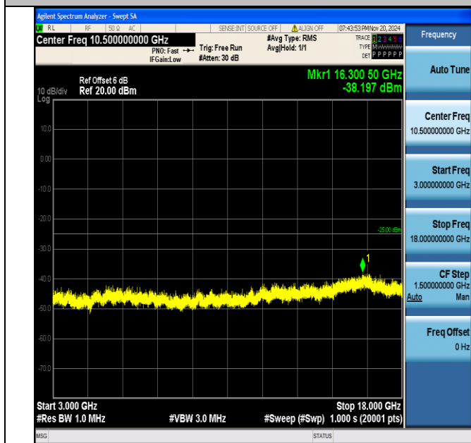
Band7_20MHz_16QAM_21100_1RB#0_3000~18000_3000~18000
