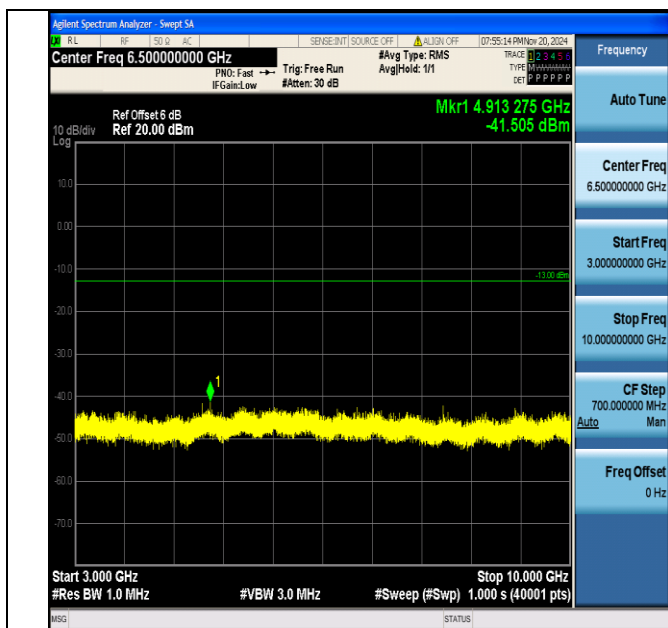
Band12_1.4MHz_QPSK_23173_1RB#0_3000~10000_3000~10000
