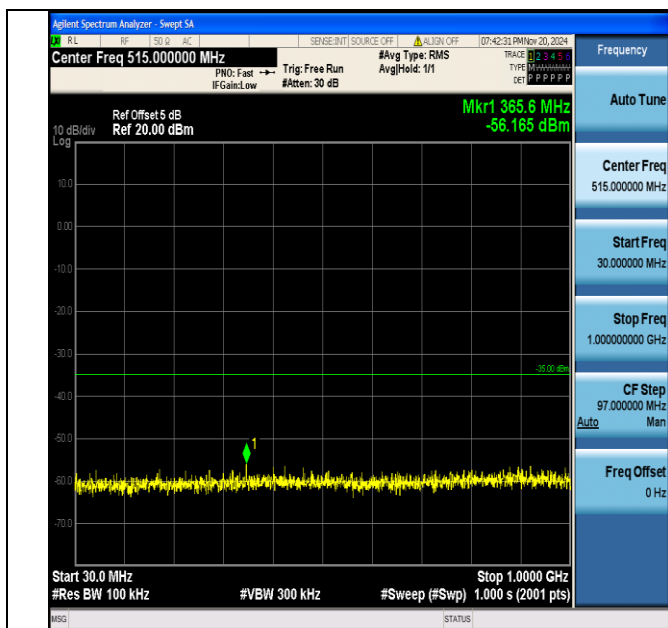
Band7_20MHz_16QAM_20850_1RB#0_30~1000_30~1000
