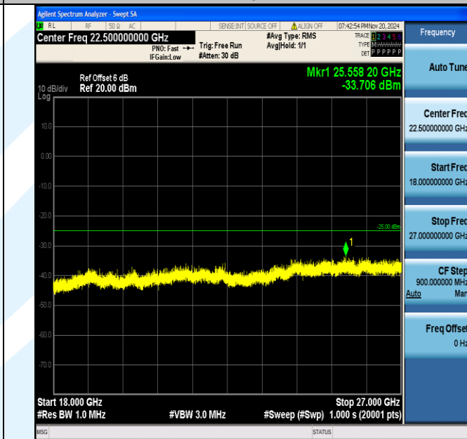
Band7_20MHz_16QAM_20850_1RB#0_18000~27000_18000~27000
