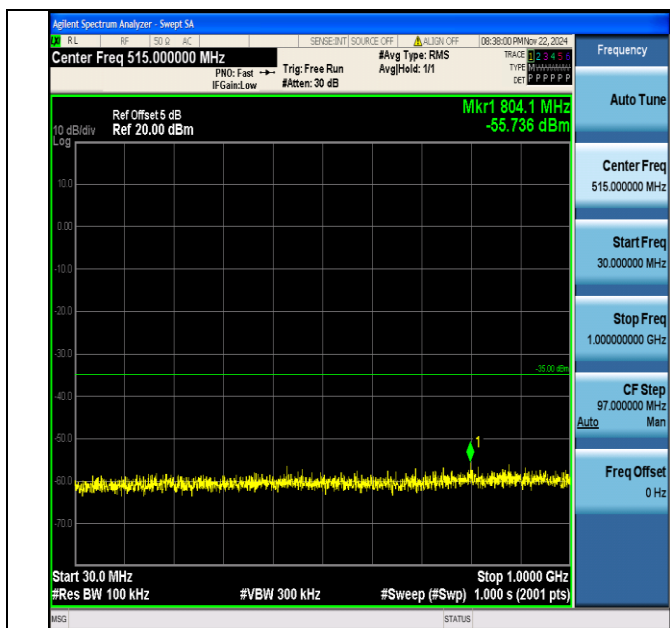
Band7_20MHz_64QAM_21100_1RB#0_30~1000_30~1000
