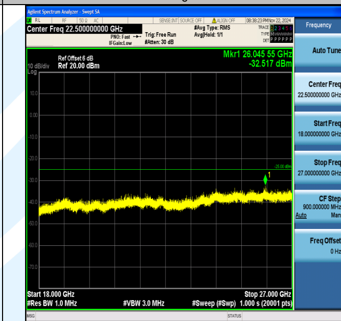
Band7_20MHz_64QAM_21100_1RB#0_18000~27000_18000~27000
