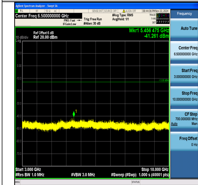
Band12_1.4MHz_64QAM_23095_1RB#0_3000~10000_3000~10000
