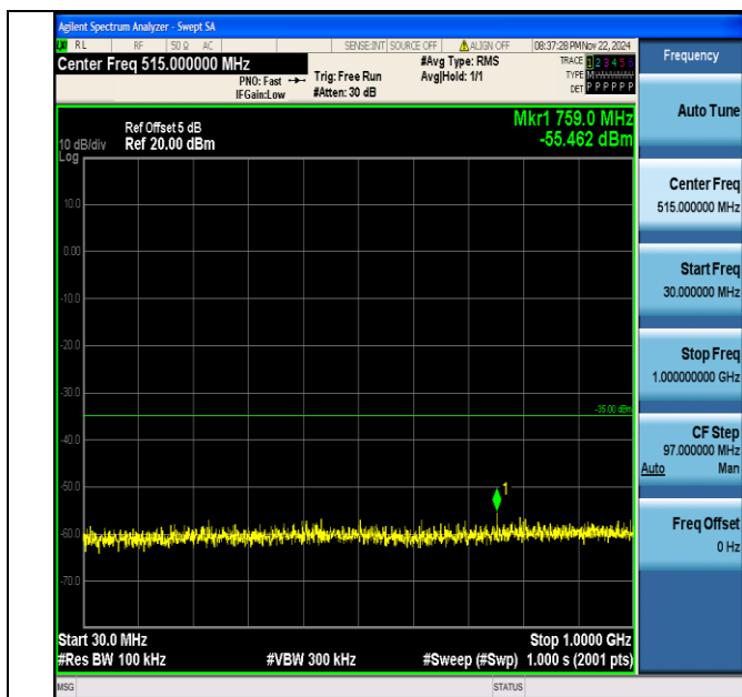
Band7_20MHz_64QAM_20850_1RB#0_30~1000_30~1000
