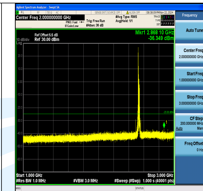
Band7_20MHz_64QAM_21100_1RB#0_1000~3000_1000~3000
