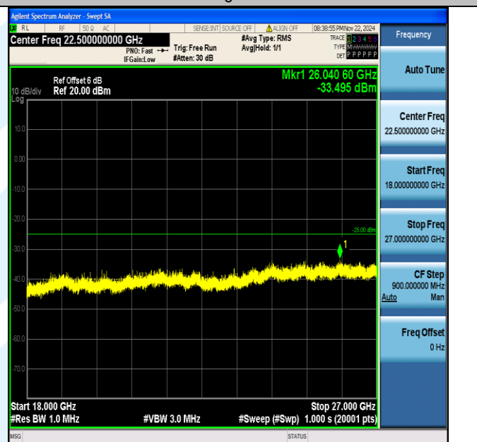
Band7_20MHz_64QAM_21350_1RB#0_18000~27000_18000~27000
