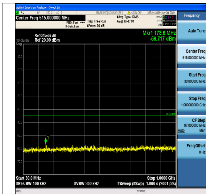
Band7_20MHz_QPSK_21350_1RB#0_30~1000_30~1000
