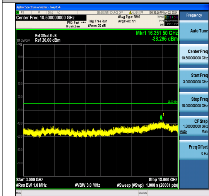
Band7_20MHz_64QAM_21100_1RB#0_3000~18000_3000~18000
