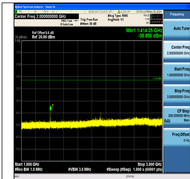
Band12_1.4MHz_QPSK_23095_1RB#0_1000~3000_1000~3000
