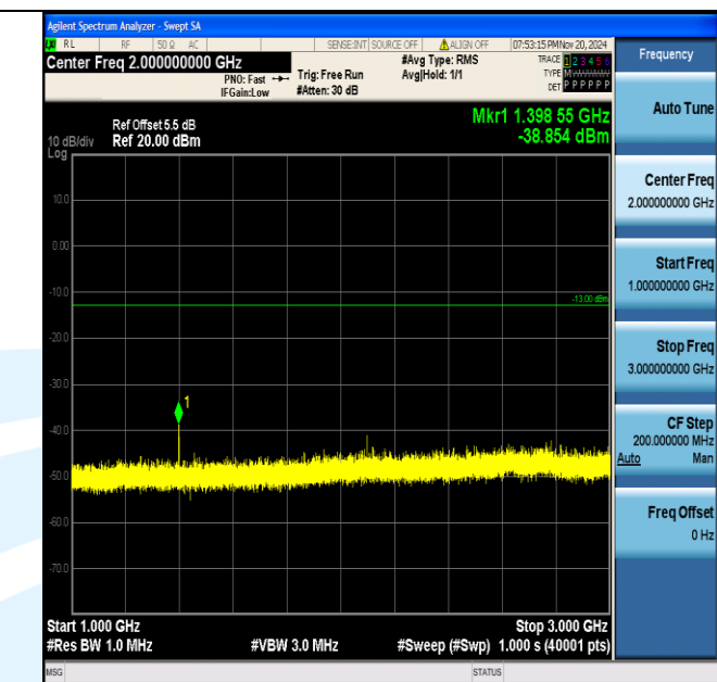
Band12_1.4MHz_QPSK_23017_1RB#0_1000~3000_1000~3000
