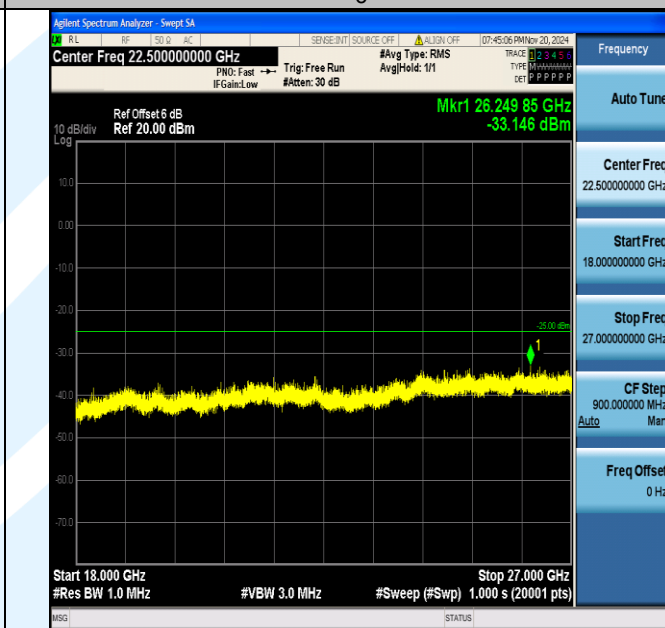
Band7_20MHz_16QAM_21350_1RB#0_18000~27000_18000~27000
