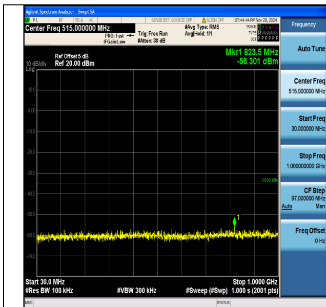
Band7_20MHz_16QAM_21350_1RB#0_30~1000_30~1000
