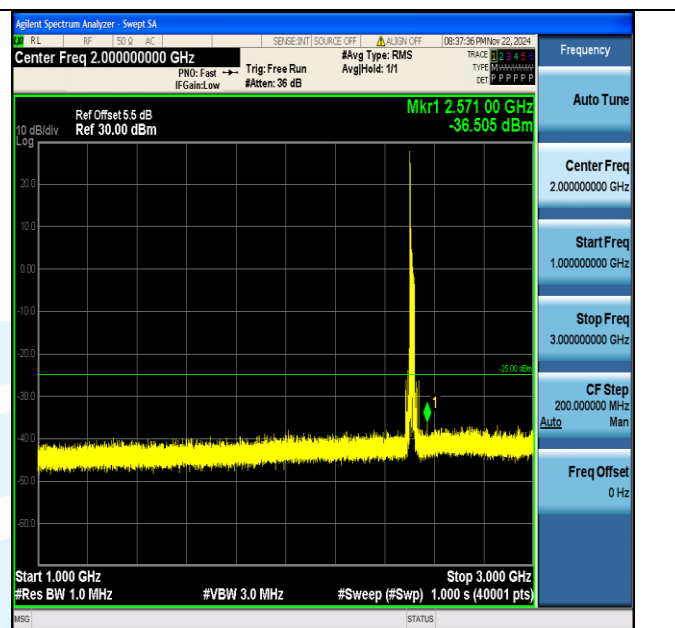
Band7_20MHz_64QAM_20850_1RB#0_1000~3000_1000~3000
