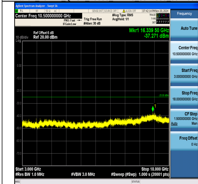
Band7_20MHz_QPSK_20850_1RB#0_3000~18000_3000~18000
