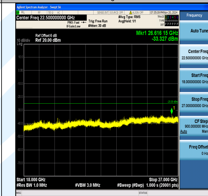
Band7_15MHz_16QAM_21375_1RB#0_18000~27000_18000~27000
