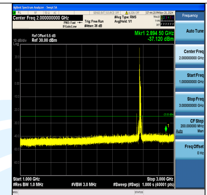
Band7_20MHz_QPSK_21350_1RB#0_1000~3000_1000~3000
