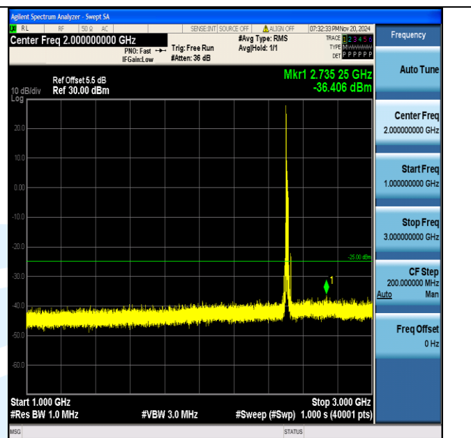
Band7_15MHz_16QAM_20825_1RB#0_1000~3000_1000~3000
