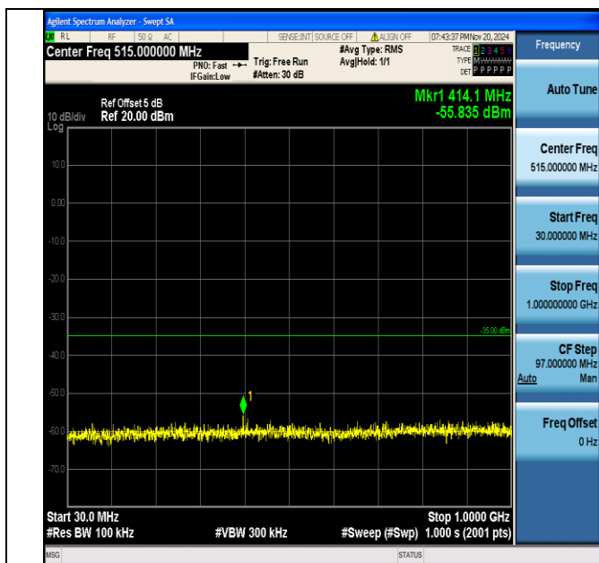
Band7_20MHz_16QAM_21100_1RB#0_30~1000_30~1000
