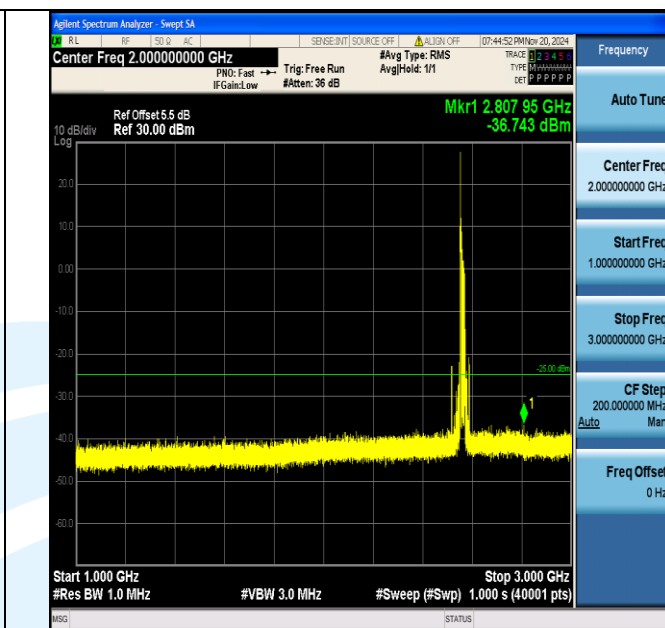
Band7_20MHz_16QAM_21350_1RB#0_1000~3000_1000~3000
