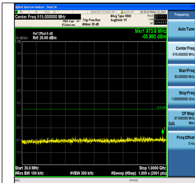
Band7_20MHz_64QAM_21350_1RB#0_30~1000_30~1000
