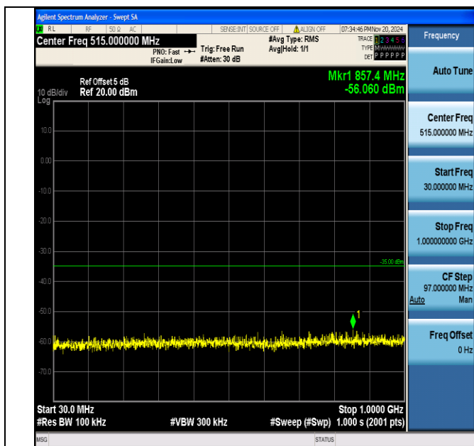
Band7_15MHz_16QAM_21375_1RB#0_30~1000_30~1000
