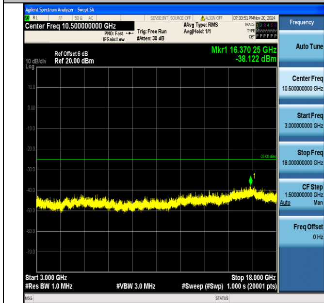
Band7_15MHz_16QAM_21100_1RB#0_3000~18000_3000~18000
