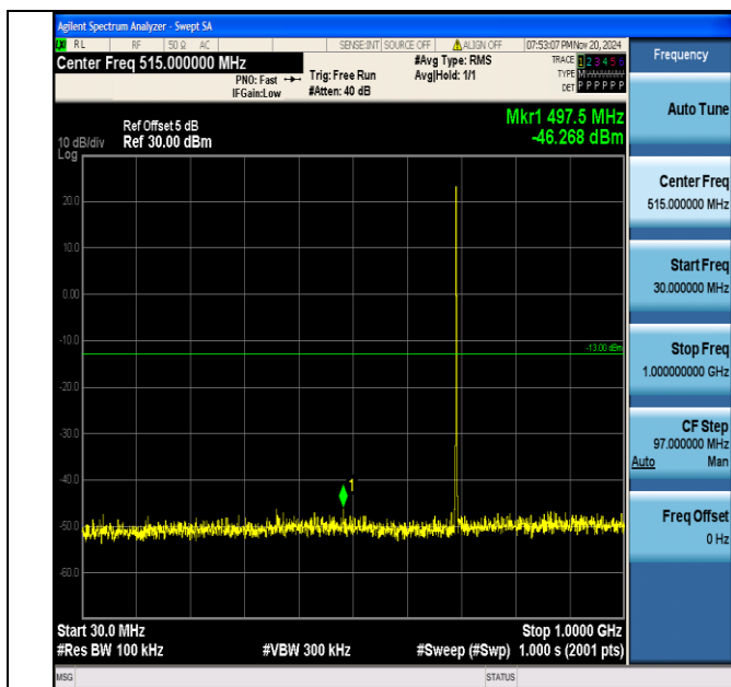
Band12_1.4MHz_QPSK_23017_1RB#0_30~1000_30~1000
