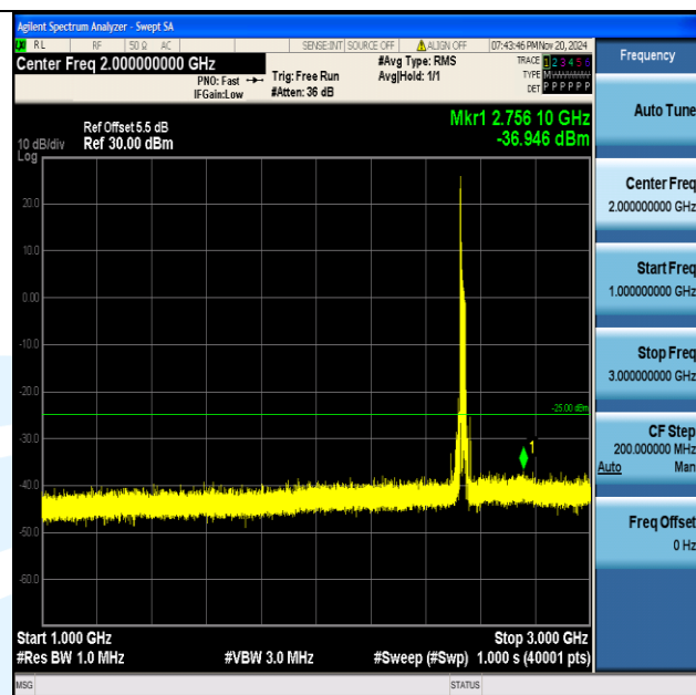
Band7_20MHz_16QAM_21100_1RB#0_1000~3000_1000~3000
