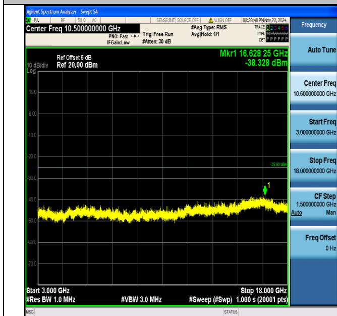
Band7_20MHz_64QAM_21350_1RB#0_3000~18000_3000~18000
