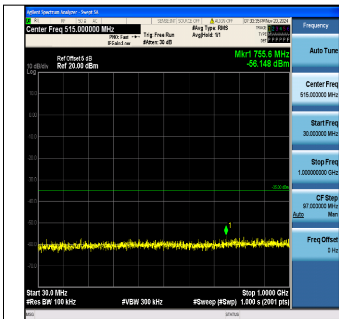
Band7_15MHz_16QAM_21100_1RB#0_30~1000_30~1000
