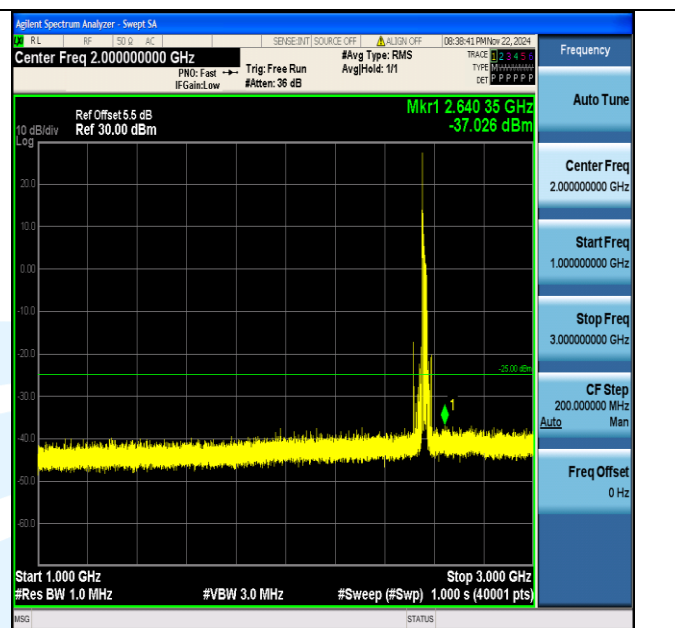
Band7_20MHz_64QAM_21350_1RB#0_1000~3000_1000~3000
