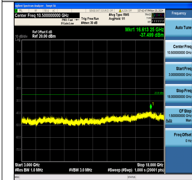
Band7_20MHz_16QAM_20850_1RB#0_3000~18000_3000~18000
