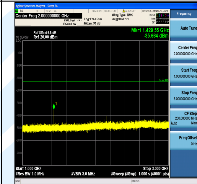
Band12_1.4MHz_QPSK_23173_1RB#0_1000~3000_1000~3000
