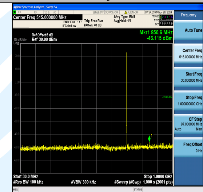
Band12_1.4MHz_QPSK_23095_1RB#0_30~1000_30~1000
