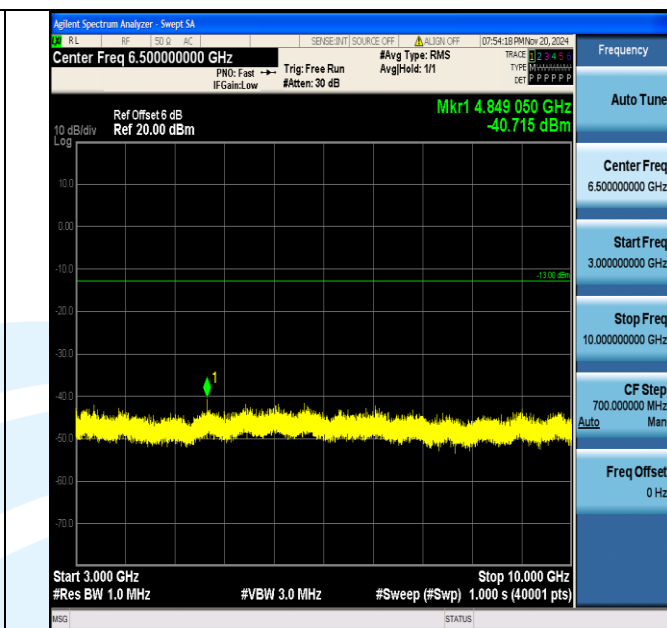
Band12_1.4MHz_QPSK_23095_1RB#0_3000~10000_3000~10000
