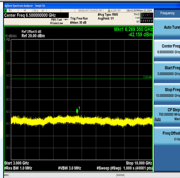
Band12_1.4MHz_64QAM_23017_1RB#0_3000~10000_3000~10000
