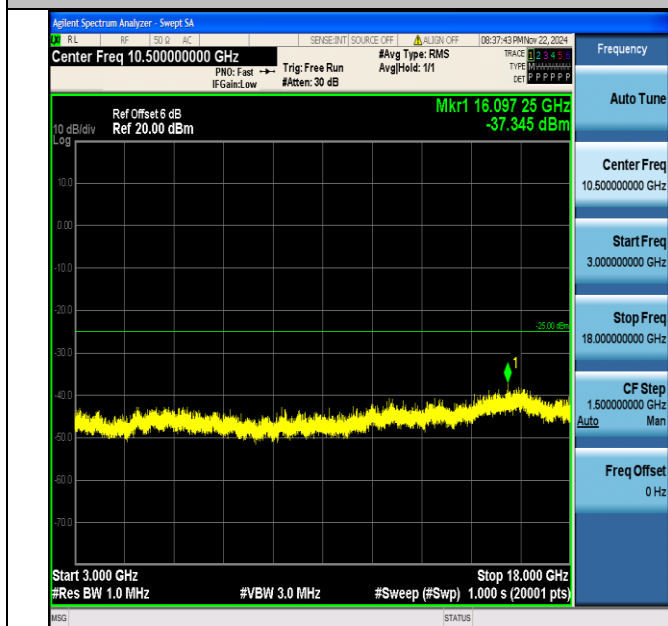
Band7_20MHz_64QAM_20850_1RB#0_3000~18000_3000~18000
