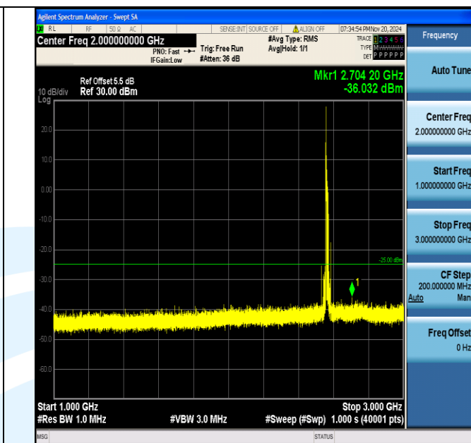
Band7_15MHz_16QAM_21375_1RB#0_1000~3000_1000~3000
