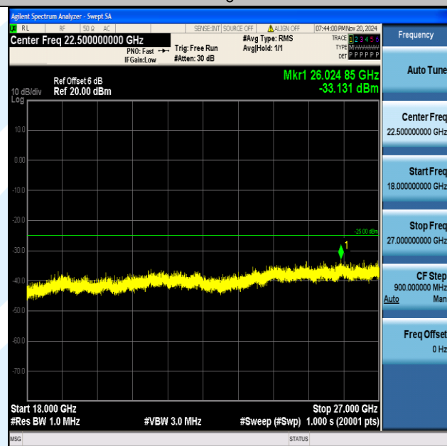
Band7_20MHz_16QAM_21100_1RB#0_18000~27000_18000~27000
