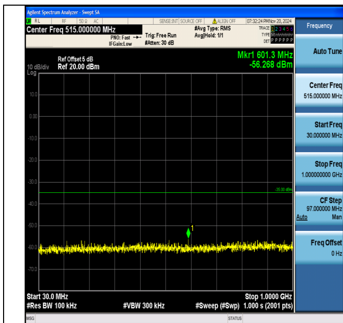
Band7_15MHz_16QAM_20825_1RB#0_30~1000_30~1000
