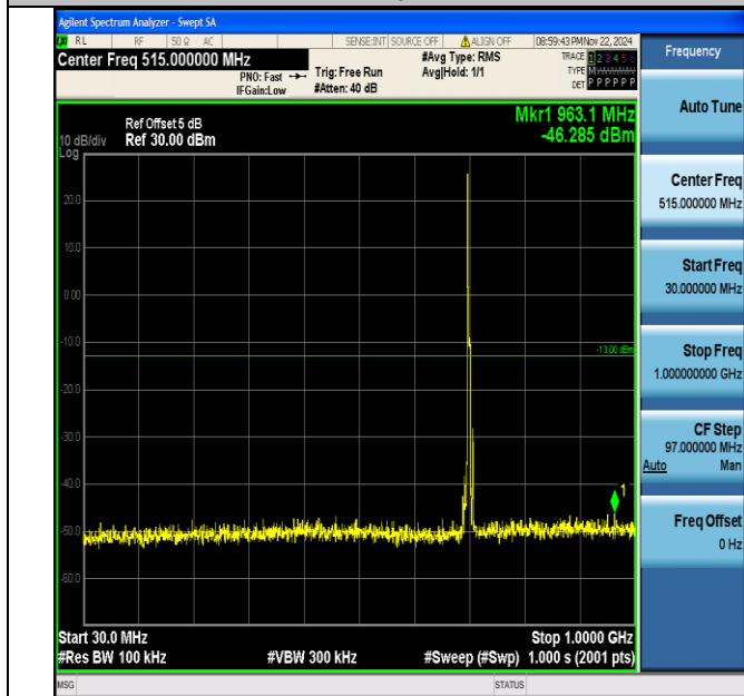
Band12_5MHz_64QAM_23095_1RB#0_30~1000_30~1000
