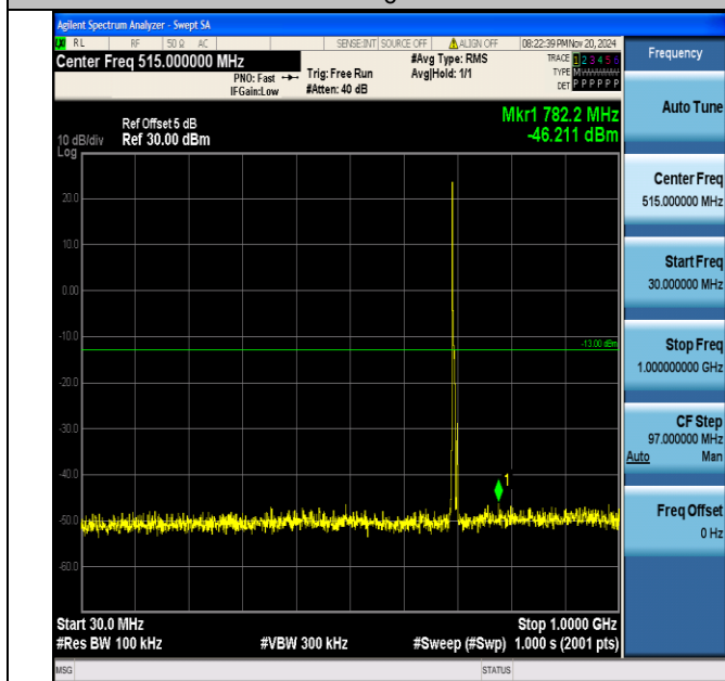
Band12_5MHz_QPSK_23035_1RB#0_30~1000_30~1000
