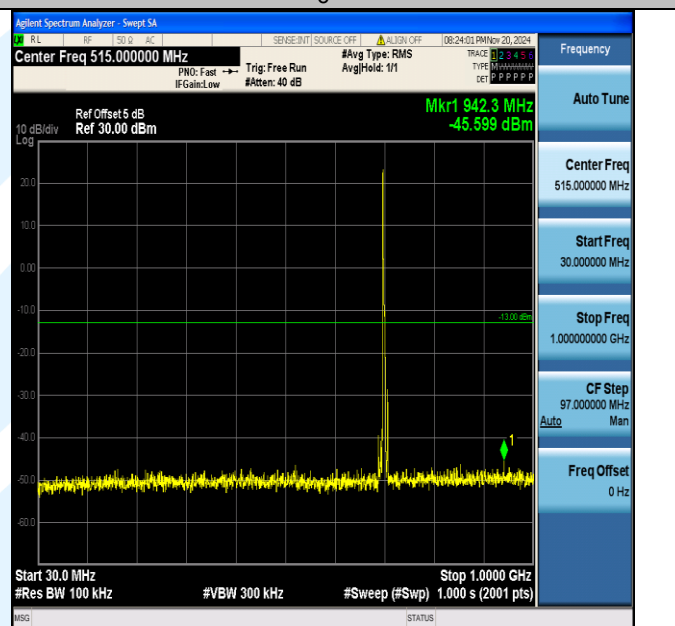
Band12_5MHz_16QAM_23095_1RB#0_30~1000_30~1000
