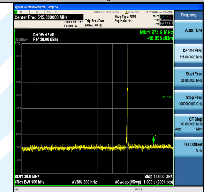
Band12_3MHz_64QAM_23095_1RB#0_30~1000_30~1000
