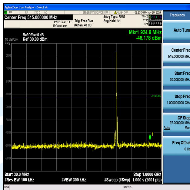
Band12_5MHz_QPSK_23095_1RB#0_30~1000_30~1000
