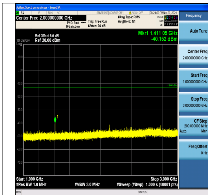
Band12_5MHz_16QAM_23095_1RB#0_1000~3000_1000~3000
