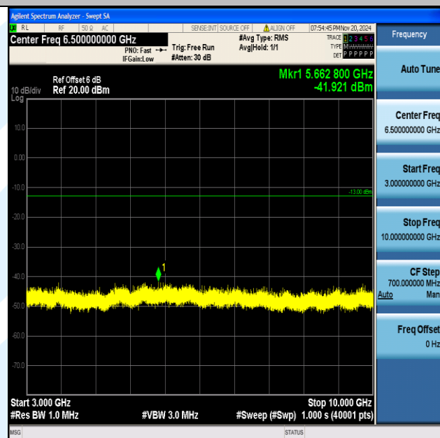
Band12_1.4MHz_16QAM_23095_1RB#0_3000~10000_3000~10000
