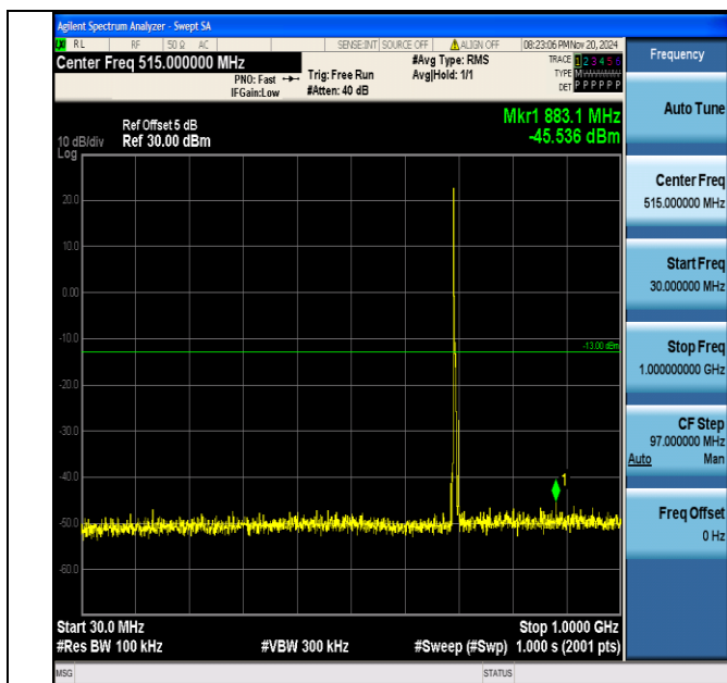
Band12_5MHz_16QAM_23035_1RB#0_30~1000_30~1000
