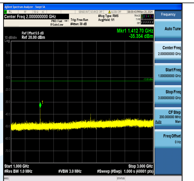
Band12_3MHz_16QAM_23095_1RB#0_1000~3000_1000~3000
