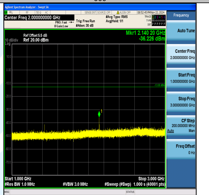
Band12_3MHz_64QAM_23165_1RB#0_1000~3000_1000~3000
