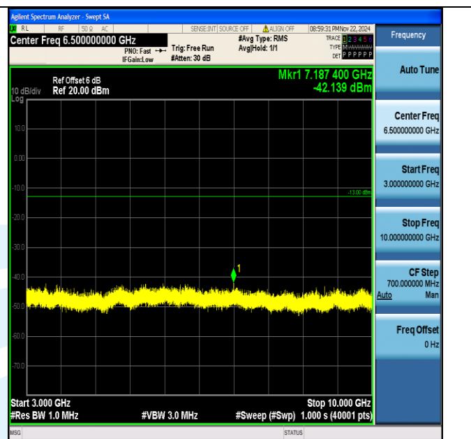
Band12_5MHz_64QAM_23035_1RB#0_3000~10000_3000~10000
