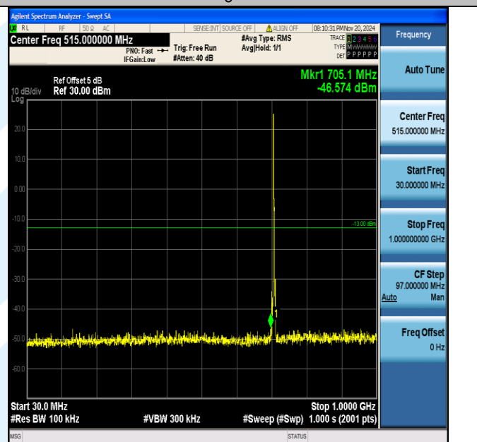
Band12_3MHz_16QAM_23165_1RB#0_30~1000_30~1000
