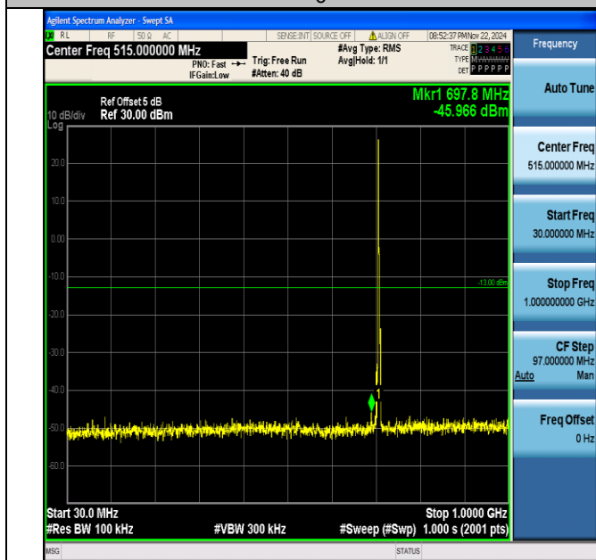
Band12_3MHz_64QAM_23165_1RB#0_30~1000_30~1000
