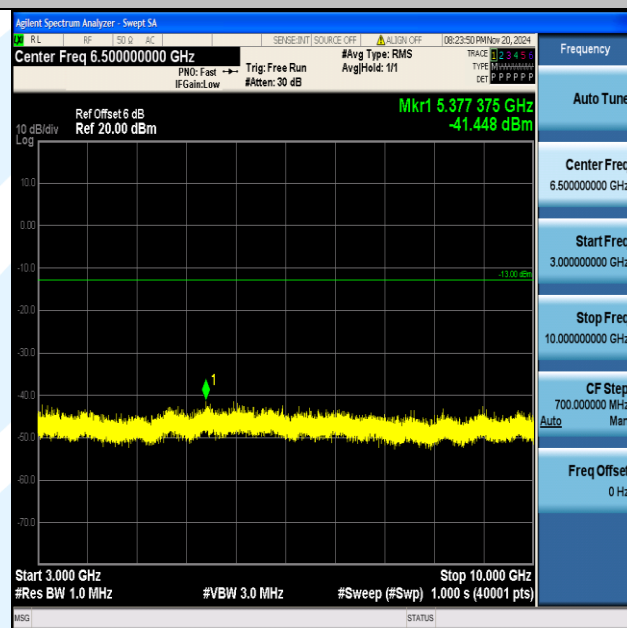
Band12_5MHz_QPSK_23095_1RB#0_3000~10000_3000~10000
