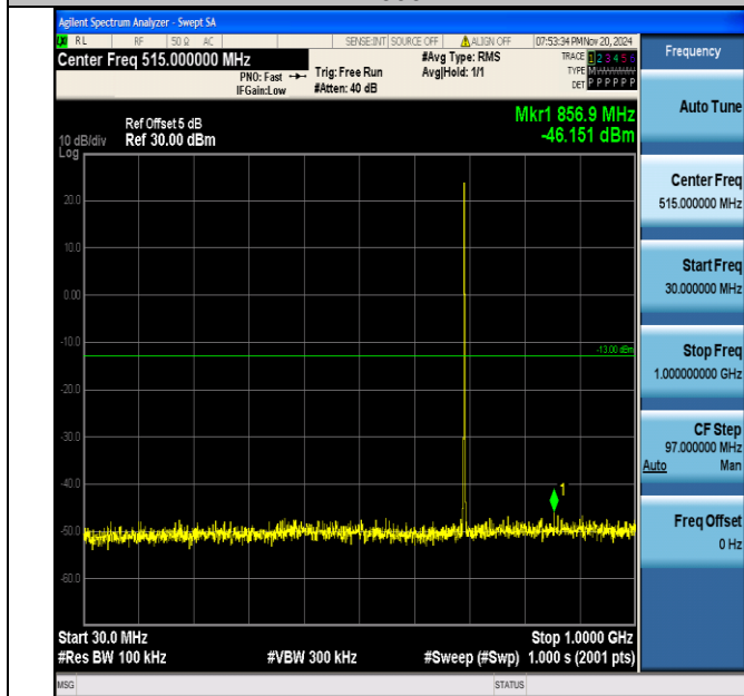
Band12_1.4MHz_16QAM_23017_1RB#0_30~1000_30~1000
