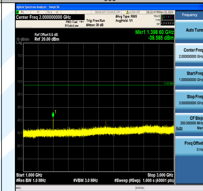
Band12_5MHz_QPSK_23035_1RB#0_1000~3000_1000~3000
