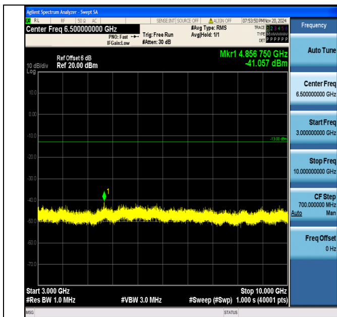
Band12_1.4MHz_16QAM_23017_1RB#0_3000~10000_3000~10000
