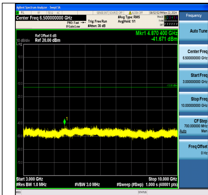
Band12_3MHz_64QAM_23165_1RB#0_3000~10000_3000~10000
