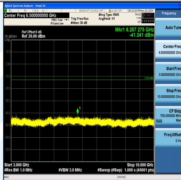
Band12_3MHz_QPSK_23165_1RB#0_3000~10000_3000~10000
