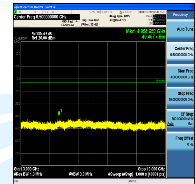
Band12_3MHz_QPSK_23025_1RB#0_3000~10000_3000~10000
