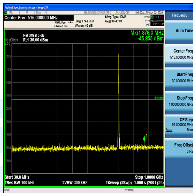
Band12_5MHz_64QAM_23155_1RB#0_30~1000_30~1000
