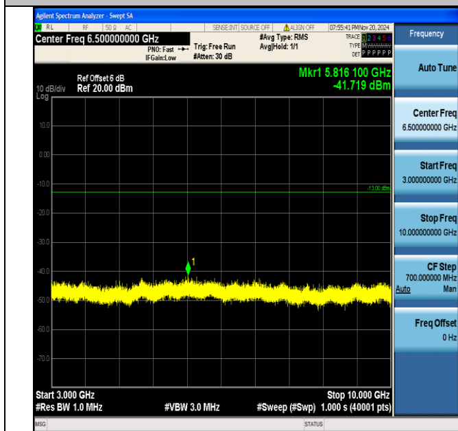
Band12_1.4MHz_16QAM_23173_1RB#0_3000~10000_3000~10000
