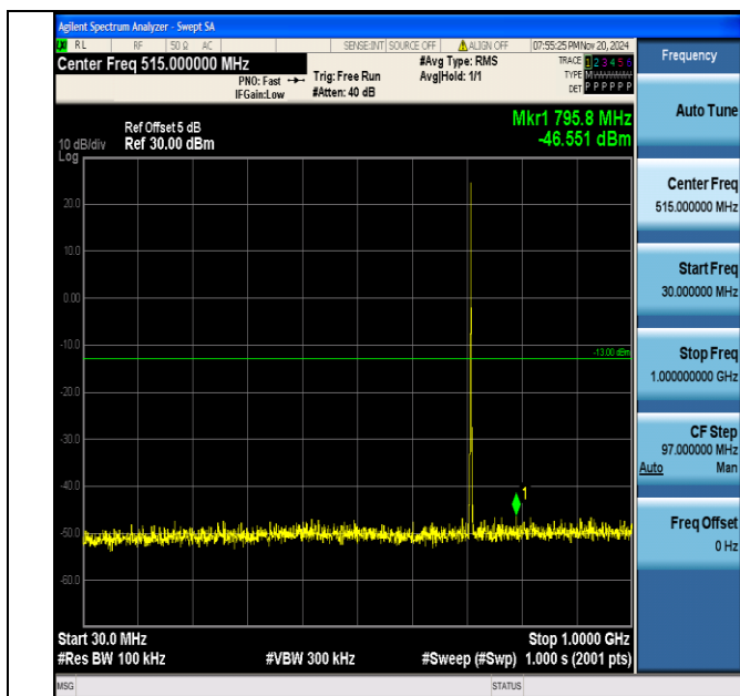
Band12_1.4MHz_16QAM_23173_1RB#0_30~1000_30~1000
