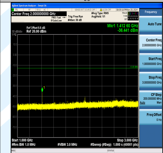
Band12_3MHz_QPSK_23095_1RB#0_1000~3000_1000~3000
