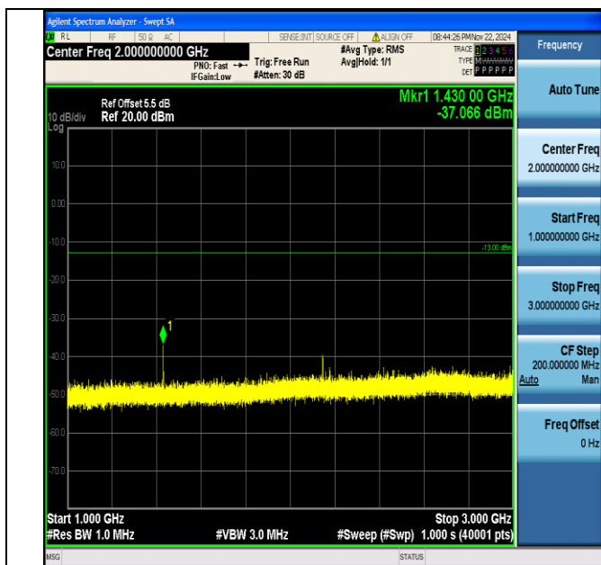
Band12_1.4MHz_64QAM_23173_1RB#0_1000~3000_1000~3000
