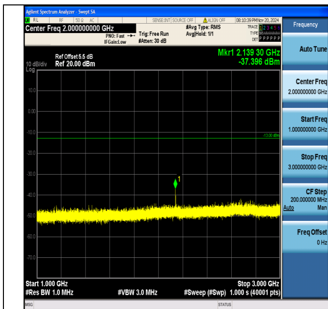
Band12_3MHz_16QAM_23165_1RB#0_1000~3000_1000~3000
