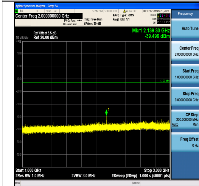
Band12_3MHz_QPSK_23165_1RB#0_1000~3000_1000~3000
