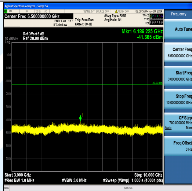
Band12_3MHz_16QAM_23025_1RB#0_3000~10000_3000~10000
