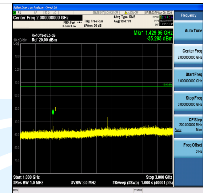
Band12_1.4MHz_16QAM_23173_1RB#0_1000~3000_1000~3000
