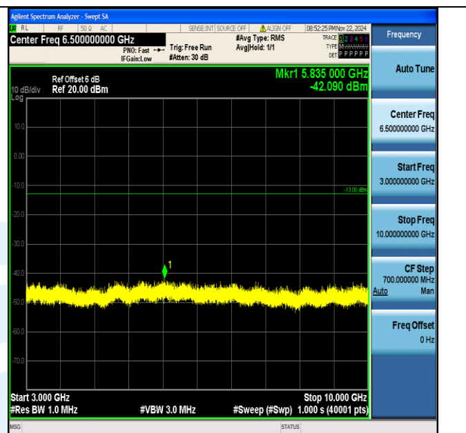
Band12_3MHz_64QAM_23095_1RB#0_3000~10000_3000~10000
