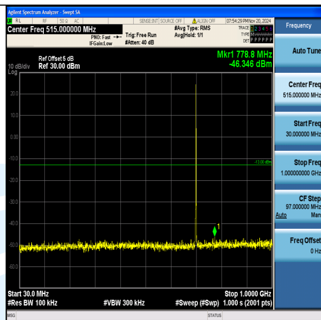
Band12_1.4MHz_16QAM_23095_1RB#0_30~1000_30~1000
