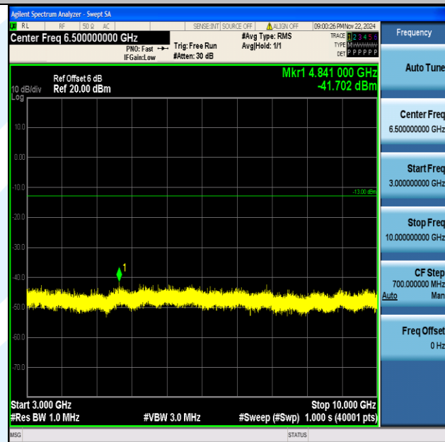
Band12_5MHz_64QAM_23155_1RB#0_3000~10000_3000~10000
