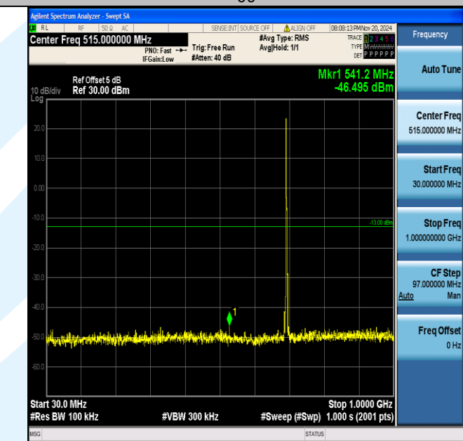
Band12_3MHz_QPSK_23025_1RB#0_30~1000_30~1000
