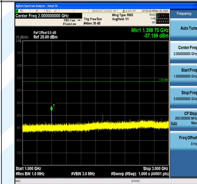
Band12_1.4MHz_16QAM_23017_1RB#0_1000~3000_1000~3000
