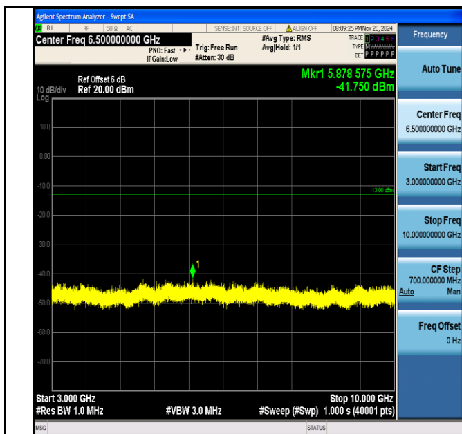
Band12_3MHz_QPSK_23095_1RB#0_3000~10000_3000~10000
