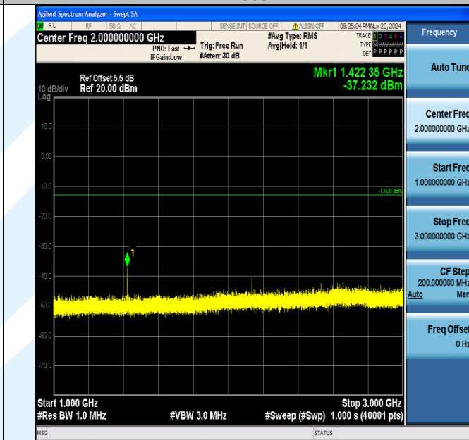
Band12_5MHz_16QAM_23155_1RB#0_1000~3000_1000~3000
