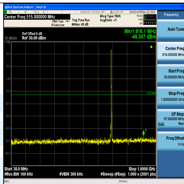
Band12_3MHz_16QAM_23025_1RB#0_30~1000_30~1000
