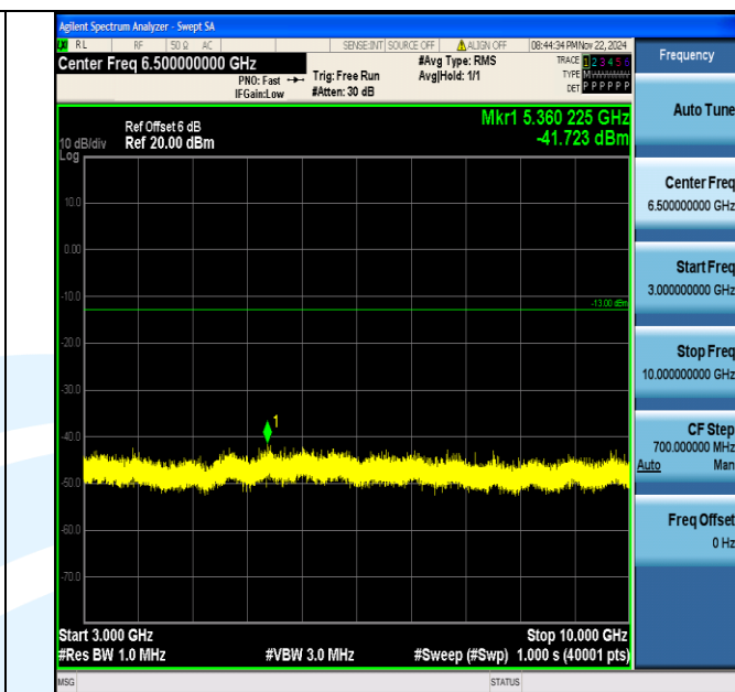
Band12_1.4MHz_64QAM_23173_1RB#0_3000~10000_3000~10000
