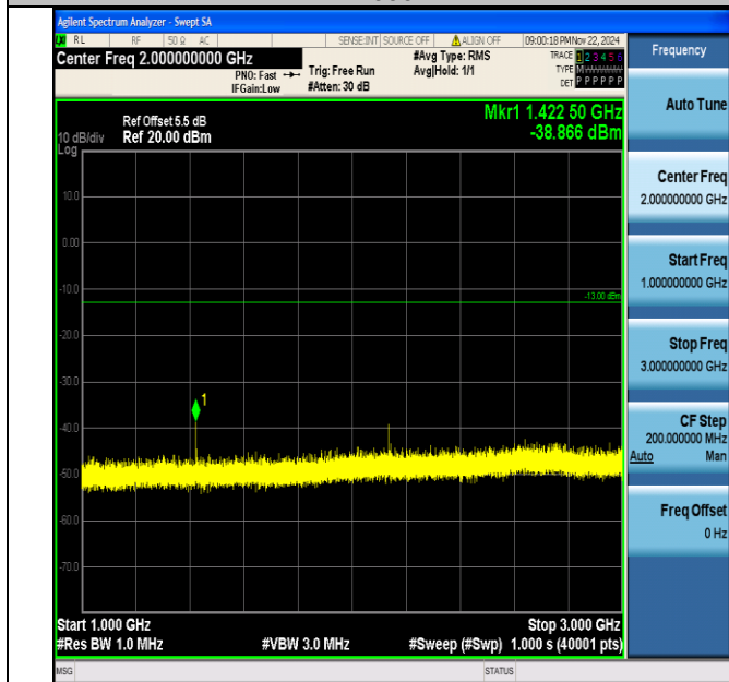
Band12_5MHz_64QAM_23155_1RB#0_1000~3000_1000~3000
