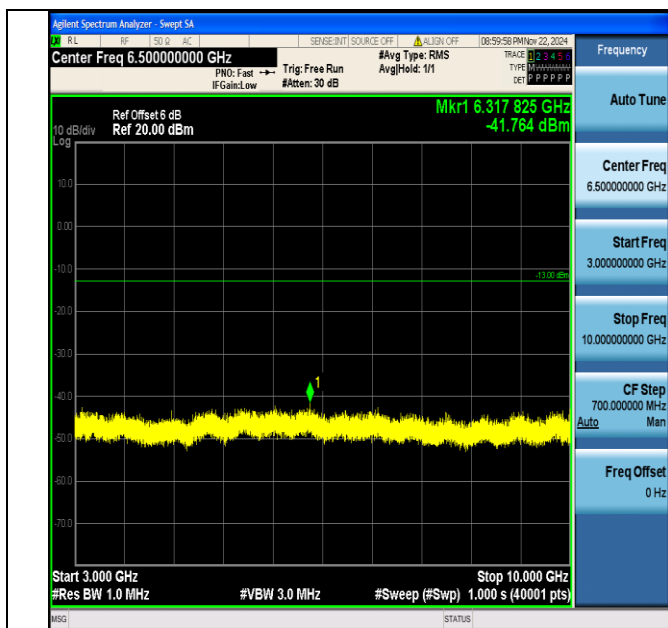
Band12_5MHz_64QAM_23095_1RB#0_3000~10000_3000~10000
