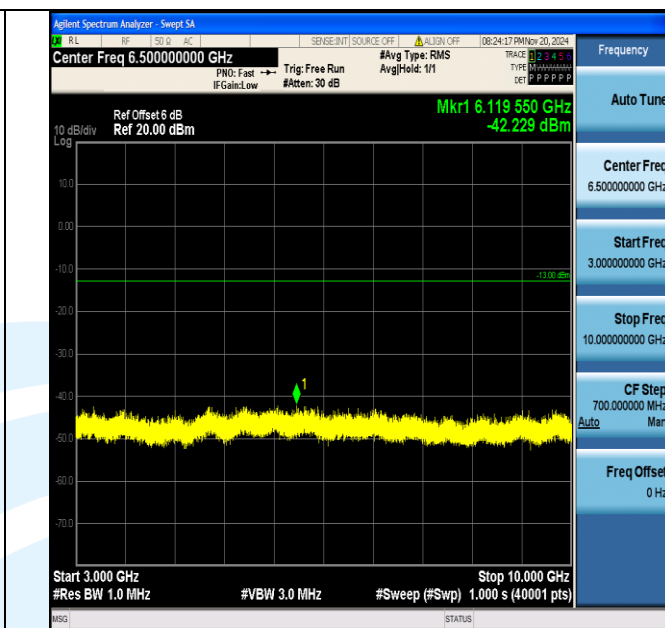
Band12_5MHz_16QAM_23095_1RB#0_3000~10000_3000~10000
