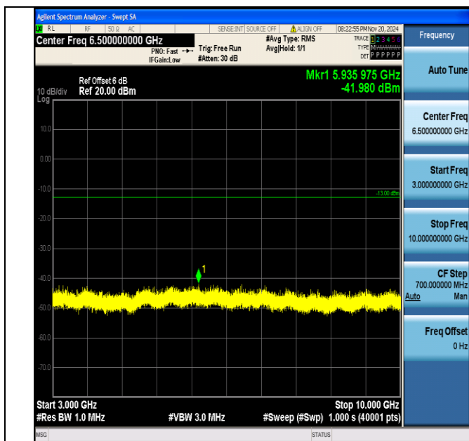
Band12_5MHz_QPSK_23035_1RB#0_3000~10000_3000~10000
