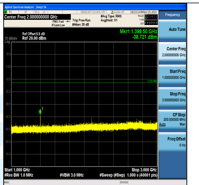
Band12_5MHz_16QAM_23035_1RB#0_1000~3000_1000~3000
