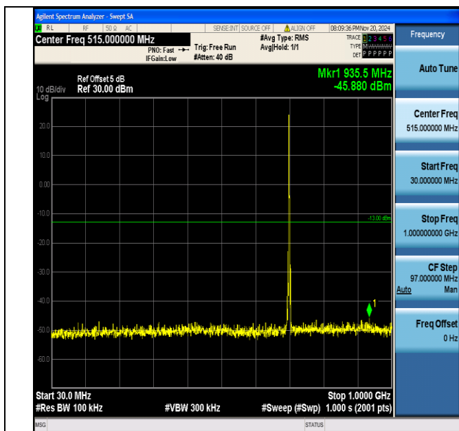
Band12_3MHz_16QAM_23095_1RB#0_30~1000_30~1000
