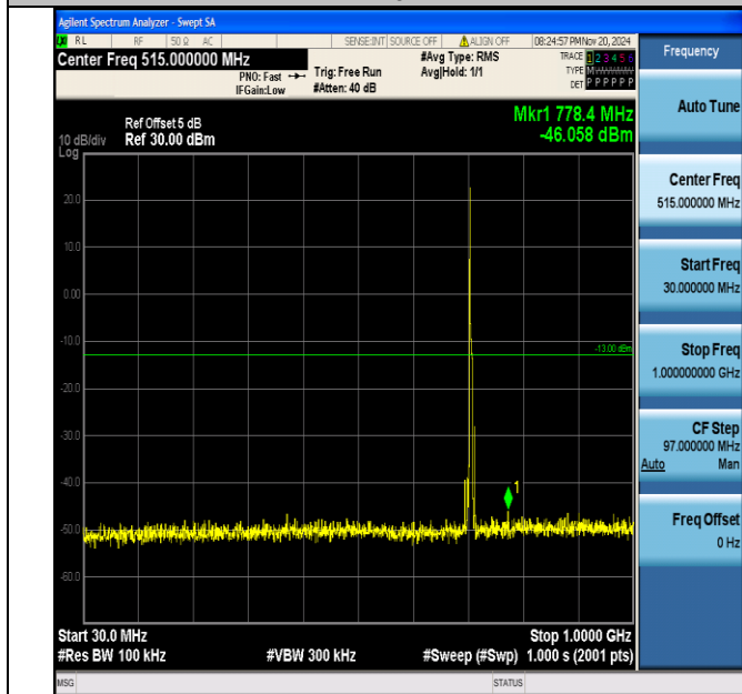
Band12_5MHz_16QAM_23155_1RB#0_30~1000_30~1000
