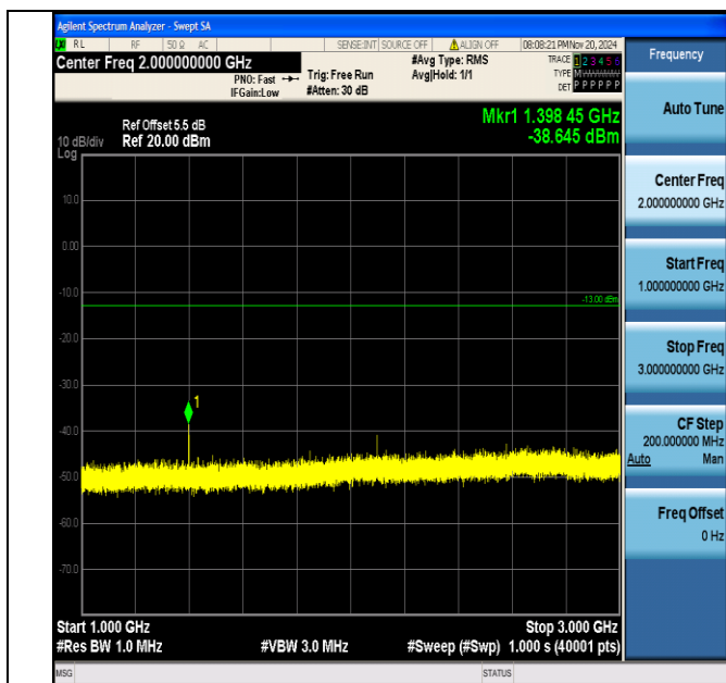
Band12_3MHz_QPSK_23025_1RB#0_1000~3000_1000~3000
