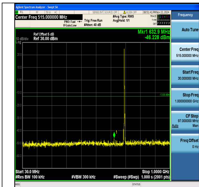
Band12_3MHz_64QAM_23025_1RB#0_30~1000_30~1000
