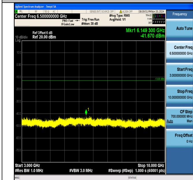
Band12_3MHz_16QAM_23095_1RB#0_3000~10000_3000~10000
