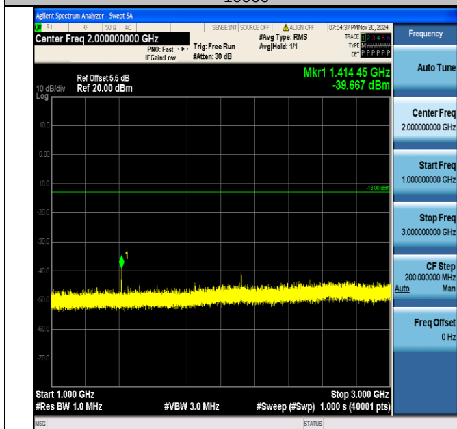
Band12_1.4MHz_16QAM_23095_1RB#0_1000~3000_1000~3000
