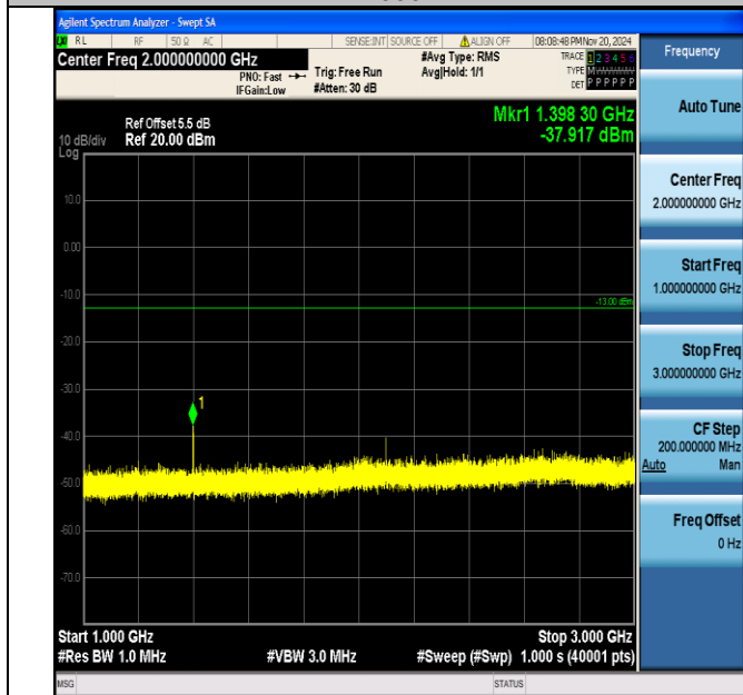
Band12_3MHz_16QAM_23025_1RB#0_1000~3000_1000~3000
