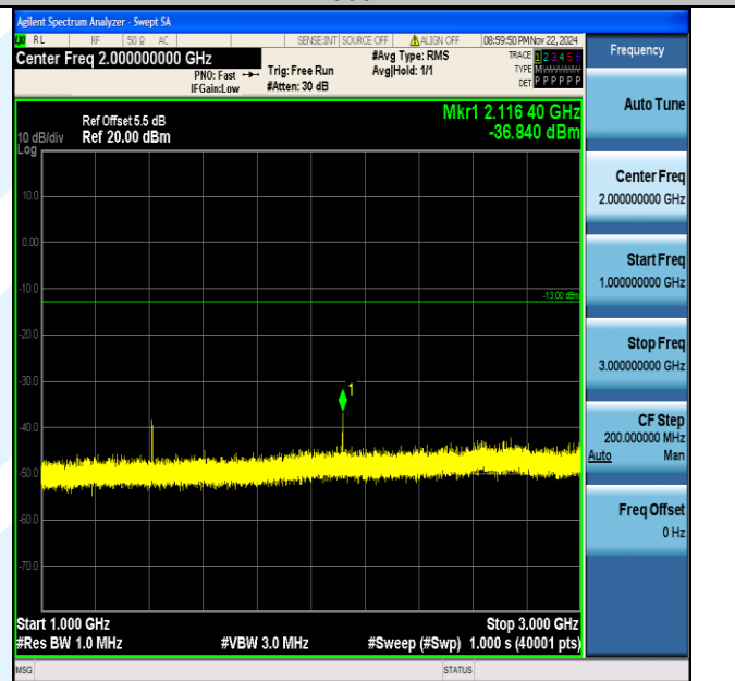
Band12_5MHz_64QAM_23095_1RB#0_1000~3000_1000~3000
