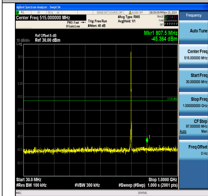
Band12_3MHz_QPSK_23095_1RB#0_30~1000_30~1000
