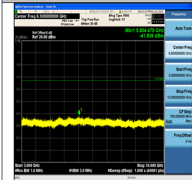
Band12_5MHz_16QAM_23035_1RB#0_3000~10000_3000~10000
