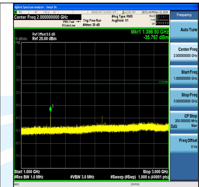
Band12_3MHz_64QAM_23025_1RB#0_1000~3000_1000~3000
