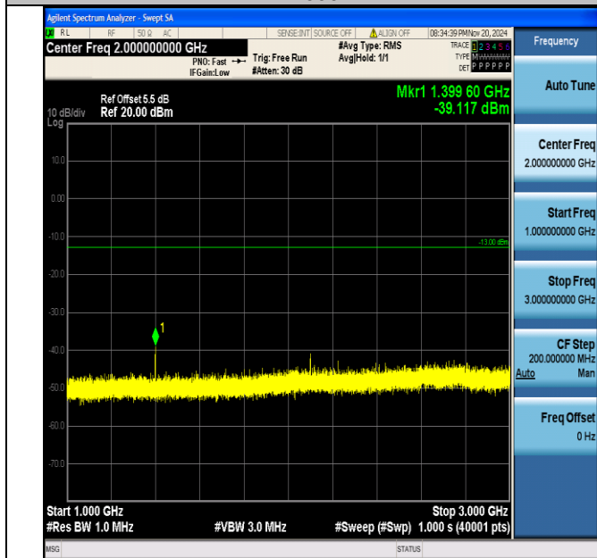
Band12_10MHz_QPSK_23060_1RB#0_1000~3000_1000~3000
