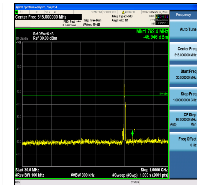
Band12_10MHz_64QAM_23130_1RB#0_30~1000_30~1000
