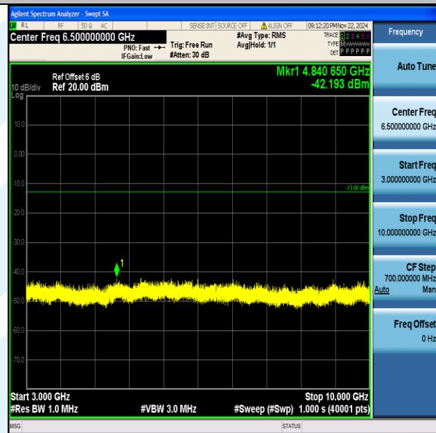
Band13_5MHz_64QAM_23205_1RB#0_3000~10000_3000~10000
