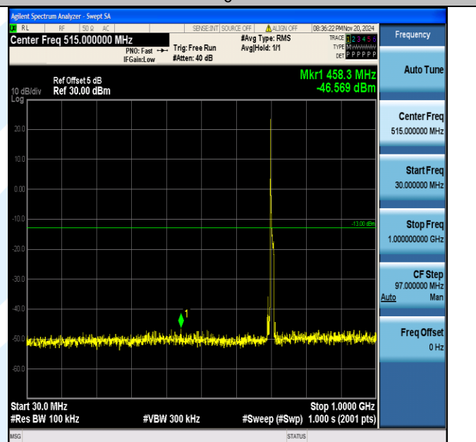
Band12_10MHz_QPSK_23130_1RB#0_30~1000_30~1000
