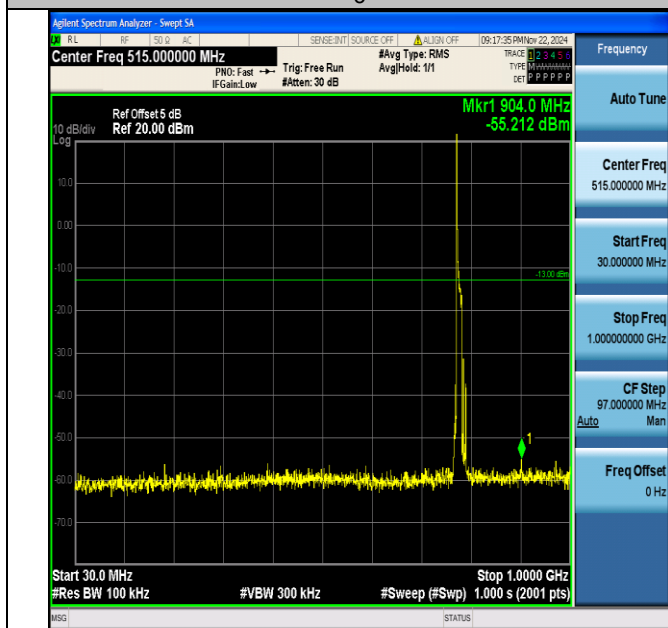
Band13_10MHz_64QAM_23230_1RB#0_30~1000_30~1000
