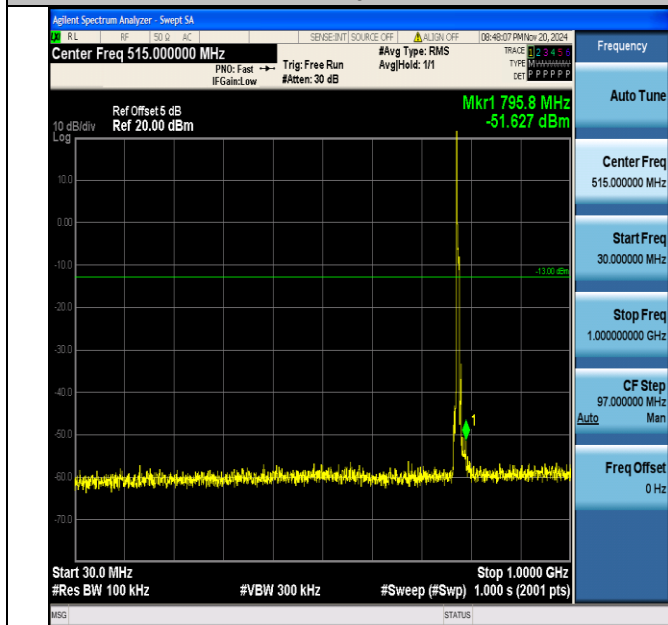
Band13_5MHz_16QAM_23205_1RB#0_30~1000_30~1000
