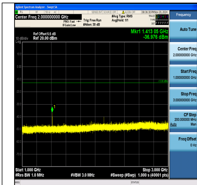
Band12_10MHz_QPSK_23130_1RB#0_1000~3000_1000~3000
