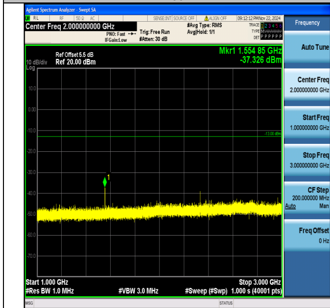
Band13_5MHz_64QAM_23205_1RB#0_1000~3000_1000~3000
