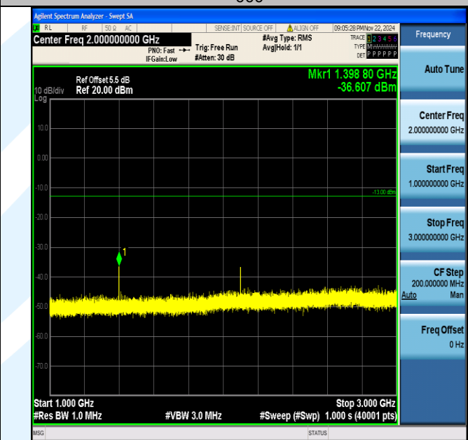
Band12_10MHz_64QAM_23060_1RB#0_1000~3000_1000~3000
