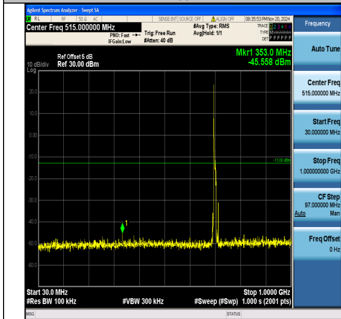
Band12_10MHz_16QAM_23095_1RB#0_30~1000_30~1000
