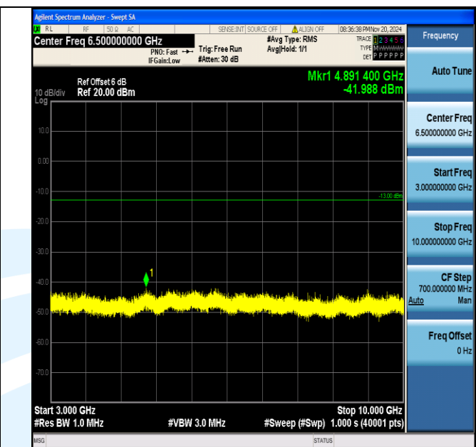
Band12_10MHz_QPSK_23130_1RB#0_3000~10000_3000~10000
