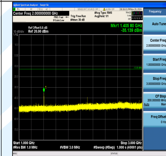
Band12_10MHz_16QAM_23095_1RB#0_1000~3000_1000~3000
