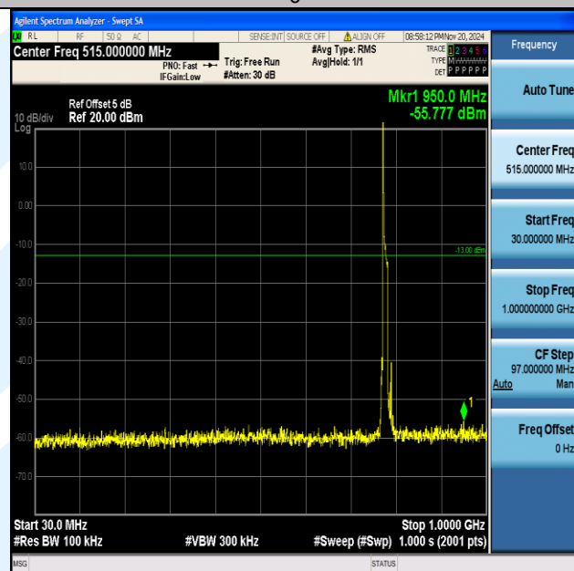
Band13_10MHz_QPSK_23230_1RB#0_30~1000_30~1000
