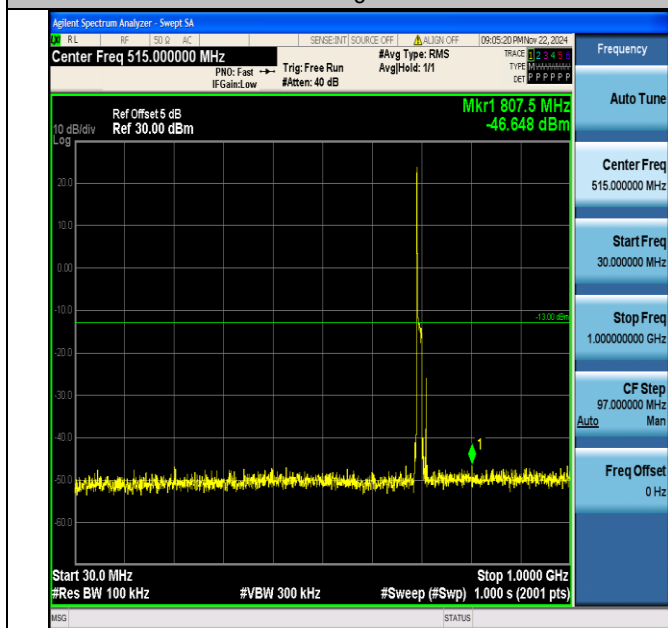
Band12_10MHz_64QAM_23060_1RB#0_30~1000_30~1000
