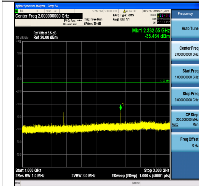
Band13_10MHz_16QAM_23230_1RB#0_1000~3000_1000~3000
