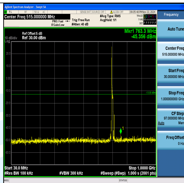
Band12_10MHz_64QAM_23095_1RB#0_30~1000_30~1000
