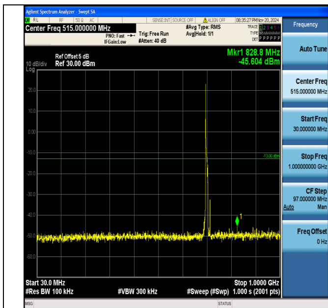
Band12_10MHz_QPSK_23095_1RB#0_30~1000_30~1000
