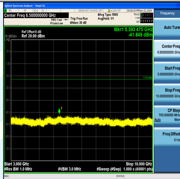
Band12_10MHz_64QAM_23095_1RB#0_3000~10000_3000~10000
