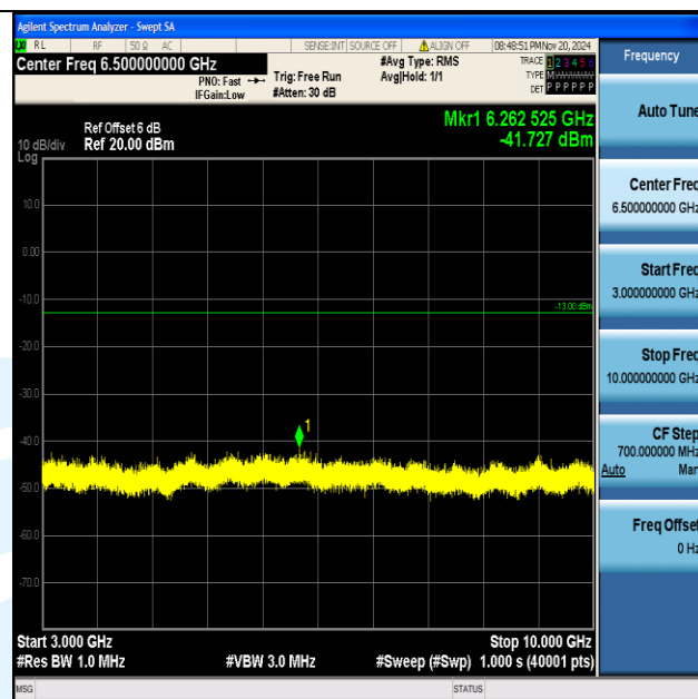
Band13_5MHz_QPSK_23230_1RB#0_3000~10000_3000~10000
