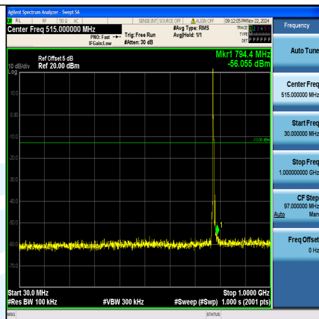
Band13_5MHz_64QAM_23205_1RB#0_30~1000_30~1000
