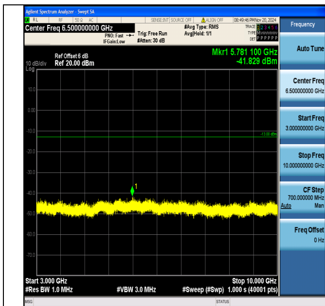
Band13_5MHz_QPSK_23255_1RB#0_3000~10000_3000~10000
