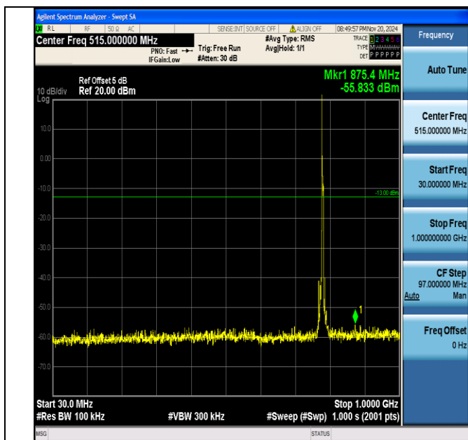
Band13_5MHz_16QAM_23255_1RB#0_30~1000_30~1000
