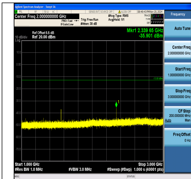
Band13_5MHz_QPSK_23230_1RB#0_1000~3000_1000~3000
