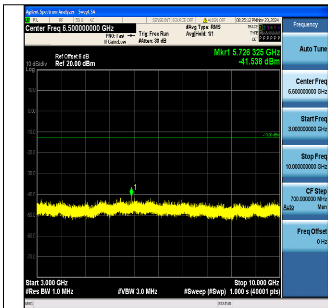
Band12_5MHz_16QAM_23155_1RB#0_3000~10000_3000~10000
