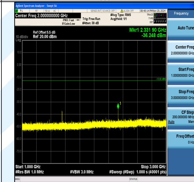
Band13_5MHz_16QAM_23205_1RB#0_1000~3000_1000~3000
