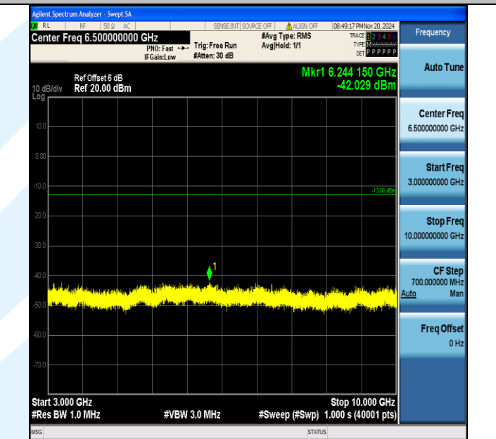
Band13_5MHz_16QAM_23230_1RB#0_3000~10000_3000~10000
