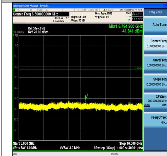
Band12_10MHz_64QAM_23130_1RB#0_3000~10000_3000~10000
