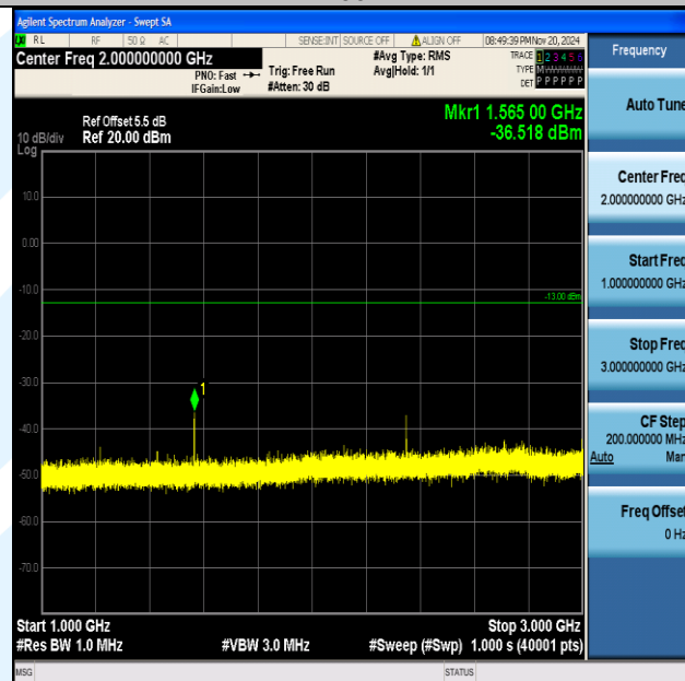
Band13_5MHz_QPSK_23255_1RB#0_1000~3000_1000~3000
