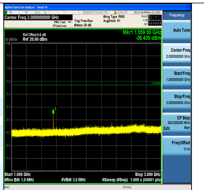
Band13_5MHz_64QAM_23230_1RB#0_1000~3000_1000~3000
