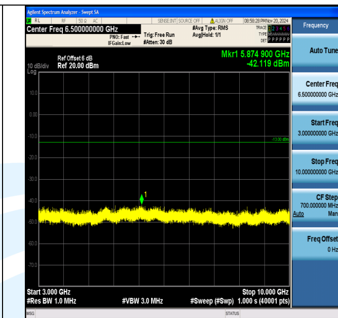
Band13_10MHz_QPSK_23230_1RB#0_3000~10000_3000~10000
