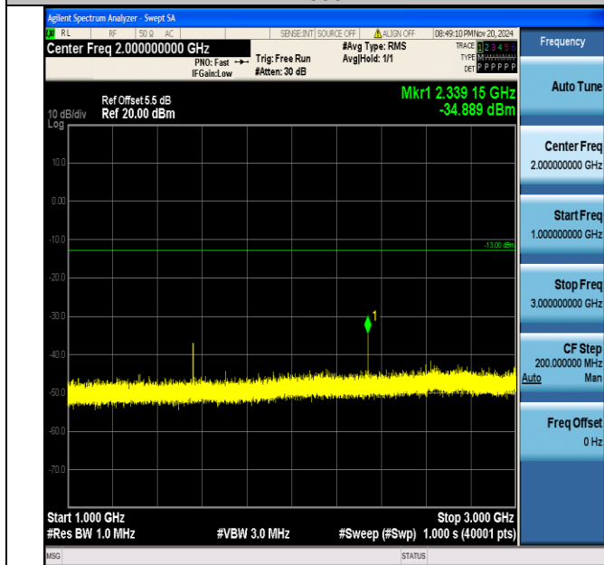
Band13_5MHz_16QAM_23230_1RB#0_1000~3000_1000~3000
