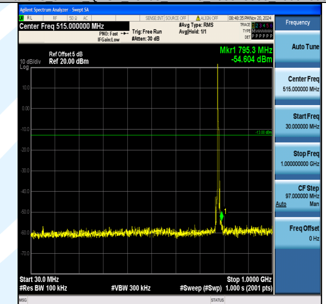
Band13_5MHz_QPSK_23230_1RB#0_30~1000_30~1000
