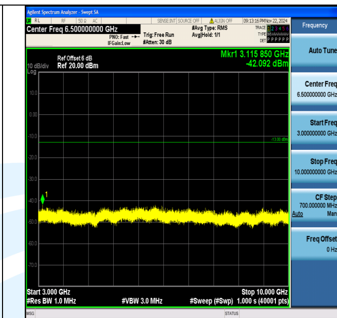
Band13_5MHz_64QAM_23255_1RB#0_3000~10000_3000~10000
