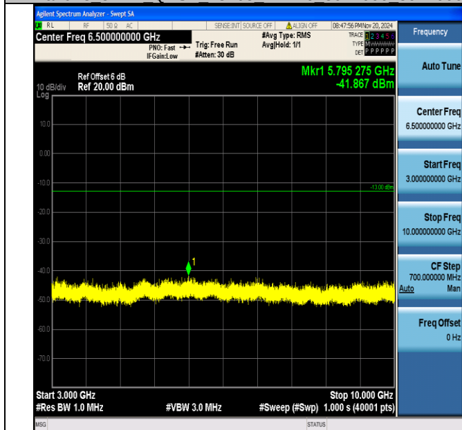
Band13_5MHz_QPSK_23205_1RB#0_3000~10000_3000~10000
