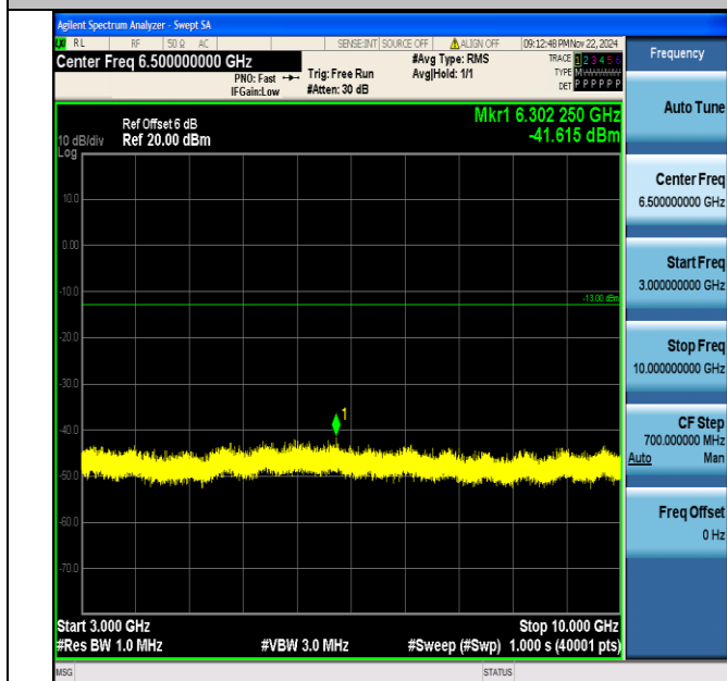
Band13_5MHz_64QAM_23230_1RB#0_3000~10000_3000~10000
