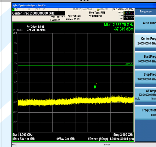
Band13_10MHz_64QAM_23230_1RB#0_1000~3000_1000~3000
