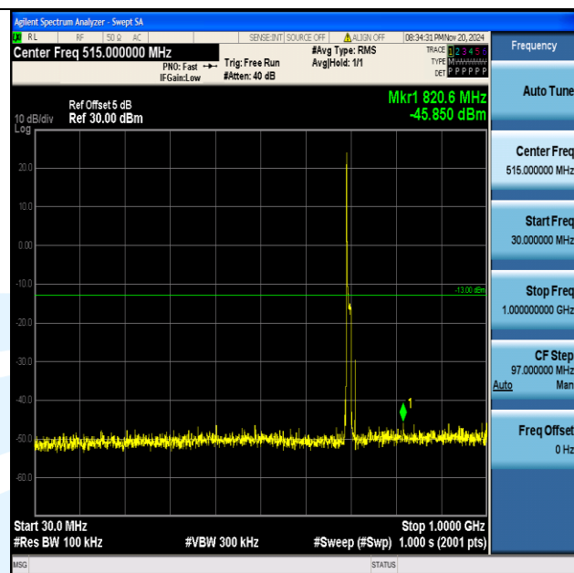
Band12_10MHz_QPSK_23060_1RB#0_30~1000_30~1000
