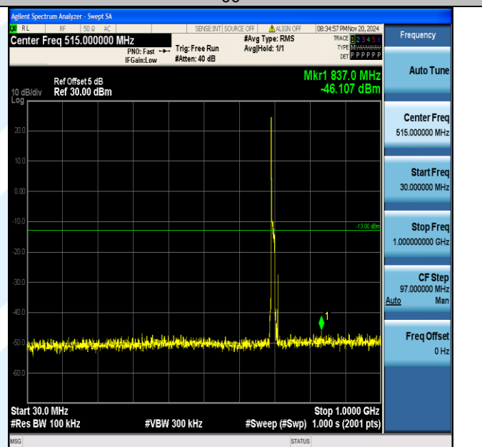
Band12_10MHz_16QAM_23060_1RB#0_30~1000_30~1000
