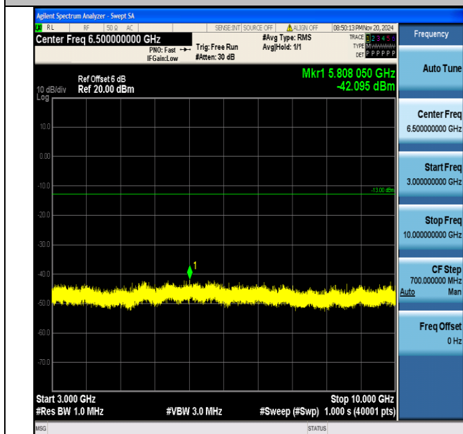
Band13_5MHz_16QAM_23255_1RB#0_3000~10000_3000~10000
