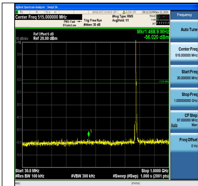
Band13_5MHz_64QAM_23230_1RB#0_30~1000_30~1000
