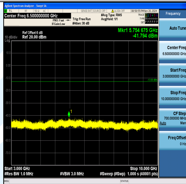
Band13_10MHz_16QAM_23230_1RB#0_3000~10000_3000~10000
