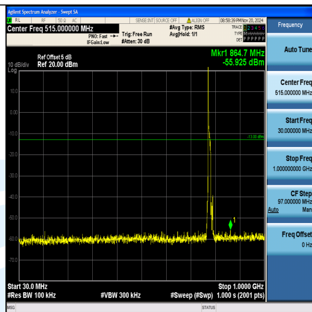
Band13_10MHz_16QAM_23230_1RB#0_30~1000_30~1000
