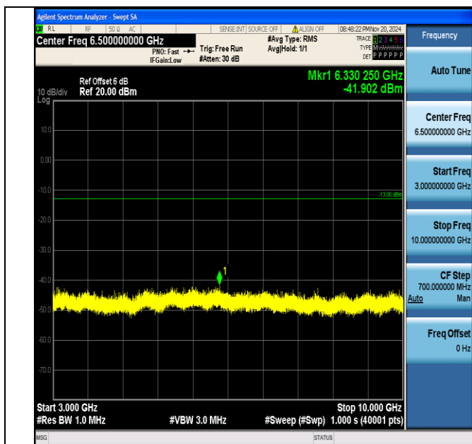
Band13_5MHz_16QAM_23205_1RB#0_3000~10000_3000~10000
