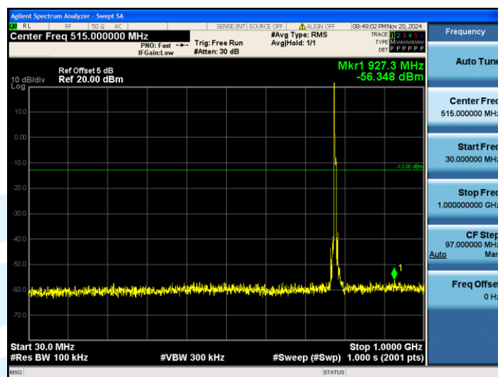
Band13_5MHz_16QAM_23230_1RB#0_30~1000_30~1000
