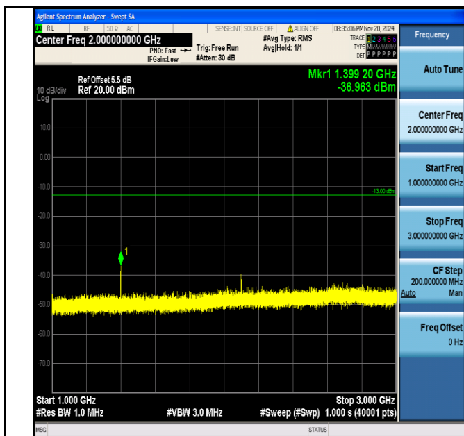
Band12_10MHz_16QAM_23060_1RB#0_1000~3000_1000~3000
