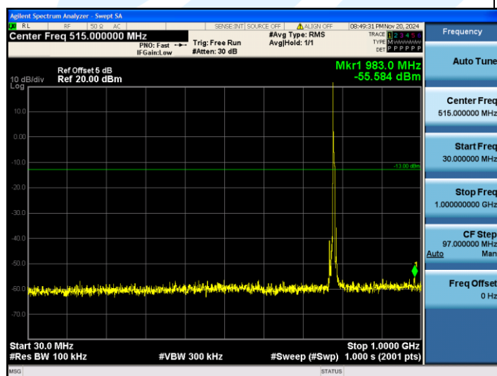
Band13_5MHz_QPSK_23255_1RB#0_30~1000_30~1000
