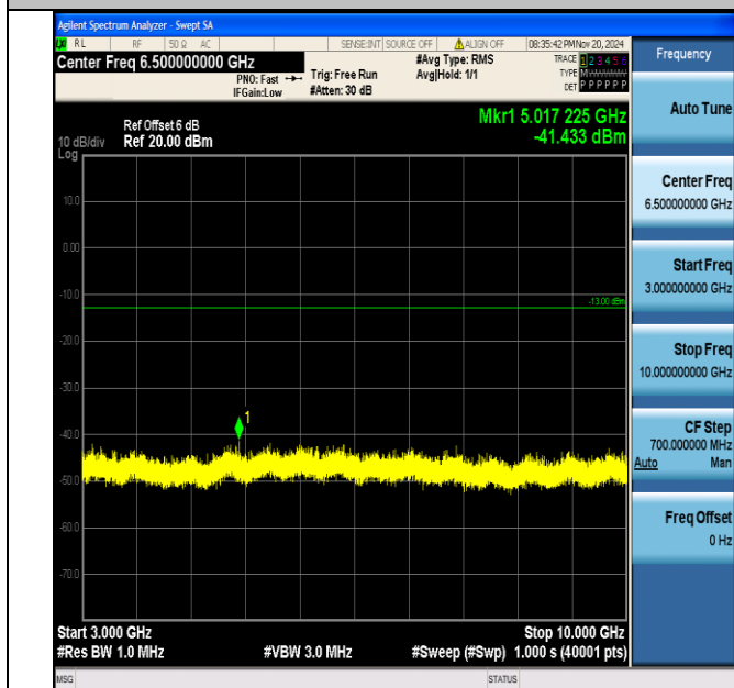
Band12_10MHz_QPSK_23095_1RB#0_3000~10000_3000~10000
