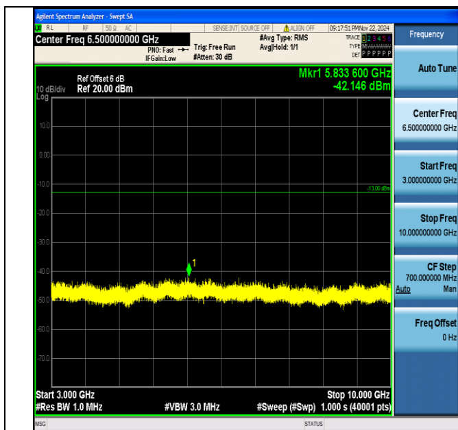
Band13_10MHz_64QAM_23230_1RB#0_3000~10000_3000~10000
