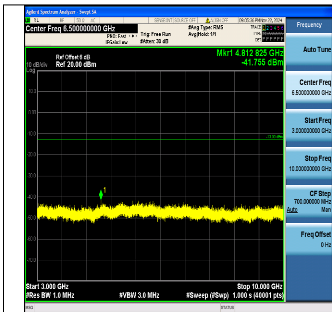
Band12_10MHz_64QAM_23060_1RB#0_3000~10000_3000~10000
