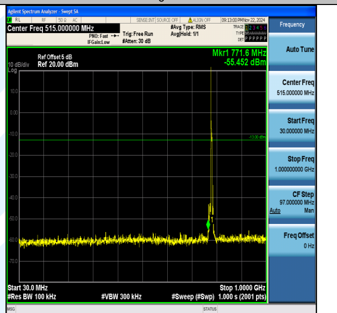
Band13_5MHz_64QAM_23255_1RB#0_30~1000_30~1000
