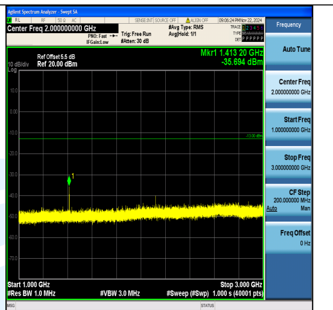
Band12_10MHz_64QAM_23130_1RB#0_1000~3000_1000~3000
