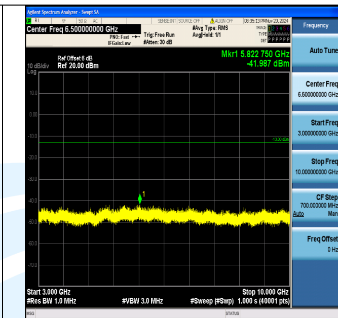
Band12_10MHz_16QAM_23060_1RB#0_3000~10000_3000~10000
