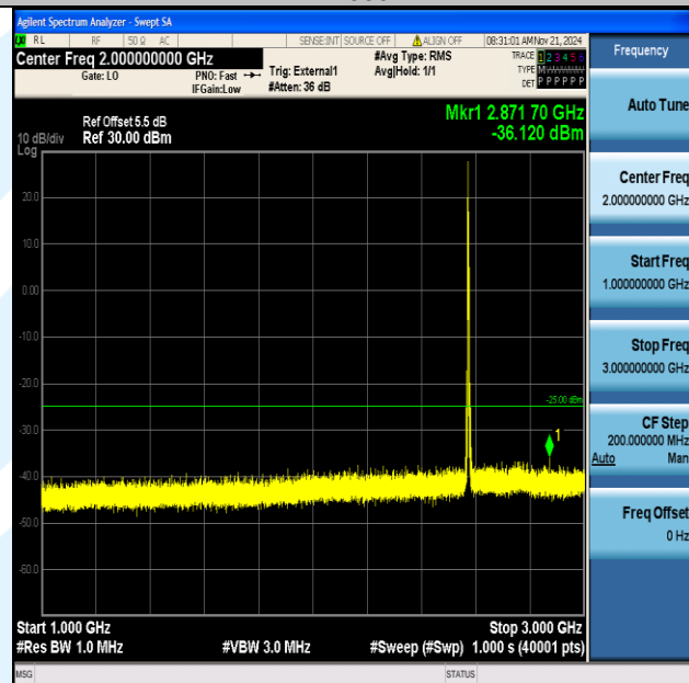
Band38_5MHz_16QAM_37775_1RB#0_1000~3000_1000~3000
