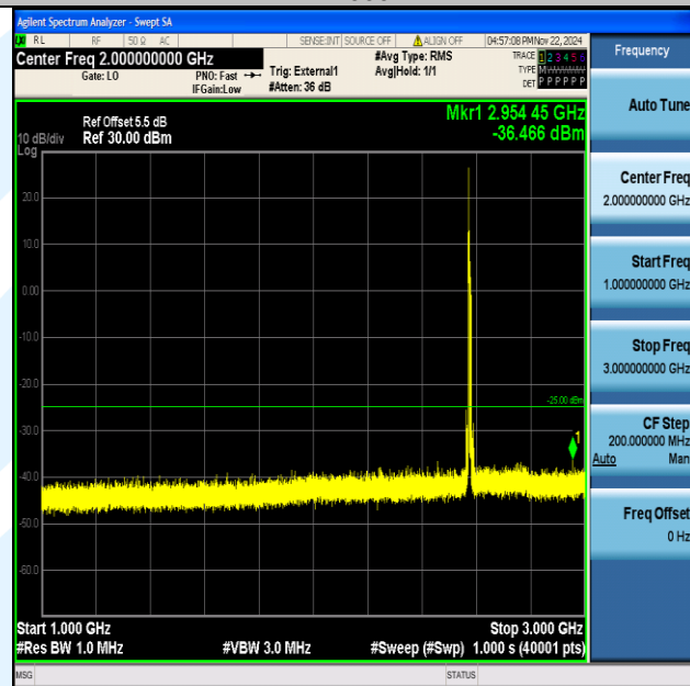
Band38_10MHz_64QAM_37800_1RB#0_1000~3000_1000~3000
