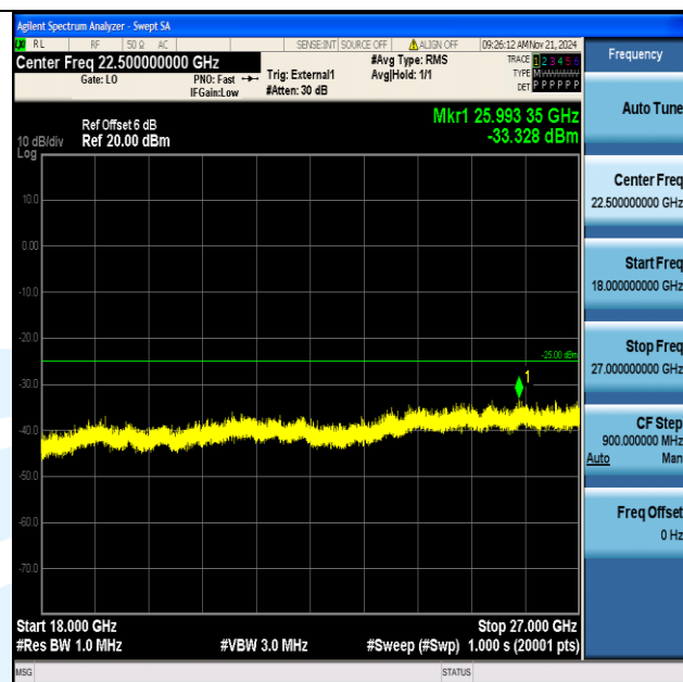
Band38_10MHz_QPSK_38200_1RB#0_18000~27000_18000~27000
