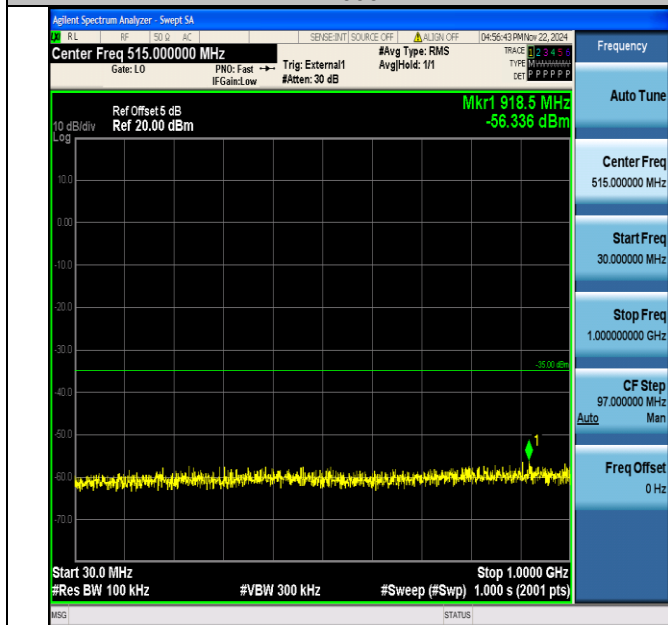
Band38_10MHz_64QAM_37800_1RB#0_30~1000_30~1000
