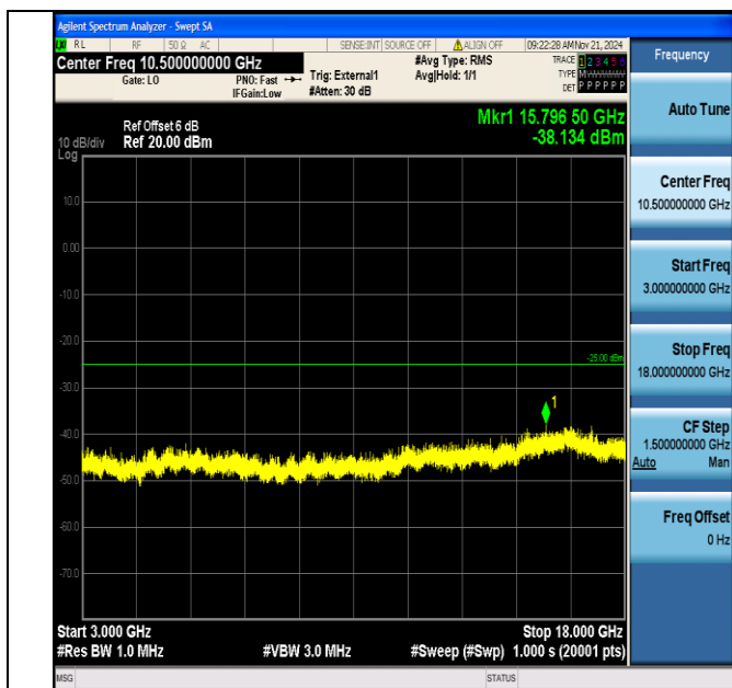
Band38_10MHz_QPSK_38000_1RB#0_3000~18000_3000~18000
