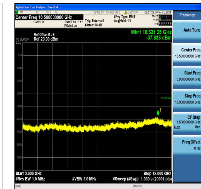
Band38_10MHz_16QAM_38200_1RB#0_3000~18000_3000~18000
