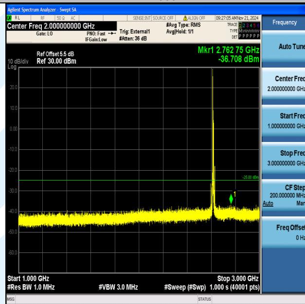
Band38_10MHz_16QAM_38200_1RB#0_1000~3000_1000~3000
