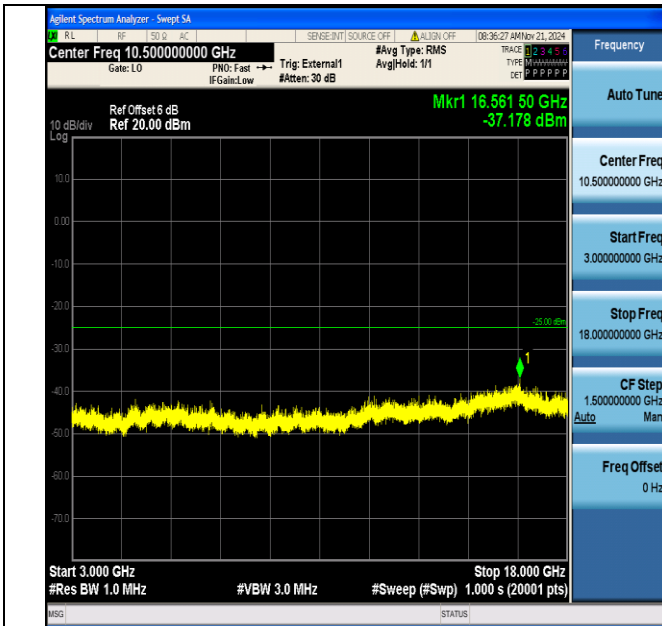
Band38_5MHz_QPSK_38225_1RB#0_3000~18000_3000~18000
