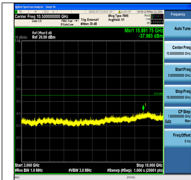
Band38_10MHz_64QAM_38000_1RB#0_3000~18000_3000~18000
