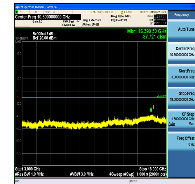
Band38_10MHz_64QAM_38200_1RB#0_3000~18000_3000~18000
