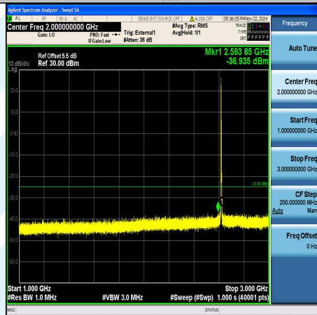
Band38_5MHz_64QAM_38225_1RB#0_1000~3000_1000~3000
