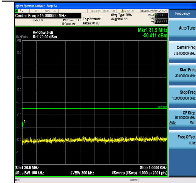
Band38_5MHz_64QAM_38000_1RB#0_30~1000_30~1000
