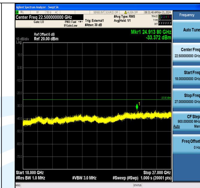
Band38_5MHz_16QAM_37775_1RB#0_18000~27000_18000~27000
