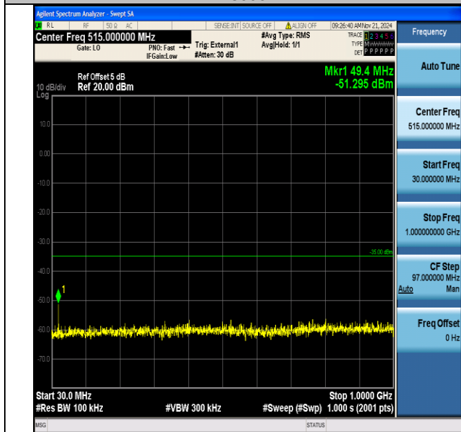
Band38_10MHz_16QAM_38200_1RB#0_30~1000_30~1000
