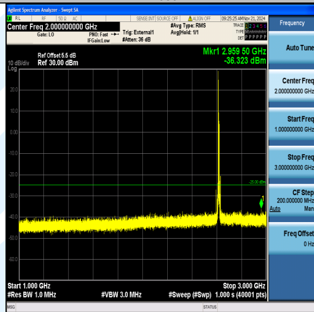
Band38_10MHz_QPSK_38200_1RB#0_1000~3000_1000~3000
