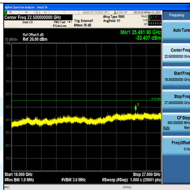
Band38_10MHz_QPSK_37800_1RB#0_18000~27000_18000~27000
