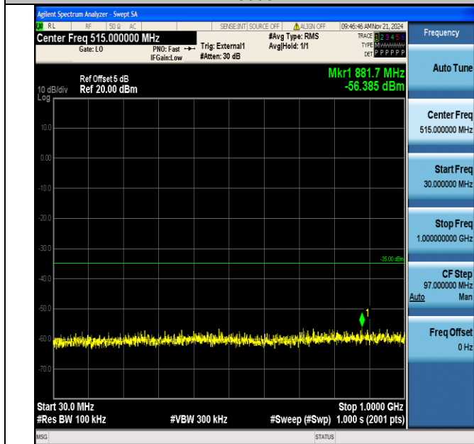
Band38_15MHz_QPSK_37825_1RB#0_30~1000_30~1000
