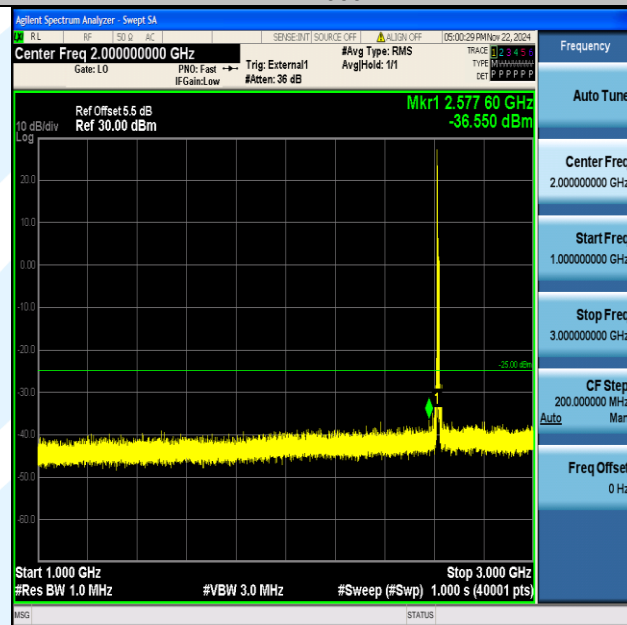
Band38_10MHz_64QAM_38200_1RB#0_1000~3000_1000~3000
