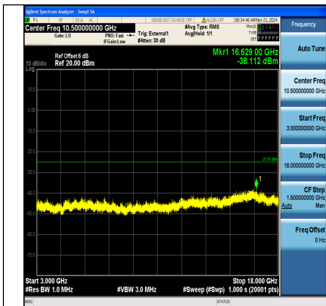
Band38_5MHz_16QAM_38000_1RB#0_3000~18000_3000~18000
