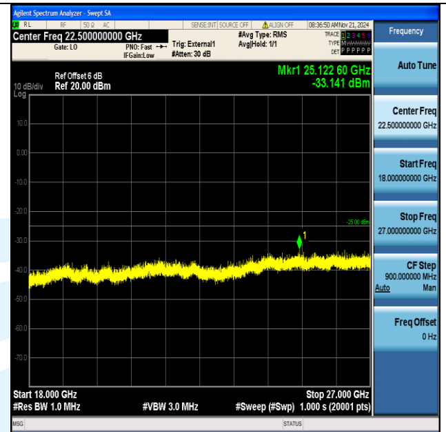
Band38_5MHz_QPSK_38225_1RB#0_18000~27000_18000~27000
