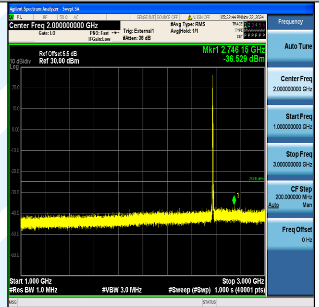
Band38_5MHz_64QAM_37775_1RB#0_1000~3000_1000~3000
