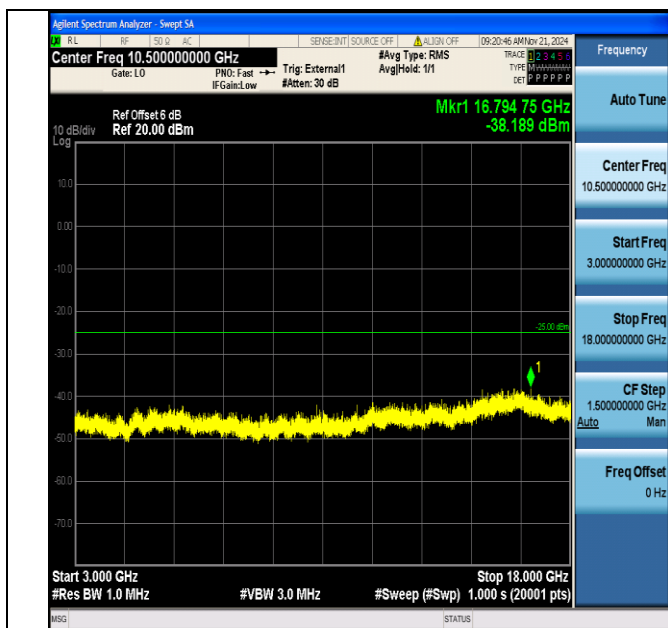
Band38_10MHz_16QAM_37800_1RB#0_3000~18000_3000~18000
