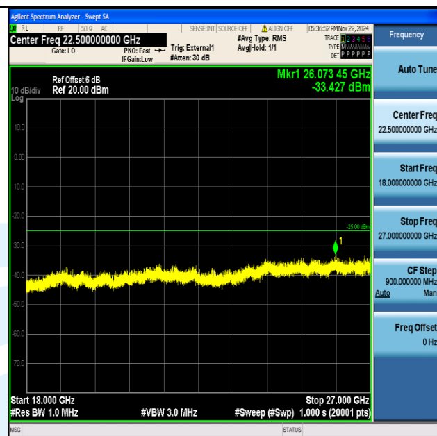
Band38_5MHz_64QAM_38225_1RB#0_18000~27000_18000~27000
