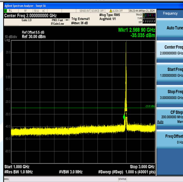
Band38_10MHz_16QAM_38000_1RB#0_1000~3000_1000~3000
