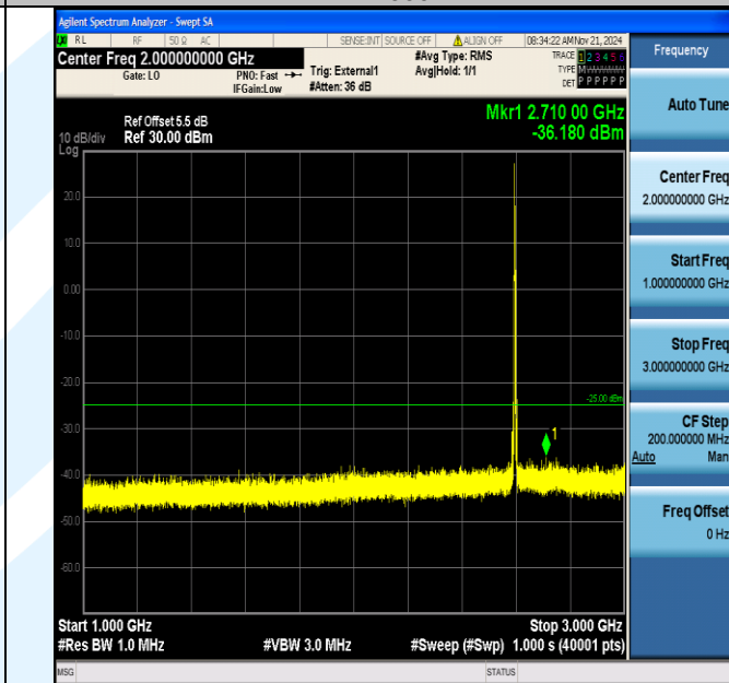
Band38_5MHz_16QAM_38000_1RB#0_1000~3000_1000~3000
