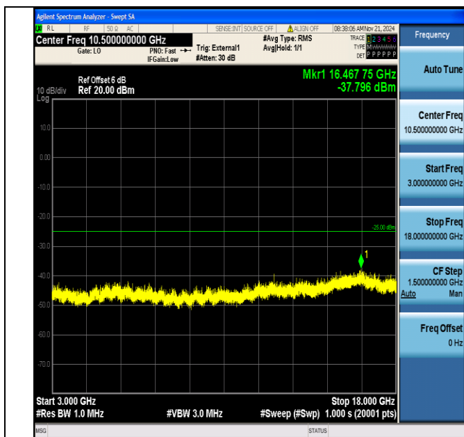
Band38_5MHz_16QAM_38225_1RB#0_3000~18000_3000~18000
