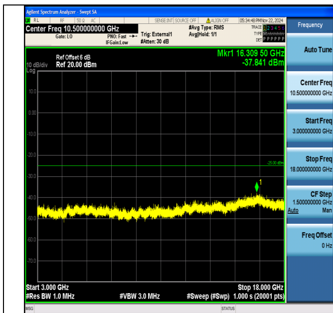
Band38_5MHz_64QAM_38000_1RB#0_3000~18000_3000~18000
