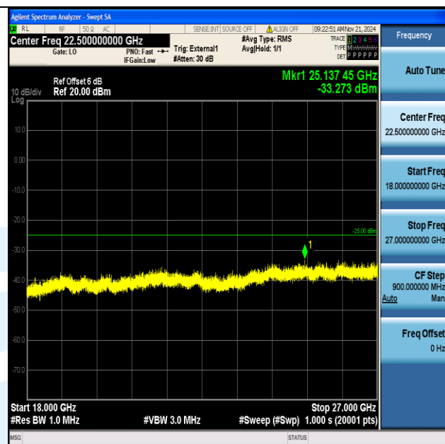
Band38_10MHz_QPSK_38000_1RB#0_18000~27000_18000~27000
