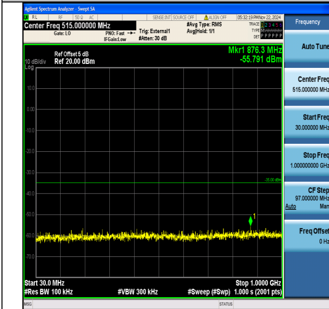
Band38_5MHz_64QAM_37775_1RB#0_30~1000_30~1000
