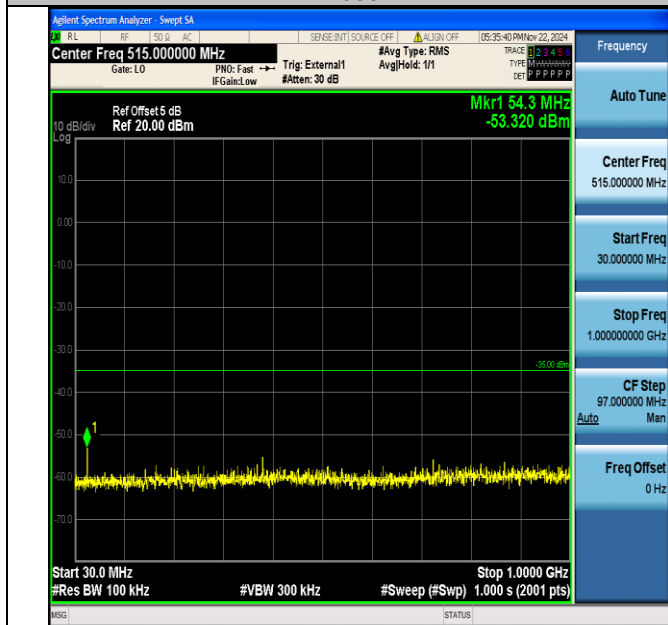
Band38_5MHz_64QAM_38225_1RB#0_30~1000_30~1000
