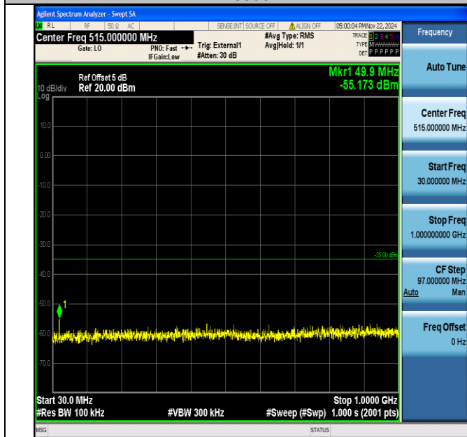
Band38_10MHz_64QAM_38200_1RB#0_30~1000_30~1000
