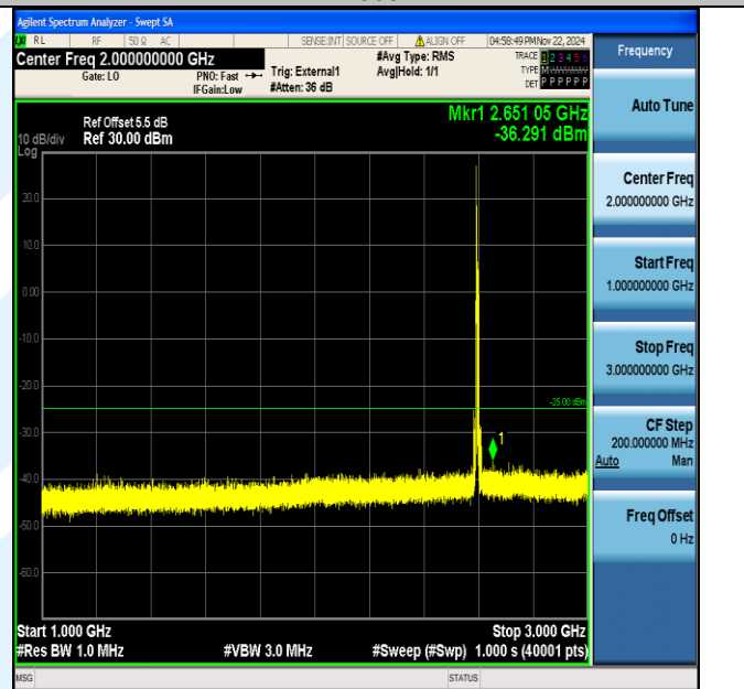
Band38_10MHz_64QAM_38000_1RB#0_1000~3000_1000~3000
