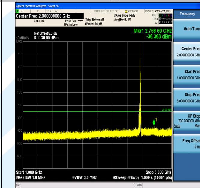
Band38_10MHz_16QAM_37800_1RB#0_1000~3000_1000~3000
