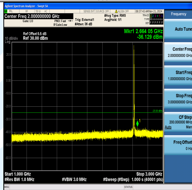
Band38_5MHz_16QAM_38225_1RB#0_1000~3000_1000~3000
