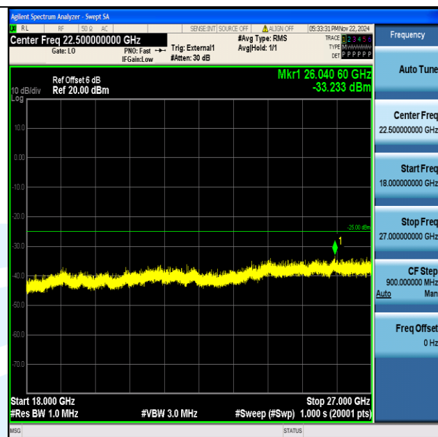
Band38_5MHz_64QAM_37775_1RB#0_18000~27000_18000~27000
