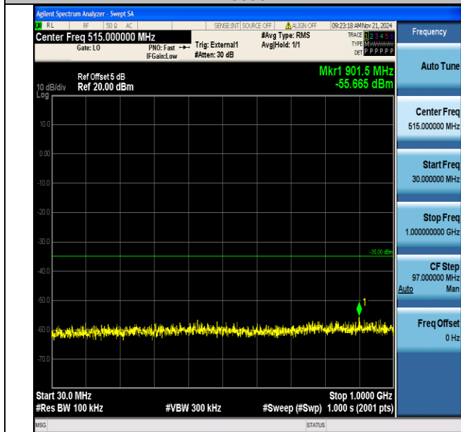
Band38_10MHz_16QAM_38000_1RB#0_30~1000_30~1000
