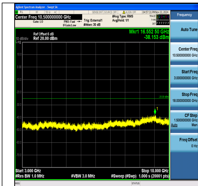
Band38_10MHz_64QAM_37800_1RB#0_3000~18000_3000~18000
