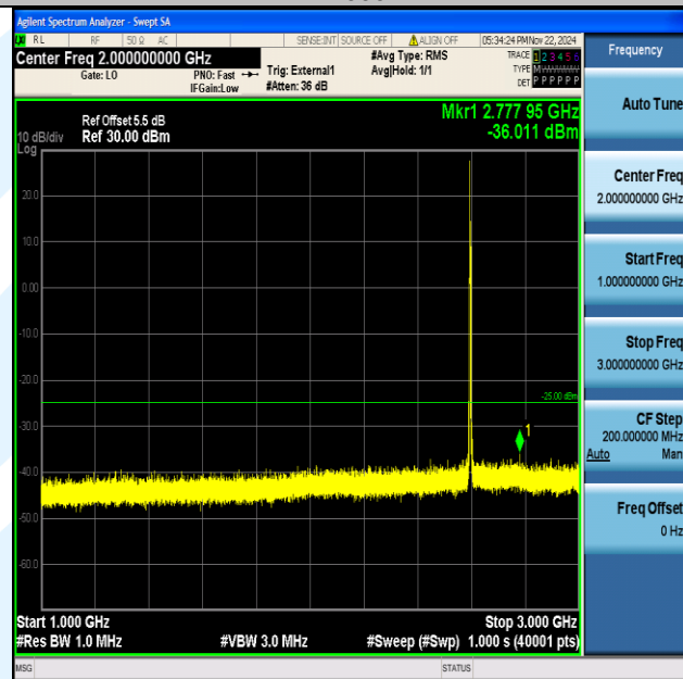
Band38_5MHz_64QAM_38000_1RB#0_1000~3000_1000~3000
