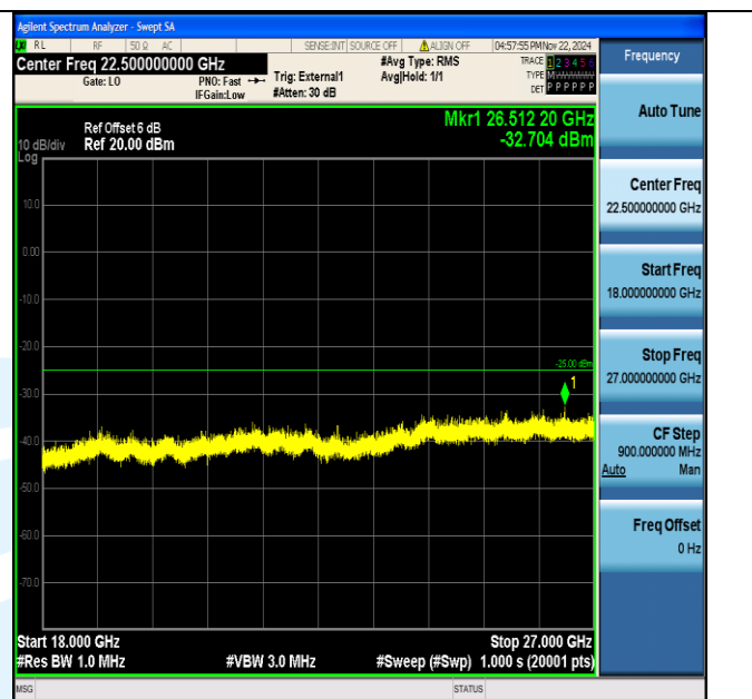
Band38_10MHz_64QAM_37800_1RB#0_18000~27000_18000~27000
