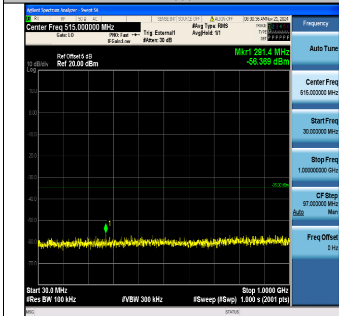
Band38_5MHz_16QAM_37775_1RB#0_30~1000_30~1000
