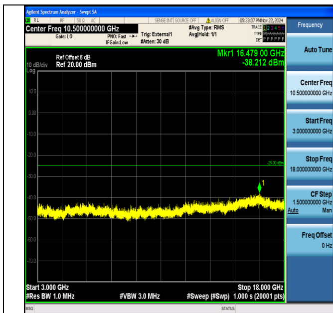
Band38_5MHz_64QAM_37775_1RB#0_3000~18000_3000~18000
