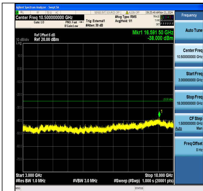
Band38_10MHz_QPSK_38200_1RB#0_3000~18000_3000~18000
