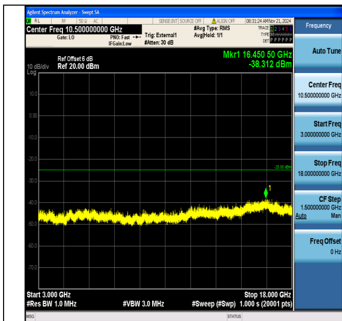
Band38_5MHz_16QAM_37775_1RB#0_3000~18000_3000~18000
