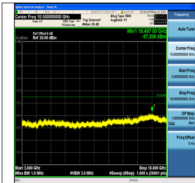
Band38_5MHz_64QAM_38225_1RB#0_3000~18000_3000~18000
