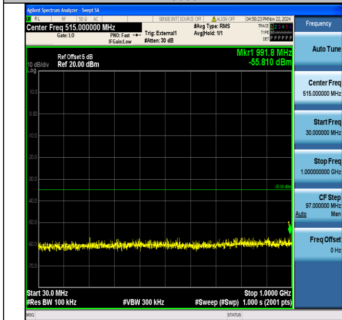
Band38_10MHz_64QAM_38000_1RB#0_30~1000_30~1000
