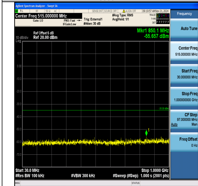
Band38_10MHz_16QAM_37800_1RB#0_30~1000_30~1000
