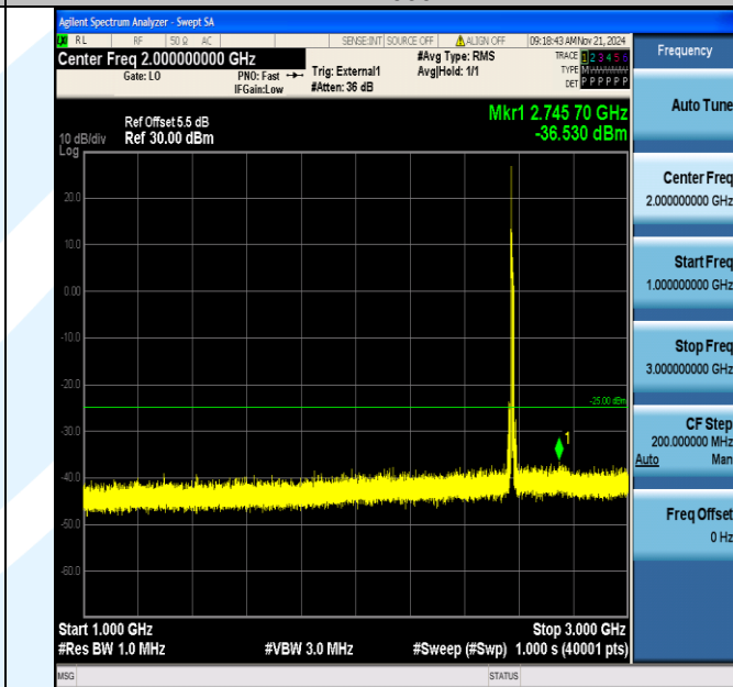
Band38_10MHz_QPSK_37800_1RB#0_1000~3000_1000~3000
