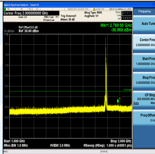
Band38_15MHz_QPSK_37825_1RB#0_1000~3000_1000~3000
