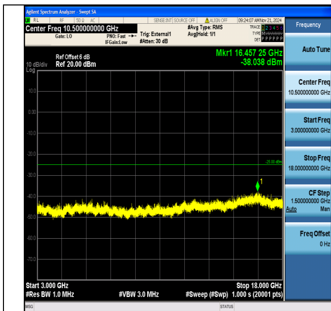
Band38_10MHz_16QAM_38000_1RB#0_3000~18000_3000~18000
