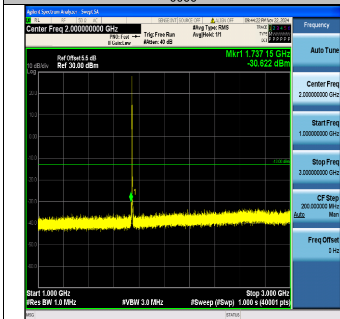
Band66_3MHz_64QAM_132322_1RB#0_1000~3000_1000~3000
