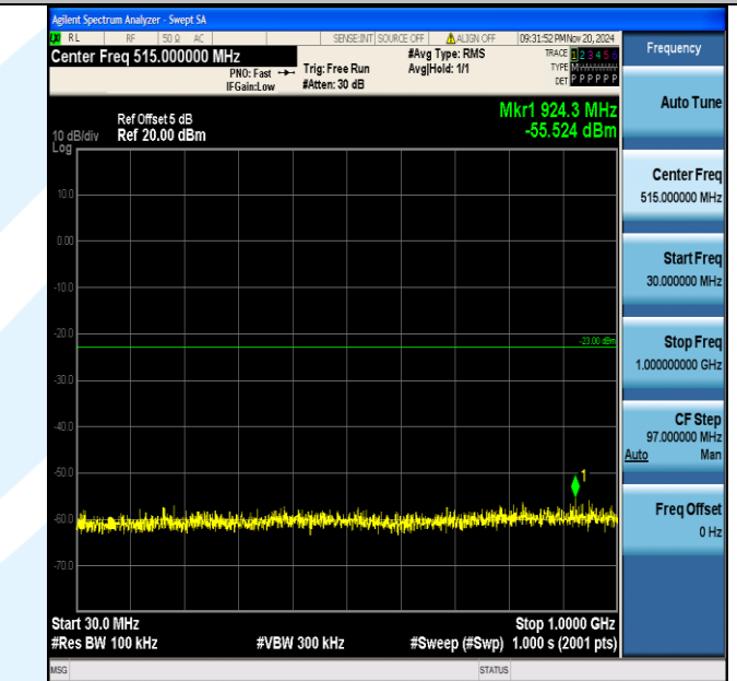
Band66_1.4MHz_16QAM_132322_1RB#0_30~1000_30~1000
