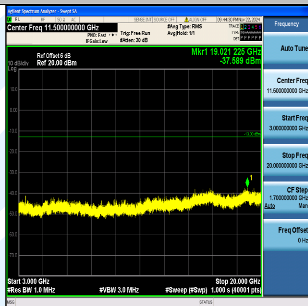
Band66_3MHz_64QAM_132322_1RB#0_3000~20000_3000~20000
