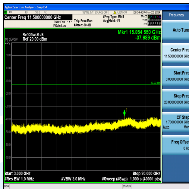
Band66_1.4MHz_64QAM_131979_1RB#0_3000~20000_3000~20000
