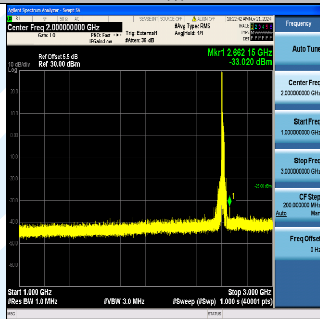
Band38_20MHz_16QAM_38150_1RB#0_1000~3000_1000~3000
