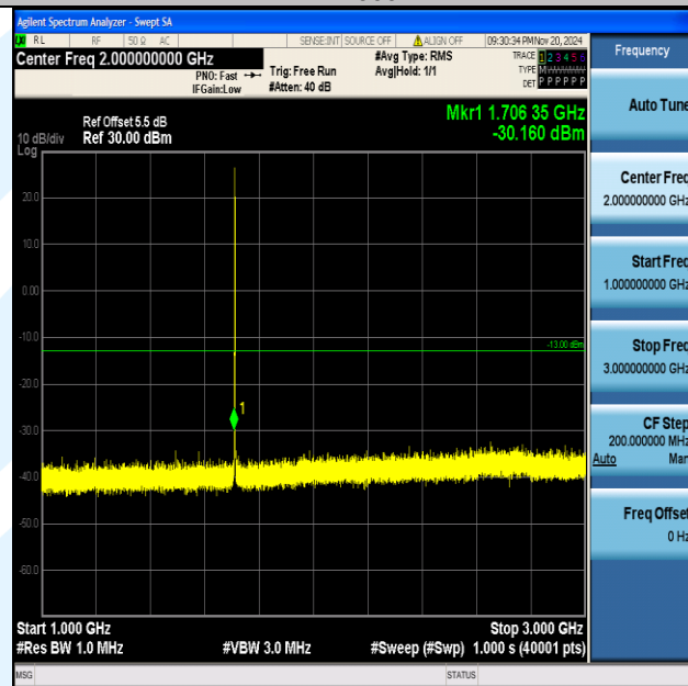
Band66_1.4MHz_QPSK_131979_1RB#0_1000~3000_1000~3000
