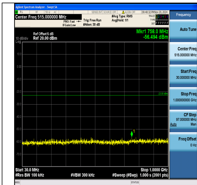
Band66_3MHz_QPSK_132322_1RB#0_30~1000_30~1000
