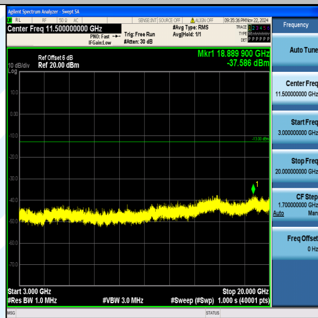
Band66_1.4MHz_64QAM_132665_1RB#0_3000~20000_3000~20000
