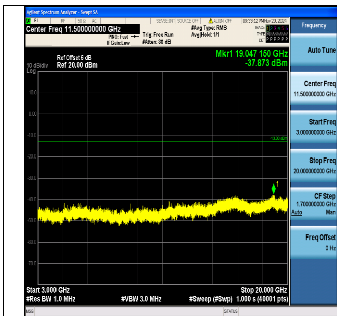
Band66_1.4MHz_16QAM_132665_1RB#0_3000~20000_3000~20000
