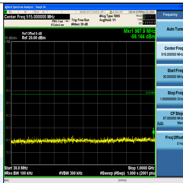
Band66_3MHz_64QAM_132322_1RB#0_30~1000_30~1000
