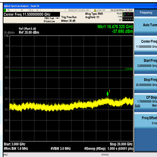
Band66_1.4MHz_16QAM_132322_1RB#0_3000~20000_3000~20000
