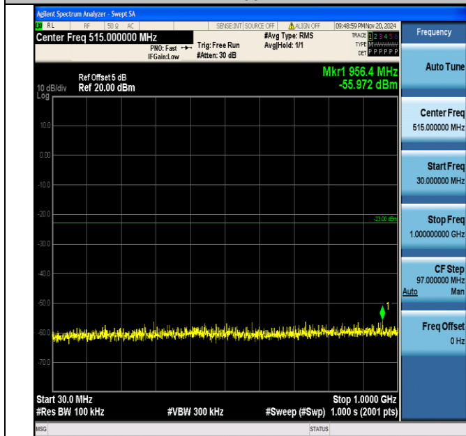
Band66_3MHz_16QAM_132322_1RB#0_30~1000_30~1000
