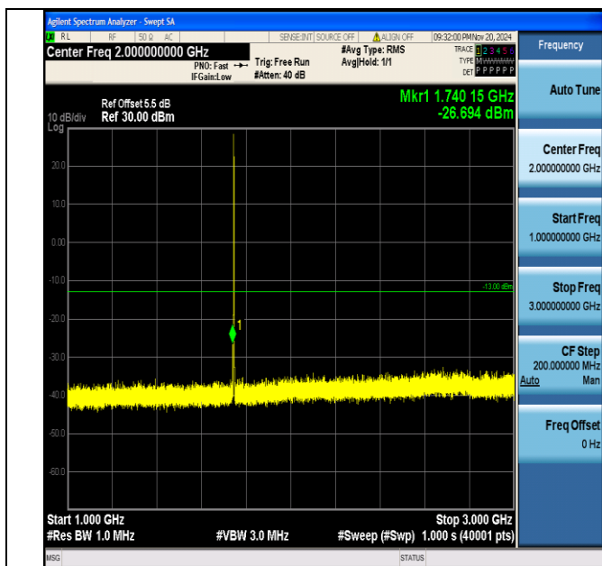
Band66_1.4MHz_16QAM_132322_1RB#0_1000~3000_1000~3000
