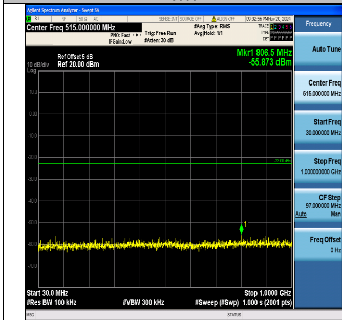
Band66_1.4MHz_16QAM_132665_1RB#0_30~1000_30~1000
