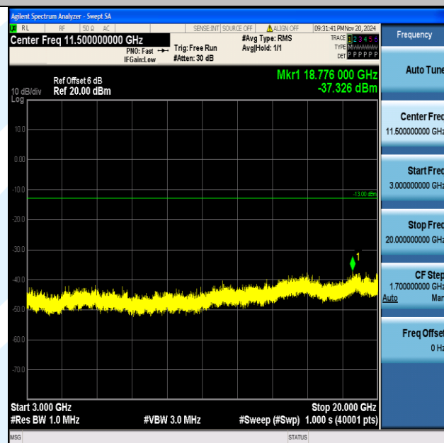
Band66_1.4MHz_QPSK_132322_1RB#0_3000~20000_3000~20000
