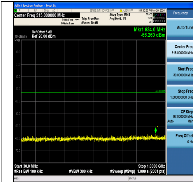
Band66_1.4MHz_16QAM_131979_1RB#0_30~1000_30~1000
