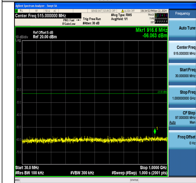
Band66_1.4MHz_64QAM_132322_1RB#0_30~1000_30~1000
