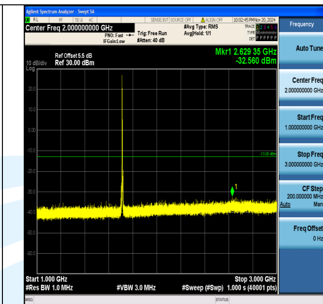
Band66_5MHz_QPSK_131997_1RB#0_1000~3000_1000~3000
