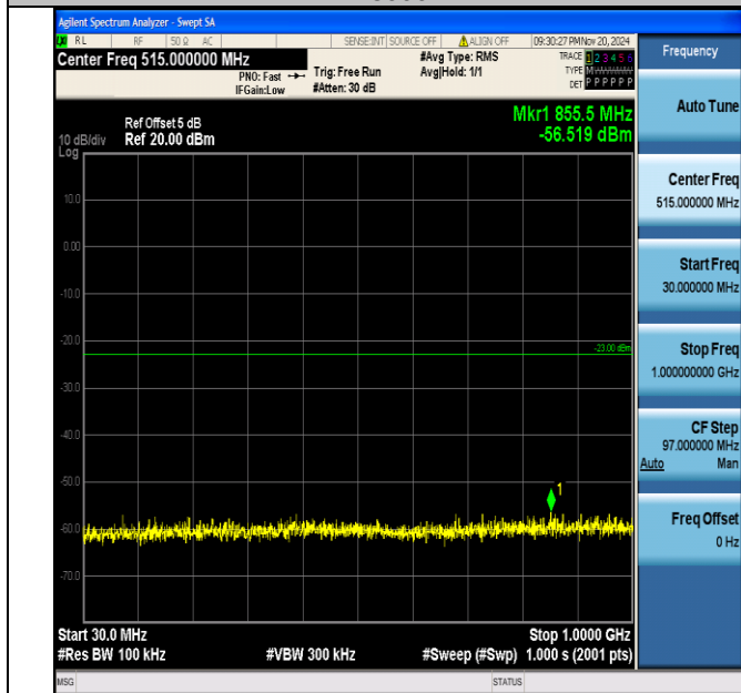
Band66_1.4MHz_QPSK_131979_1RB#0_30~1000_30~1000
