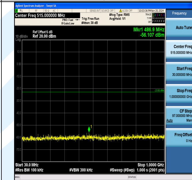
Band66_5MHz_QPSK_132322_1RB#0_30~1000_30~1000
