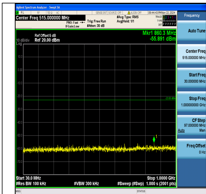
Band66_3MHz_64QAM_132657_1RB#0_30~1000_30~1000
