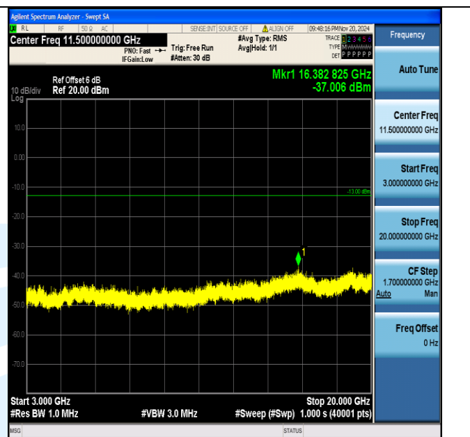
Band66_3MHz_16QAM_131987_1RB#0_3000~20000_3000~20000
