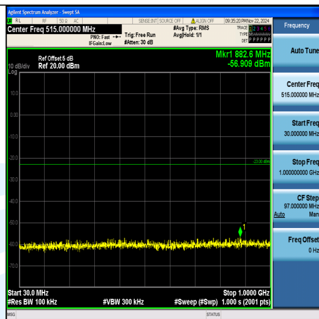
Band66_1.4MHz_64QAM_132665_1RB#0_30~1000_30~1000
