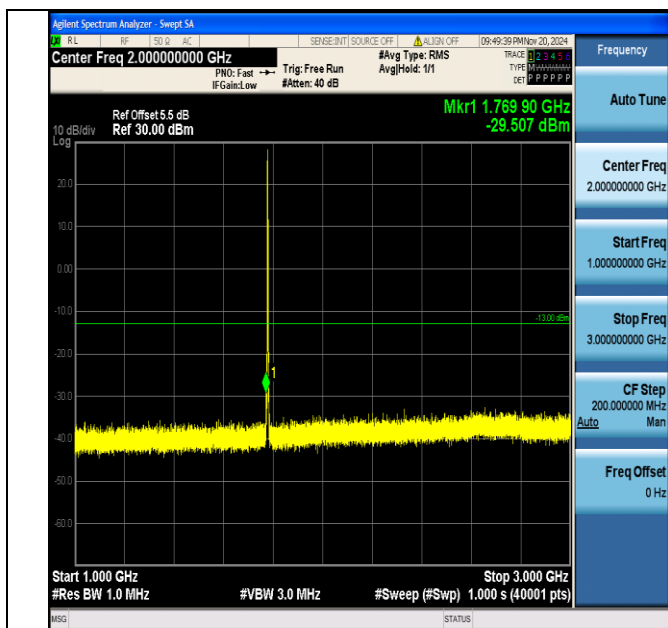
Band66_3MHz_QPSK_132657_1RB#0_1000~3000_1000~3000
