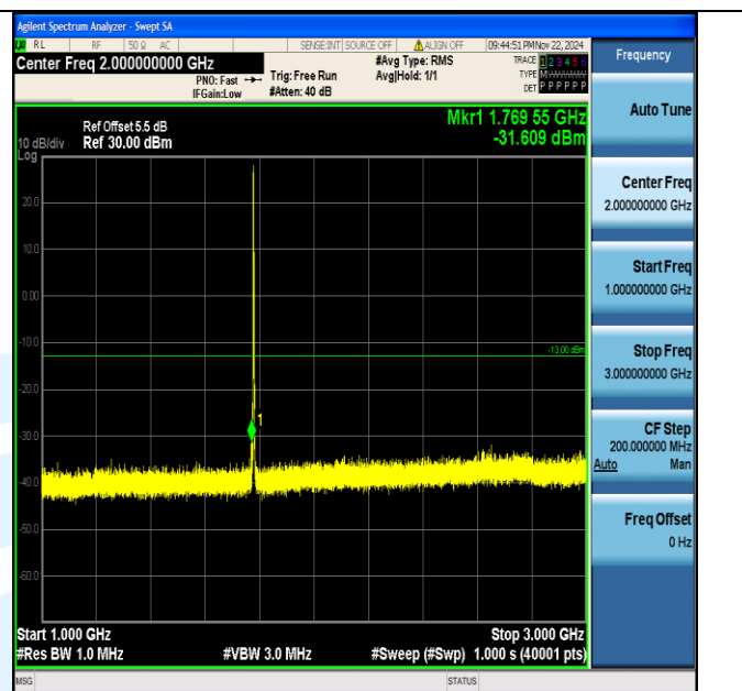
Band66_3MHz_64QAM_132657_1RB#0_1000~3000_1000~3000
