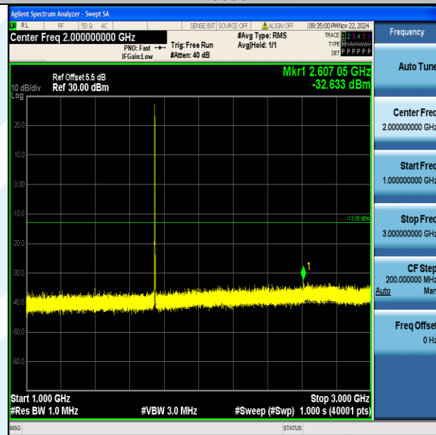
Band66_1.4MHz_64QAM_132322_1RB#0_1000~3000_1000~3000
