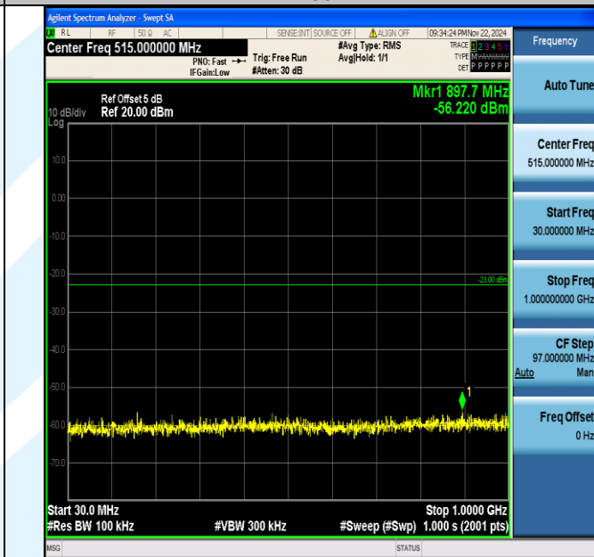
Band66_1.4MHz_64QAM_131979_1RB#0_30~1000_30~1000
