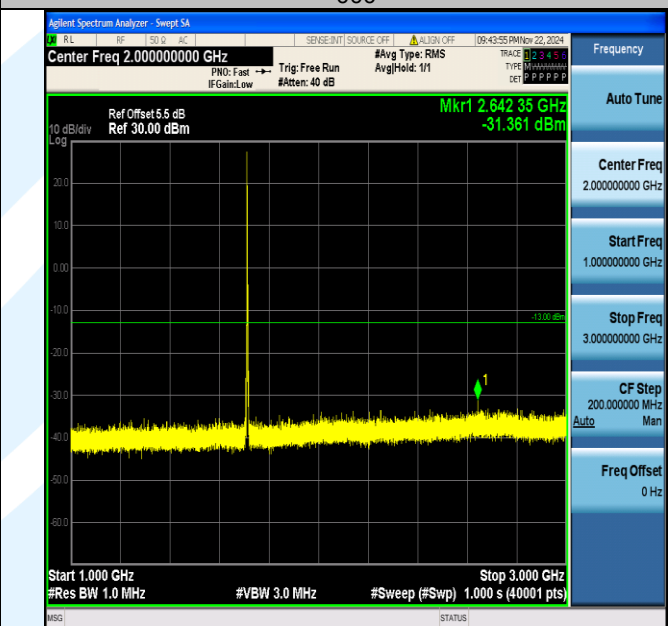
Band66_3MHz_64QAM_131987_1RB#0_1000~3000_1000~3000
