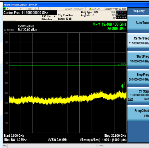
Band66_10MHz_QPSK_132622_1RB#0_3000~20000_3000~20000
