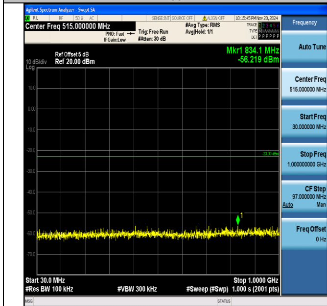
Band66_10MHz_QPSK_132322_1RB#0_30~1000_30~1000
