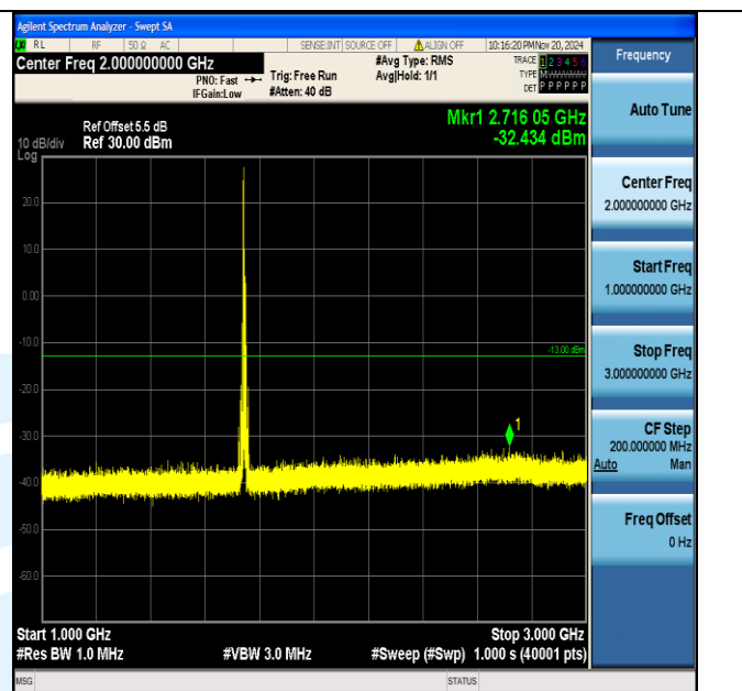
Band66_10MHz_16QAM_132322_1RB#0_1000~3000_1000~3000
