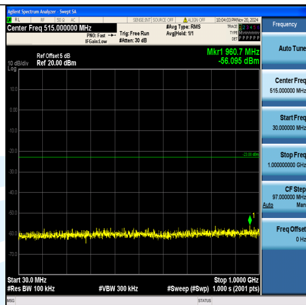
Band66_5MHz_16QAM_132322_1RB#0_30~1000_30~1000
