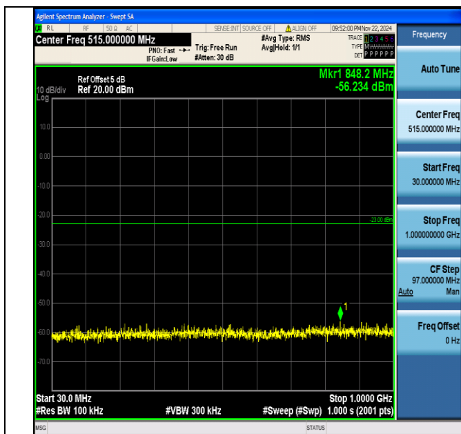
Band66_5MHz_64QAM_132322_1RB#0_30~1000_30~1000
