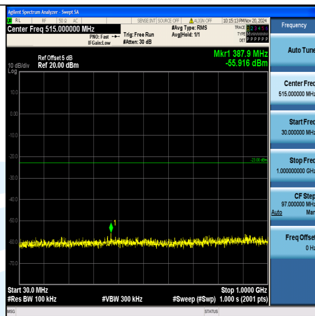
Band66_10MHz_16QAM_132022_1RB#0_30~1000_30~1000
