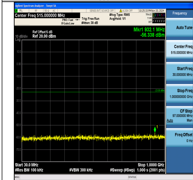
Band66_15MHz_QPSK_132047_1RB#0_30~1000_30~1000
