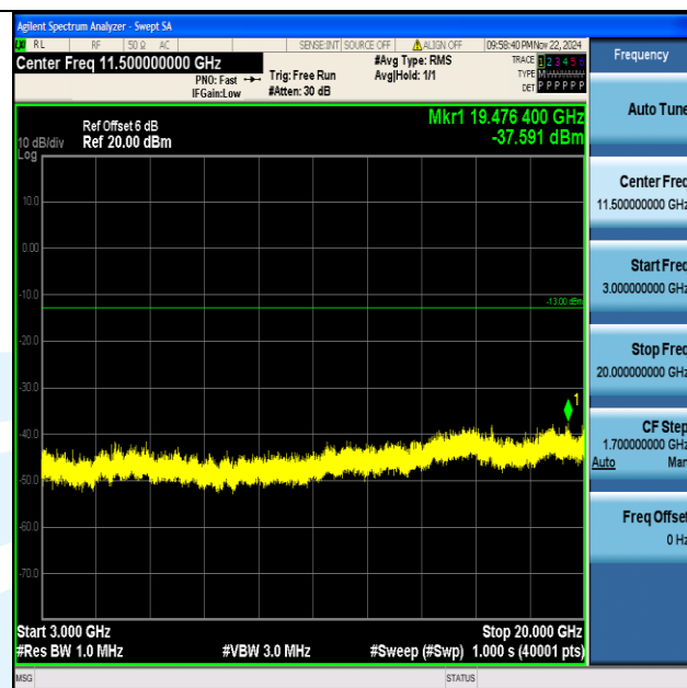
Band66_10MHz_64QAM_132322_1RB#0_3000~20000_3000~20000
