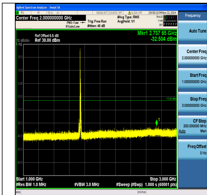
Band66_10MHz_64QAM_132322_1RB#0_1000~3000_1000~3000
