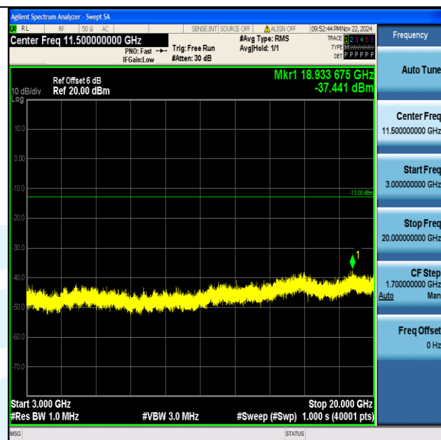
Band66_5MHz_64QAM_132647_1RB#0_3000~20000_3000~20000
