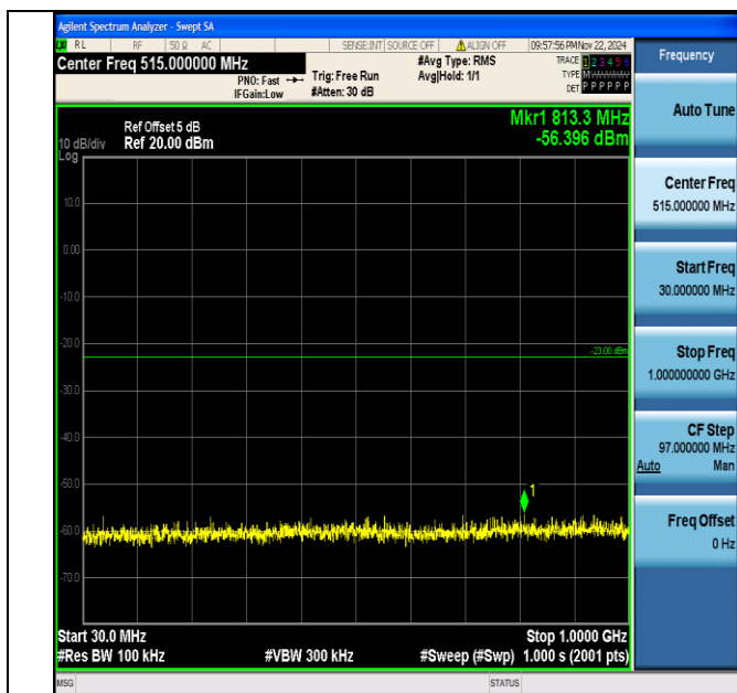
Band66_10MHz_64QAM_132022_1RB#0_30~1000_30~1000
