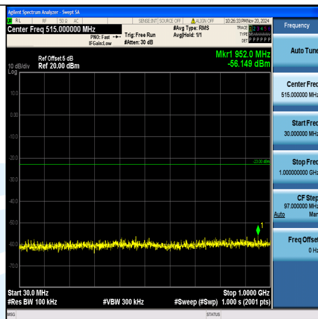
Band66_15MHz_QPSK_132322_1RB#0_30~1000_30~1000
