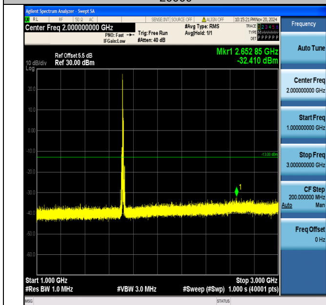
Band66_10MHz_16QAM_132022_1RB#0_1000~3000_1000~3000
