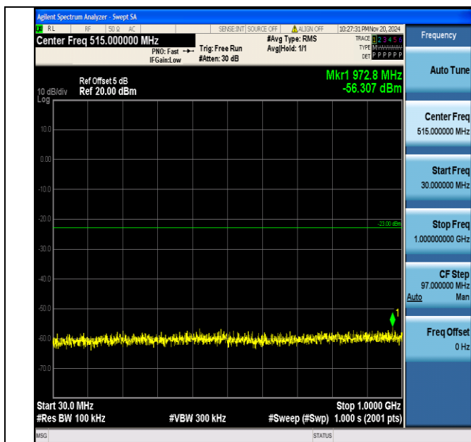
Band66_15MHz_QPSK_132597_1RB#0_30~1000_30~1000
