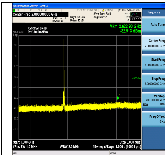
Band66_5MHz_QPSK_132322_1RB#0_1000~3000_1000~3000
