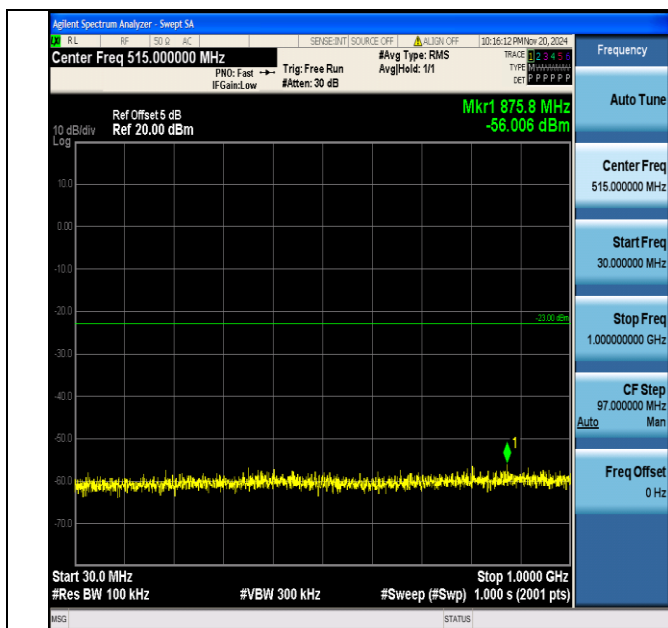
Band66_10MHz_16QAM_132322_1RB#0_30~1000_30~1000
