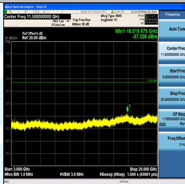
Band66_10MHz_16QAM_132022_1RB#0_3000~20000_3000~20000
