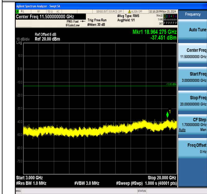
Band66_10MHz_16QAM_132322_1RB#0_3000~20000_3000~20000
