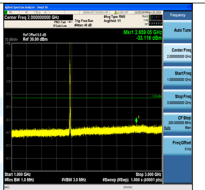
Band66_5MHz_16QAM_132647_1RB#0_1000~3000_1000~3000
