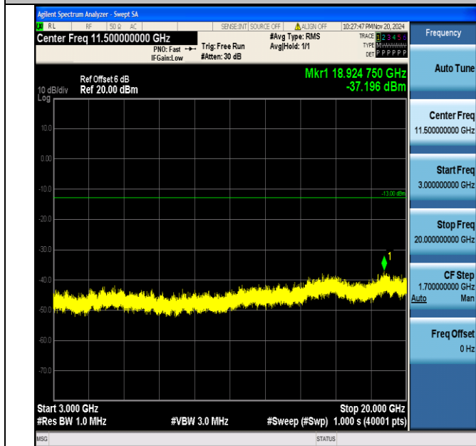
Band66_15MHz_QPSK_132597_1RB#0_3000~20000_3000~20000
