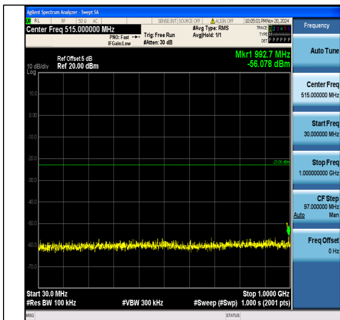
Band66_5MHz_16QAM_132647_1RB#0_30~1000_30~1000
