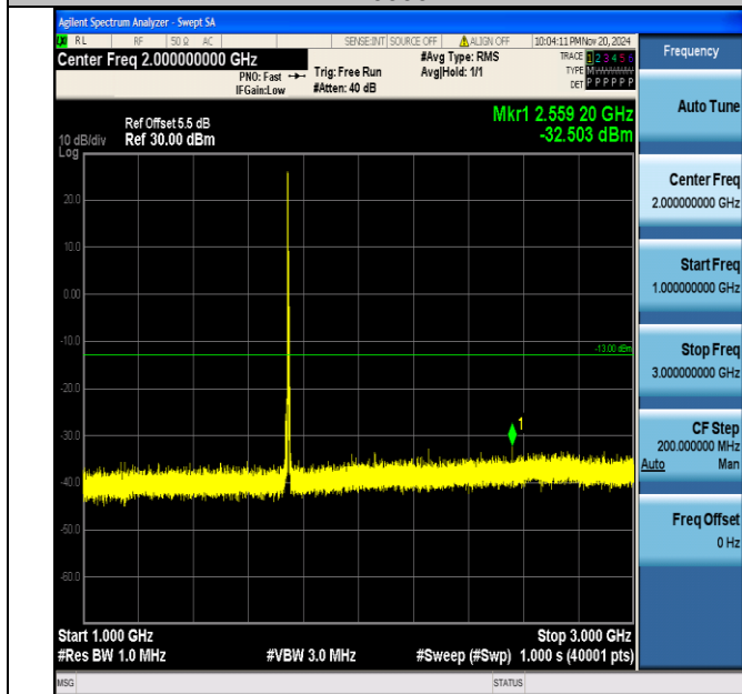
Band66_5MHz_16QAM_132322_1RB#0_1000~3000_1000~3000
