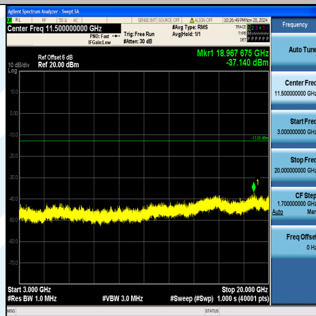
Band66_15MHz_QPSK_132322_1RB#0_3000~20000_3000~20000
