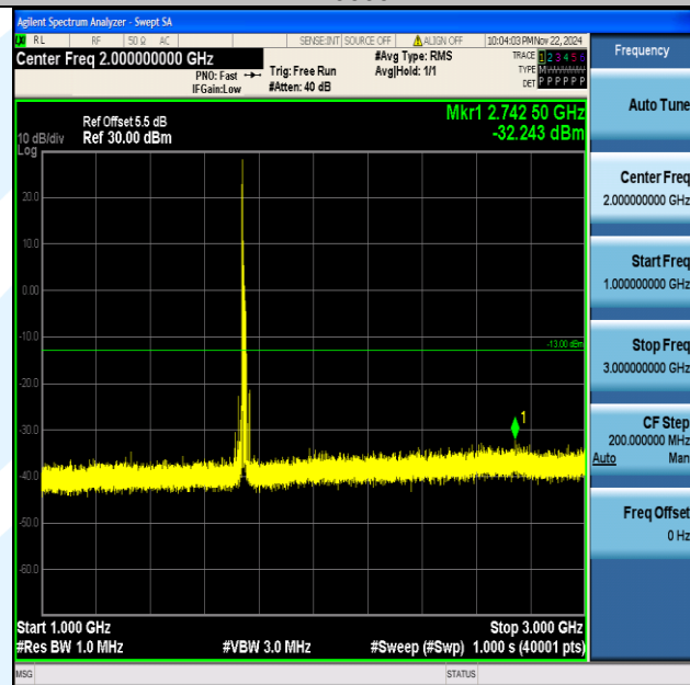
Band66_15MHz_64QAM_132322_1RB#0_1000~3000_1000~3000
