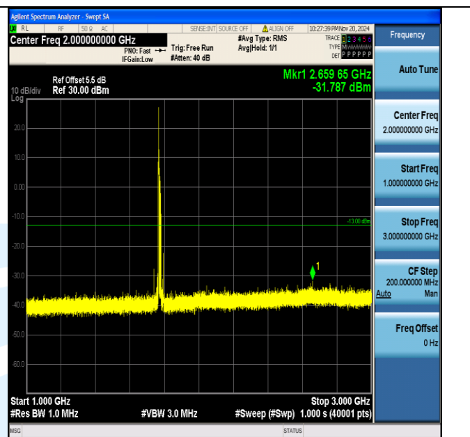
Band66_15MHz_QPSK_132597_1RB#0_1000~3000_1000~3000
