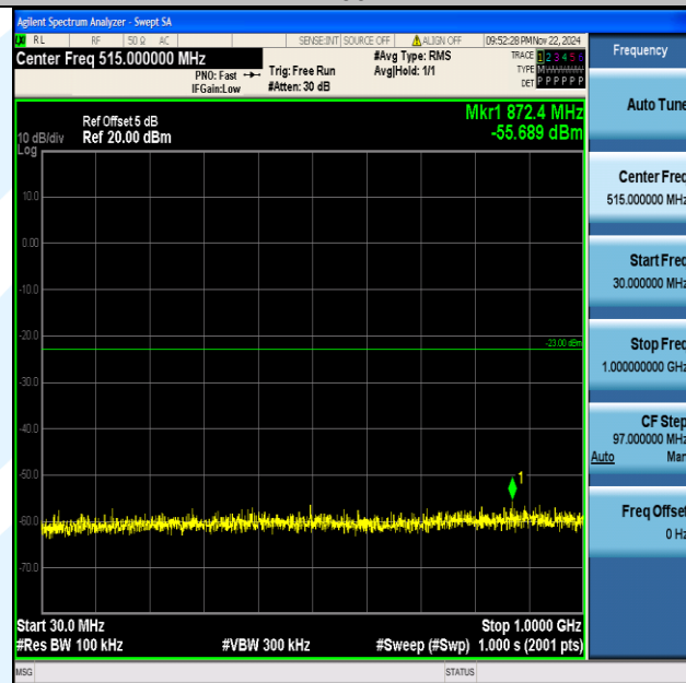
Band66_5MHz_64QAM_132647_1RB#0_30~1000_30~1000
