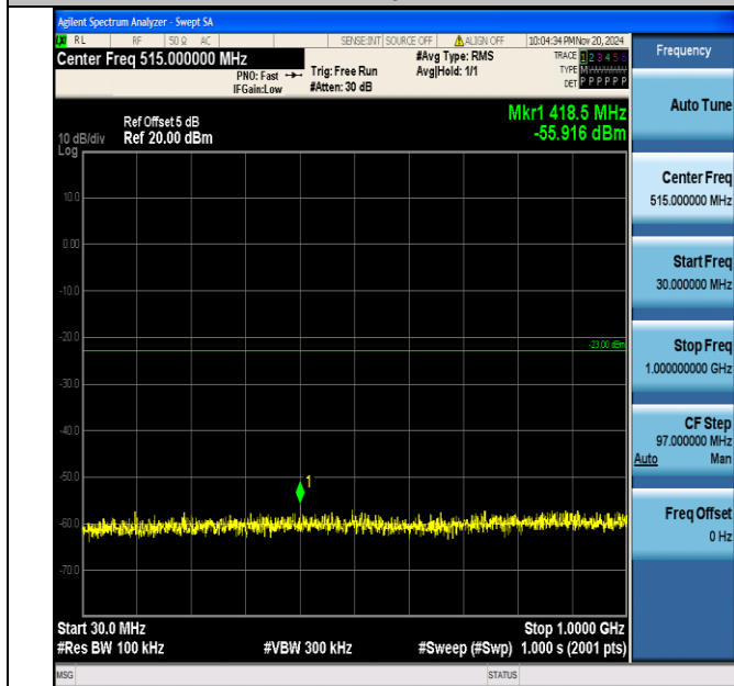
Band66_5MHz_QPSK_132647_1RB#0_30~1000_30~1000
