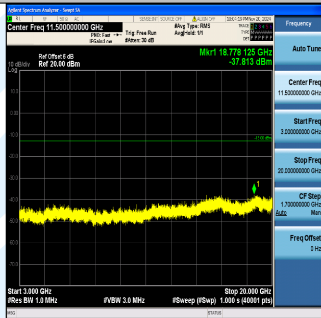
Band66_5MHz_16QAM_132322_1RB#0_3000~20000_3000~20000
