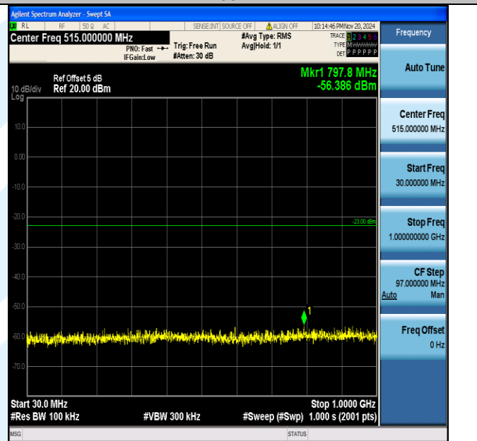
Band66_10MHz_QPSK_132022_1RB#0_30~1000_30~1000
