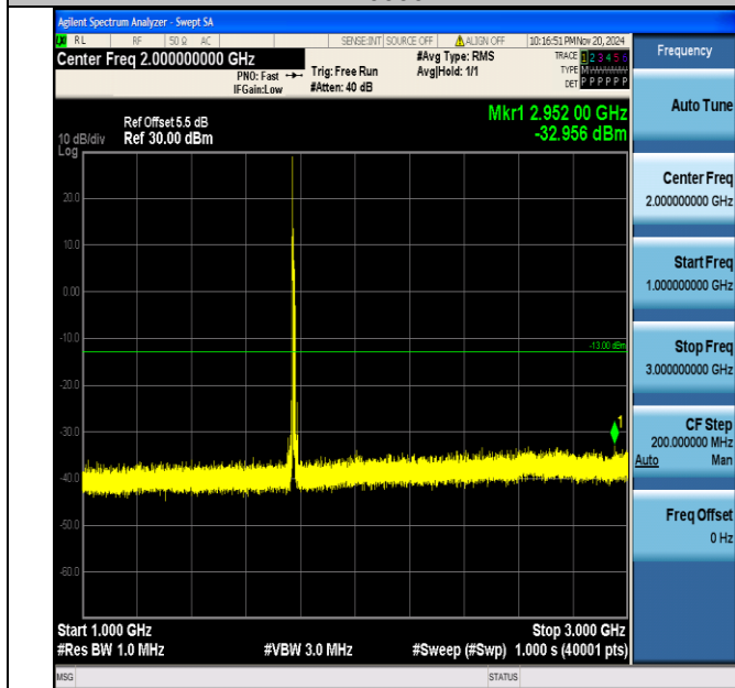
Band66_10MHz_QPSK_132622_1RB#0_1000~3000_1000~3000
