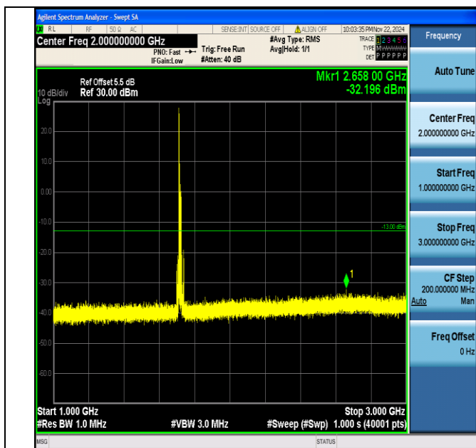
Band66_15MHz_64QAM_132047_1RB#0_1000~3000_1000~3000
