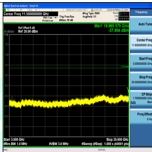
Band66_15MHz_64QAM_132047_1RB#0_3000~20000_3000~20000
