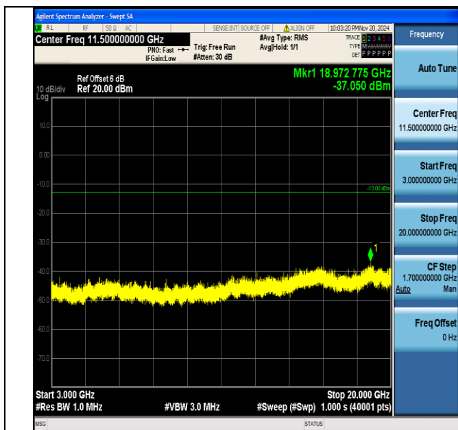
Band66_5MHz_16QAM_131997_1RB#0_3000~20000_3000~20000
