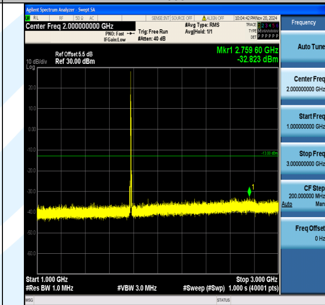
Band66_5MHz_QPSK_132647_1RB#0_1000~3000_1000~3000
