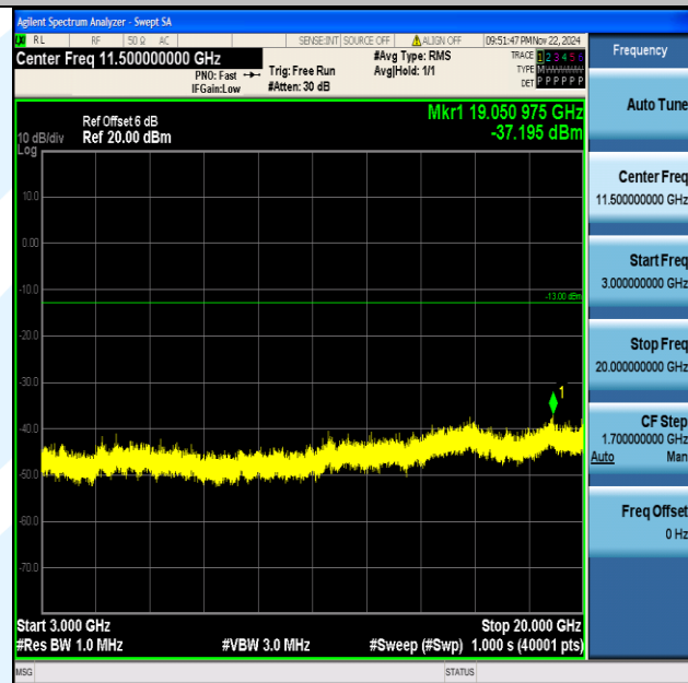
Band66_5MHz_64QAM_131997_1RB#0_3000~20000_3000~20000
