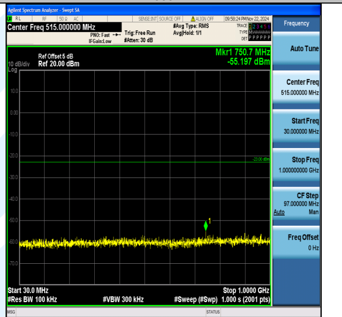
Band66_10MHz_64QAM_132322_1RB#0_30~1000_30~1000
