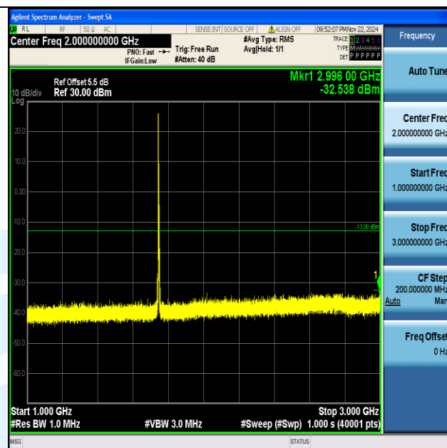
Band66_5MHz_64QAM_132322_1RB#0_1000~3000_1000~3000
