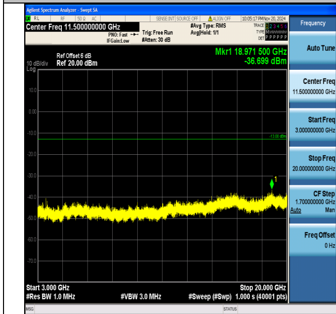
Band66_5MHz_16QAM_132647_1RB#0_3000~20000_3000~20000
