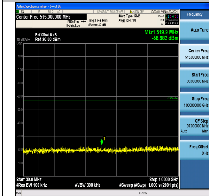
Band66_5MHz_16QAM_131997_1RB#0_30~1000_30~1000
