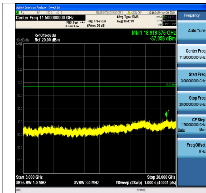
Band66_10MHz_QPSK_132322_1RB#0_3000~20000_3000~20000
