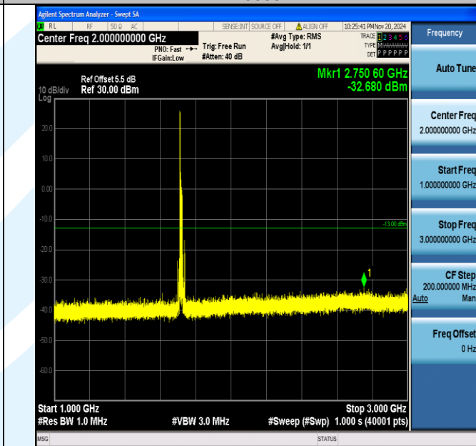
Band66_15MHz_QPSK_132047_1RB#0_1000~3000_1000~3000
