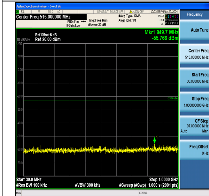
Band66_15MHz_64QAM_132322_1RB#0_30~1000_30~1000
