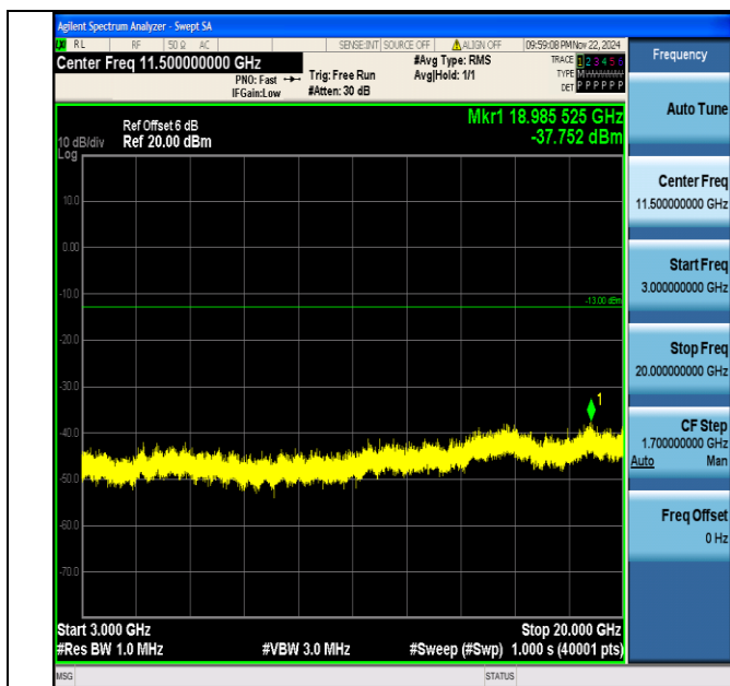
Band66_10MHz_64QAM_132622_1RB#0_3000~20000_3000~20000
