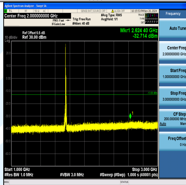
Band66_10MHz_QPSK_132322_1RB#0_1000~3000_1000~3000
