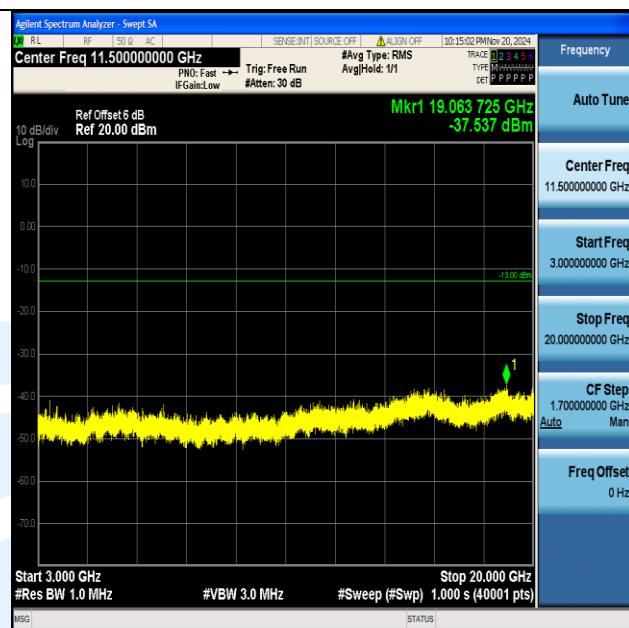
Band66_10MHz_QPSK_132022_1RB#0_3000~20000_3000~20000
