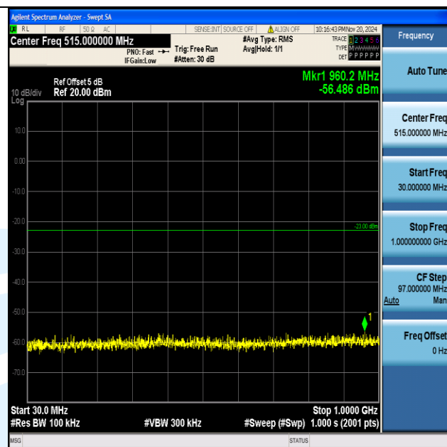
Band66_10MHz_QPSK_132622_1RB#0_30~1000_30~1000
