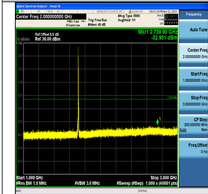
Band66_5MHz_64QAM_131997_1RB#0_1000~3000_1000~3000
