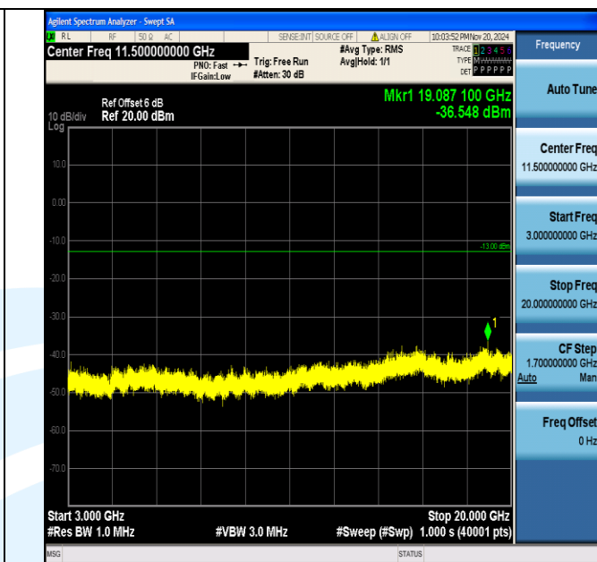
Band66_5MHz_QPSK_132322_1RB#0_3000~20000_3000~20000
