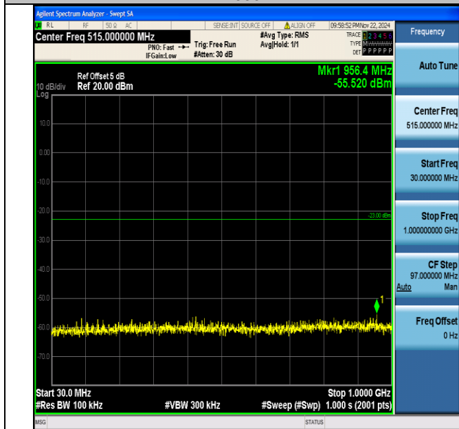
Band66_10MHz_64QAM_132622_1RB#0_30~1000_30~1000
