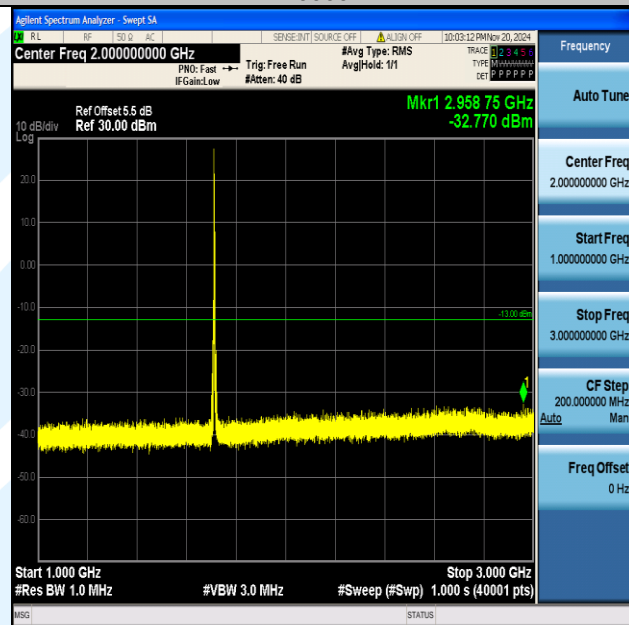
Band66_5MHz_16QAM_131997_1RB#0_1000~3000_1000~3000
