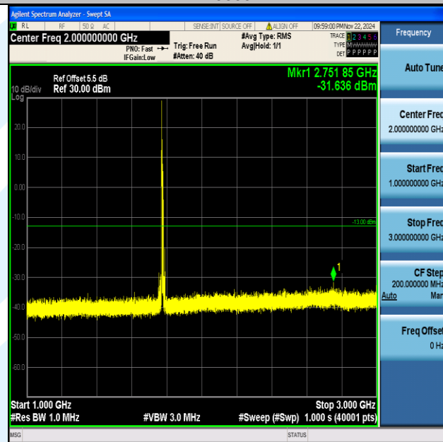
Band66_10MHz_64QAM_132622_1RB#0_1000~3000_1000~3000
