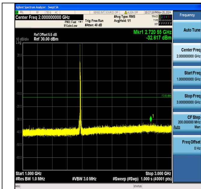
Band66_10MHz_16QAM_132622_1RB#0_1000~3000_1000~3000
