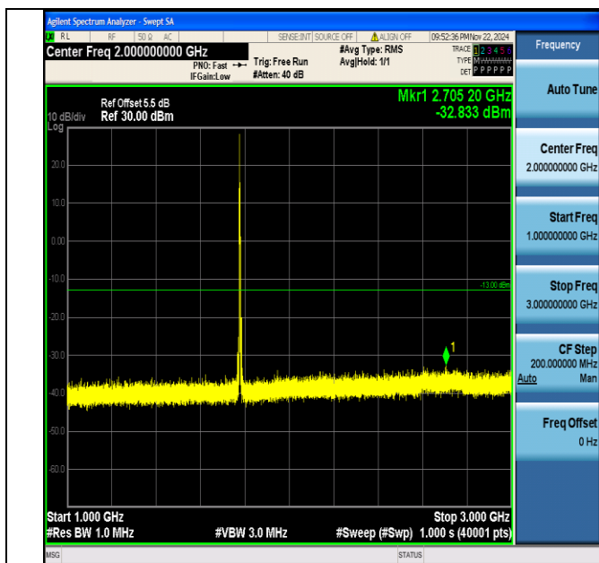
Band66_5MHz_64QAM_132647_1RB#0_1000~3000_1000~3000
