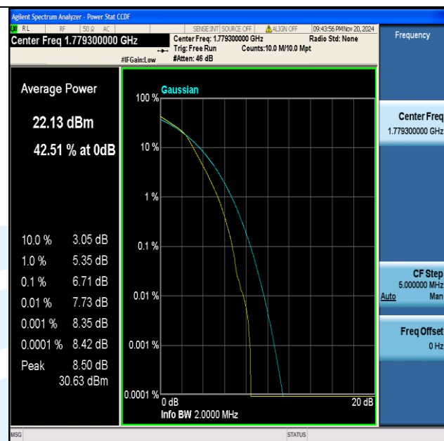
Band66-1.4MHz-16QAM-132665-6RB#0-PASS
