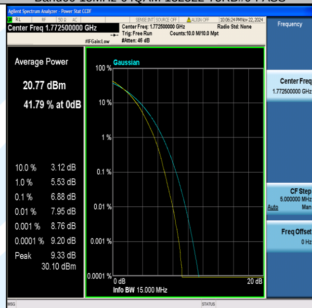
Band66-15MHz-64QAM-132597-75RB#0-PASS
