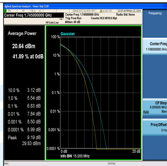
Band66-15MHz-64QAM-132322-75RB#0-PASS
