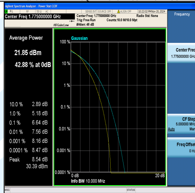
Band66-10MHz-16QAM-132622-50RB#0-PASS
