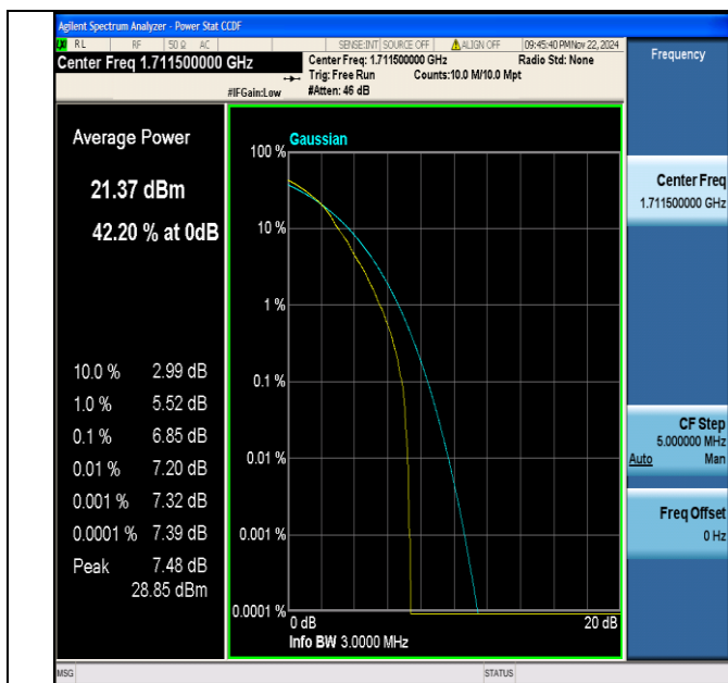
Band66-3MHz-64QAM-131987-1RB#0-PASS
