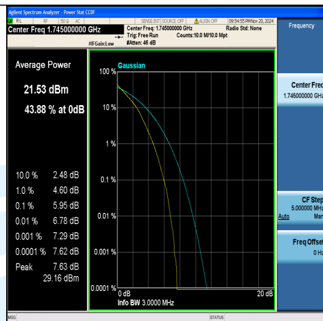
Band66-3MHz-QPSK-132322-15RB#0-PASS
