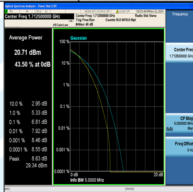
Band66-5MHz-64QAM-131997-25RB#0-PASS
