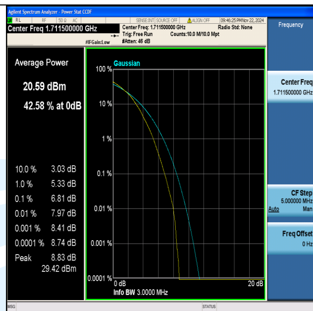
Band66-3MHz-64QAM-131987-15RB#0-PASS
