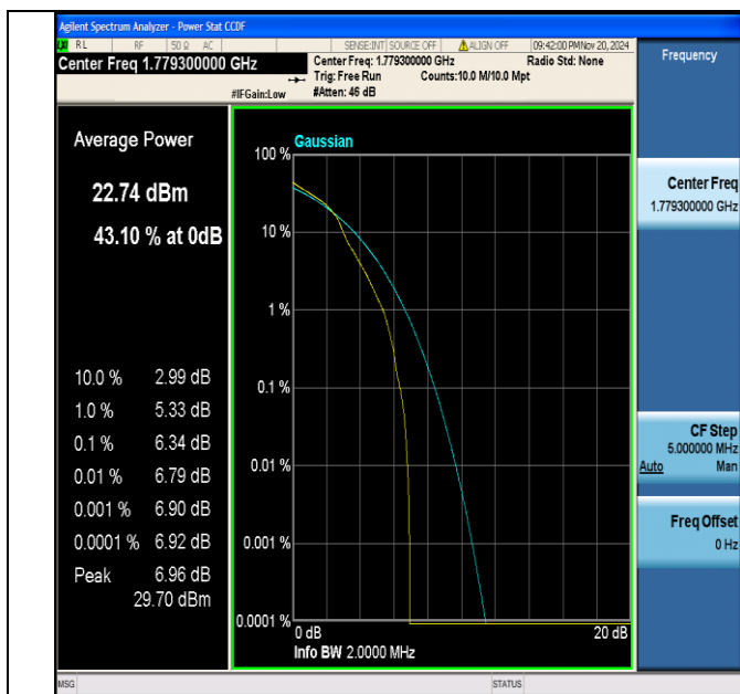
Band66-1.4MHz-16QAM-132665-1RB#0-PASS
