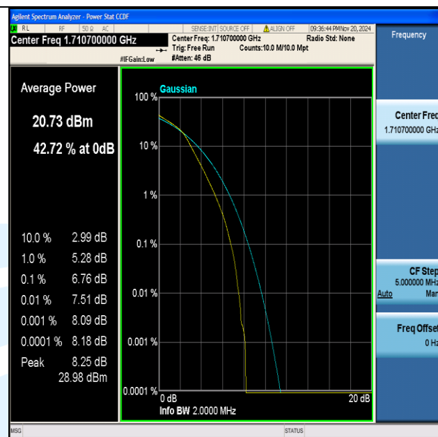
Band66-1.4MHz-16QAM-131979-6RB#0-PASS
