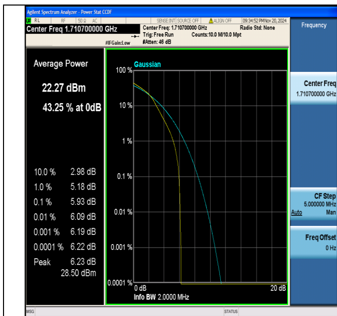
Band66-1.4MHz-16QAM-131979-1RB#0-PASS
