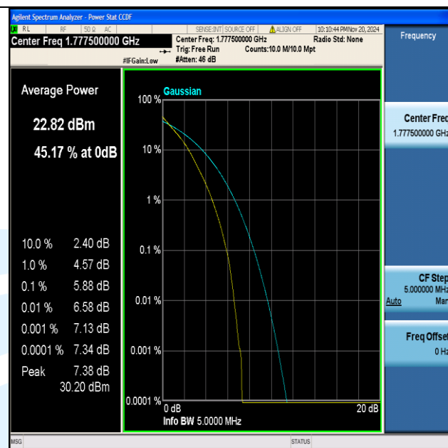
Band66-5MHz-QPSK-132647-25RB#0-PASS
