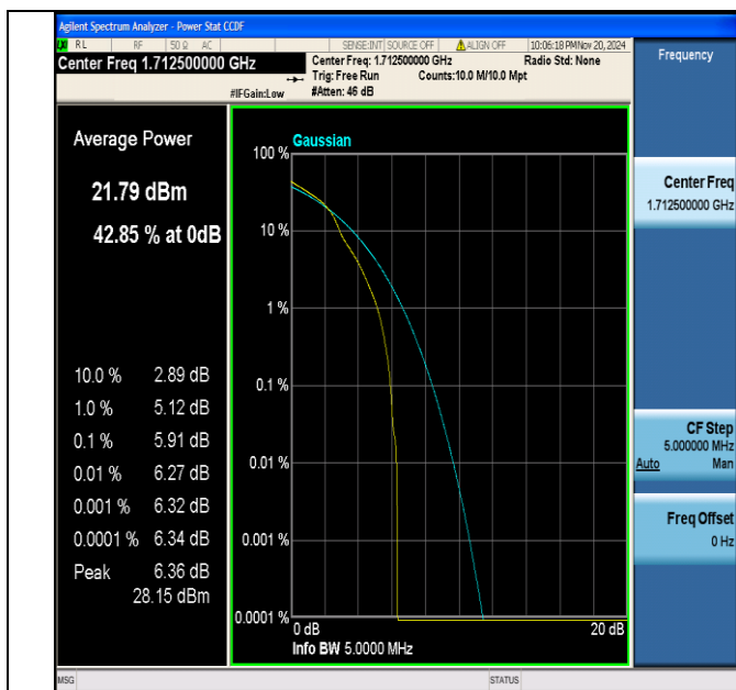
Band66-5MHz-16QAM-131997-1RB#0-PASS
