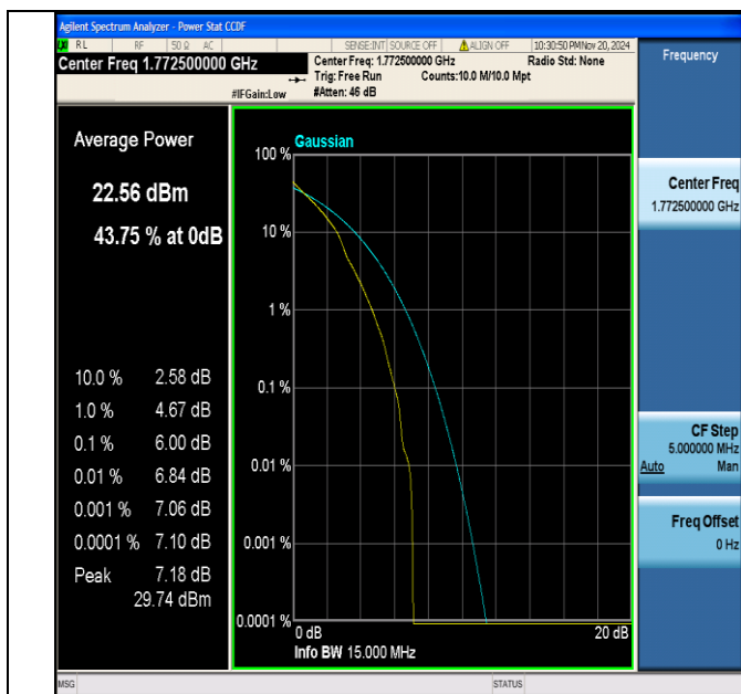
Band66-15MHz-QPSK-132597-1RB#0-PASS
