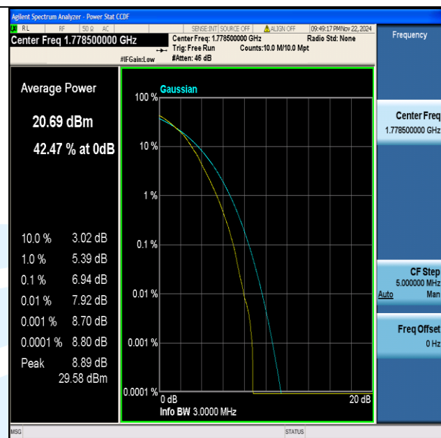
Band66-3MHz-64QAM-132657-15RB#0-PASS
