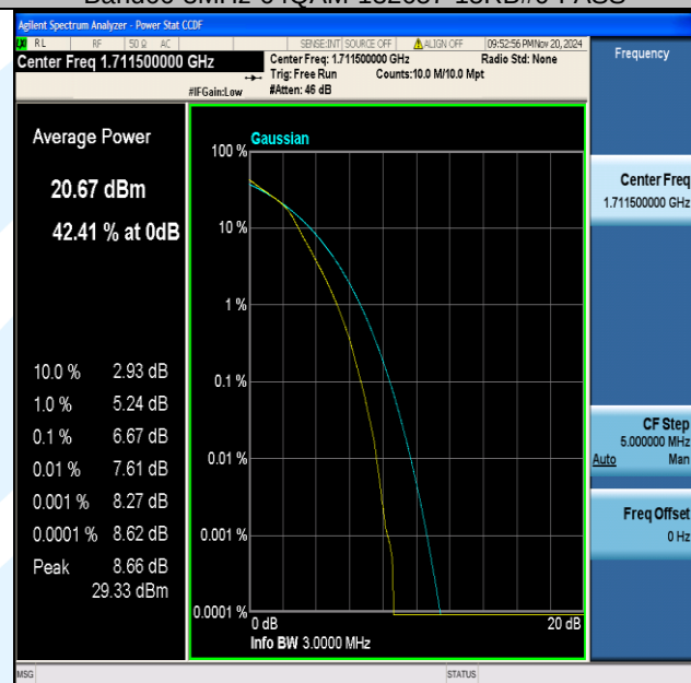
Band66-3MHz-16QAM-131987-15RB#0-PASS
