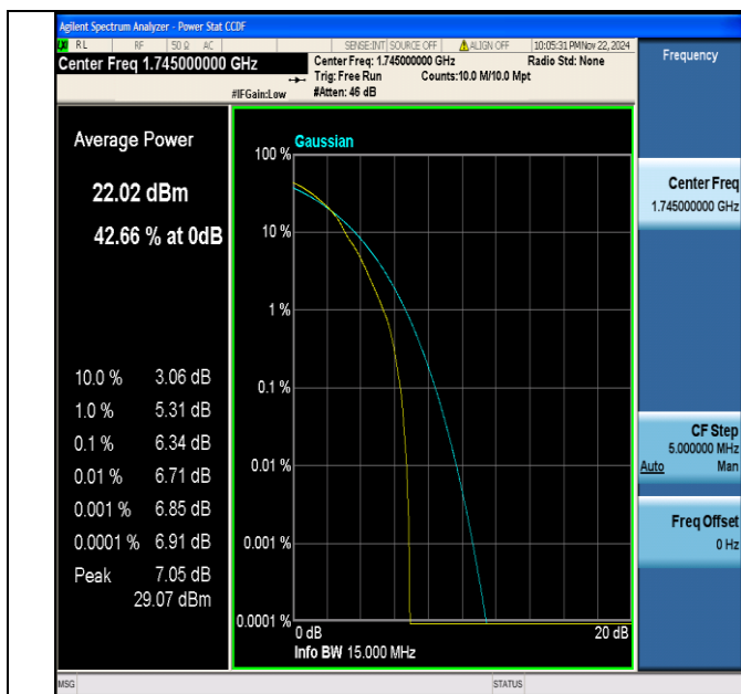
Band66-15MHz-64QAM-132322-1RB#0-PASS
