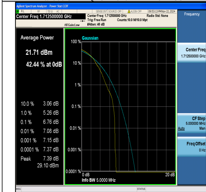
Band66-5MHz-64QAM-131997-1RB#0-PASS
