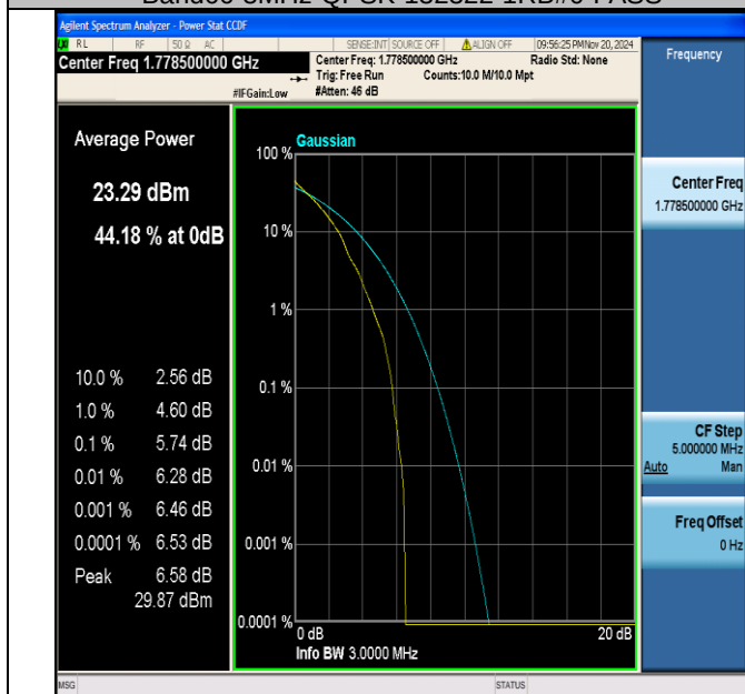
Band66-3MHz-QPSK-132657-1RB#0-PASS
