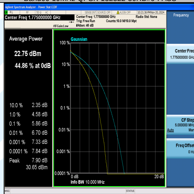
Band66-10MHz-QPSK-132622-50RB#0-PASS
