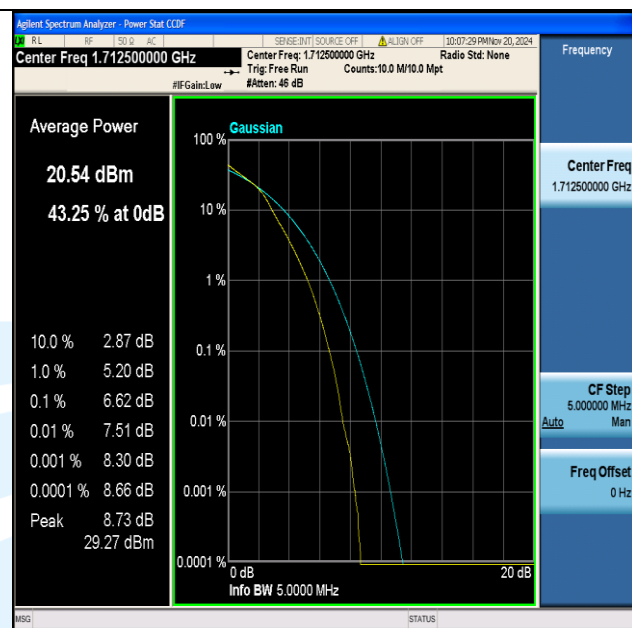
Band66-5MHz-16QAM-131997-25RB#0-PASS
