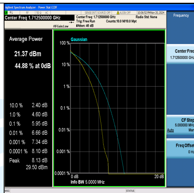
Band66-5MHz-QPSK-131997-25RB#0-PASS
