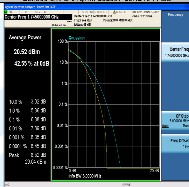
Band66-3MHz-64QAM-132322-15RB#0-PASS
