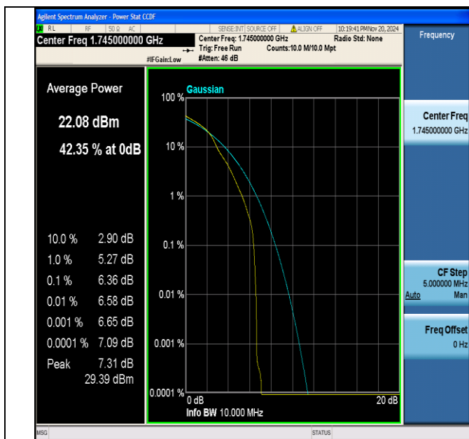
Band66-10MHz-16QAM-132322-1RB#0-PASS
