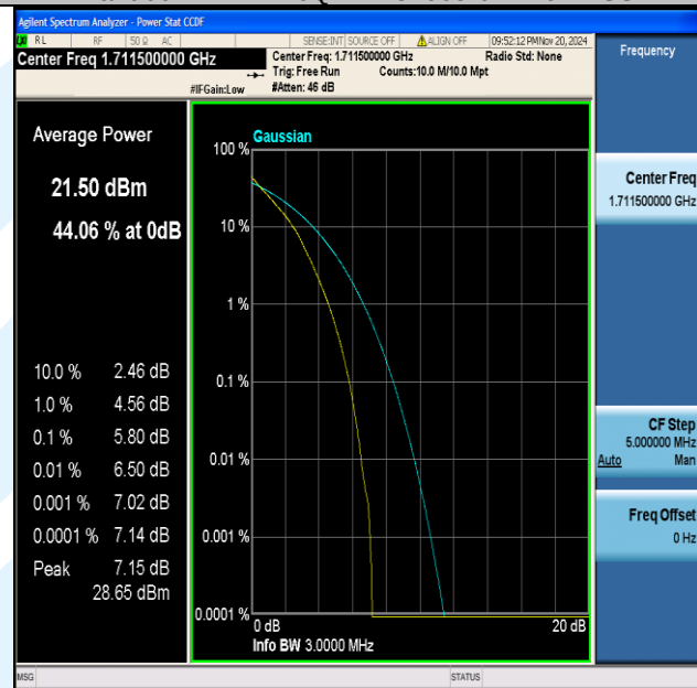
Band66-3MHz-QPSK-131987-15RB#0-PASS
