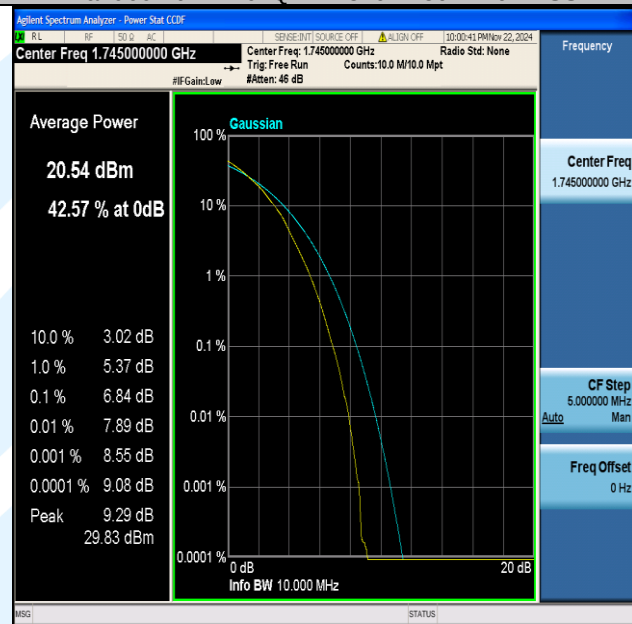
Band66-10MHz-64QAM-132322-50RB#0-PASS
