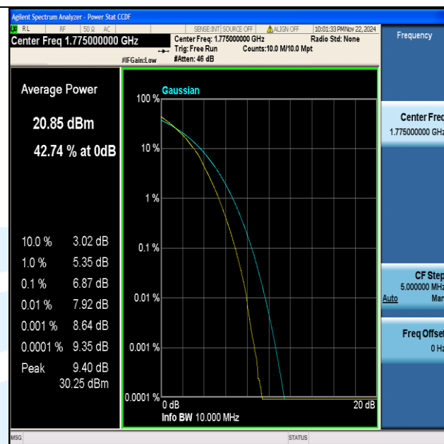
Band66-10MHz-64QAM-132622-50RB#0-PASS
