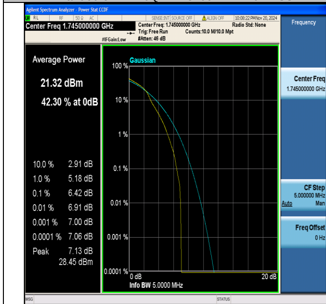
Band66-5MHz-16QAM-132322-1RB#0-PASS
