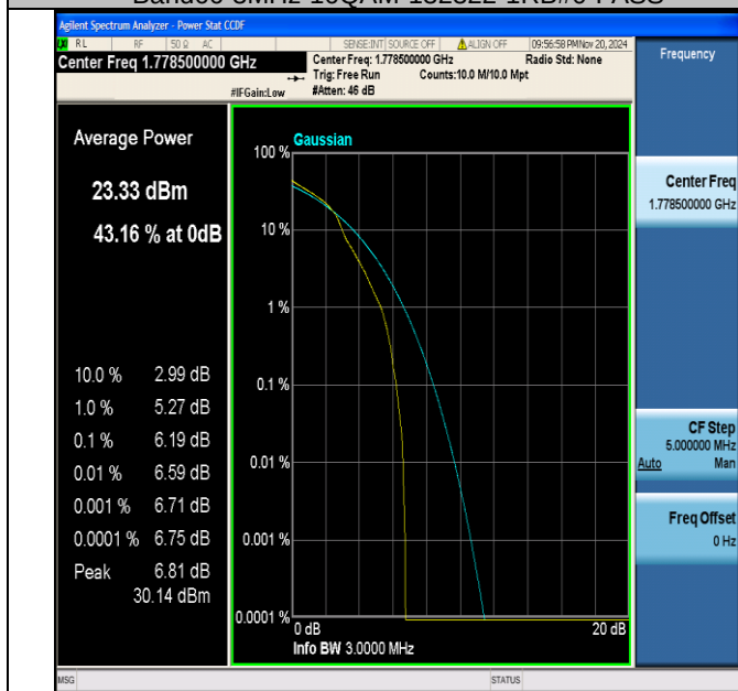
Band66-3MHz-16QAM-132657-1RB#0-PASS
