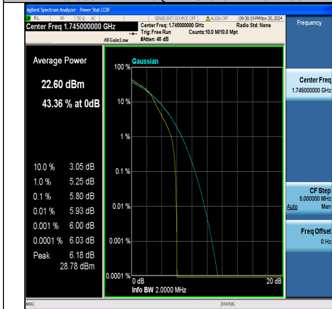
Band66-1.4MHz-16QAM-132322-1RB#0-PASS
