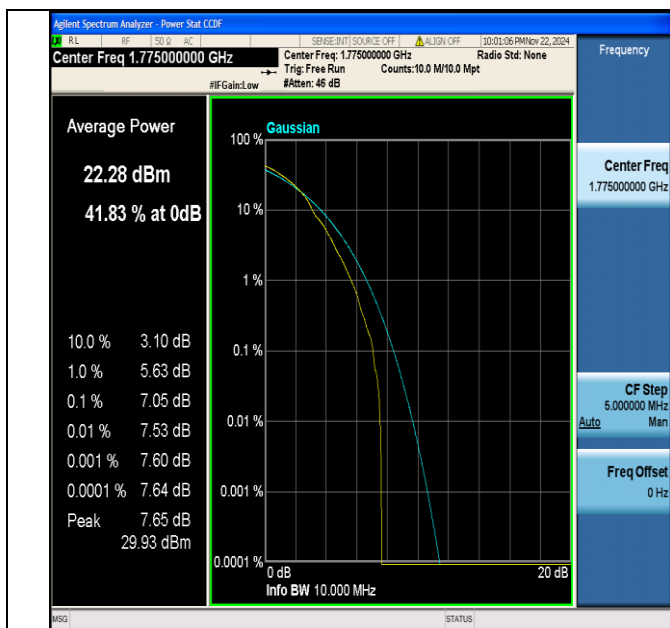
Band66-10MHz-64QAM-132622-1RB#0-PASS
