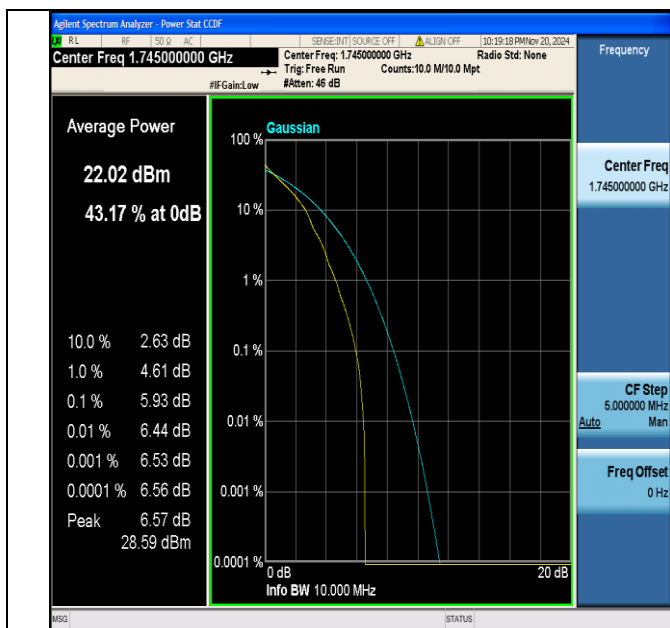
Band66-10MHz-QPSK-132322-1RB#0-PASS
