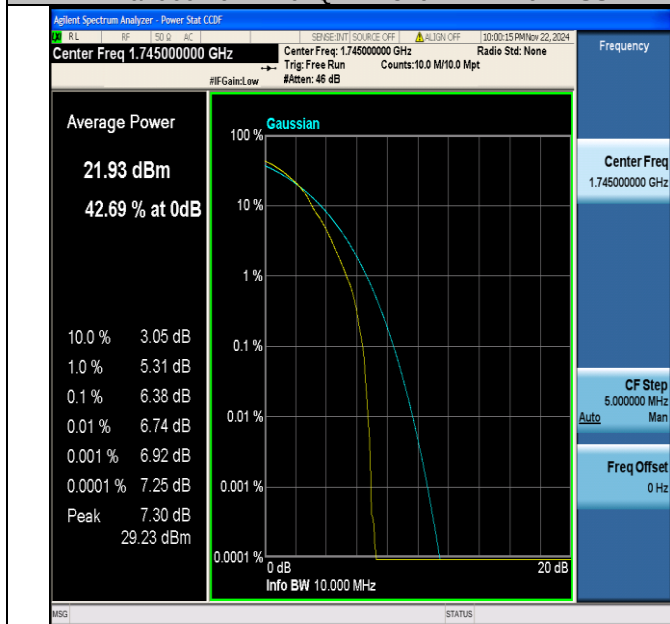
Band66-10MHz-64QAM-132322-1RB#0-PASS
