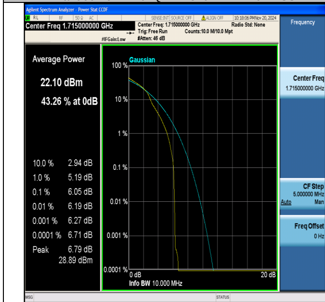
Band66-10MHz-16QAM-132022-1RB#0-PASS
