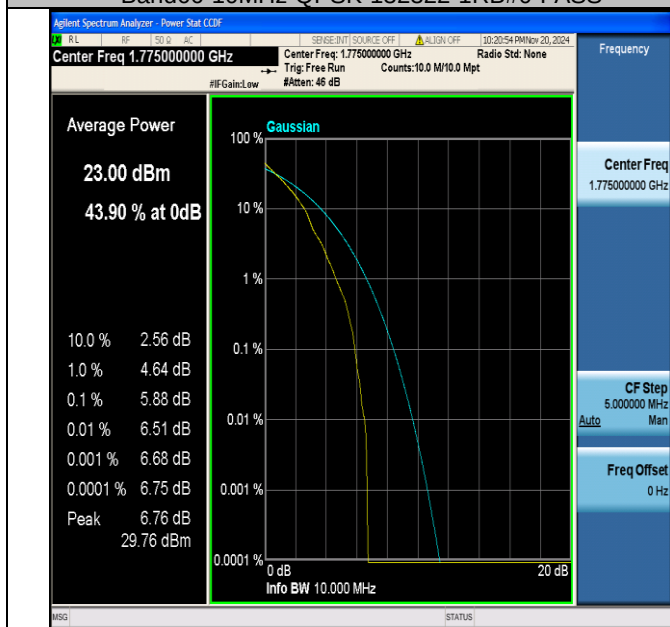
Band66-10MHz-QPSK-132622-1RB#0-PASS
