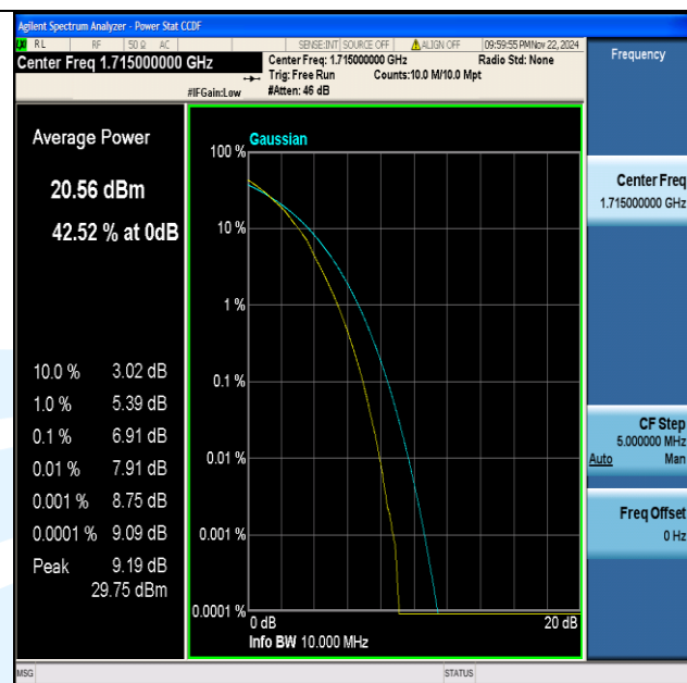
Band66-10MHz-64QAM-132022-50RB#0-PASS
