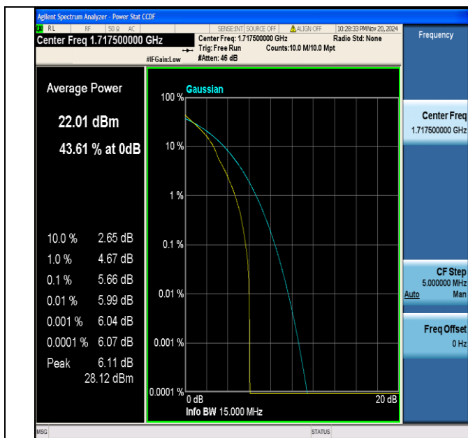
Band66-15MHz-QPSK-132047-1RB#0-PASS
