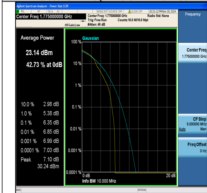
Band66-10MHz-16QAM-132622-1RB#0-PASS
