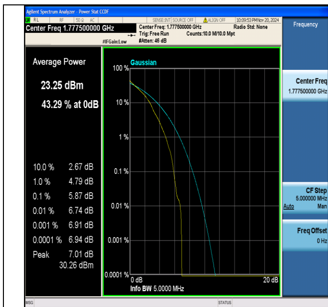
Band66-5MHz-QPSK-132647-1RB#0-PASS
