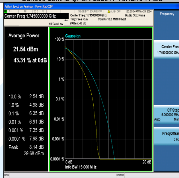
Band66-15MHz-QPSK-132322-75RB#0-PASS
