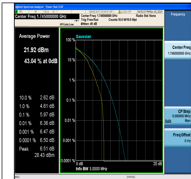
Band66-3MHz-QPSK-132322-1RB#0-PASS
