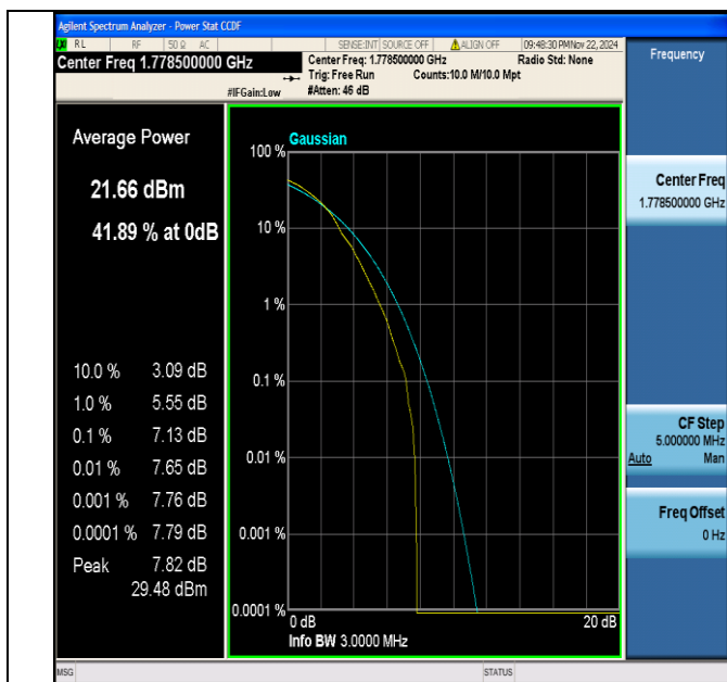
Band66-3MHz-64QAM-132657-1RB#0-PASS
