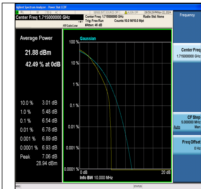
Band66-10MHz-64QAM-132022-1RB#0-PASS
