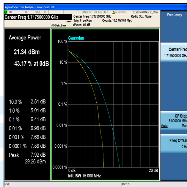
Band66-15MHz-QPSK-132047-75RB#0-PASS
