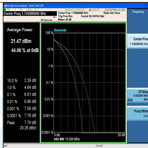
Band66-10MHz-QPSK-132322-50RB#0-PASS
