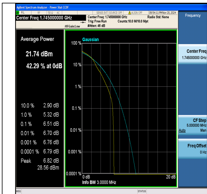
Band66-3MHz-16QAM-132322-1RB#0-PASS
