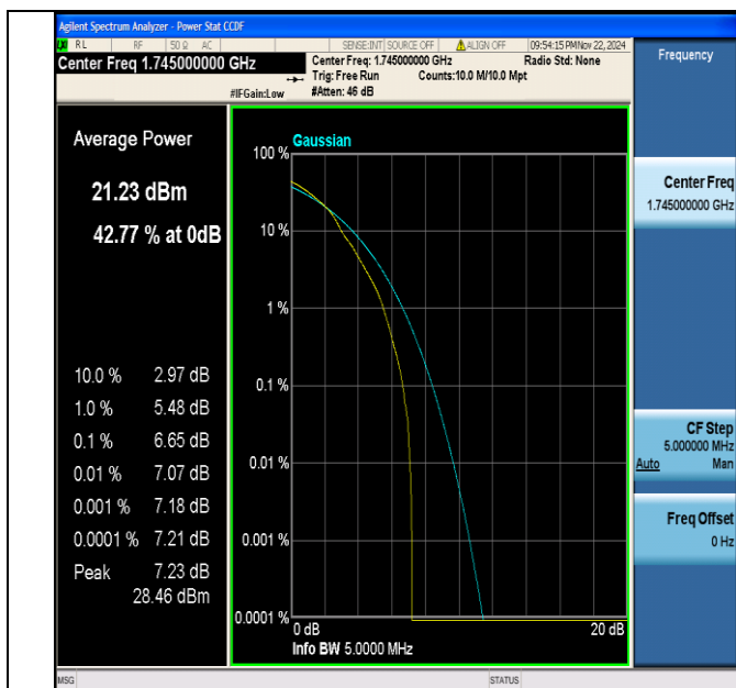
Band66-5MHz-64QAM-132322-1RB#0-PASS
