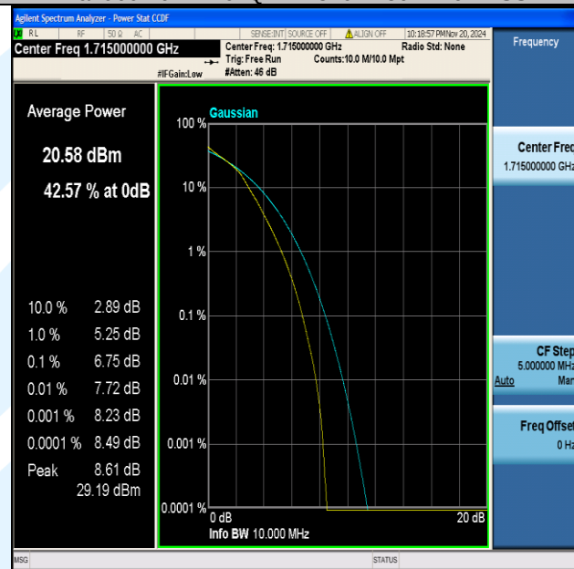
Band66-10MHz-16QAM-132022-50RB#0-PASS
