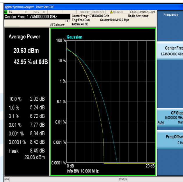
Band66-10MHz-16QAM-132322-50RB#0-PASS
