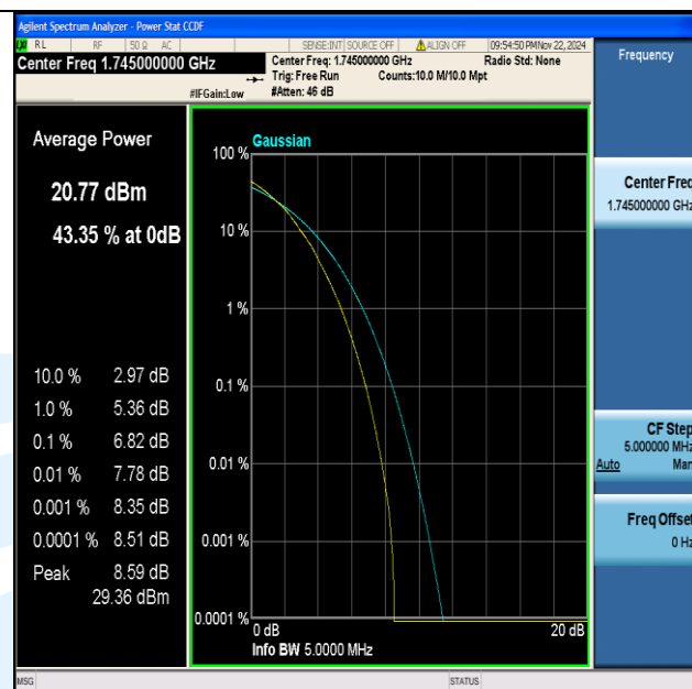
Band66-5MHz-64QAM-132322-25RB#0-PASS
