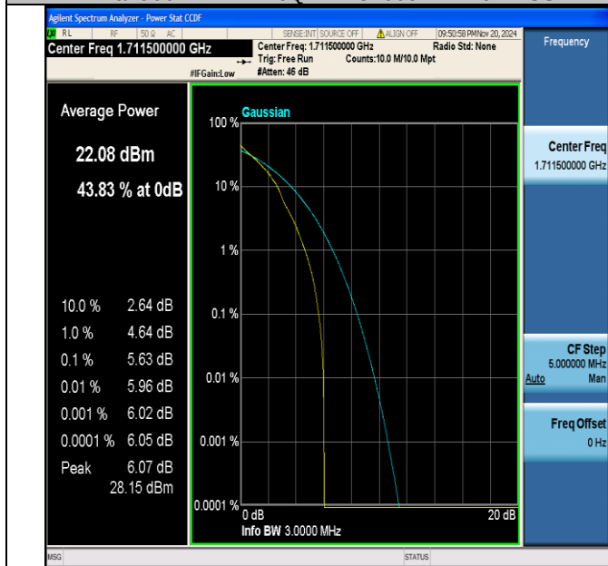
Band66-3MHz-QPSK-131987-1RB#0-PASS
