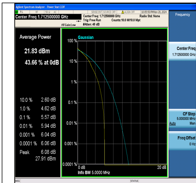
Band66-5MHz-QPSK-131997-1RB#0-PASS
