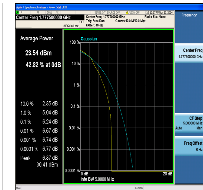
Band66-5MHz-16QAM-132647-1RB#0-PASS
