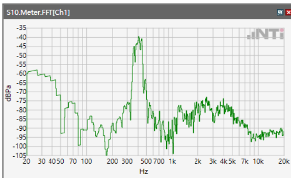
ANSI/TIA 5050-2018 \ 8N HAC OFF \ WB 23.85 kbps\ 5.2 Receive path – distortion and noise\ LTE BAND 71
