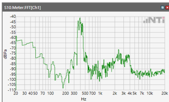
ANSI/TIA 5050-2018 \ 8N HAC OFF \ NB 12.2kbps\ 5.2 Receive path – distortion and noise\ WLAN 2.4GHz
