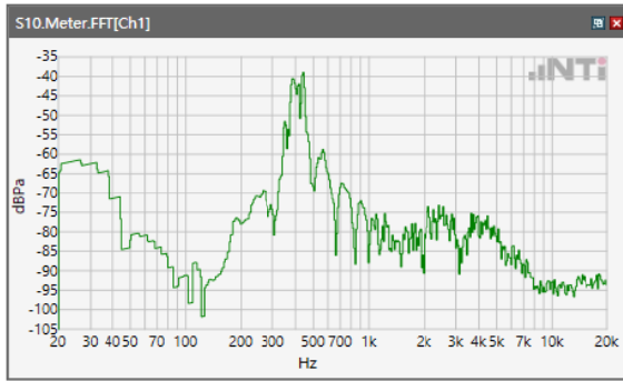
ANSI/TIA 5050-2018 \ 8N HAC OFF \ WB 23.85 kbps\ 5.2 Receive path – distortion and noise\ LTE Band 66
