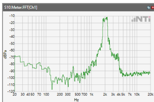
ANSI/TIA 5050-2018 \ 2N HAC ON \ NB 12.2kbps\ 5.2 Receive path – distortion and noise\WCDMA Band V
