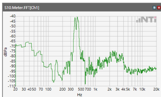
ANSI/TIA 5050-2018 \ 2N HAC ON \ NB 12.2kbps\ 5.2 Receive path – distortion and noise\LTE Band 12
