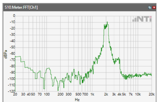
ANSI/TIA 5050-2018 \ 2N HAC ON \ NB 12.2kbps\ 5.2 Receive path – distortion and noise\WCDMA Band V
