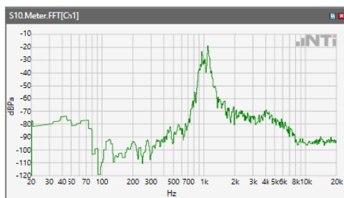
ANSI/TIA 5050-2018 \ 2N HAC ON \ NB 12.2kpbs\ 5.2 Receive path – distortion and noise\LTE Band 66
