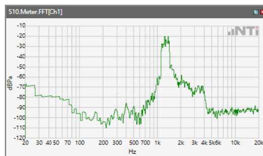
ANSI/TIA 5050-2018 \ 8N HAC OFF \ WB 23.85 kbps \ 5.2 Receive path – distortion and noise\ LTE Band 12
