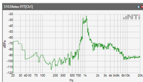
ANSI/TIA 5050-2018 \ 2N HAC ON \ NB 12.2kpbs\ 5.2 Receive path – distortion and noise\WLAN 2.4GHz
