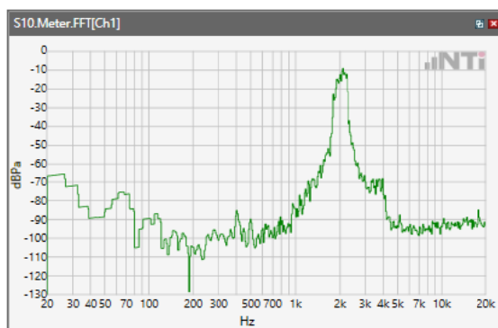
ANSI/TIA 5050-2018 \ 2N HAC ON \ NB 12.2kbps\ 5.2 Receive path – distortion and noise\LTE Band 2
