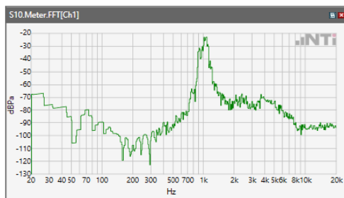
ANSI/TIA 5050-2018 \ 2N HAC ON \ NB 12.2kpbs\ 5.2 Receive path – distortion and noise\LTE BAND 71
