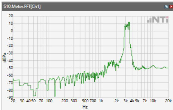
ANSI/TIA 5050-2018 \ 8N HAC OFF \ WB 23.85 kbps\ 5.2 Receive path – distortion and noise\WLAN 2.4GHz
