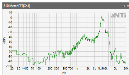
ANSI/TIA 5050-2018 \ 8N HAC OFF \ WB 23.85 kbps\ 5.2 Receive path – distortion and noise\ LTE Band 7
