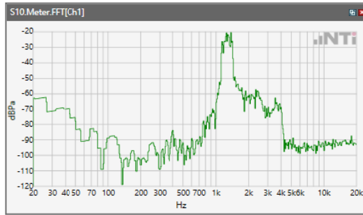
ANSI/TIA 5050-2018 \ 8N HAC OFF \ WB 23.85 kbps \ 5.2 Receive path – distortion and noise\LTE Band 5
