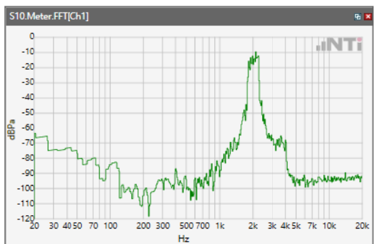
ANSI/TIA 5050-2018 \ 2N HAC ON \ NB 12.2kbps\ 5.2 Receive path – distortion and noise\LTE Band 5
