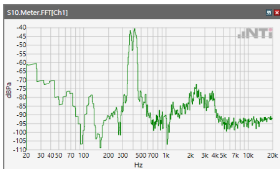
ANSI/TIA 5050-2018 \ 2N HAC ON \ NB 12.2kbps\ 5.2 Receive path – distortion and noise\LTE Band 7
