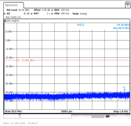
Band66-3MHz-16QAM-132322-1RB#0-30~1000-P ASS
