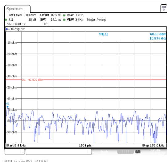
Band66-3MHz-16QAM-132322-1RB#0-0.009~0.15 -PASS
