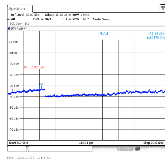
Band66-3MHz-QPSK-132322-1RB#0-3000~2000 0-PASS
