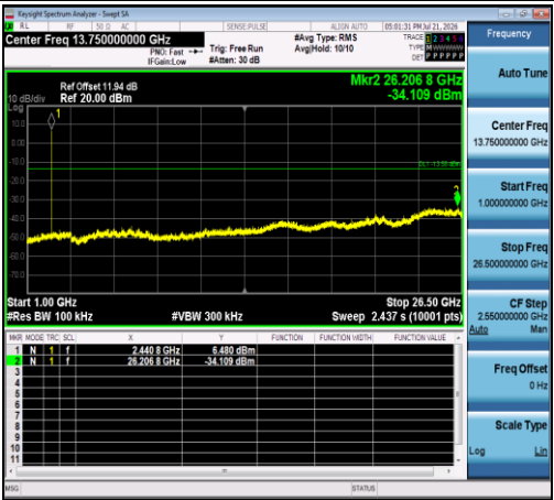
DH5-Ant1-2441-1000~26500-PASS
