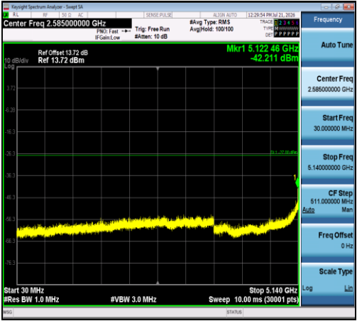
11AC20SISO-Ant1-5200-30~5140-PASS
