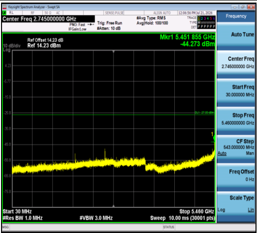
11N40SISO-Ant1-5550-30~5460-PASS
