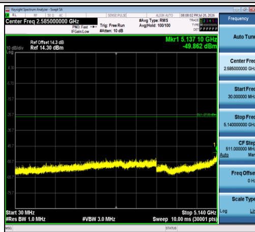
11A-Ant1-5320-30~5140-PASS
