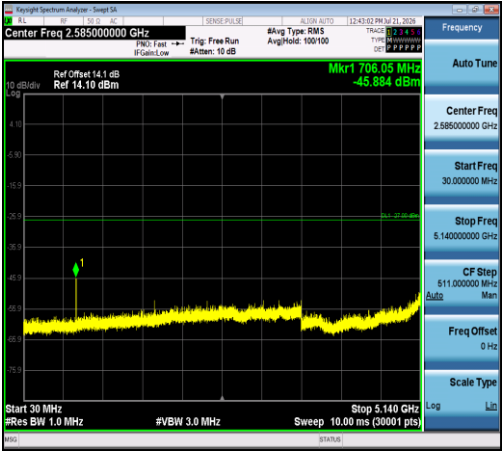
11AC20SISO-Ant1-5280-30~5140-PASS
