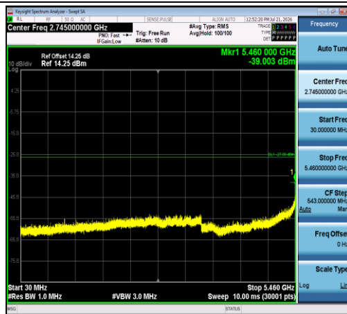
11AC20SISO-Ant1-5500-30~5460-PASS
