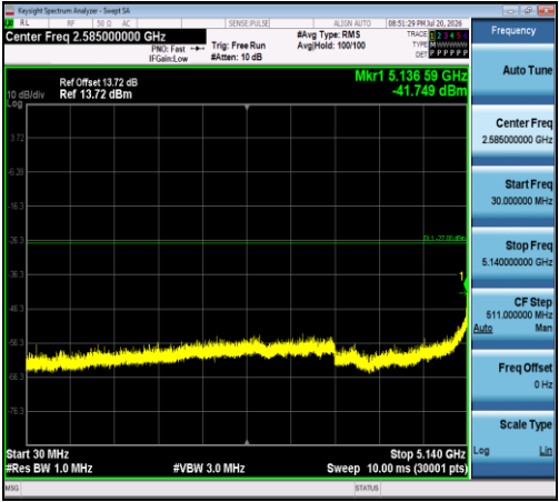
11N20SISO-Ant1-5200-30~5140-PASS
