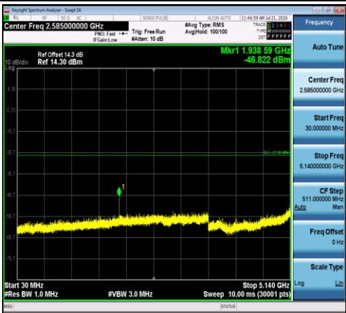
11N40SISO-Ant1-5310-30~5140-PASS
