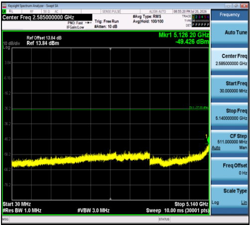
11N20SISO-Ant1-5240-30~5140-PASS
