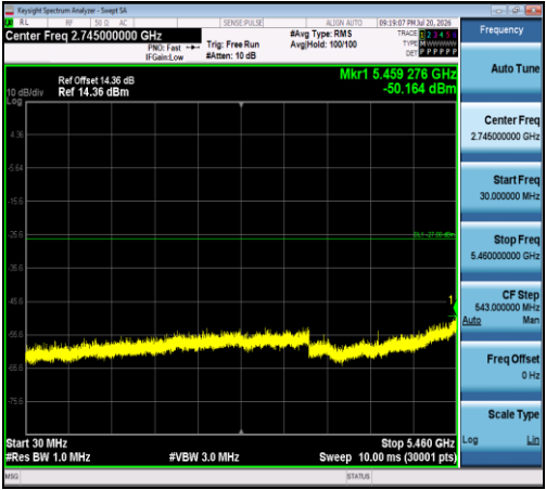
11N20SISO-Ant1-5580-30~5460-PASS
