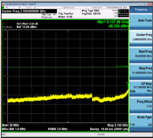
11A-Ant1-5240-30~5140-PASS
