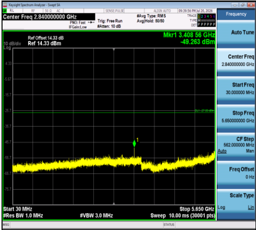
11N20SISO-Ant1-5785-30~5650-PASS
