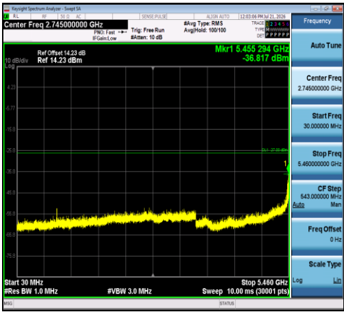
11N40SISO-Ant1-5510-30~5460-PASS
