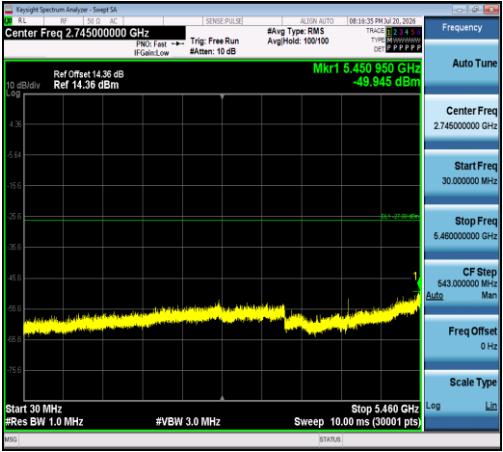
11A-Ant1-5580-30~5460-PASS
