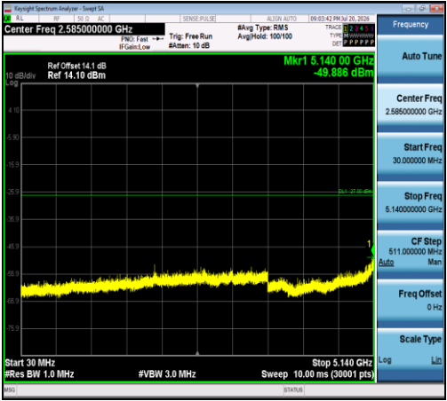
11N20SISO-Ant1-5280-30~5140-PASS
