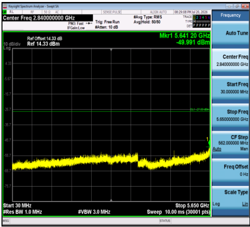
11A-Ant1-5785-30~5650-PASS
