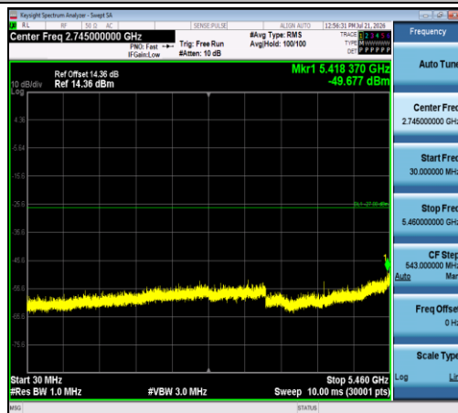
11AC20SISO-Ant1-5580-30~5460-PASS
