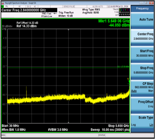
11N40SISO-Ant1-5755-30~5650-PASS
