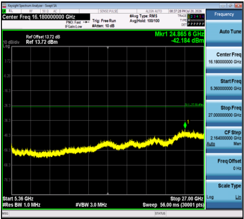
11N20SISO-Ant1-5180-5360~40000-PASS
