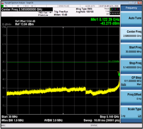
11N40SISO-Ant1-5230-30~5140-PASS
