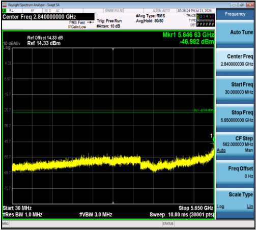
11AC40SISO-Ant1-5755-30~5650-PASS
