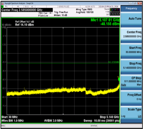
11AC40SISO-Ant1-5270-30~5140-PASS
