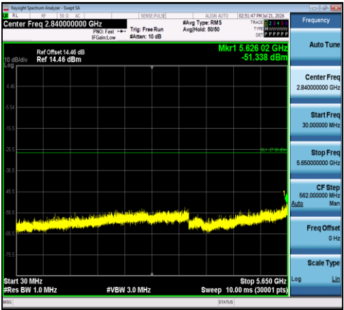
11AC20SISO-Ant1-5825-30~5650-PASS
