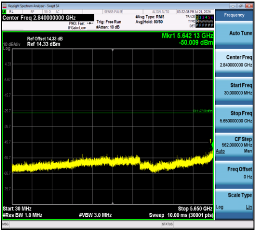
11AC40SISO-Ant1-5795-30~5650-PASS
