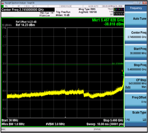
11AC40SISO-Ant1-5510-30~5460-PASS
