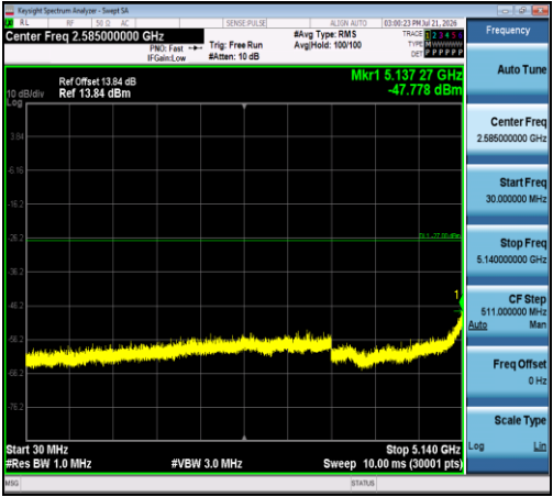
11AC40SISO-Ant1-5230-30~5140-PASS
