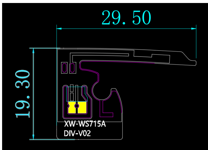
Dimensional drawing of diversity antenna
