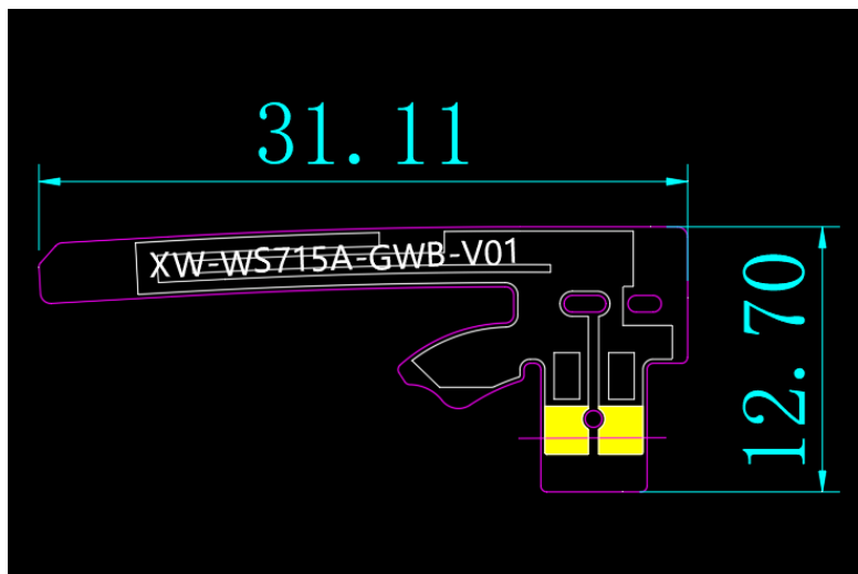
Dimensional drawing of diversity antenna
